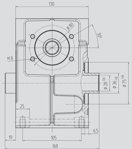
Fig. 2 Output shaft for clamp connection 80 84 136
