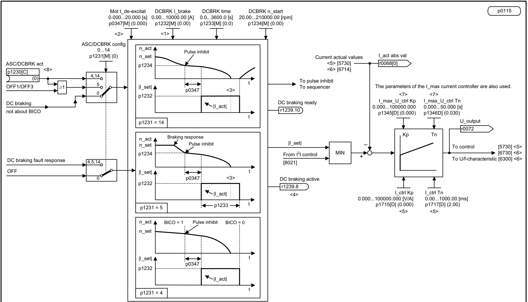
Fig. 3-268 7017 – DC braking (p0300 = 1xx)
