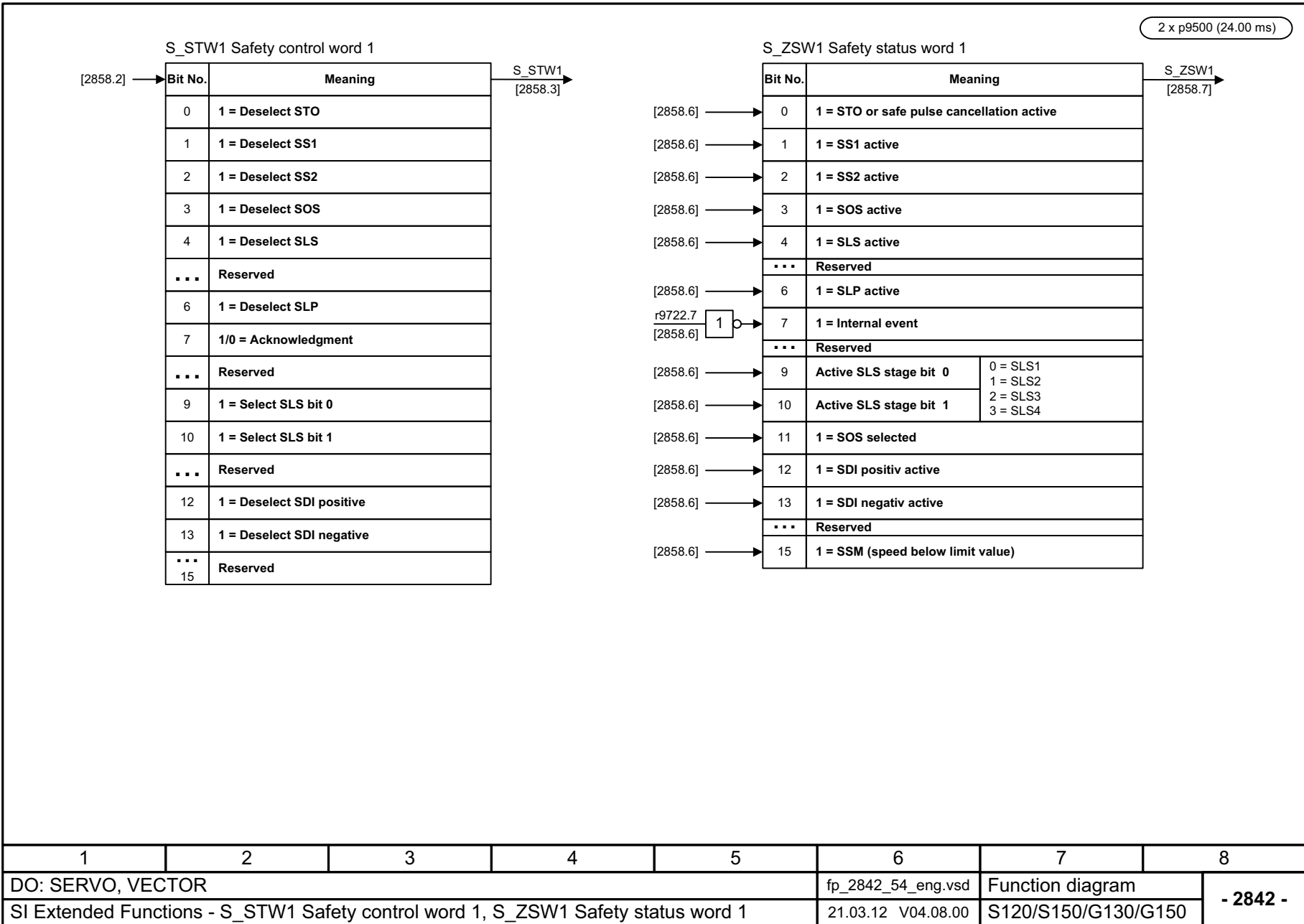
Fig. 3-129 2842 – S_STW1 Safety control word 1, S_ZSW1 Safety status word 1
