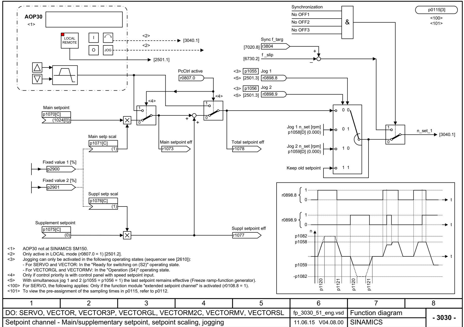
Fig. 3-154 3030 – Main/supplementary setpoint, setpoint scaling, jogging
