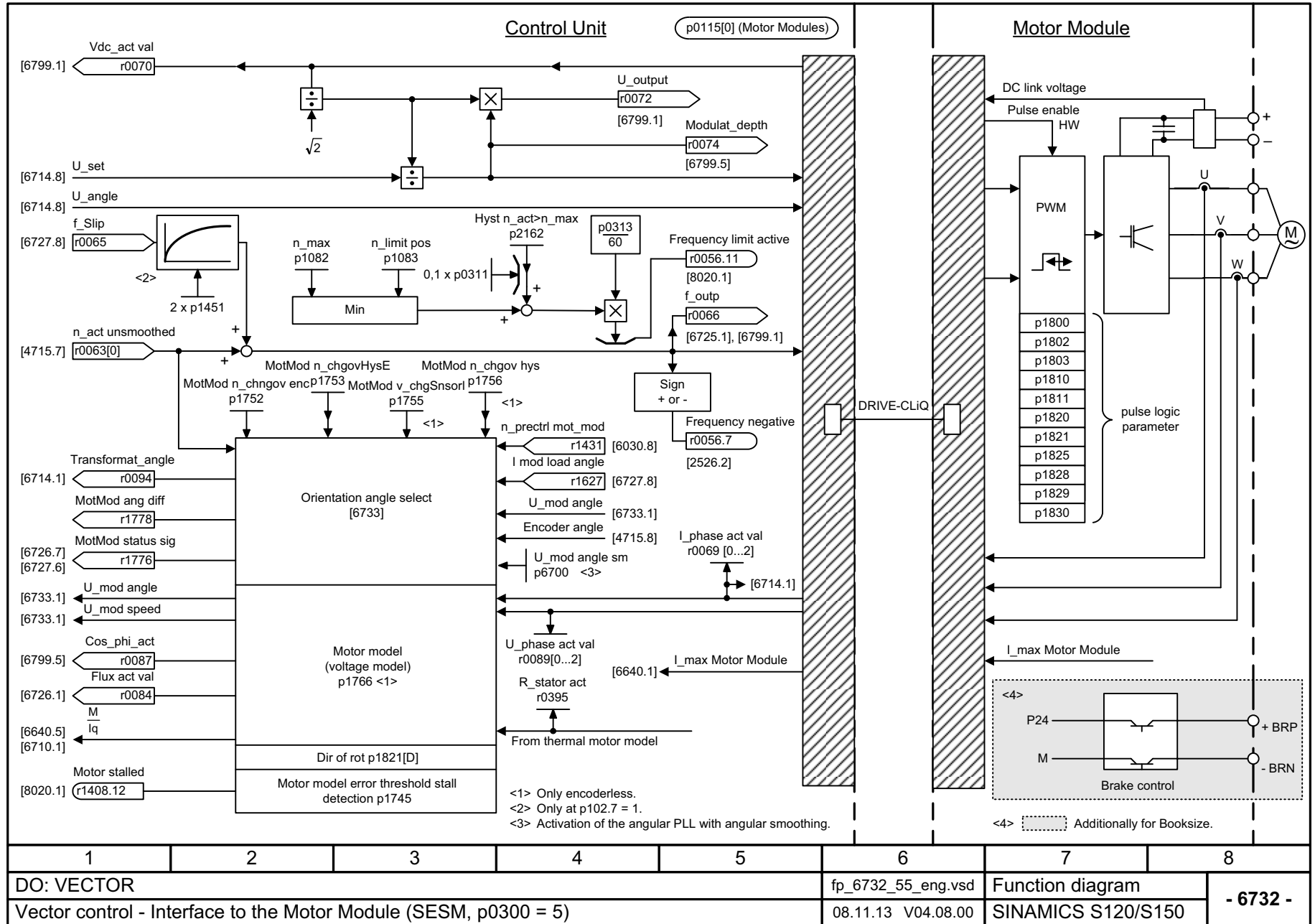
Fig. 3-256 6732 – Interface to the Motor Module (FEM, p0300 = 5)
