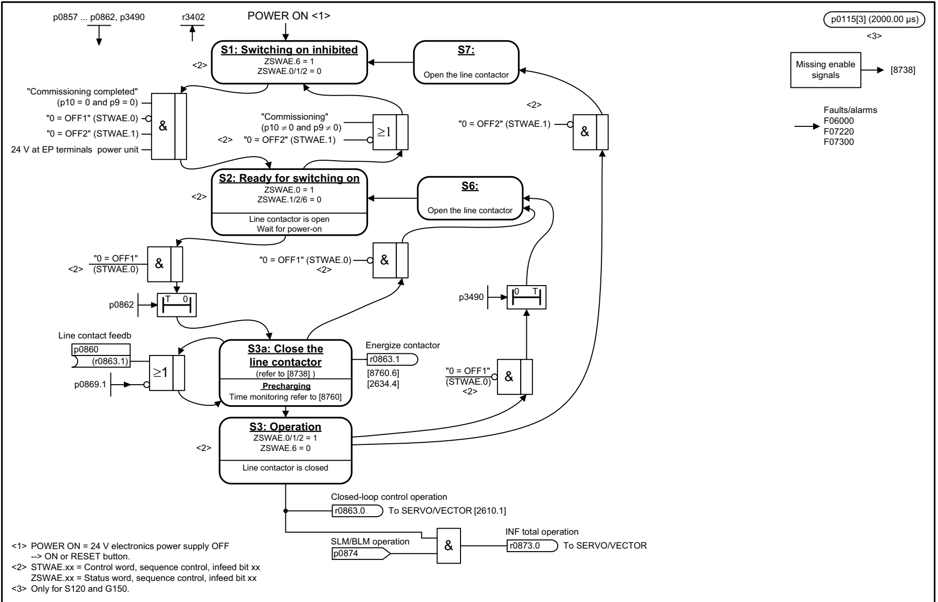
Fig. 3-320 8732 – Sequencer
