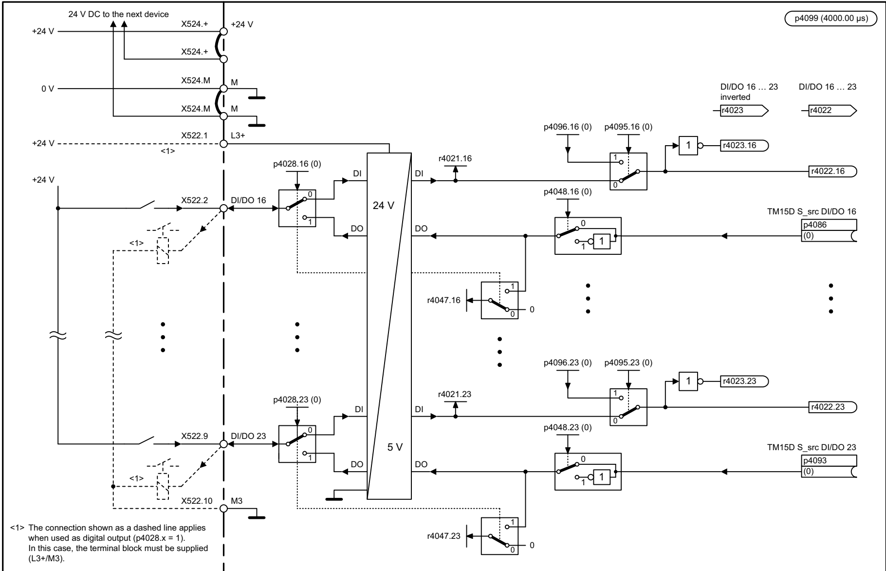
Fig. 3-362 9402 – Digital inputs/outputs, bidirectional (DI/DO 16 ... DI/DO 23)
