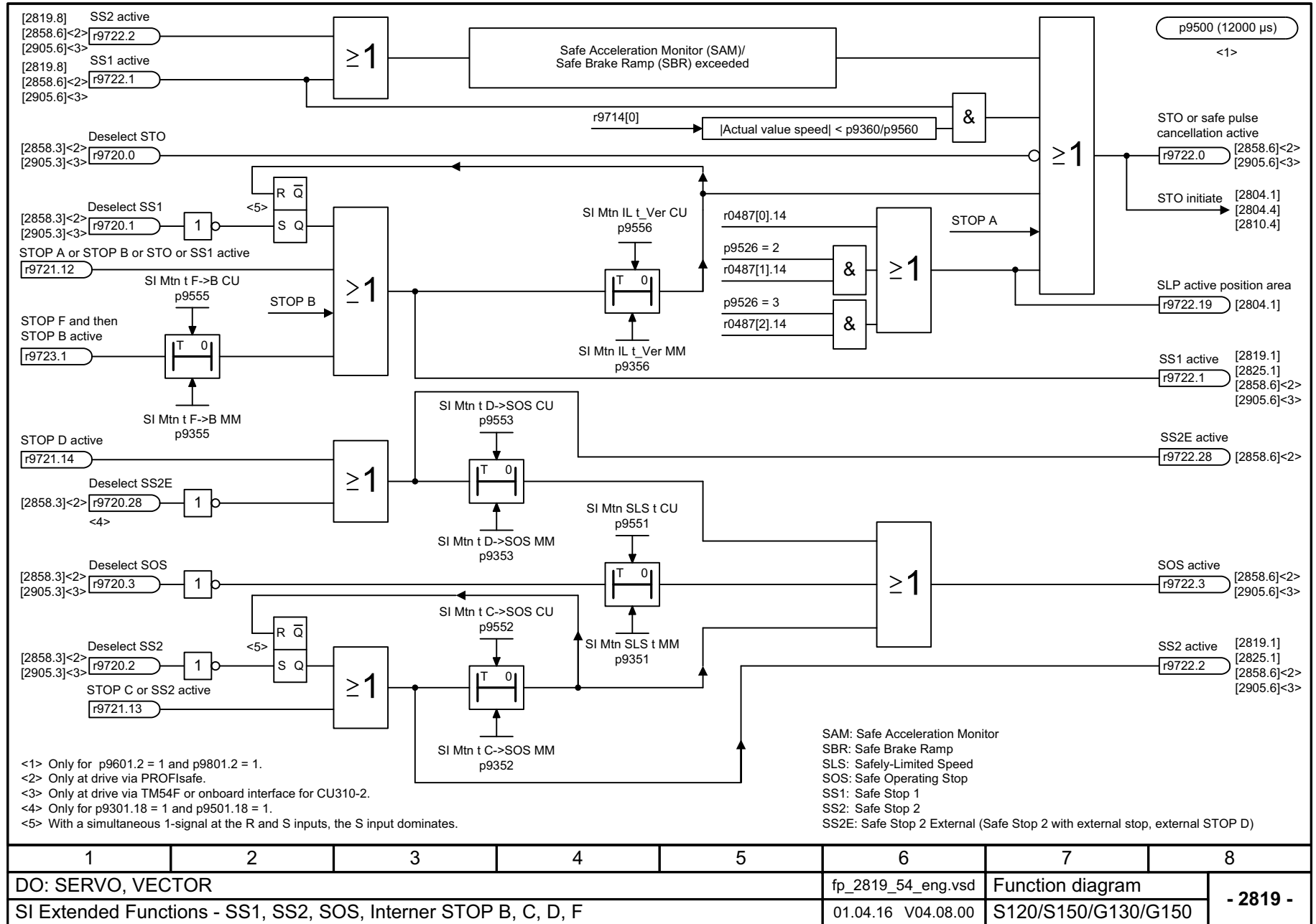
Fig. 3-119 2819 – SS1, SS2, SOS, internal STOP B, C, D, F
