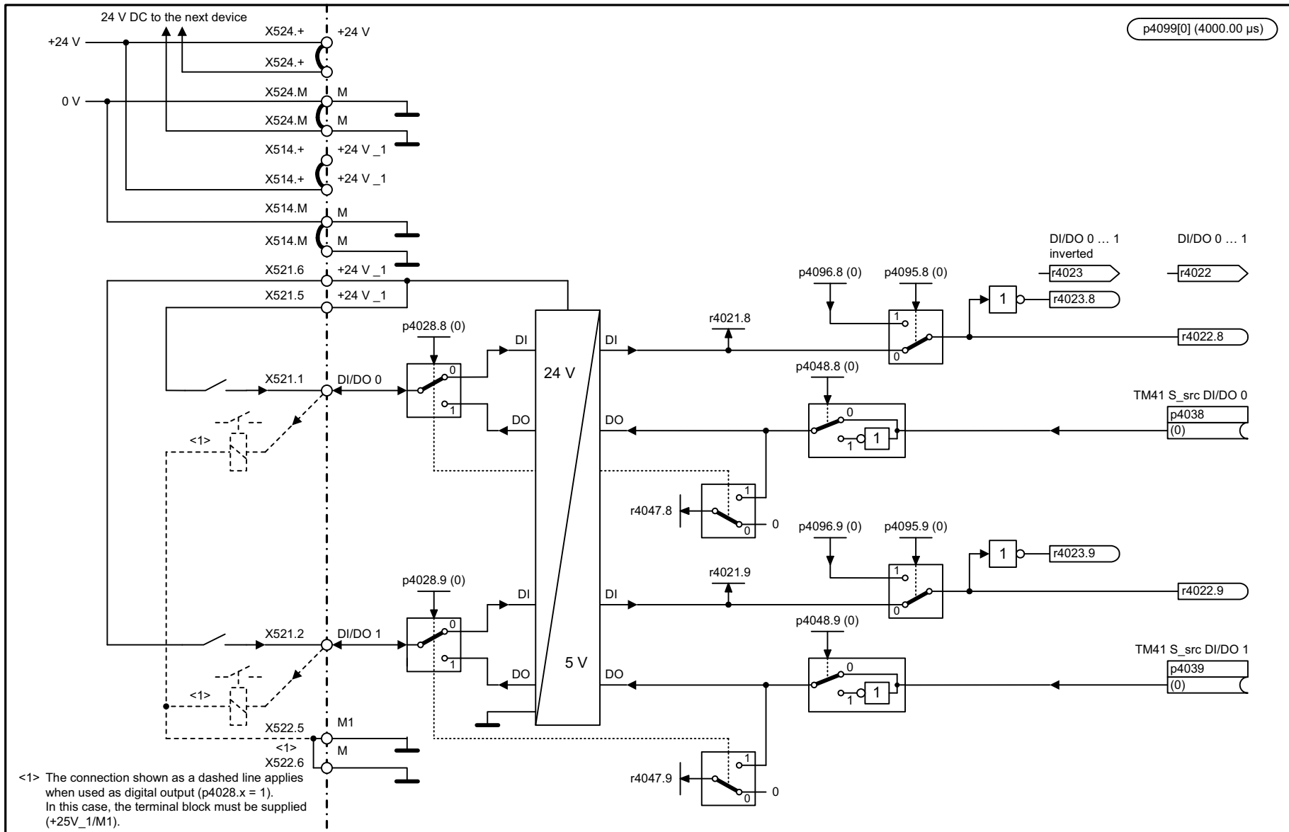
Fig. 3-381 9661 – Digital inputs/outputs, bidirectional (DI/DO 0 ... DI/DO 1)
