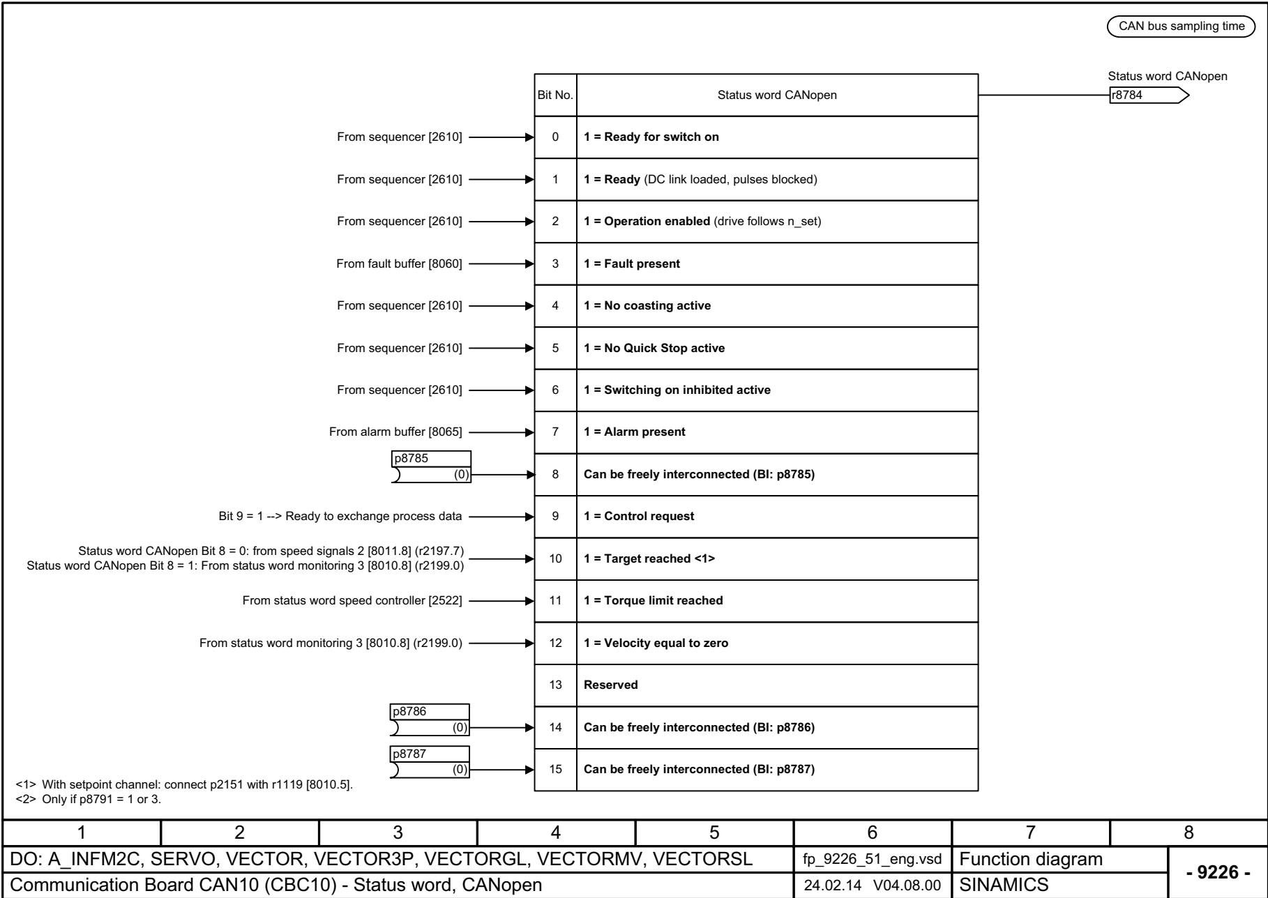
Fig. 3-357 9226 – Status word, CANopen
