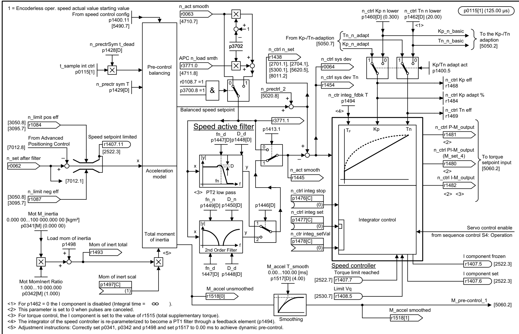
Fig. 3-207 5042 – Speed controller, torque/speed precontrol with encoder (p1402.4 = 1)
