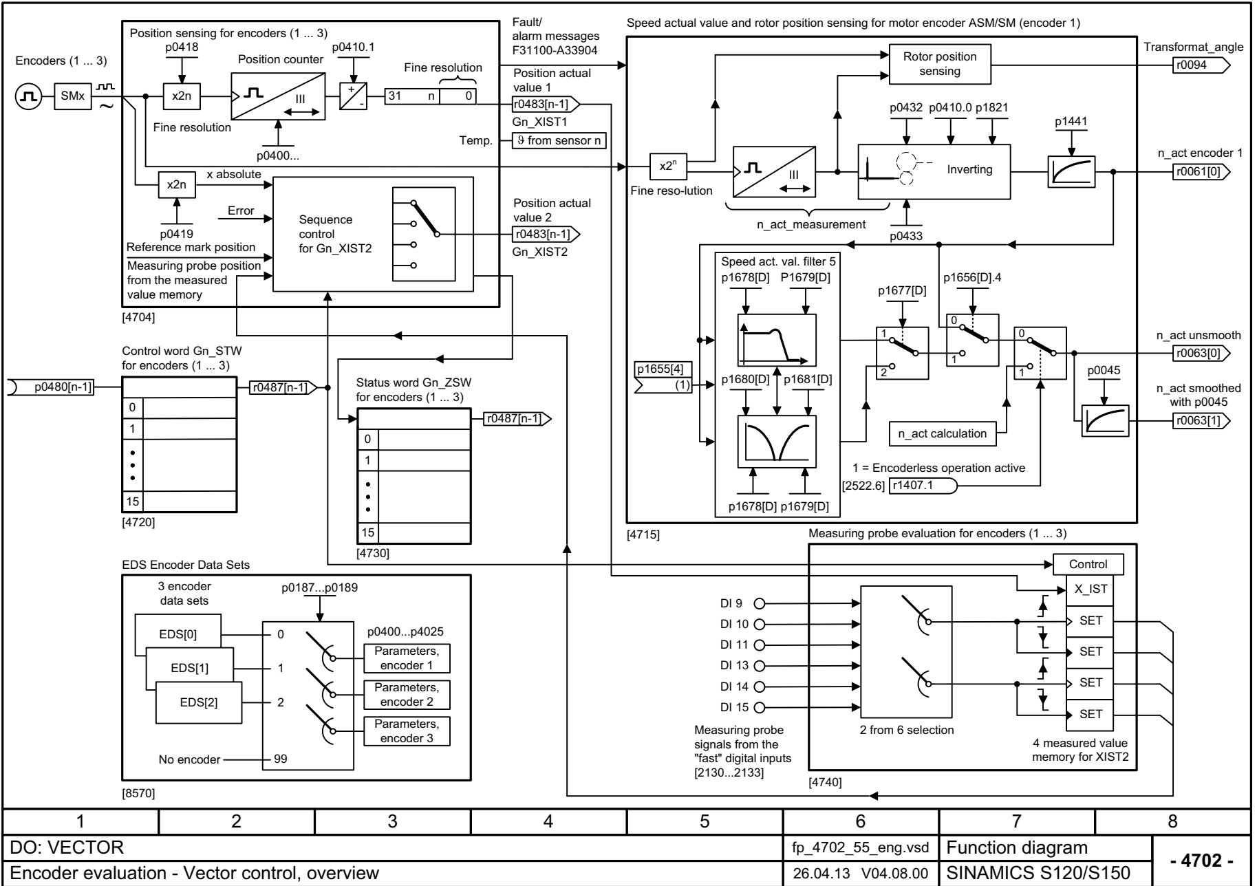
Fig. 3-183 4702 – Vector control, overview
