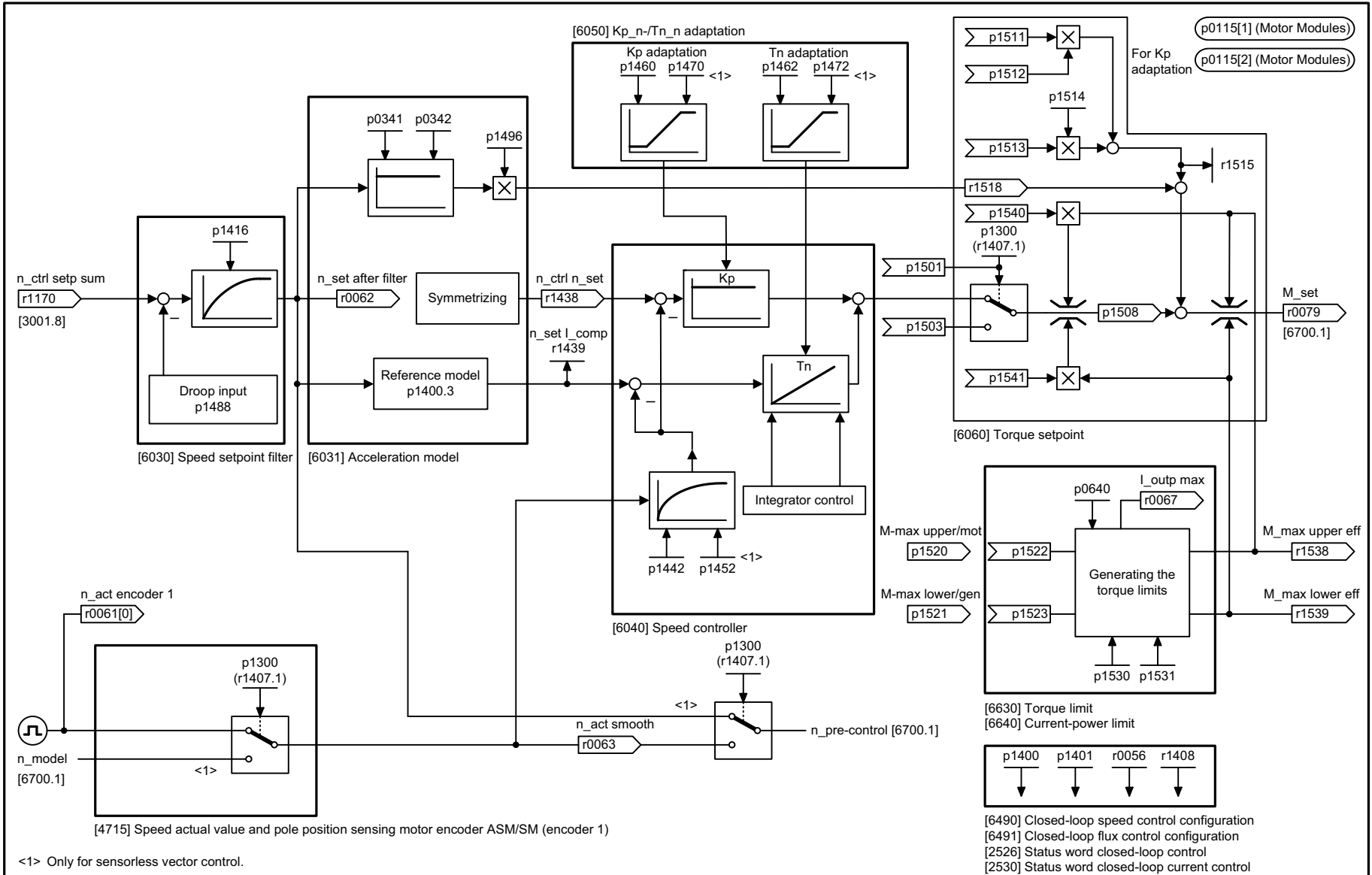
Fig. 3-227 6020 – Speed control and generation of the torque limits, overview
