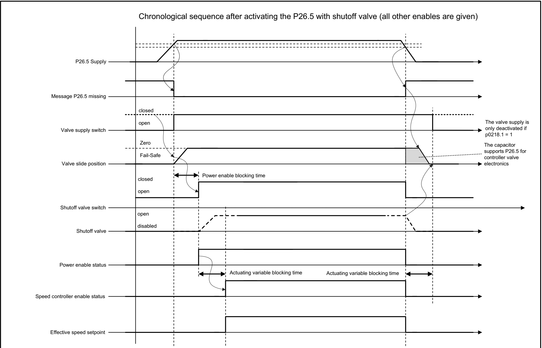
Fig. 3-200 4990 – P24 management with shutoff valve
