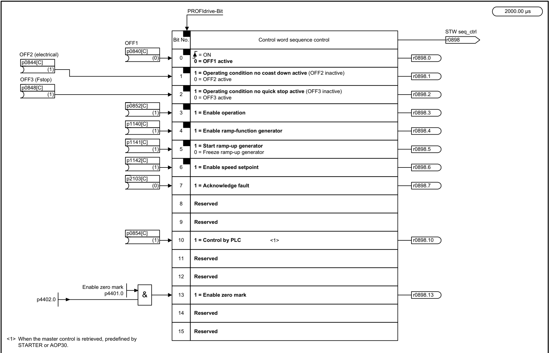
Fig. 3-387 9678 – Control word, sequence control (p4400 = 0)
