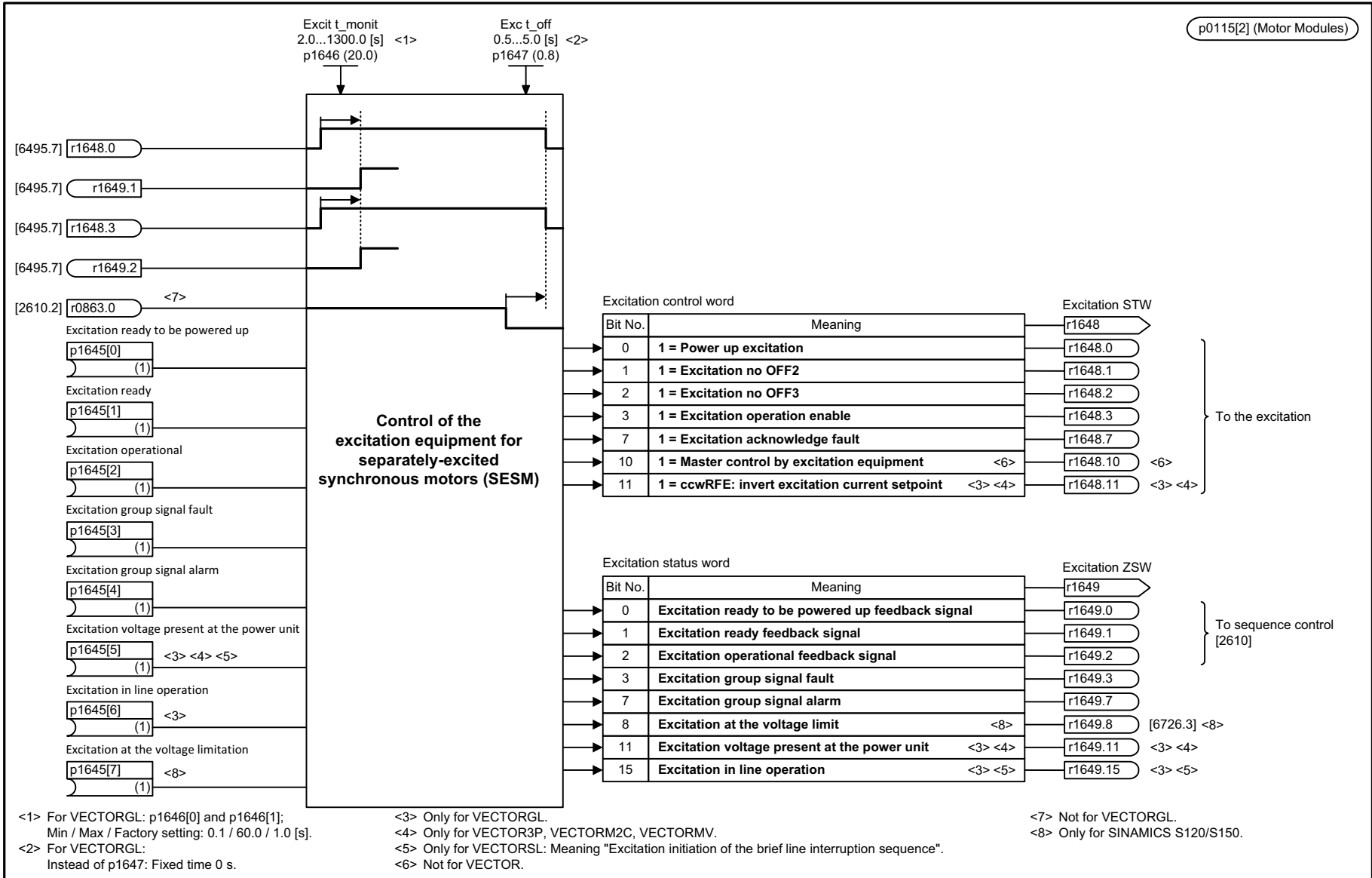
Fig. 3-241 6495 – Excitation (FEM, p0300 = 5)
