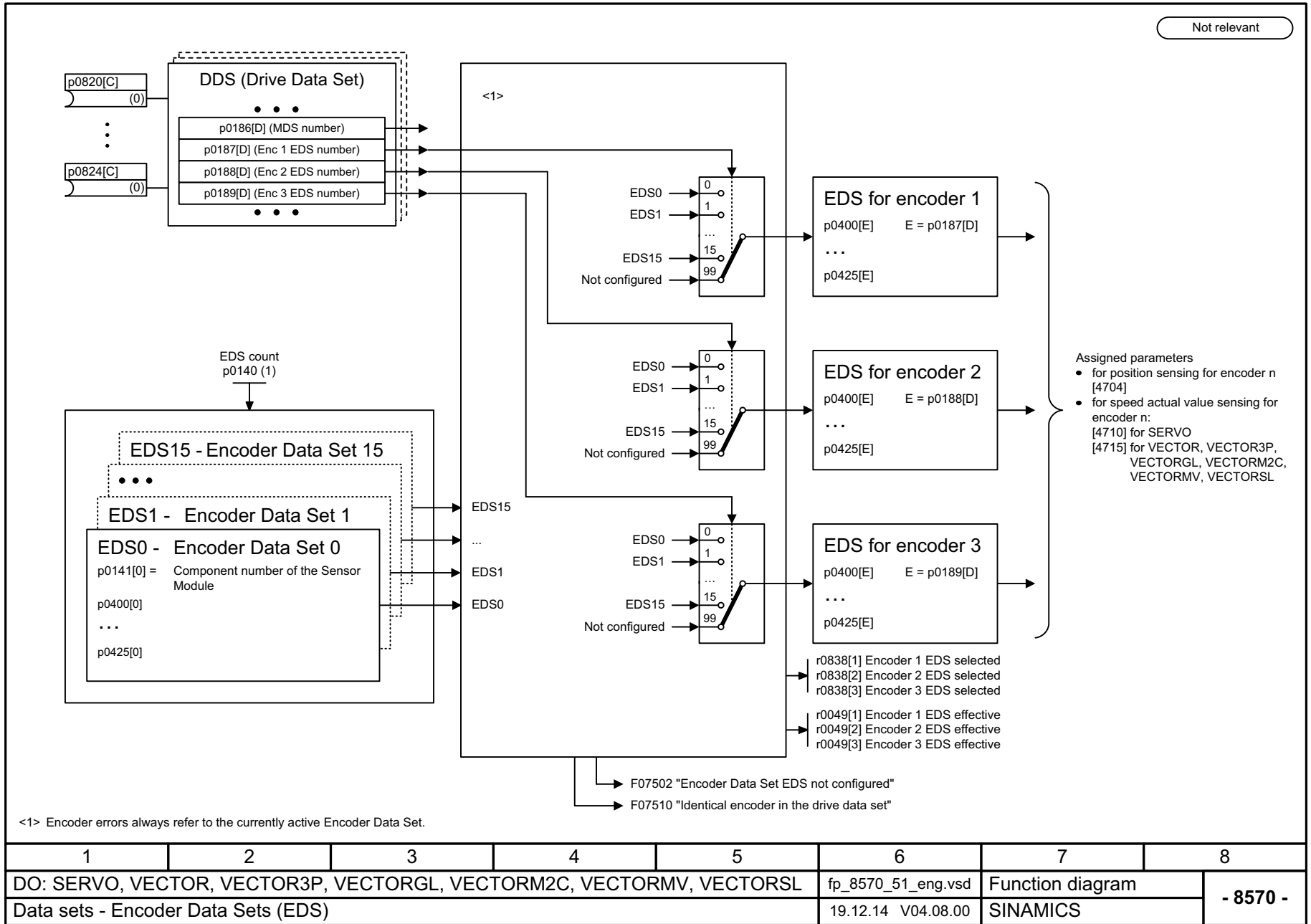
Fig. 3-314 8570 – Encoder Data Sets (EDS)
