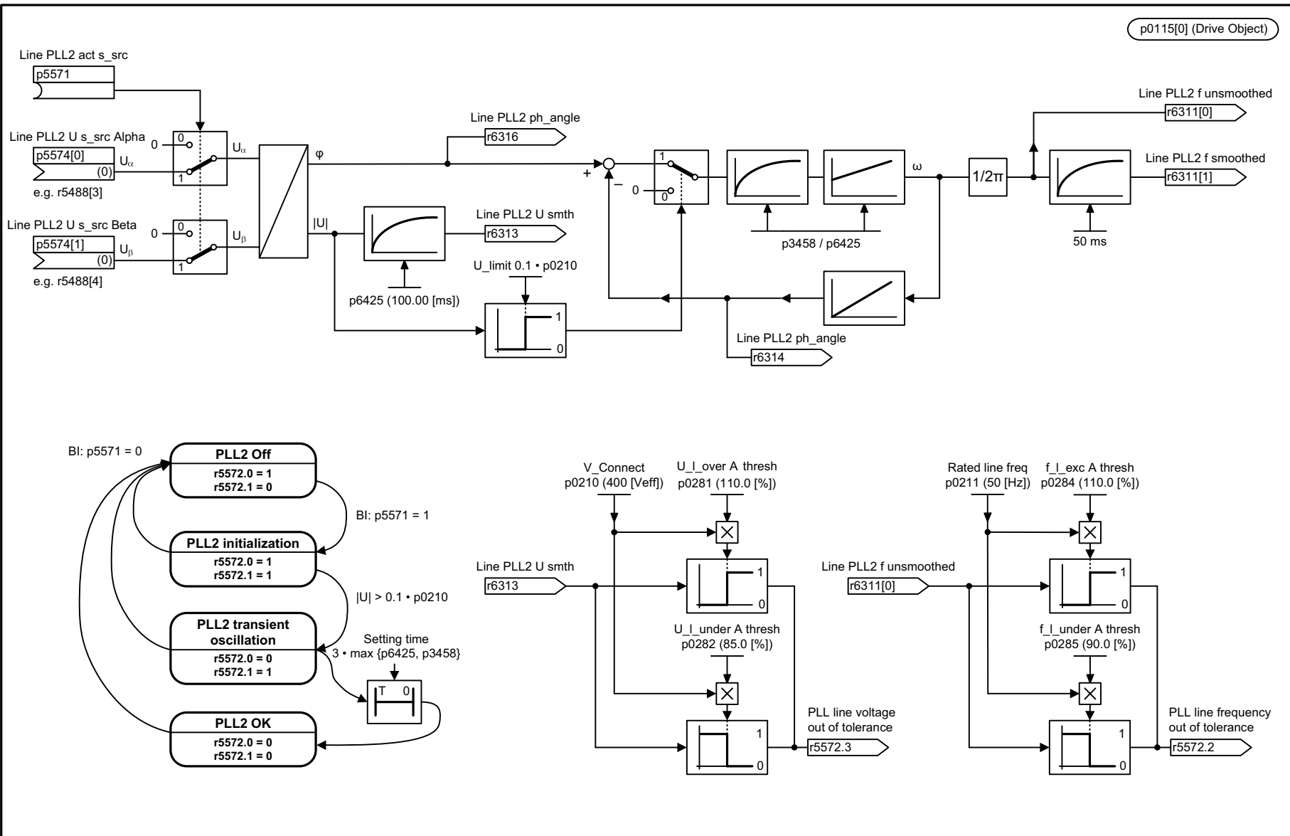
Fig. 3-285 7992 – PLL2 (phase locked loop 2)
