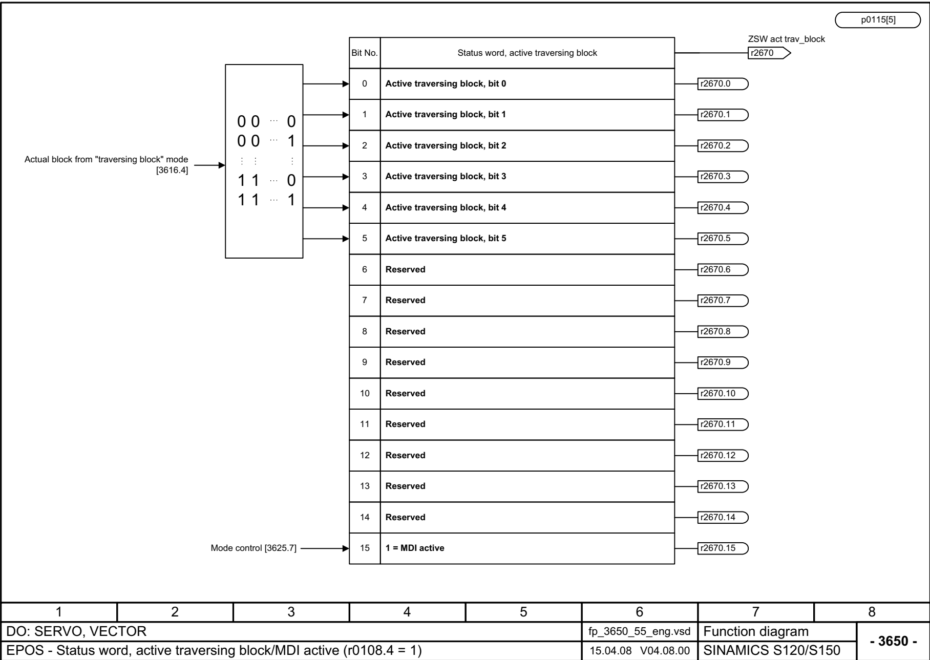
Fig. 3-177 3650 – Status word, active traversing block/MDI active (r0108.4 = 1)
