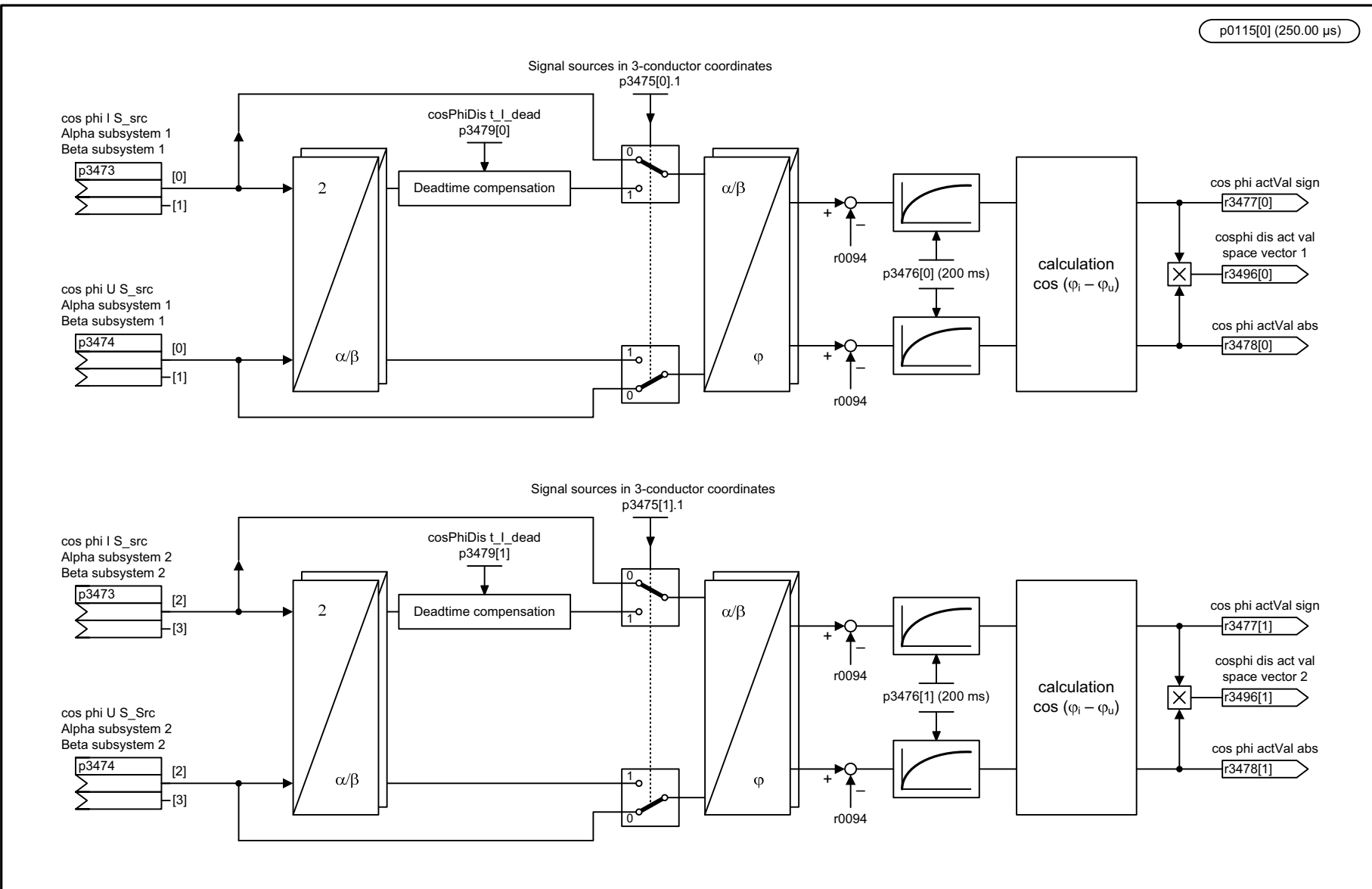
Fig. 3-344 8951 - Cos phi display (r0108.10 = 1)
