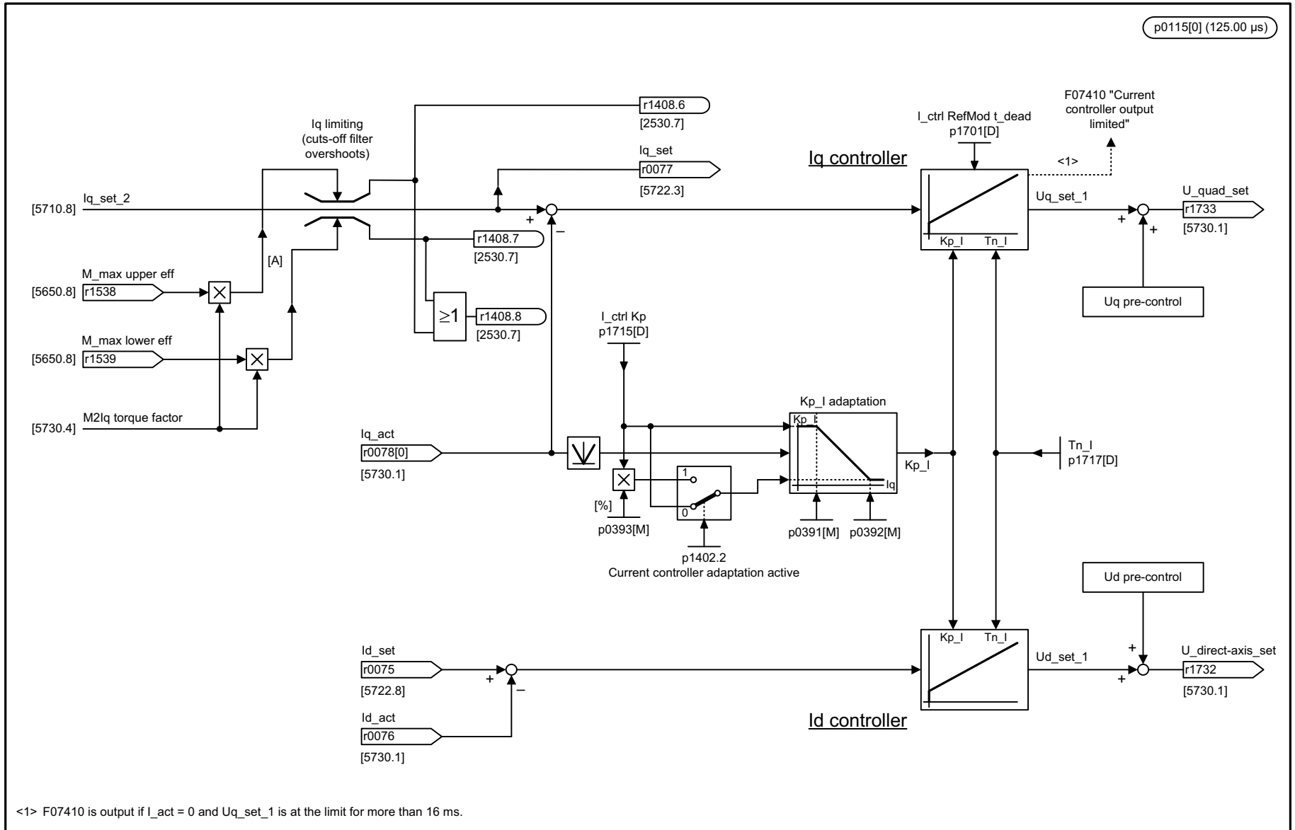
Fig. 3-224 5714 – Iq and Id controllers
