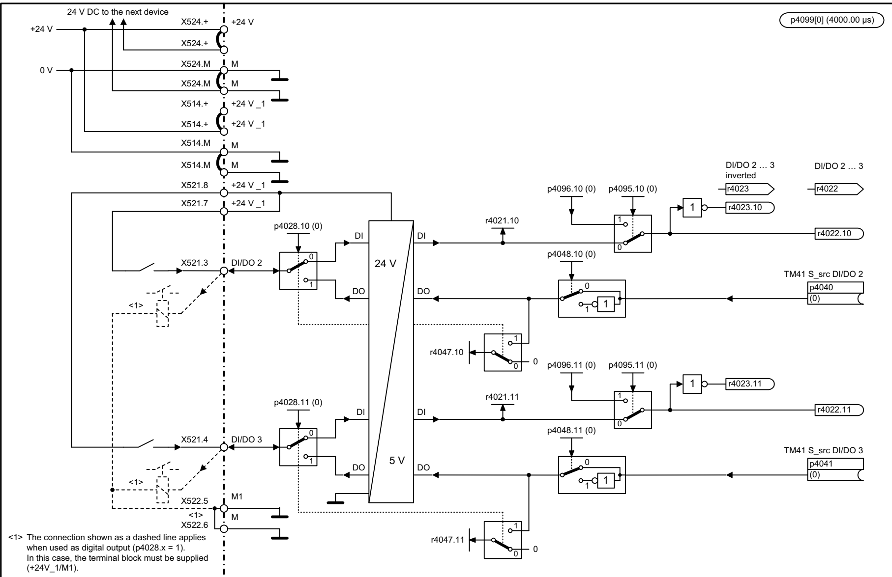
Fig. 3-382 9662 – Digital inputs/outputs, bidirectional (DI/DO 2 ... DI/DO 3)
