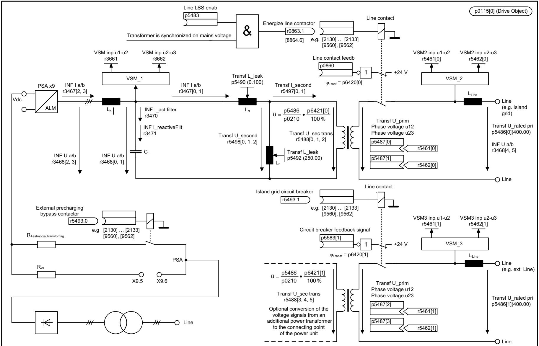
Fig. 3-283 7990 – Transformer model (p5480 = 1)
