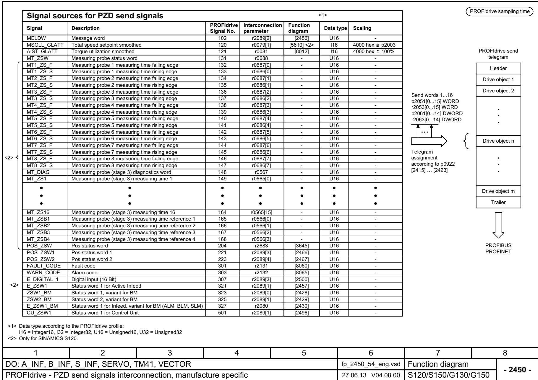
Fig. 3-60 2450 – PZD send signals interconnection, manufacturer-specific
