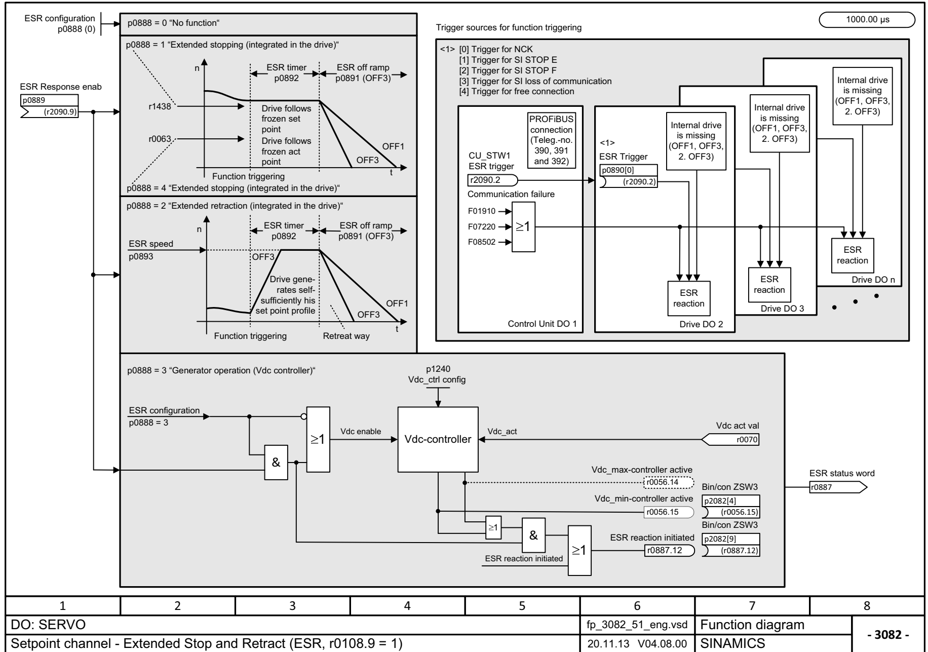
Fig. 3-160 3082 – Extended Stop and Retract (ESR, r0108.9 = 1)
