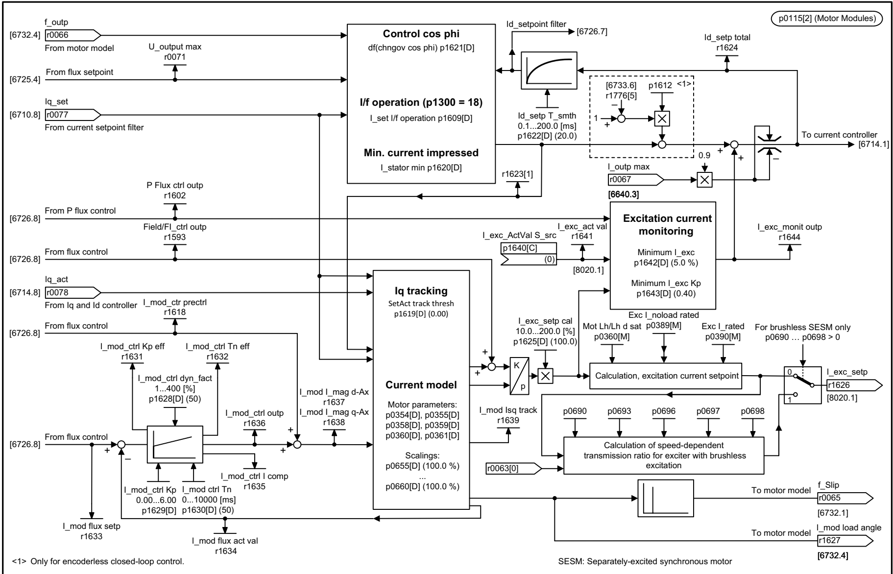
Fig. 3-253 6727 – Current model, excitation current monitoring, control cos phi (FEM, p0300 = 5)
