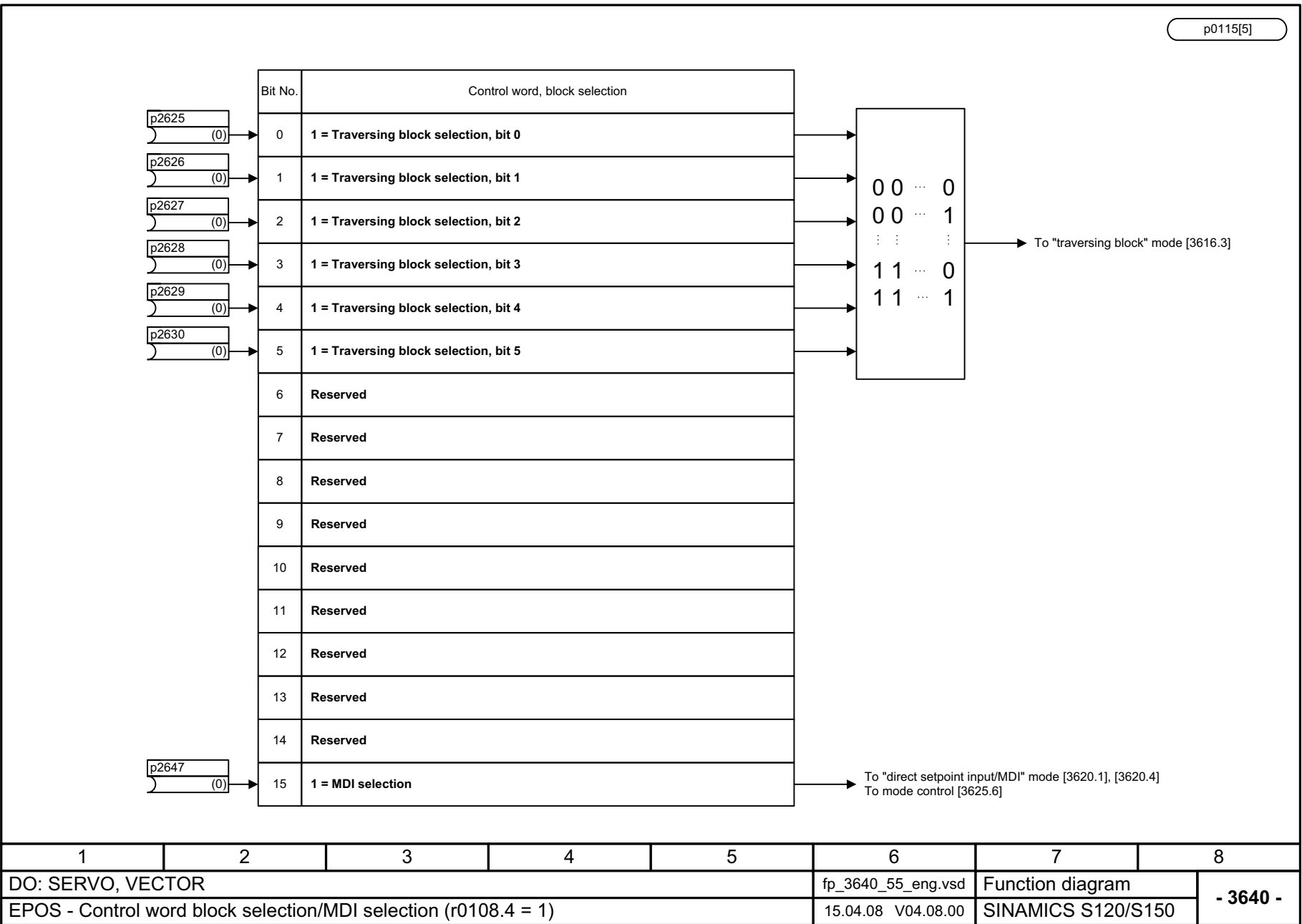
Fig. 3-174 3640 – Control word, block selection/MDI selection (r0108.4 = 1)
