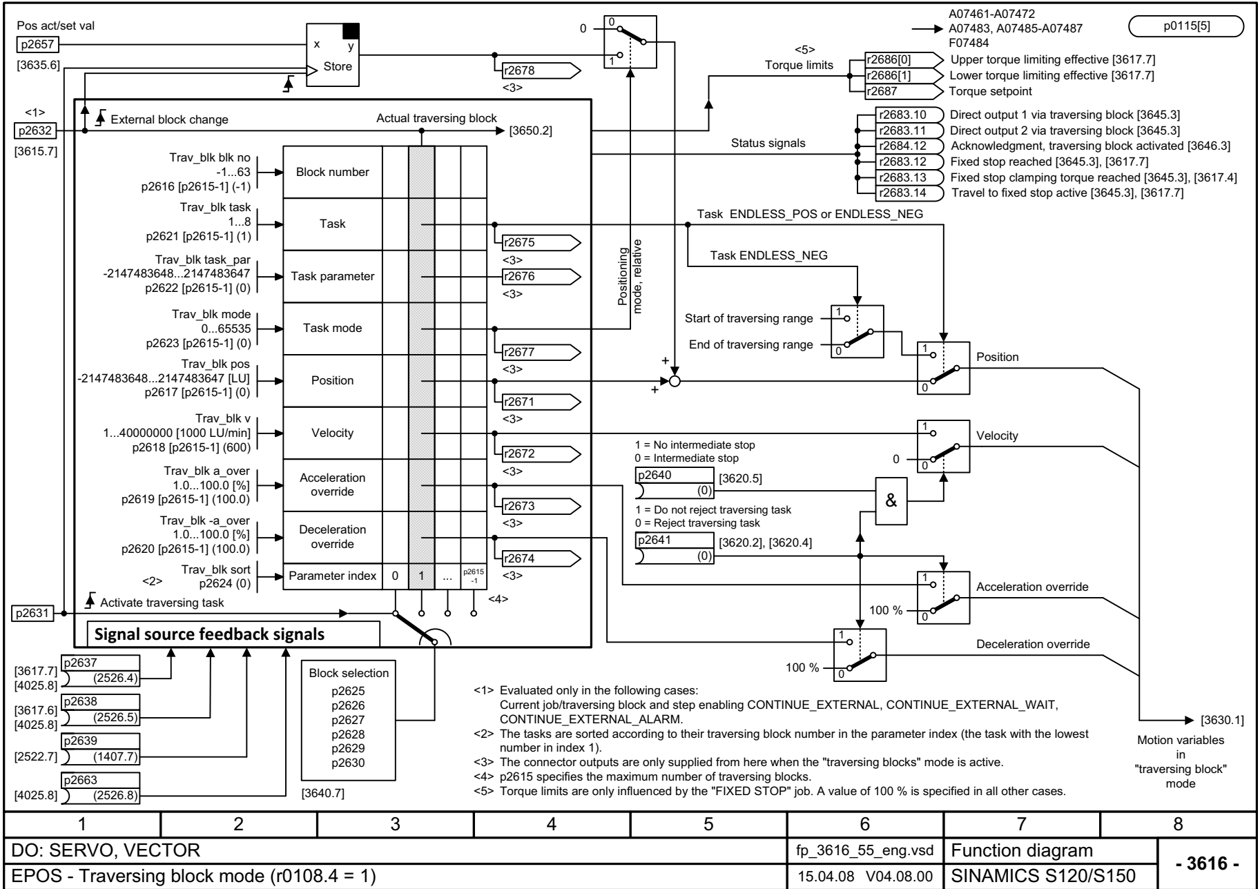
Fig. 3-167 3616 - Traversing block mode (r0108.4 = 1)
