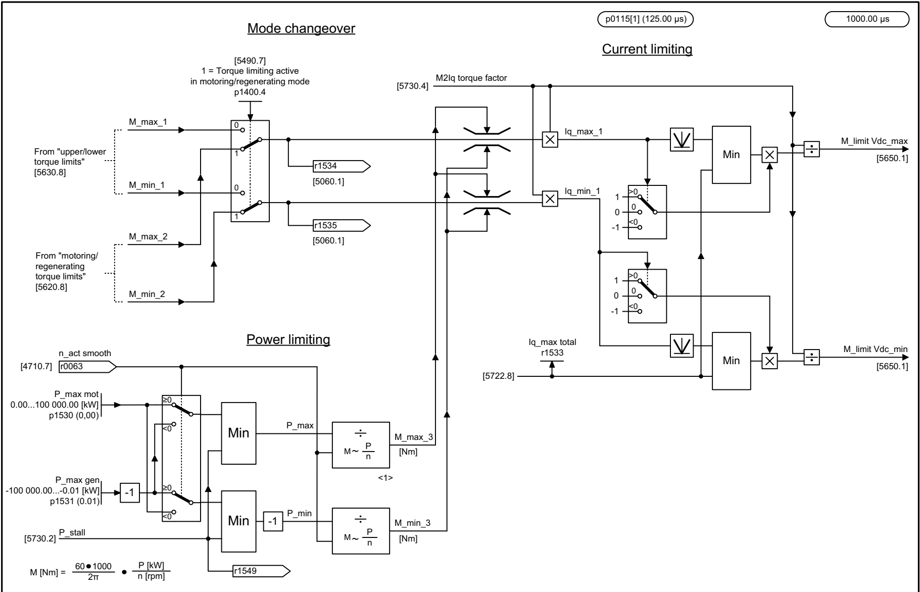
Fig. 3-219 5640 – Mode changeover, power/current limiting
