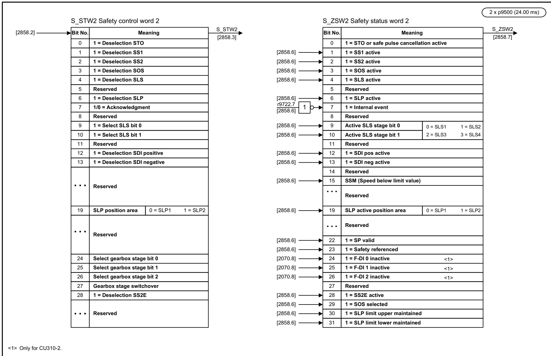
Fig. 3-130 2843 – S_STW2 Safety control word 2, S_ZSW2 Safety status word 2
