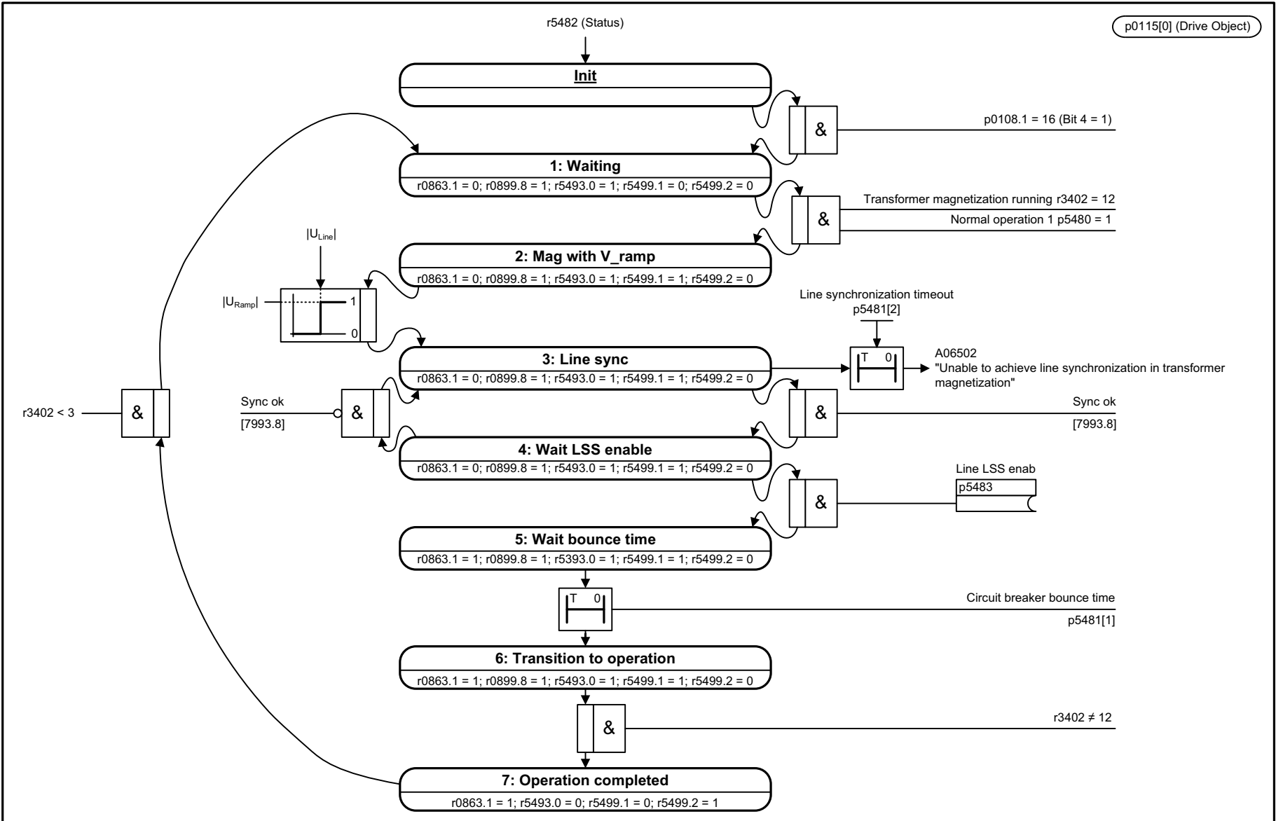
Fig. 3-287 7994 – Transformer magnetization, sequence control
