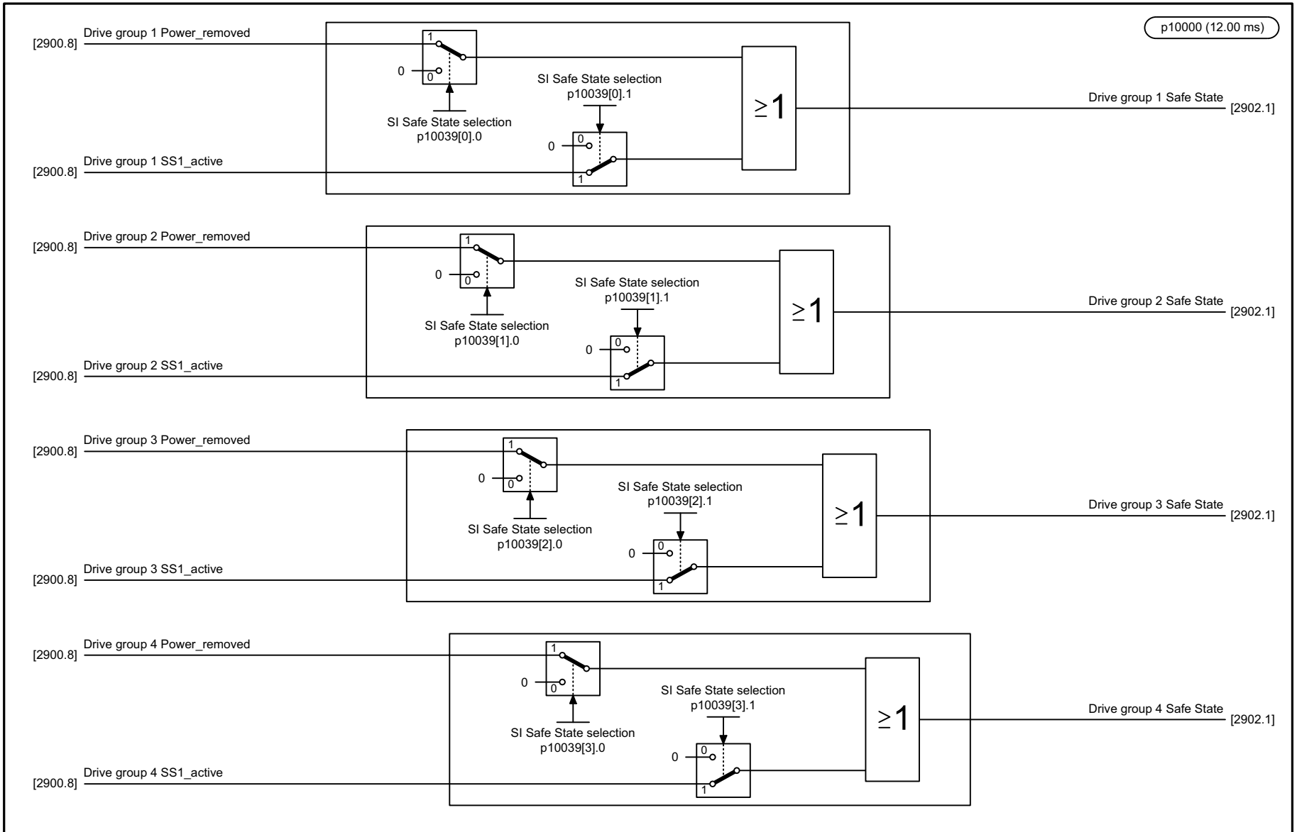
Fig. 3-144 2901 – Basic Functions safe state selection
