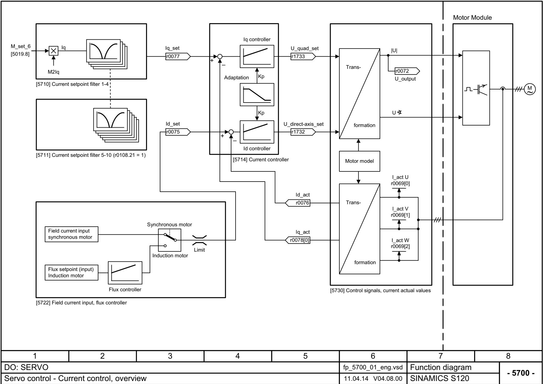
Fig. 3-221 5700 – Current control, overview
