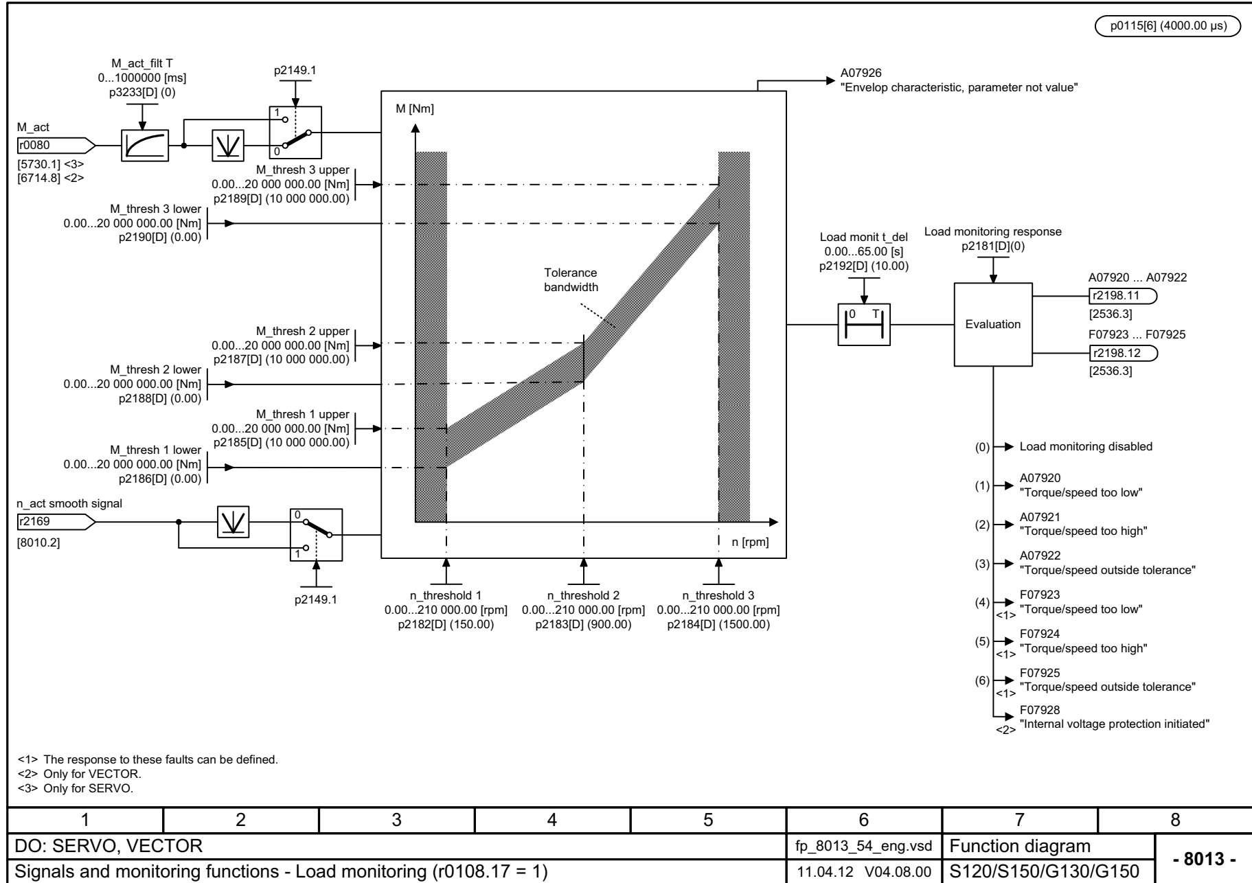
Fig. 3-296 8013 – Load monitoring (r0108.17 = 1)
