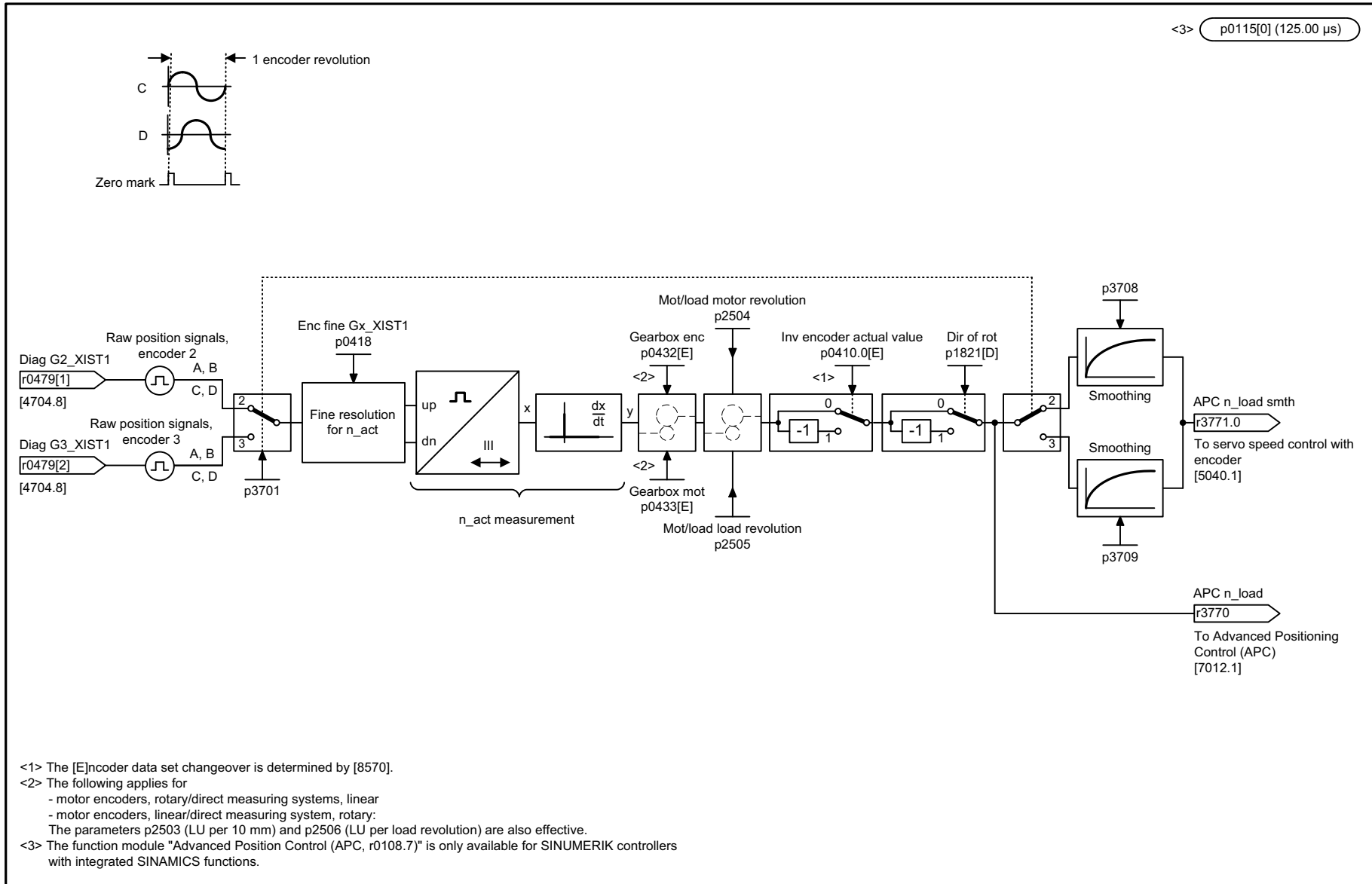
Fig. 3-186 4711 – Speed actual value sensing, encoders 2, 3 (r0108.7 = 1, APC activated)
