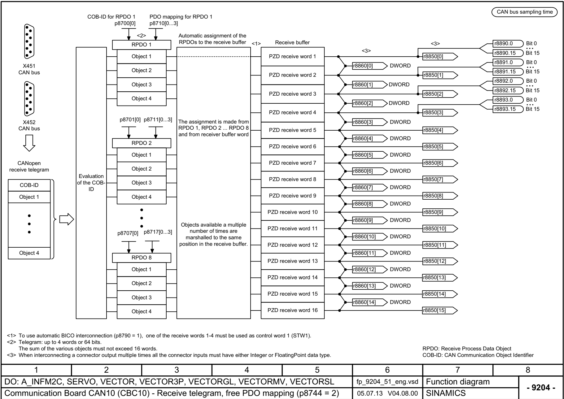
Fig. 3-352 9204 – Receive telegram, free PDO mapping (p8744 = 2)
