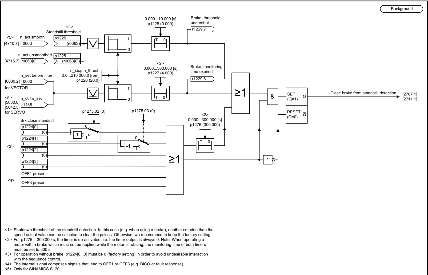
Fig. 3-108 2704 – Extended brake control, zero-speed detection (r0108.14 = 1)
