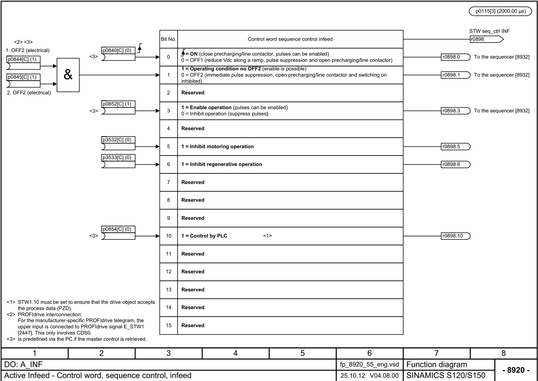
Fig. 3-334 8920 – Control word, sequence control infeed
