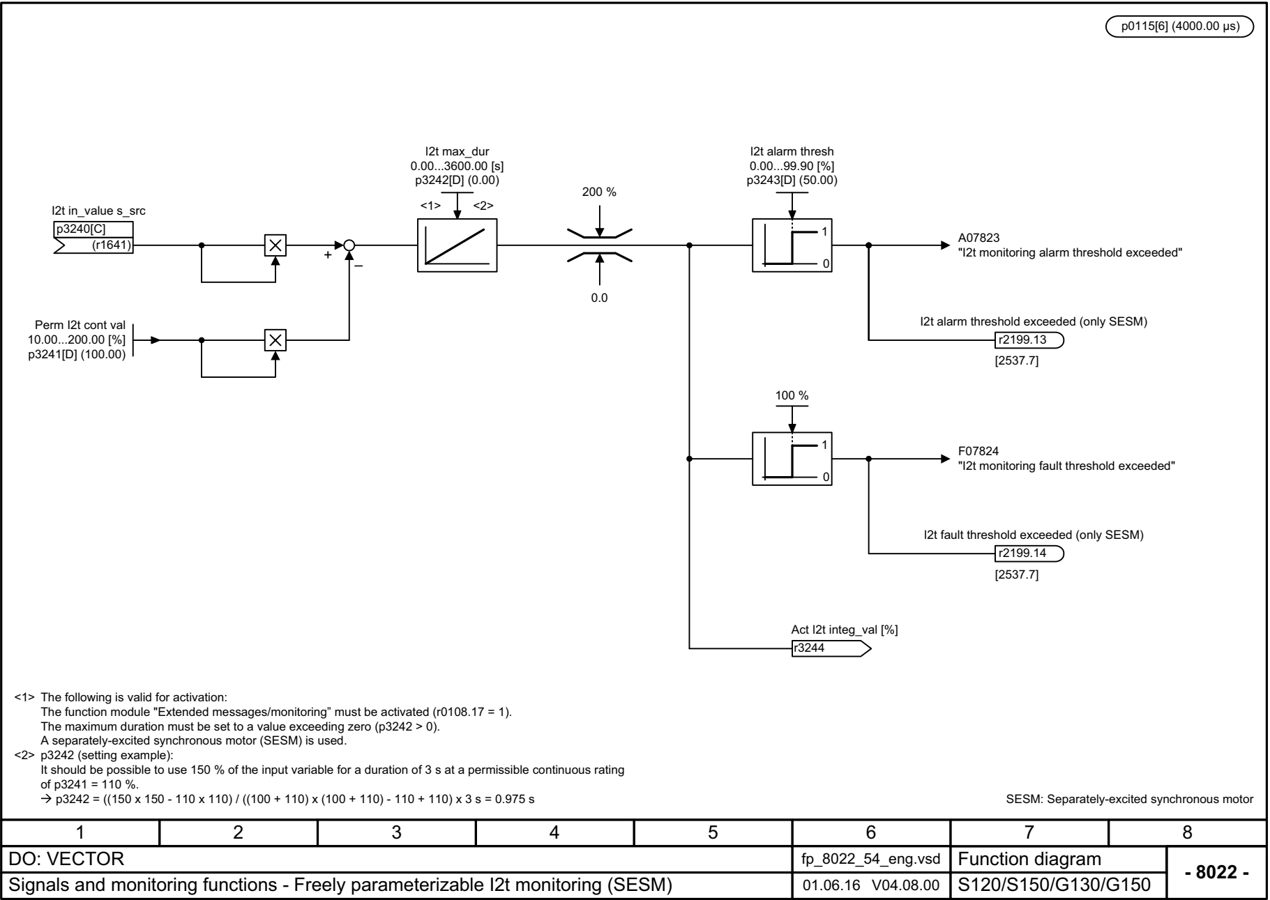
Fig. 3-303 8022 – Freely parameterizable I2t monitoring (SESM)
