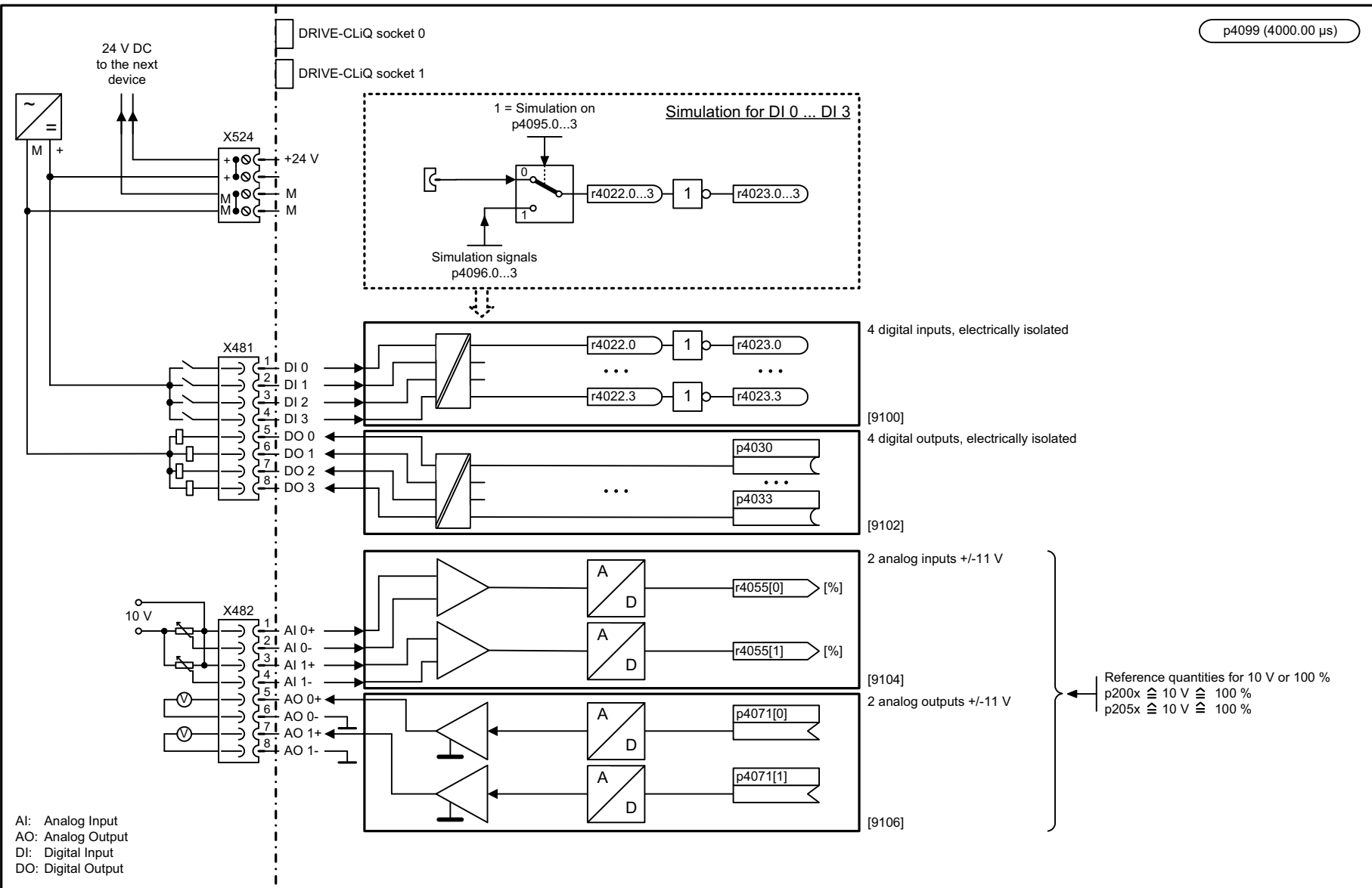
Fig. 3-347 9099 – Overview
