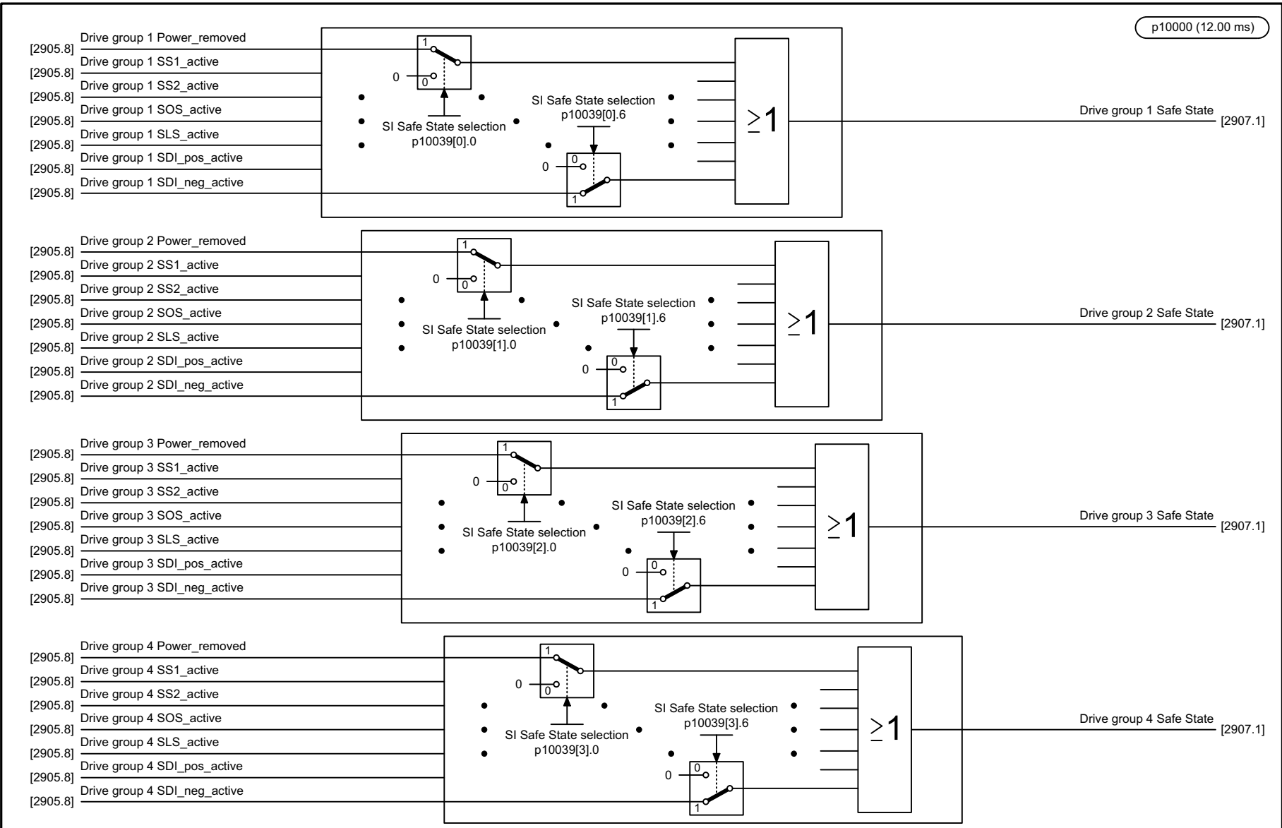
Fig. 3-147 2906 – Extended Functions safe state selection
