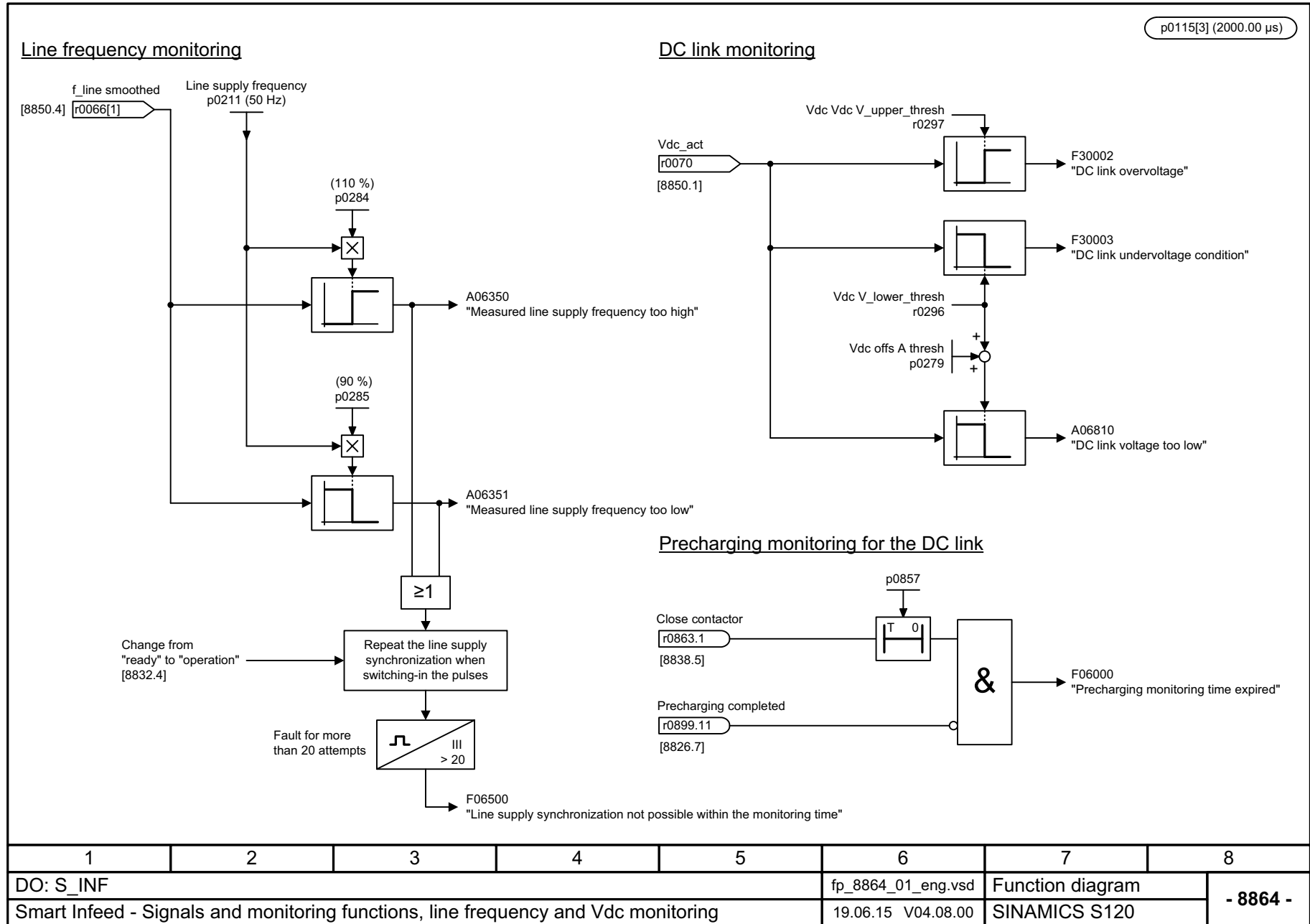
Fig. 3-332 8864 – Signals and monitoring functions, line frequency and Vdc monitoring
