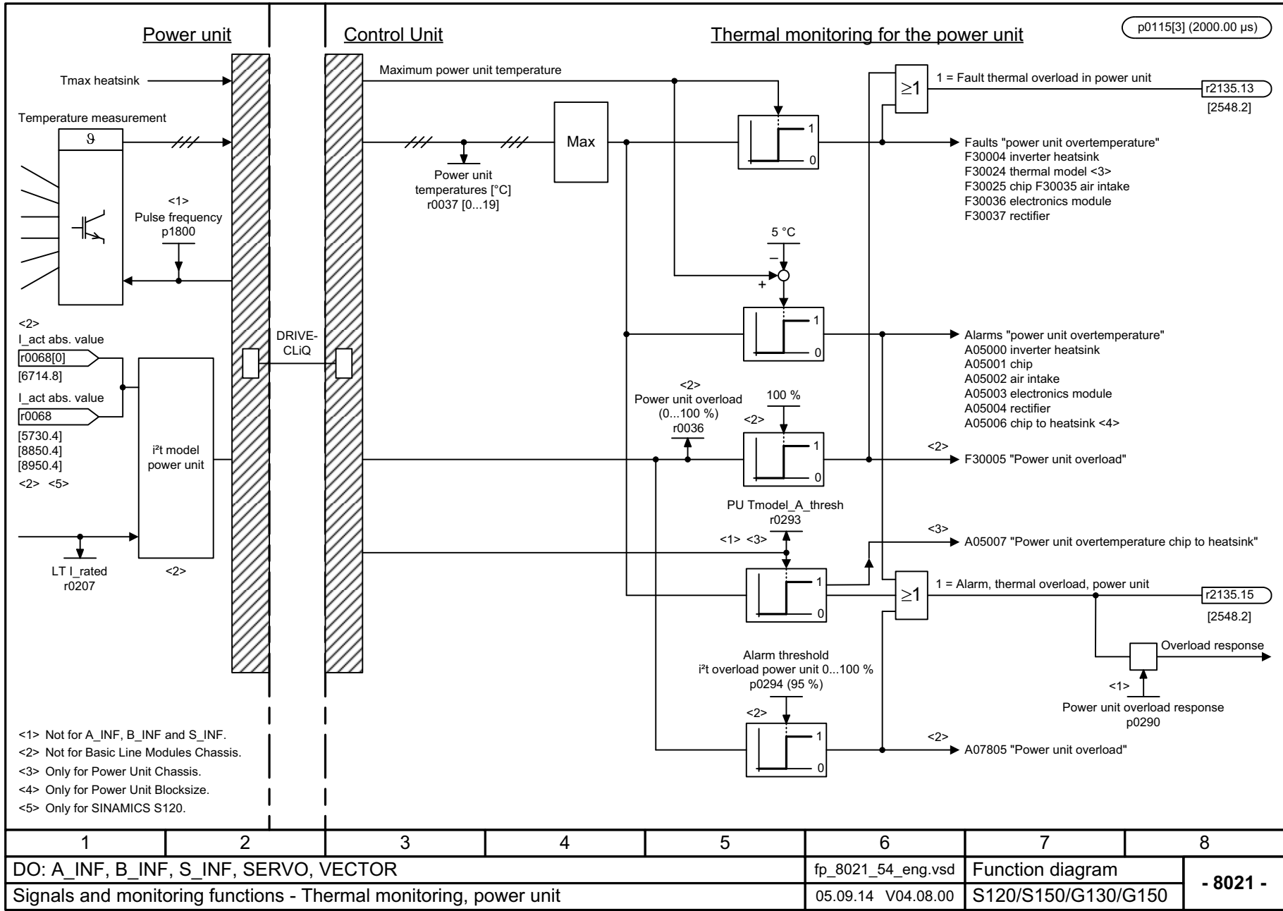
Fig. 3-302 8021 – Thermal monitoring, power unit
