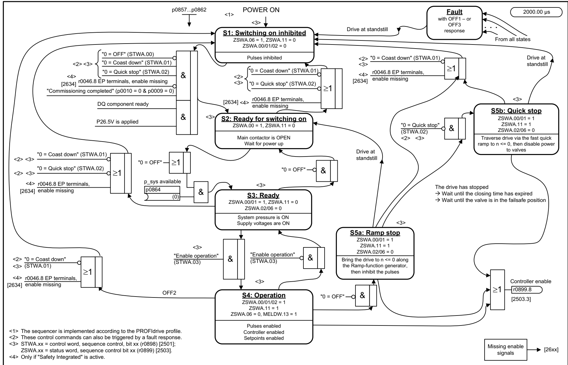
Fig. 3-199 4985 – Sequencer
