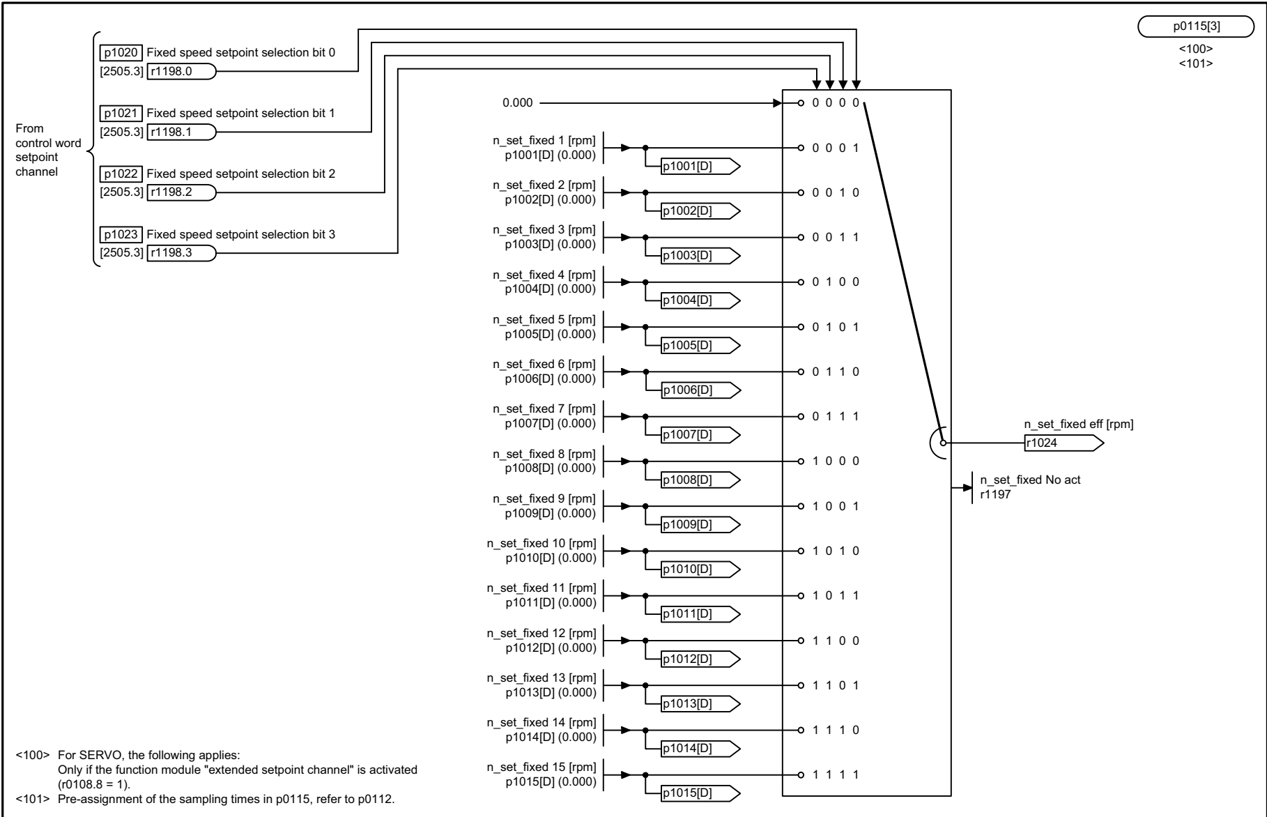
Fig. 3-152 3010 – Fixed speed setpoints
