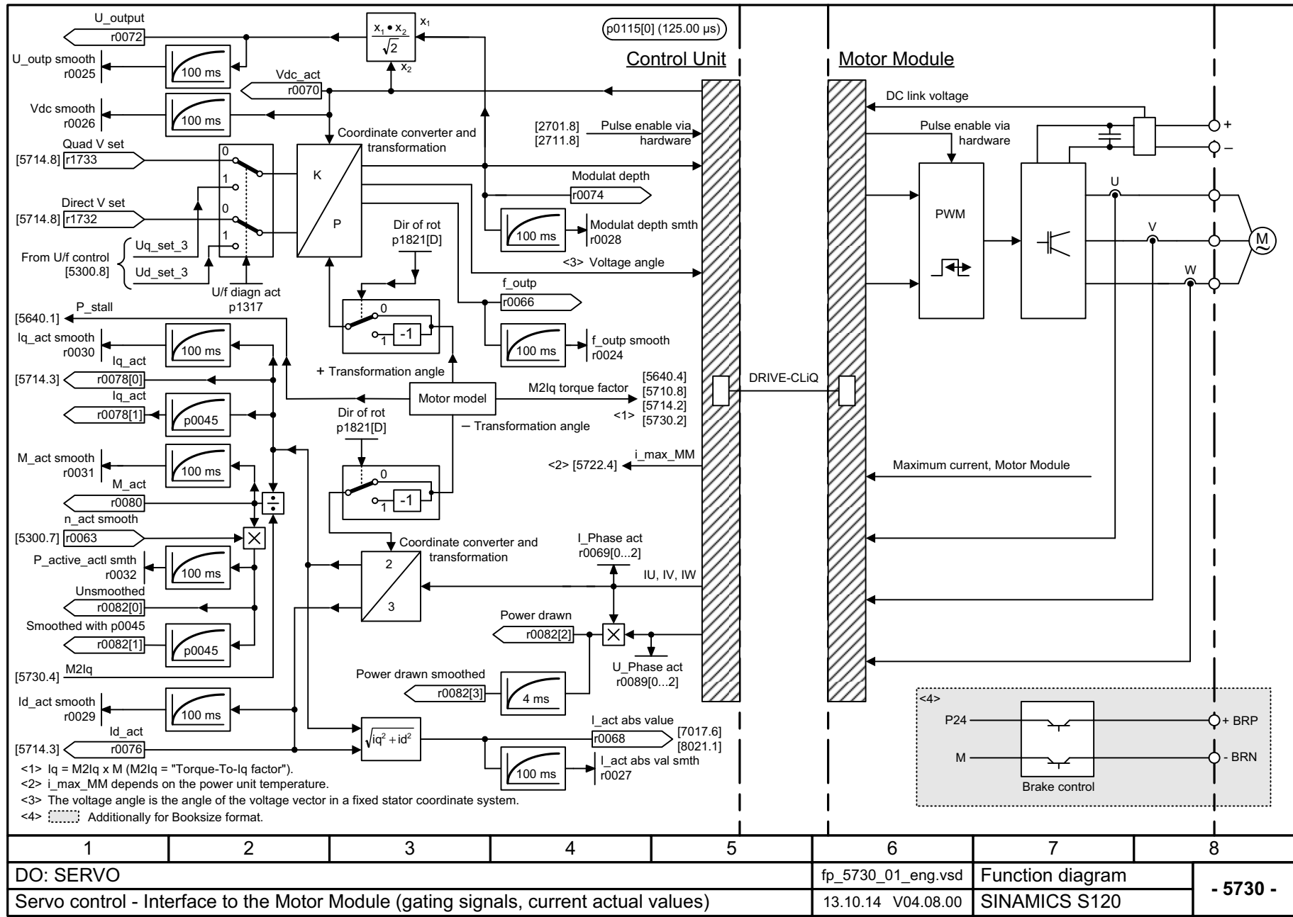
Fig. 3-226 5730 – Interface to the Motor Module (gating signals, current actual values)
