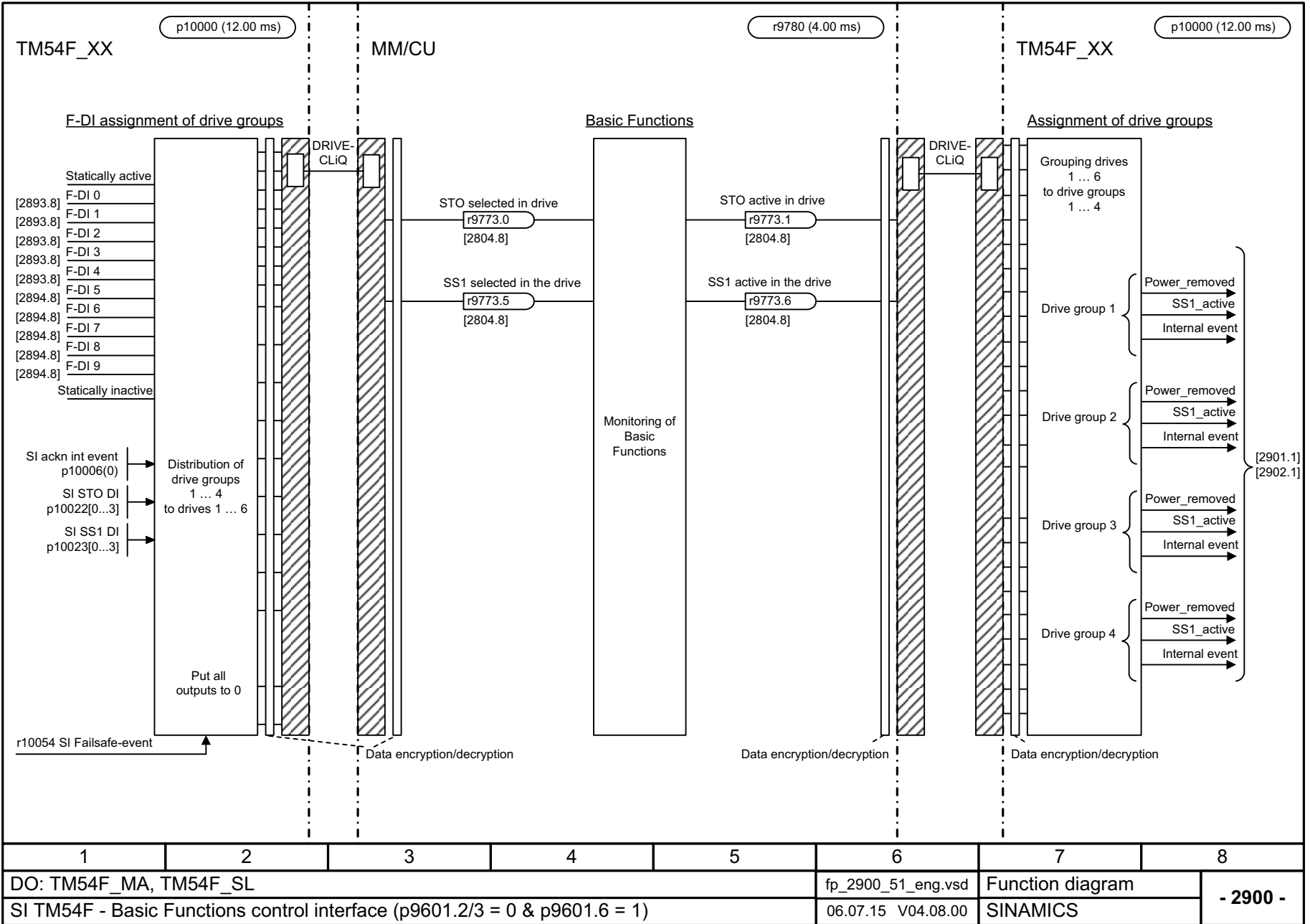
Fig. 3-143 2900 – Basic Functions control interface (p9601.2/3 = 0 & p9601.6 = 1)
