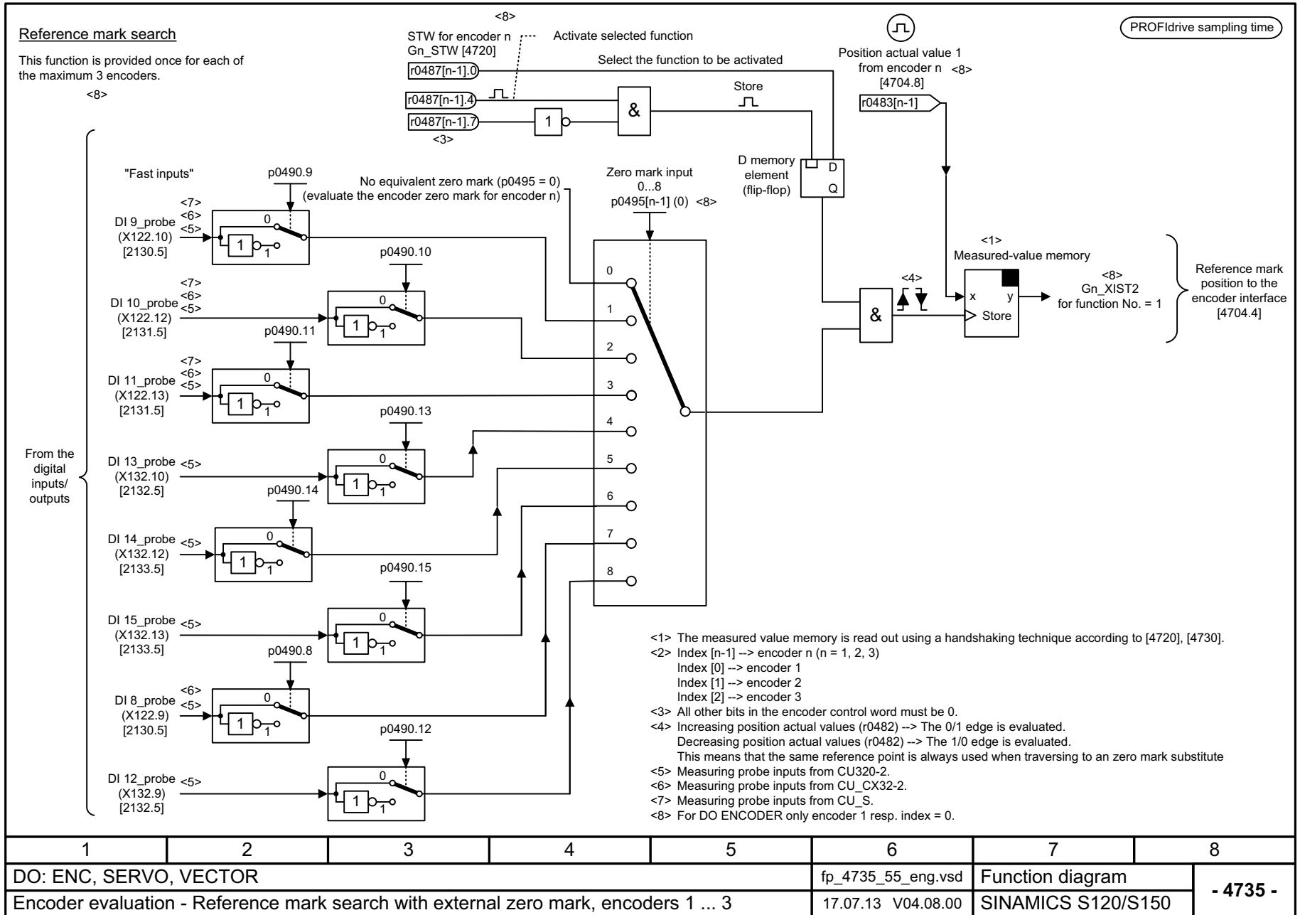
Fig. 3-190 4735 – Reference mark search with external zero mark, encoders 1 ... 3
