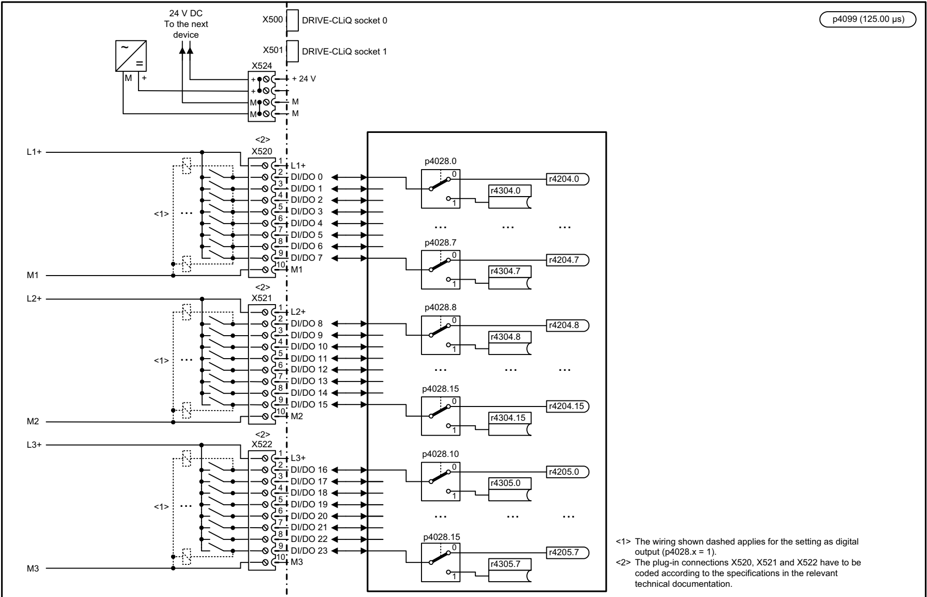
Fig. 3-358 9389 – Overview TM15 (SIMOTION)
