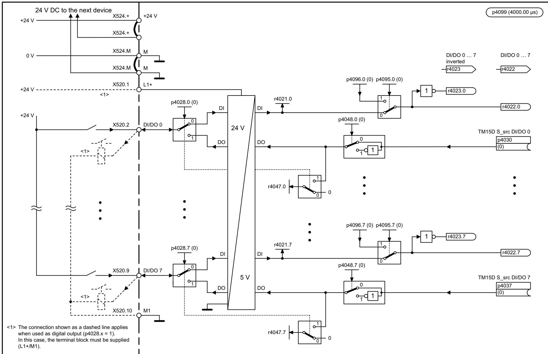
Fig. 3-360 9400 – Digital inputs/outputs, bidirectional (DI/DO 0 ... DI/DO 7)
