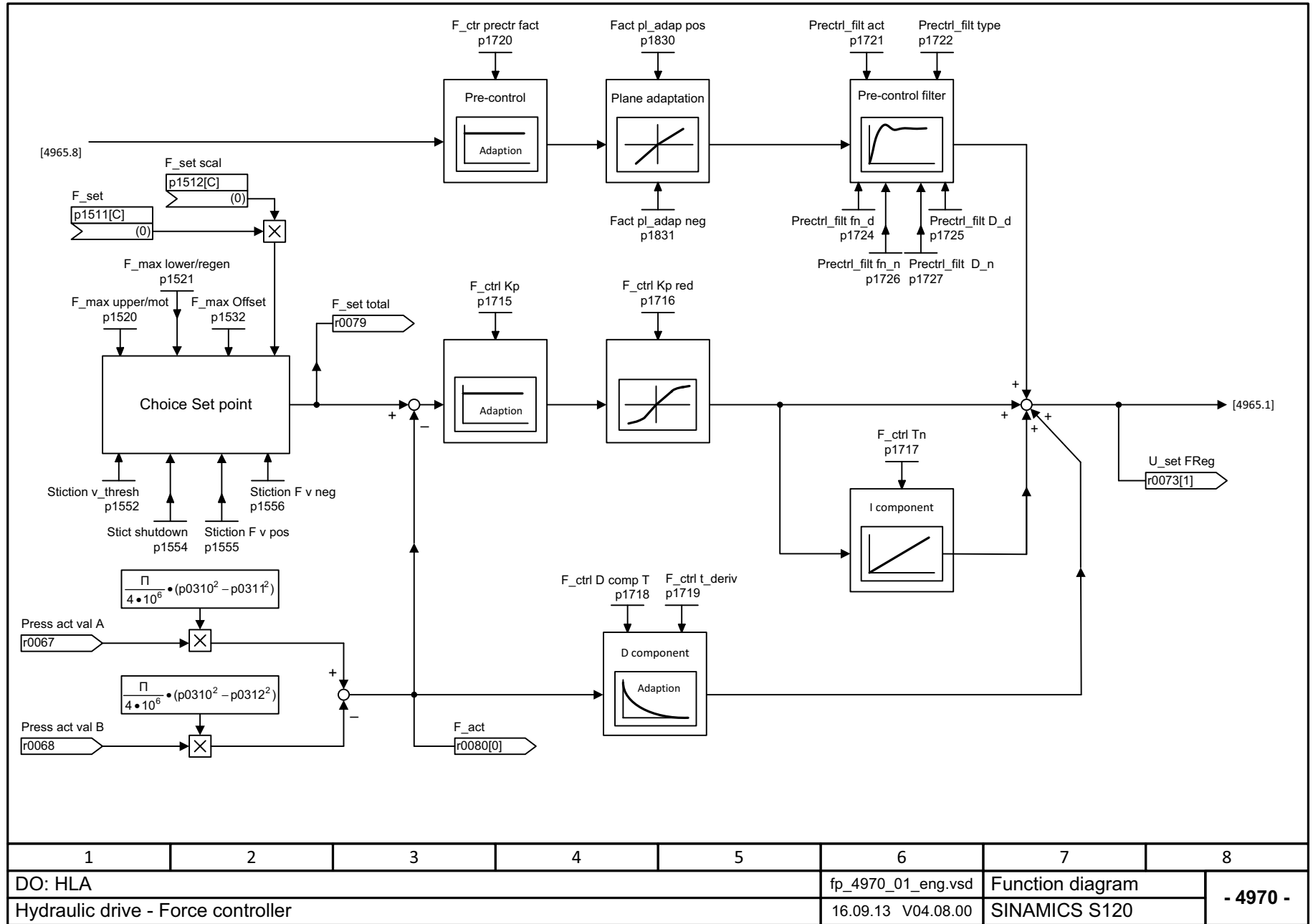
Fig. 3-195 4970 – Force controller
