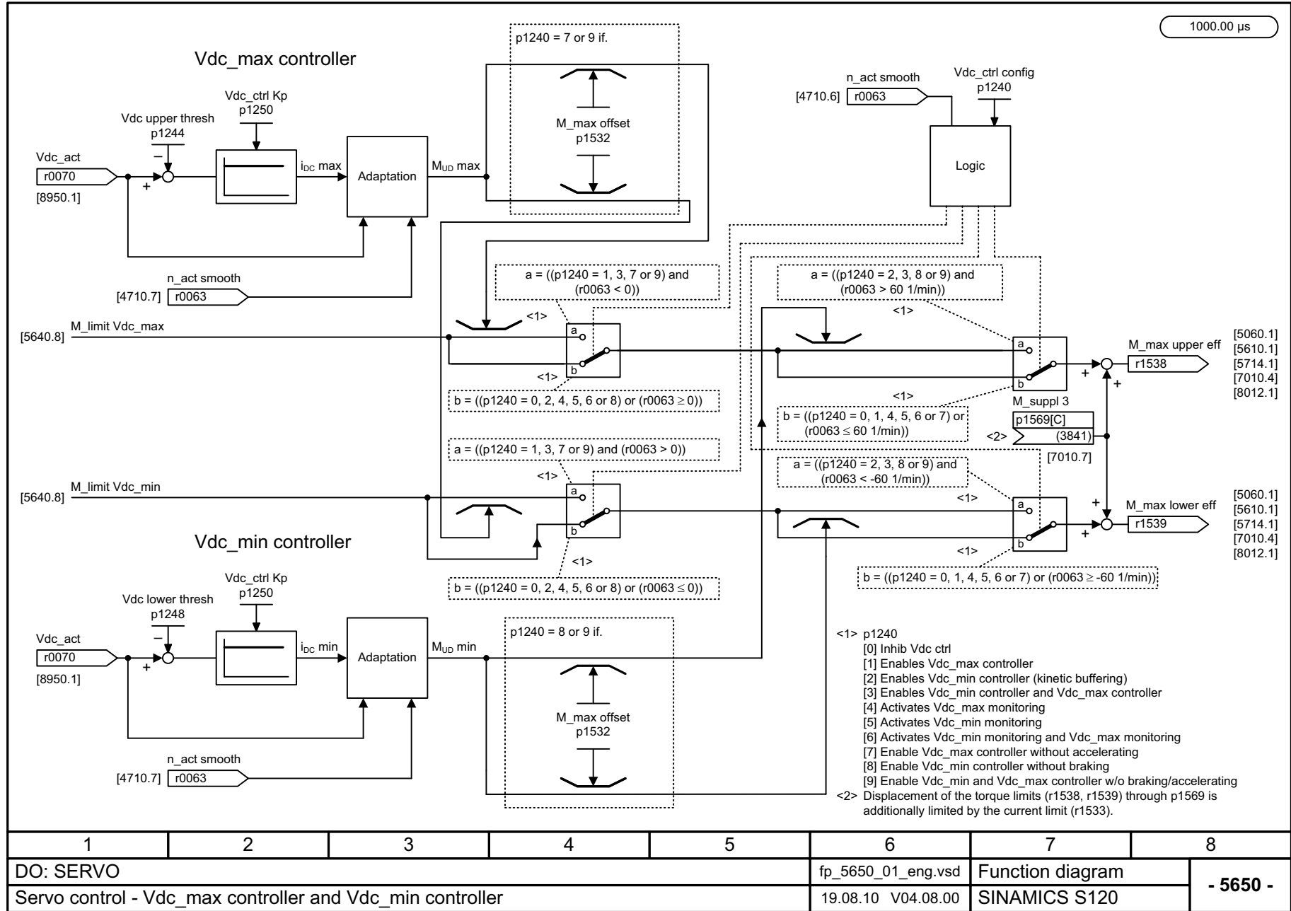
Fig. 3-220 5650 – Vdc_max controller and Vdc_min controller
