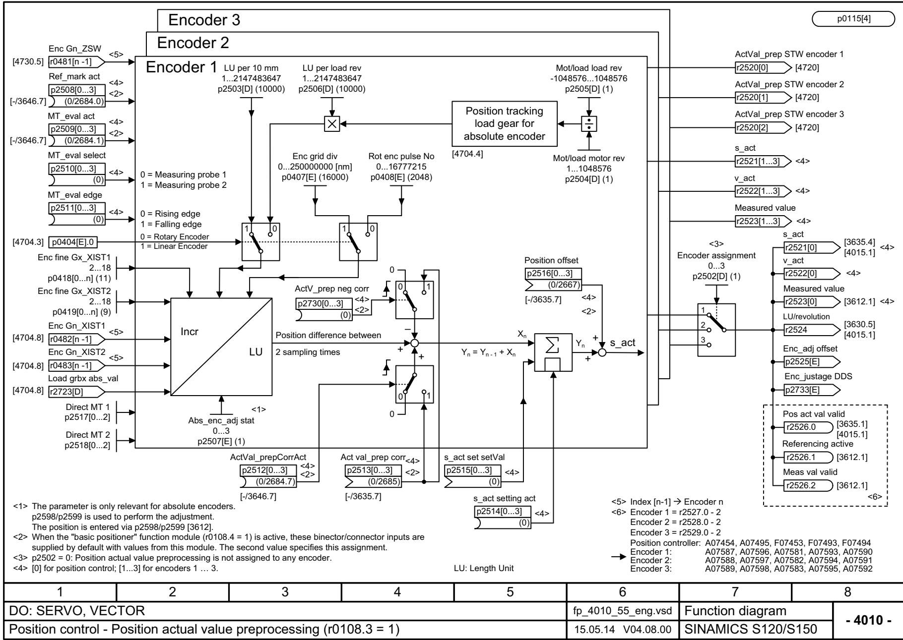
Fig. 3-178 4010 – Position actual value preprocessing (r0108.3 = 1)
