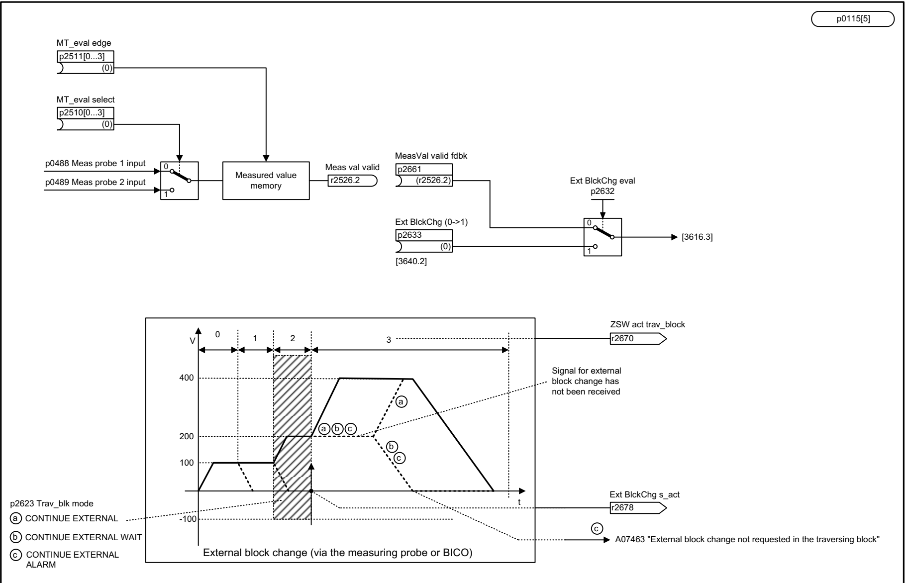
Fig. 3-166 3615 – Traversing block mode, external block change (r0108.4 = 1)
