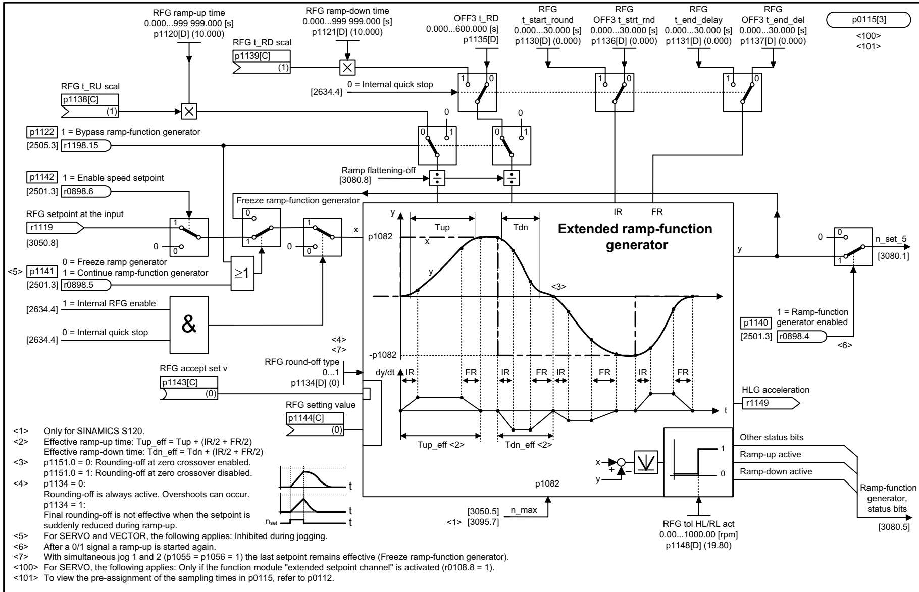
Fig. 3-158 3070 – Extended ramp-function generator
