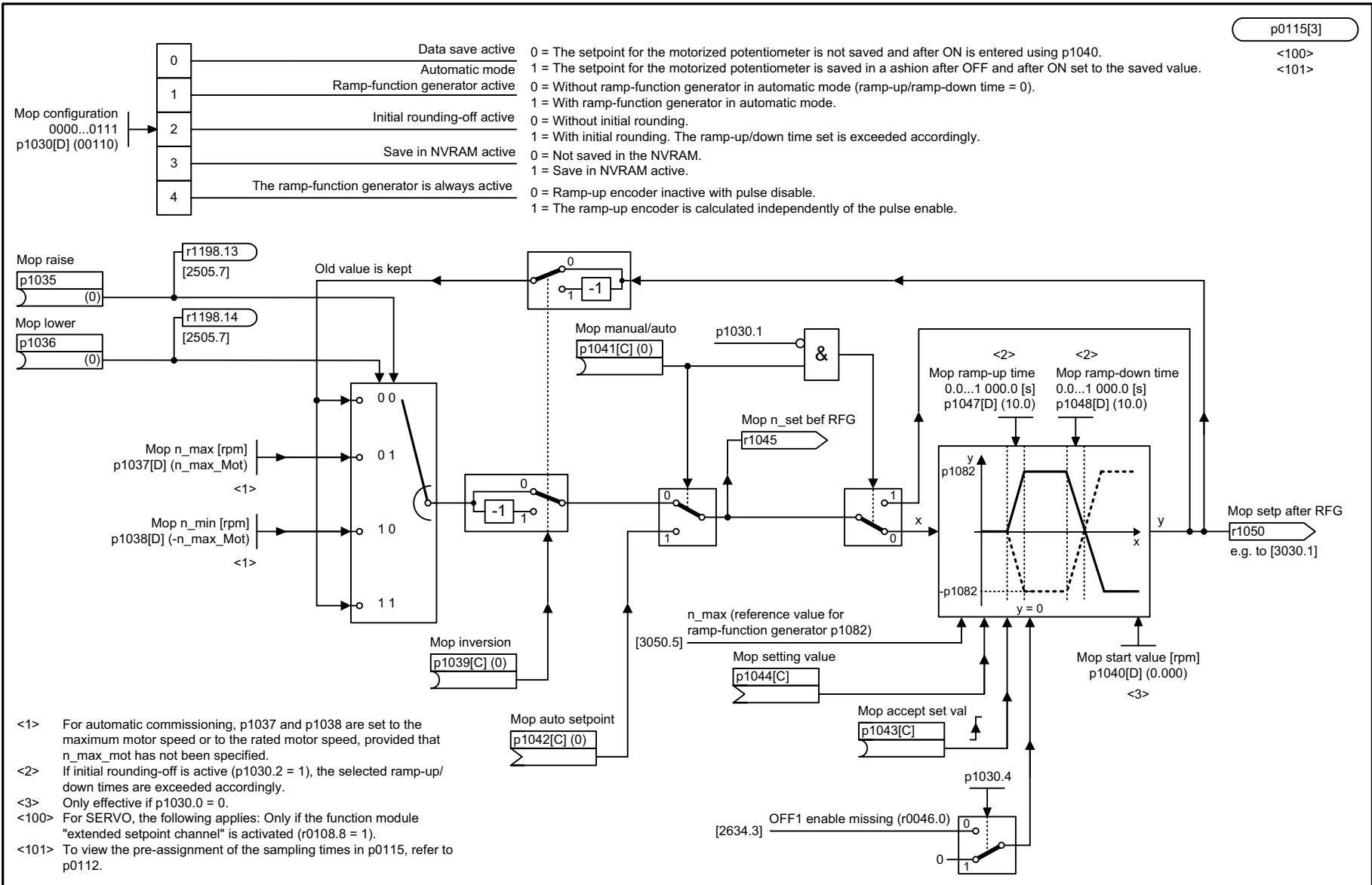
Fig. 3-153 3020 – Motorized potentiometer
