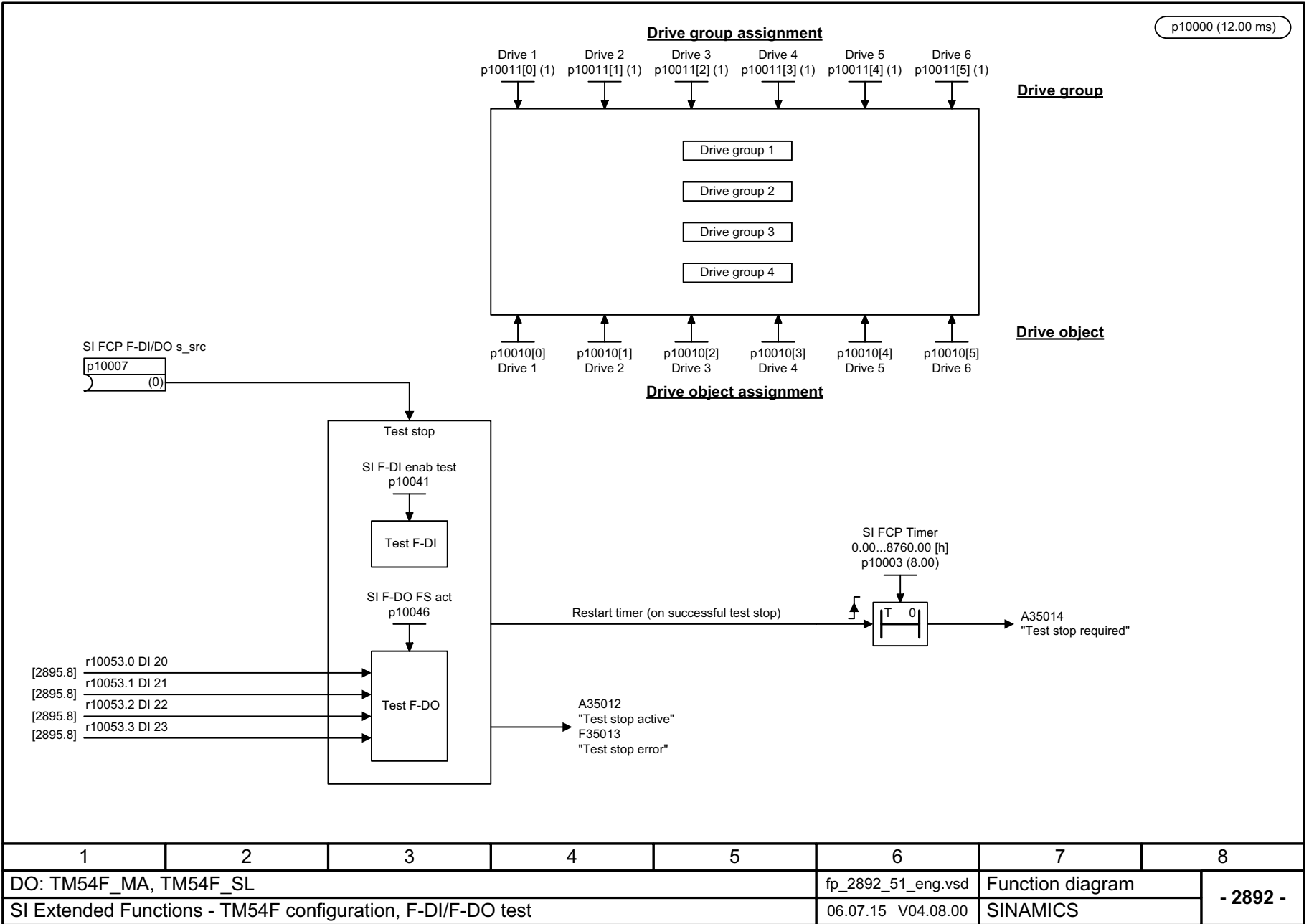
Fig. 3-139 2892 – Configuration, F-DI/F-DO Test
