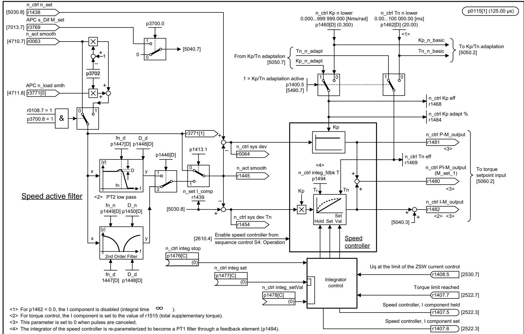
Fig. 3-206 5040 – Speed controller with encoder
