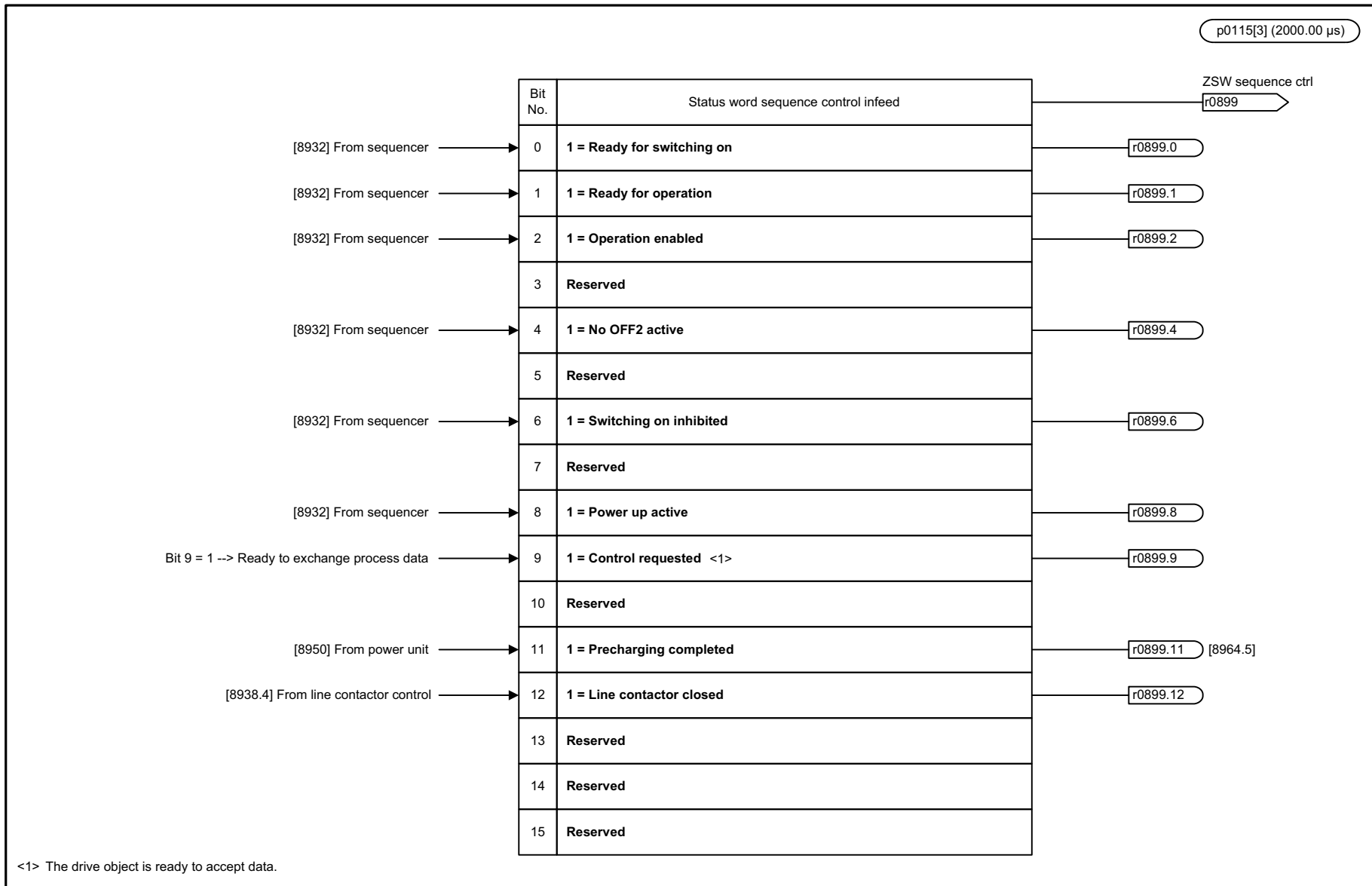
Fig. 3-335 8926 – Status word, sequence control infeed
