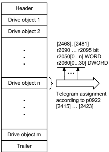
Fig. 3-51 2439 – PZD receive signals interconnection, profile-specific
