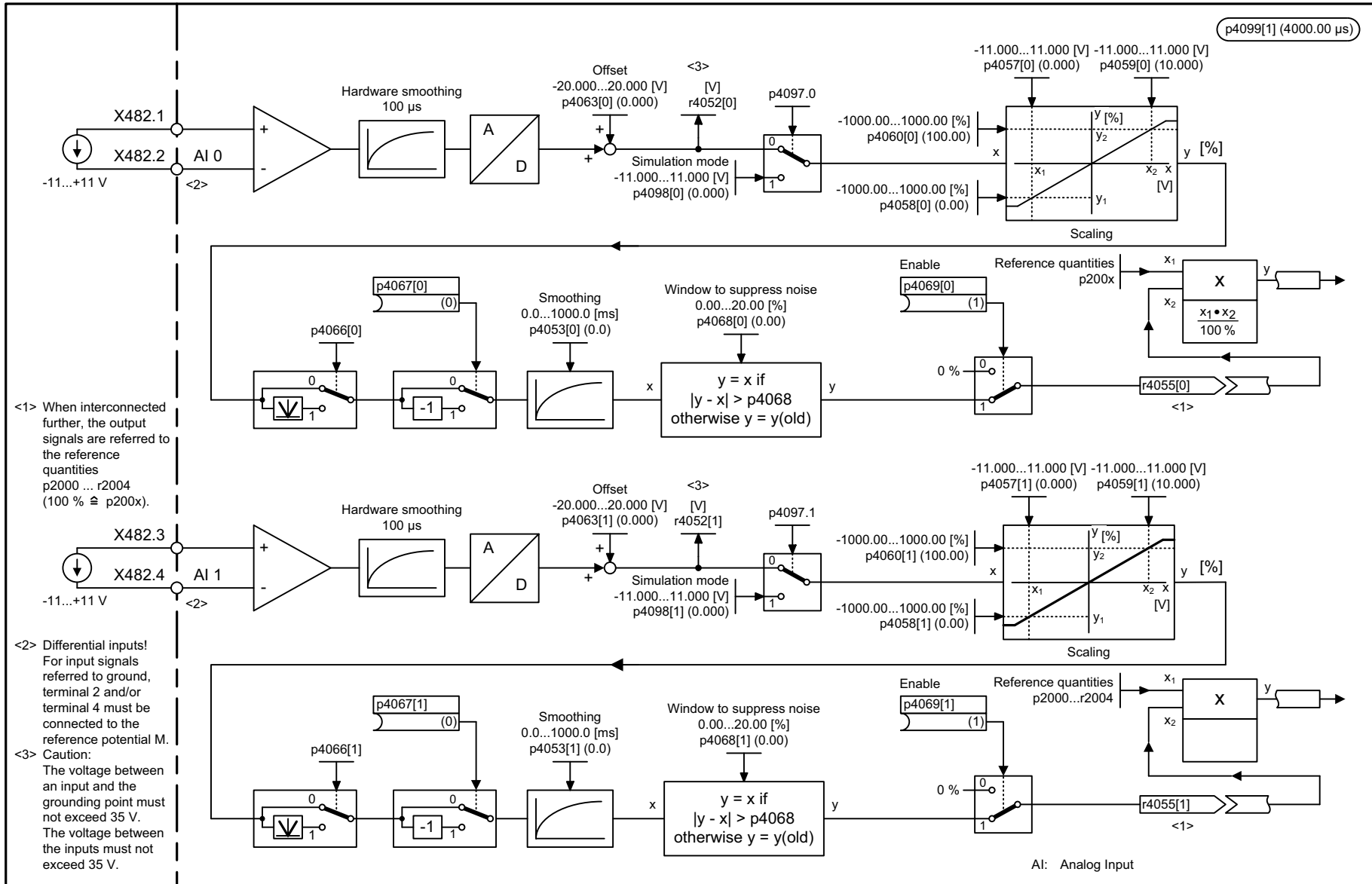
Fig. 3-350 9104 – Analog inputs (AI 0 ... AI 1)
