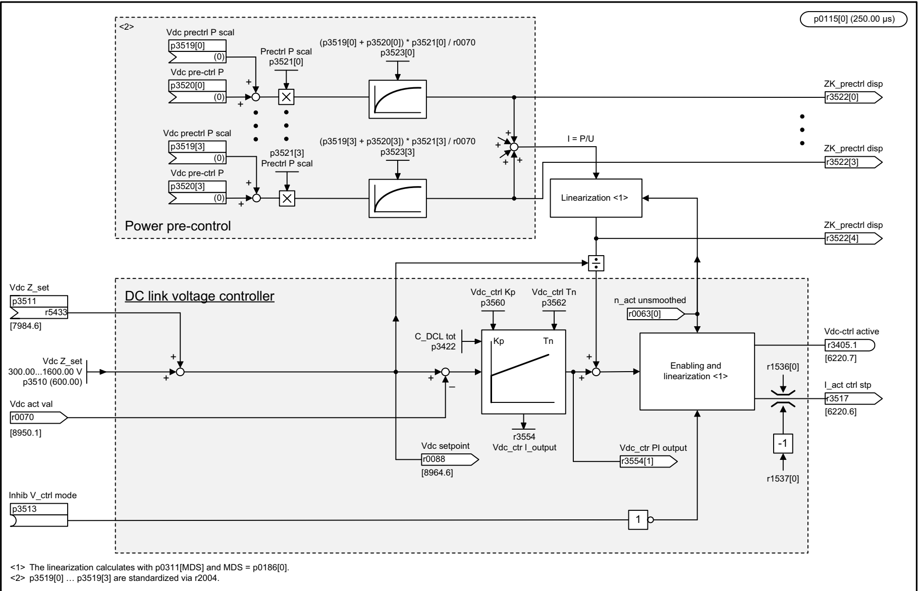
Fig. 3-275 7960 – DC link voltage controller (r0108.16 = 1)
