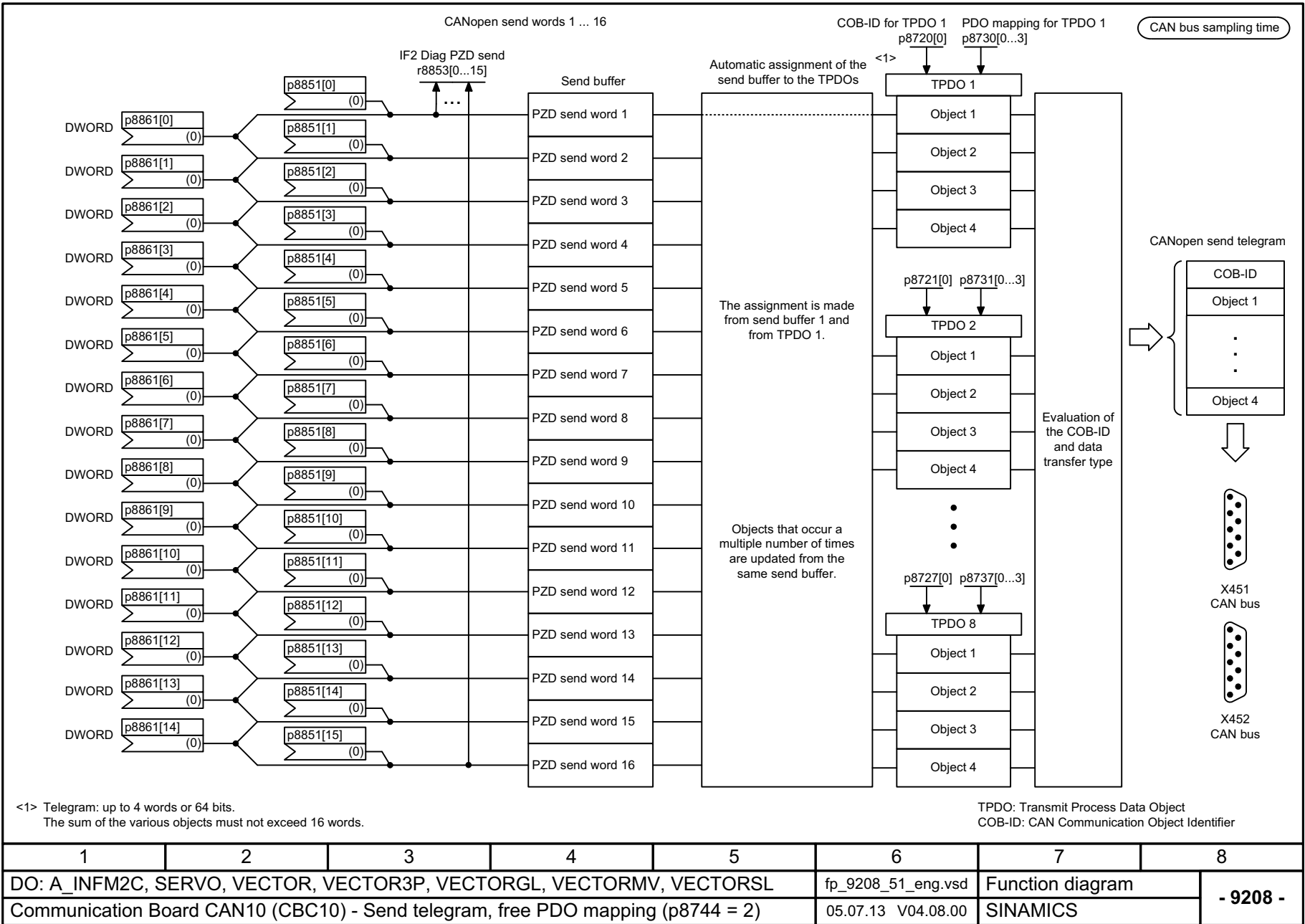
Fig. 3-354 9208 – Send telegram, free PDO mapping (p8744 = 2)
