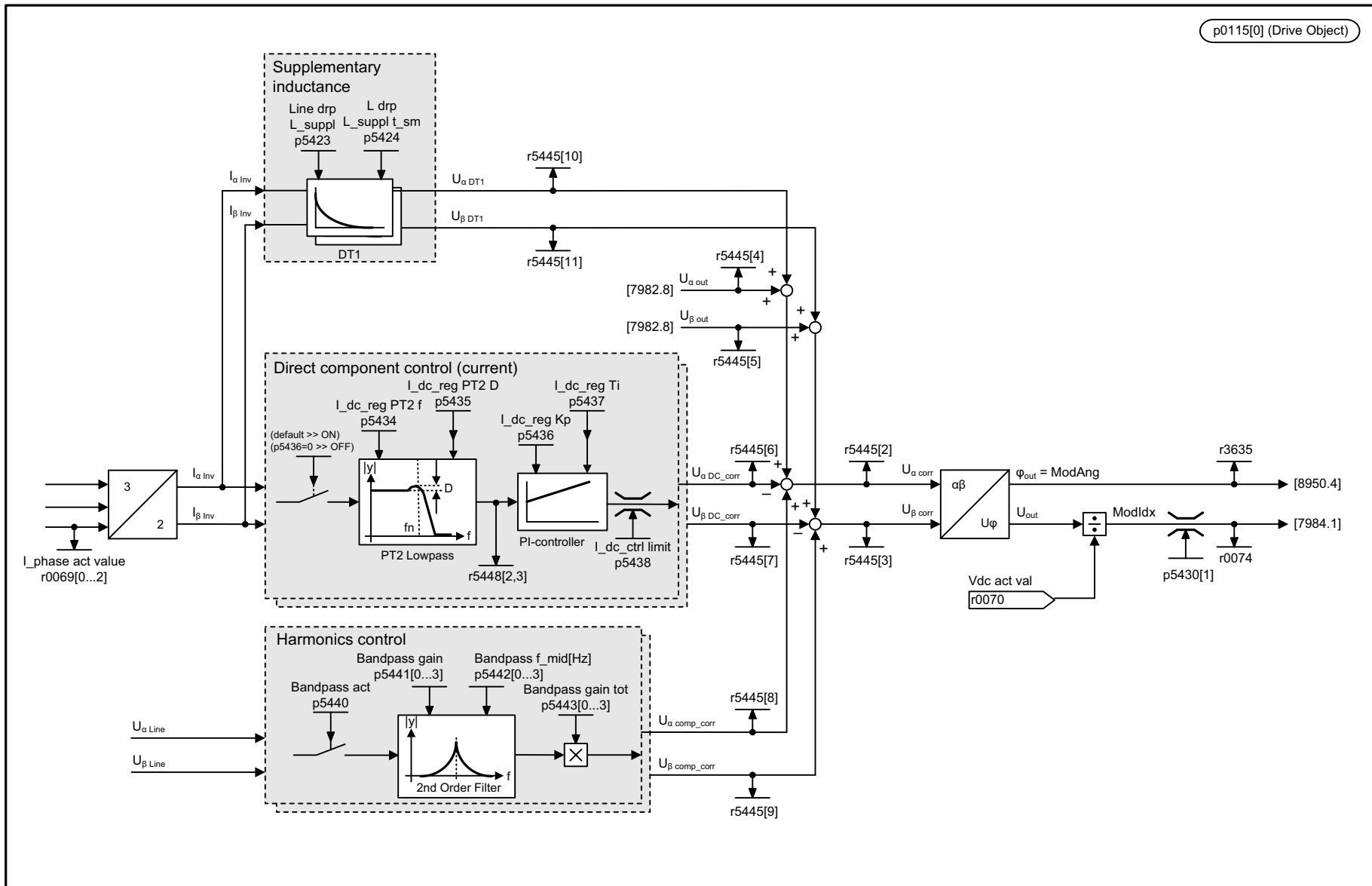
Fig. 3-277 7983 – Direct component control, harmonics control
