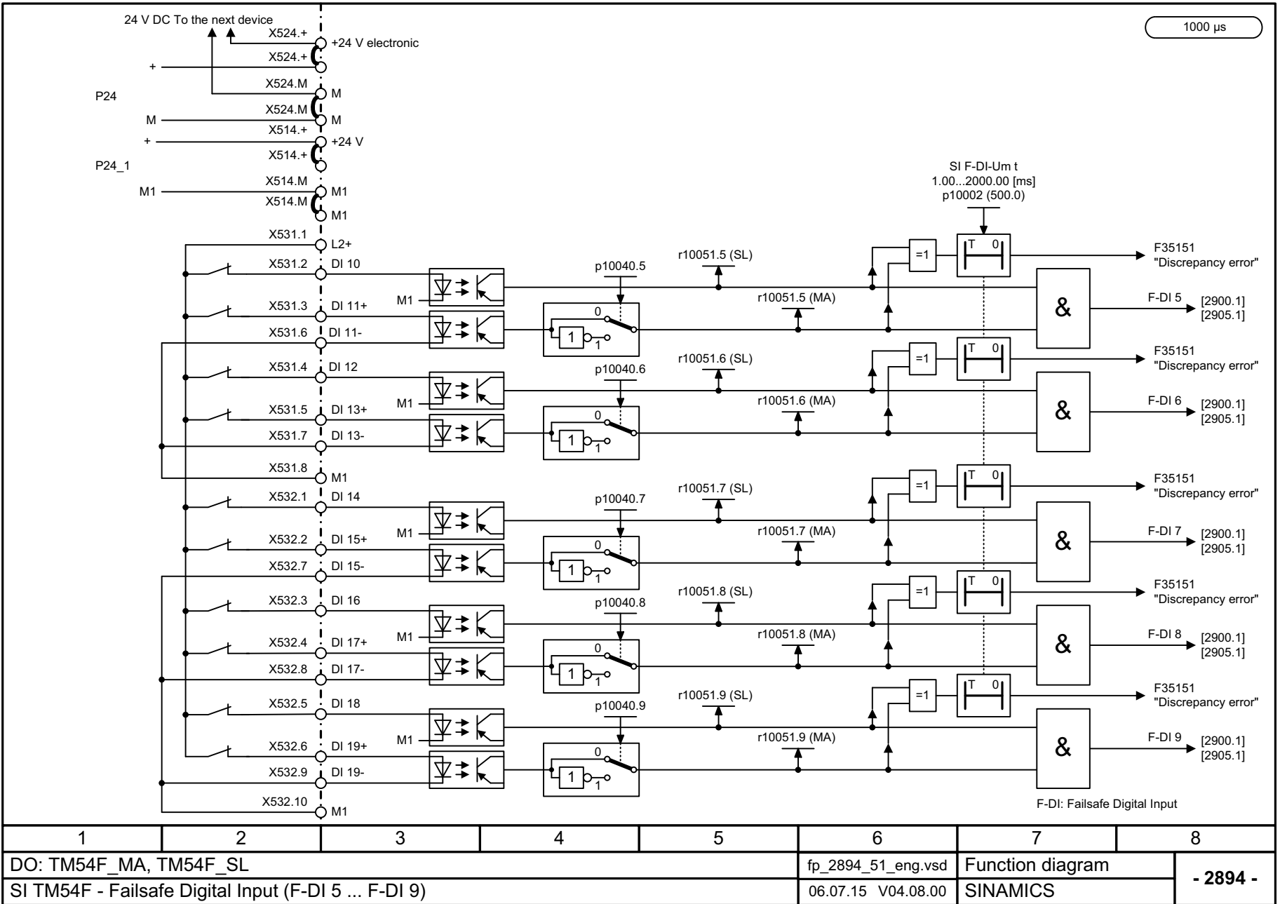
Fig. 3-141 2894 – Fail-safe digital inputs (F-DI 5 ... F-DI 9)
