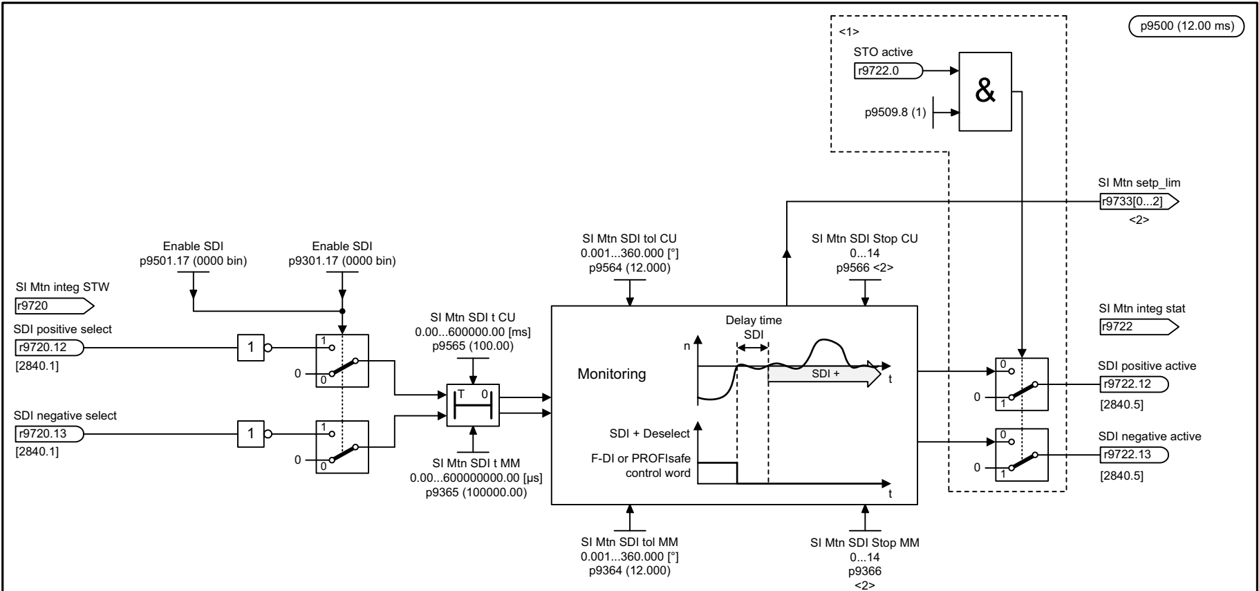
Fig. 3-124 2824 - SDI (Safe Direction)
