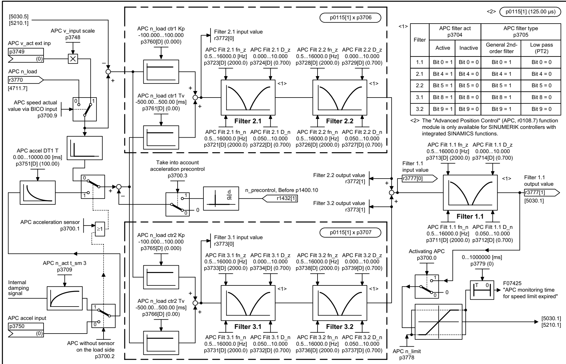
Fig. 3-264 7012 - Advanced Positioning Control (APC, r0108.7 = 1)
