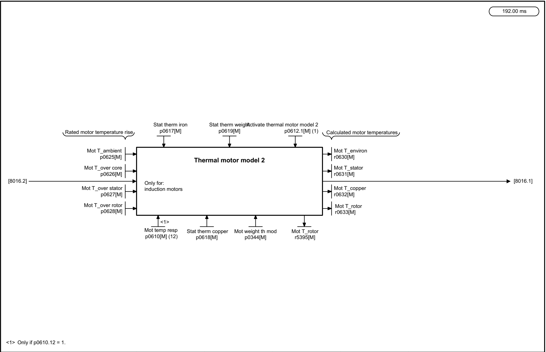
Fig. 3-299 8018 – Motor temperature model 2
