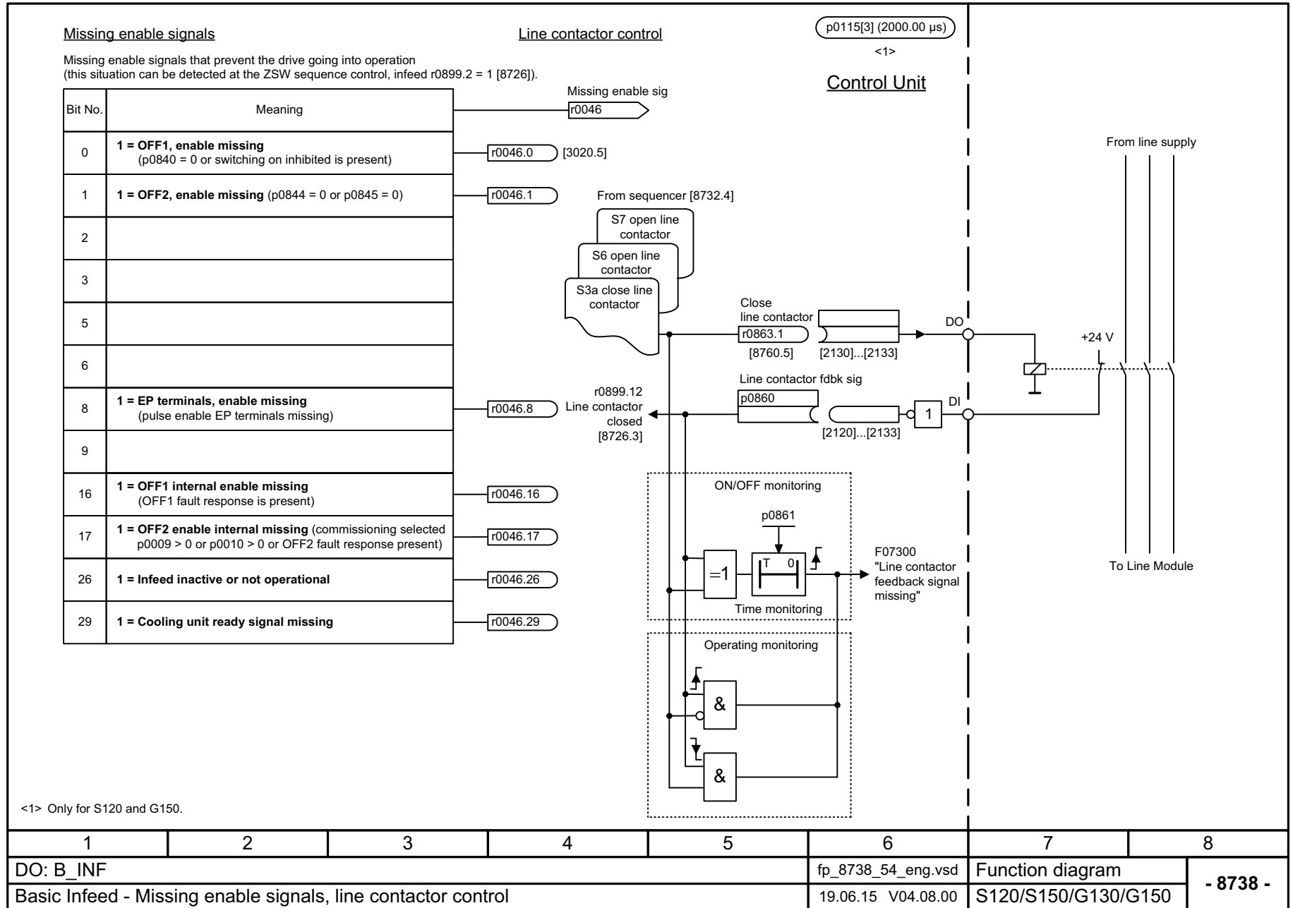
Fig. 3-321 8738 – Missing enable signals, line contactor control
