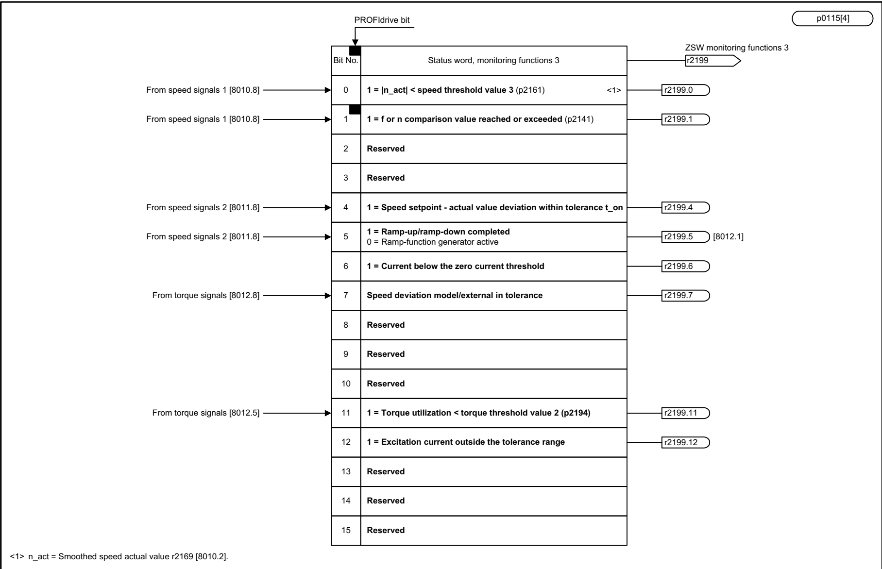
Fig. 3-102 2537 – Status word, monitoring functions 3
