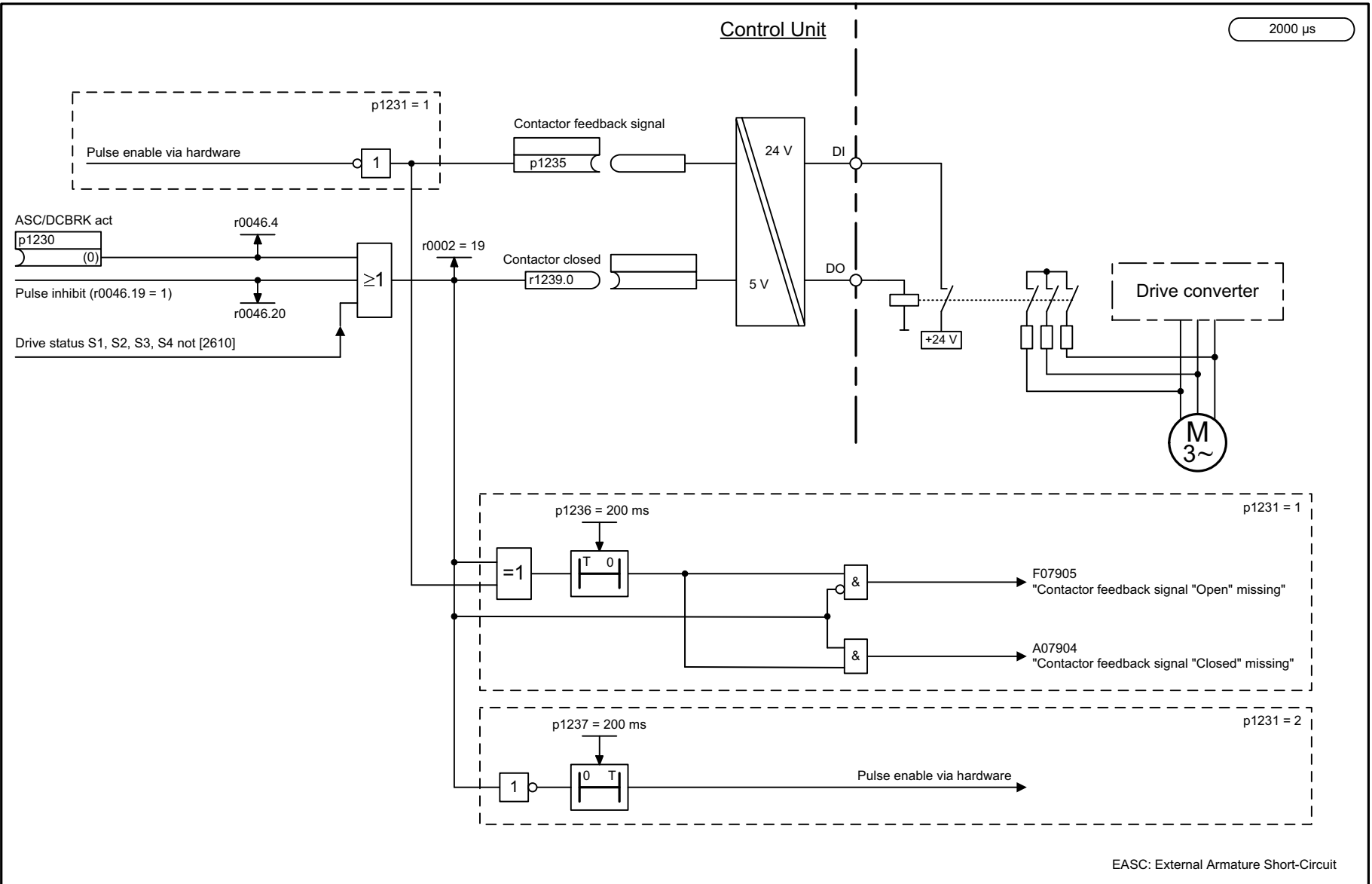
Fig. 3-266 7014 – External armature short-circuit (EASC, p0300 = 2xx or 4xx)
