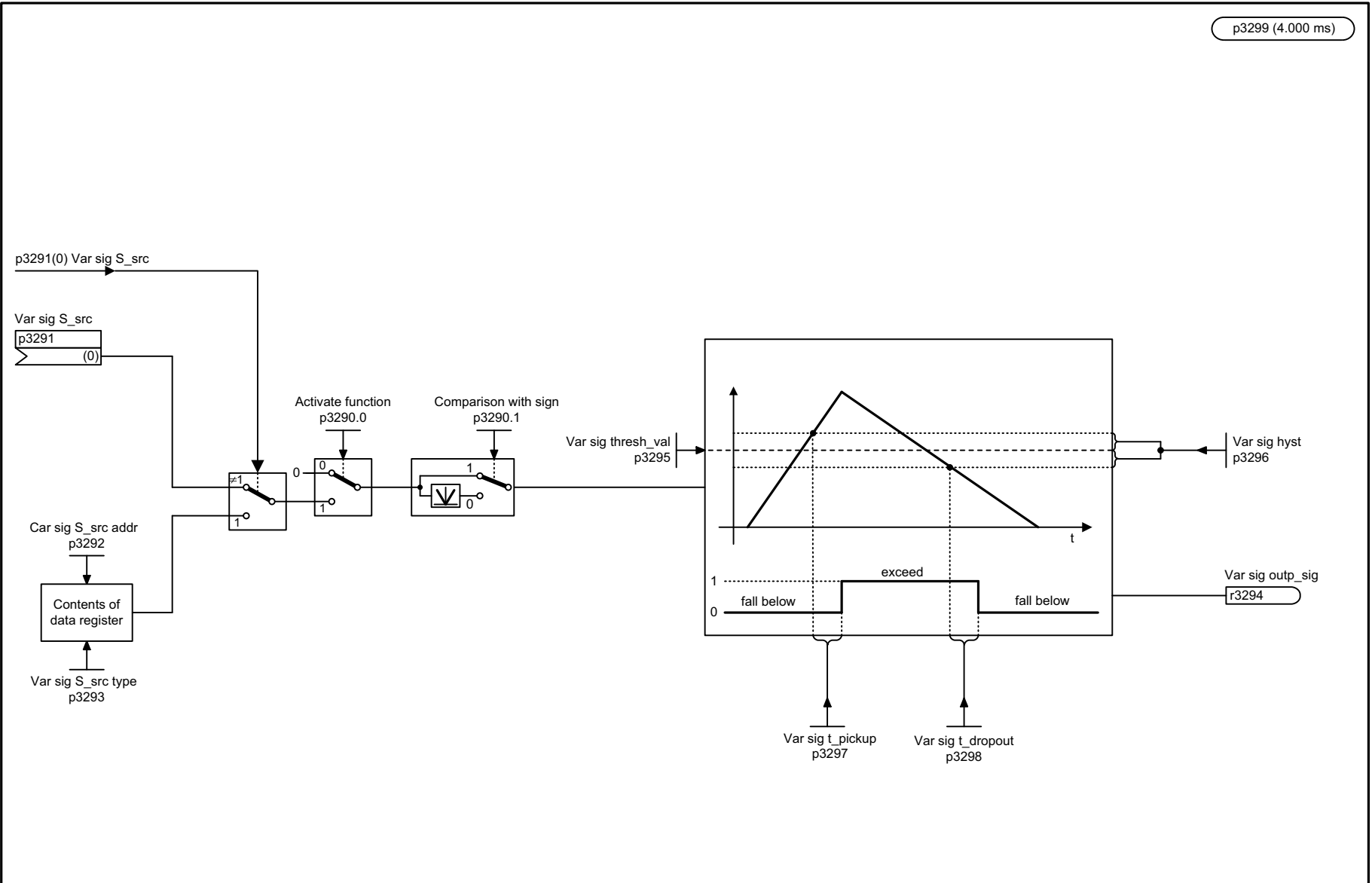
Fig. 3-213 5301 – Signaling function variable
