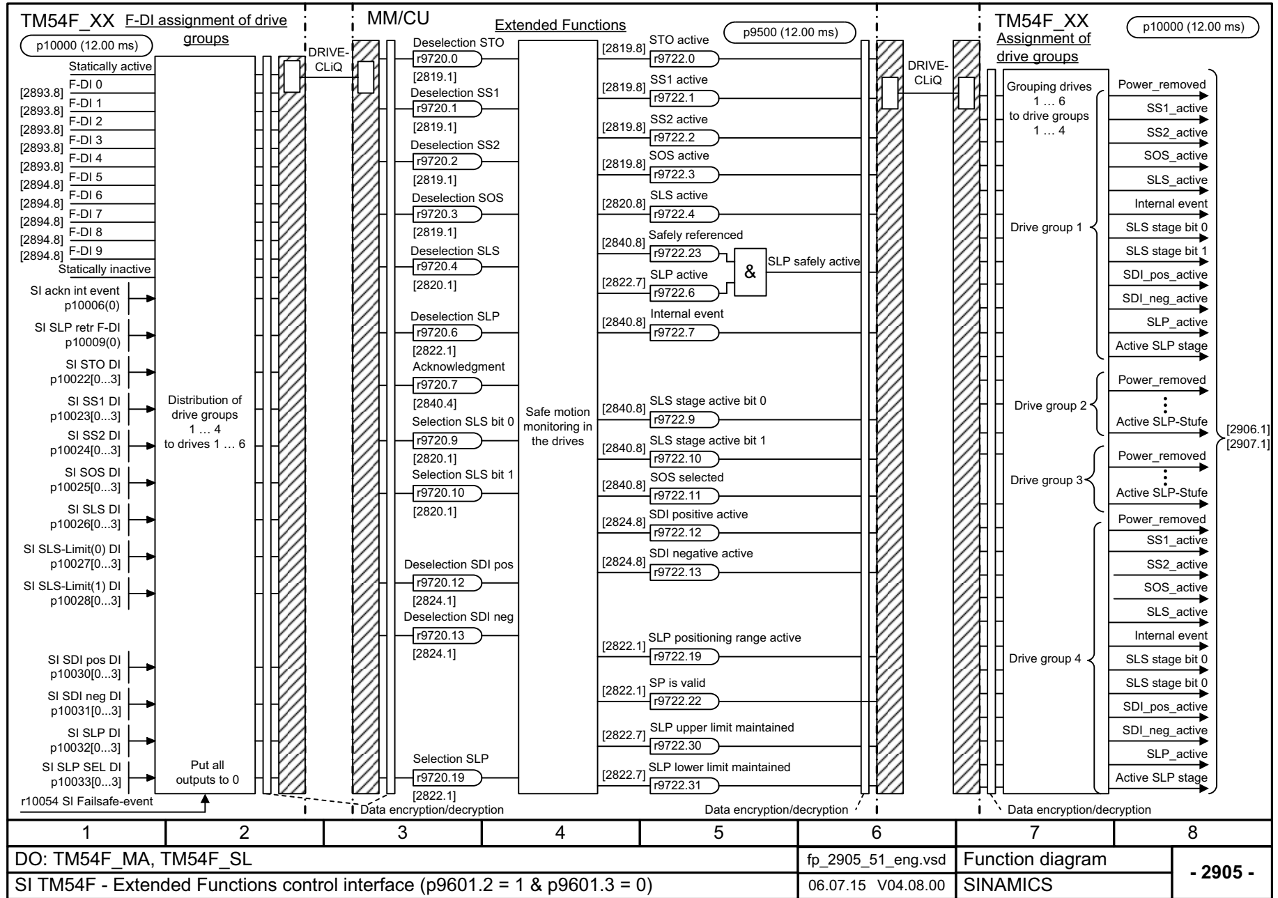
Fig. 3-146 2905 – Extended Functions control interface (p9601.2 = 1 & p9601.3 = 0)
