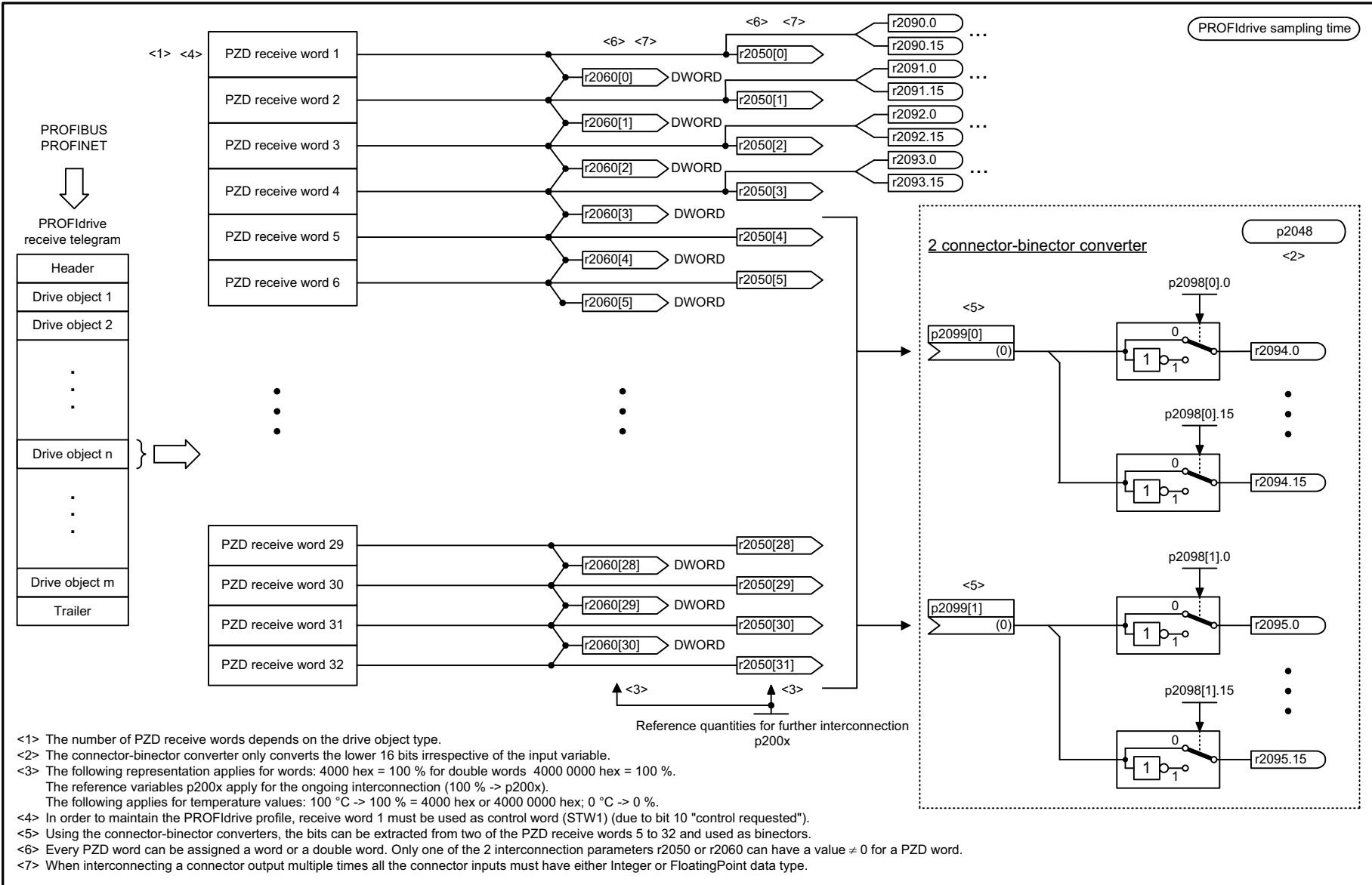
Fig. 3-73 2468 - IF1 receive telegram, free interconnection via BICO (p0922 = 999)
