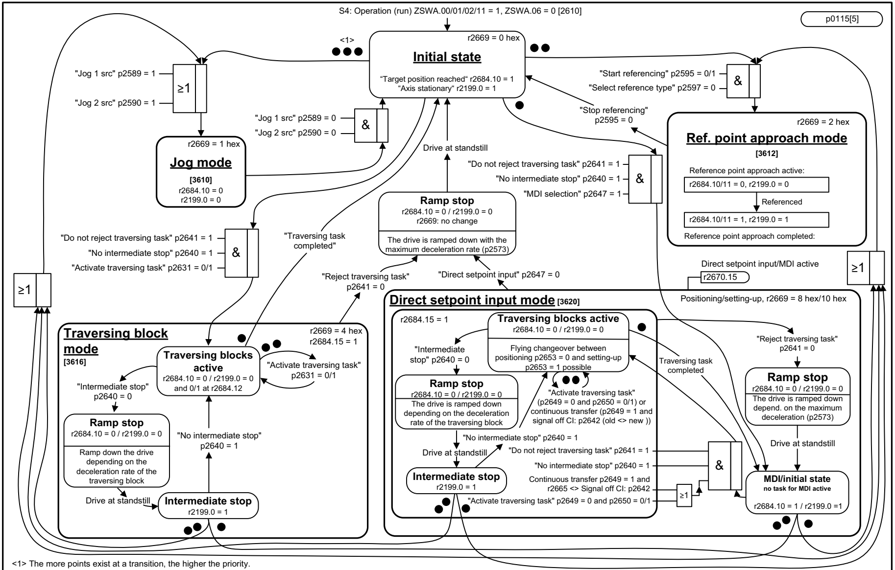
Fig. 3-171 3625 - Mode control (r0108.4 = 1)
