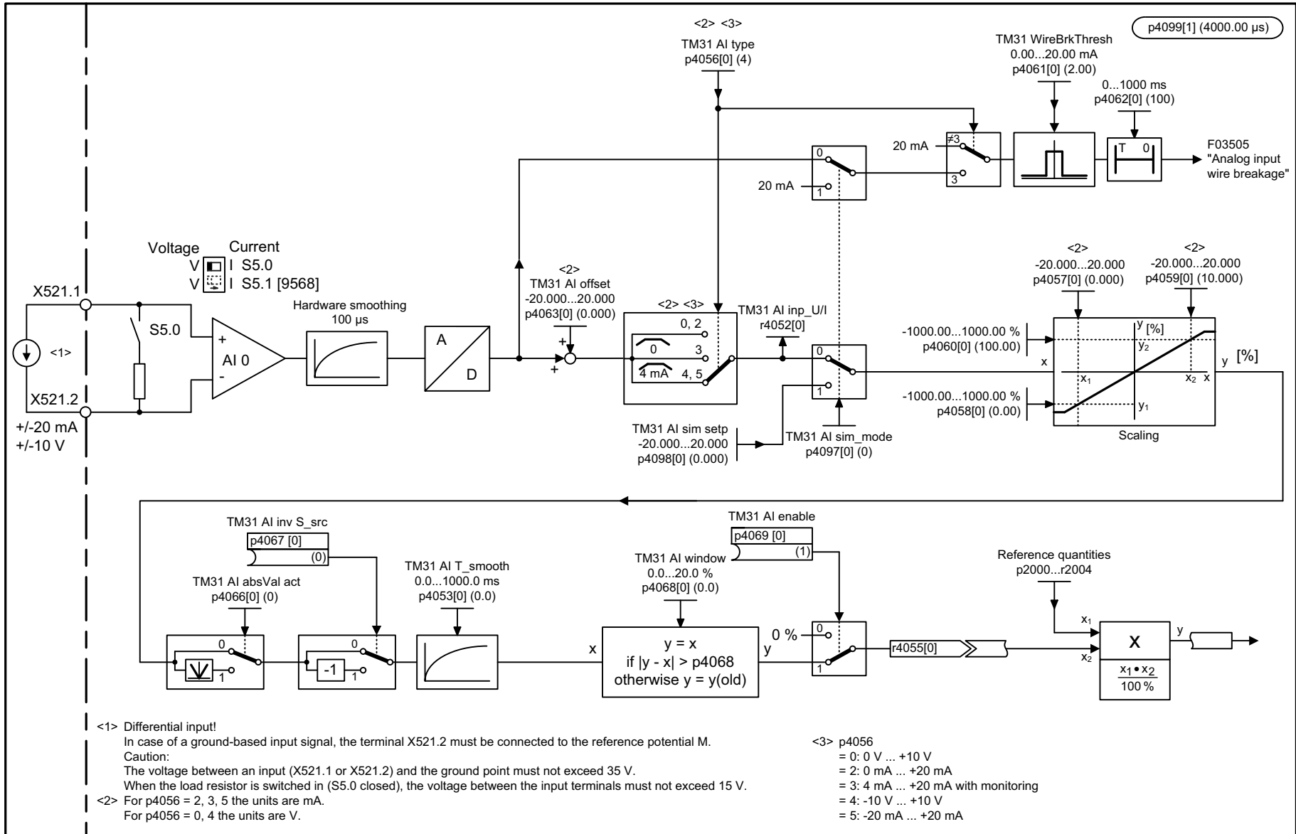
Fig. 3-370 9566 – Analog input 0 (AI 0)
