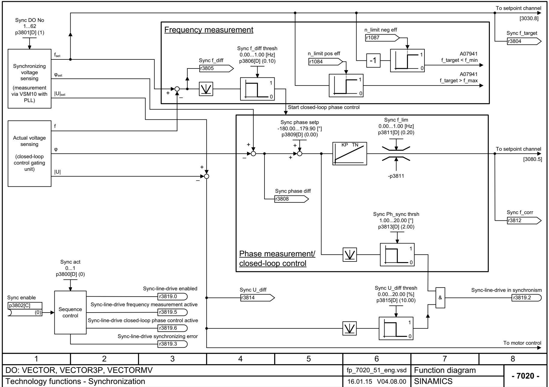
Fig. 3-269 7020 – Synchronization
