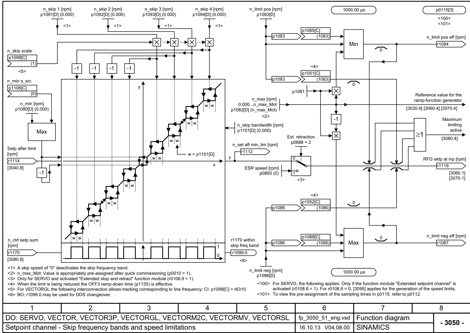
Fig. 3-156 3050 – Skip frequency bands and speed limitations
