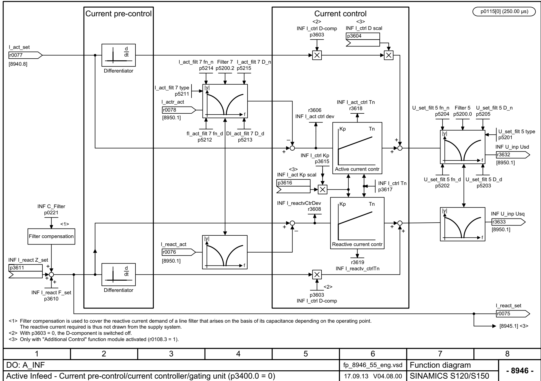
Fig. 3-341 8946 – Current pre-control/current controller/gating unit (p3400.0 = 0)
