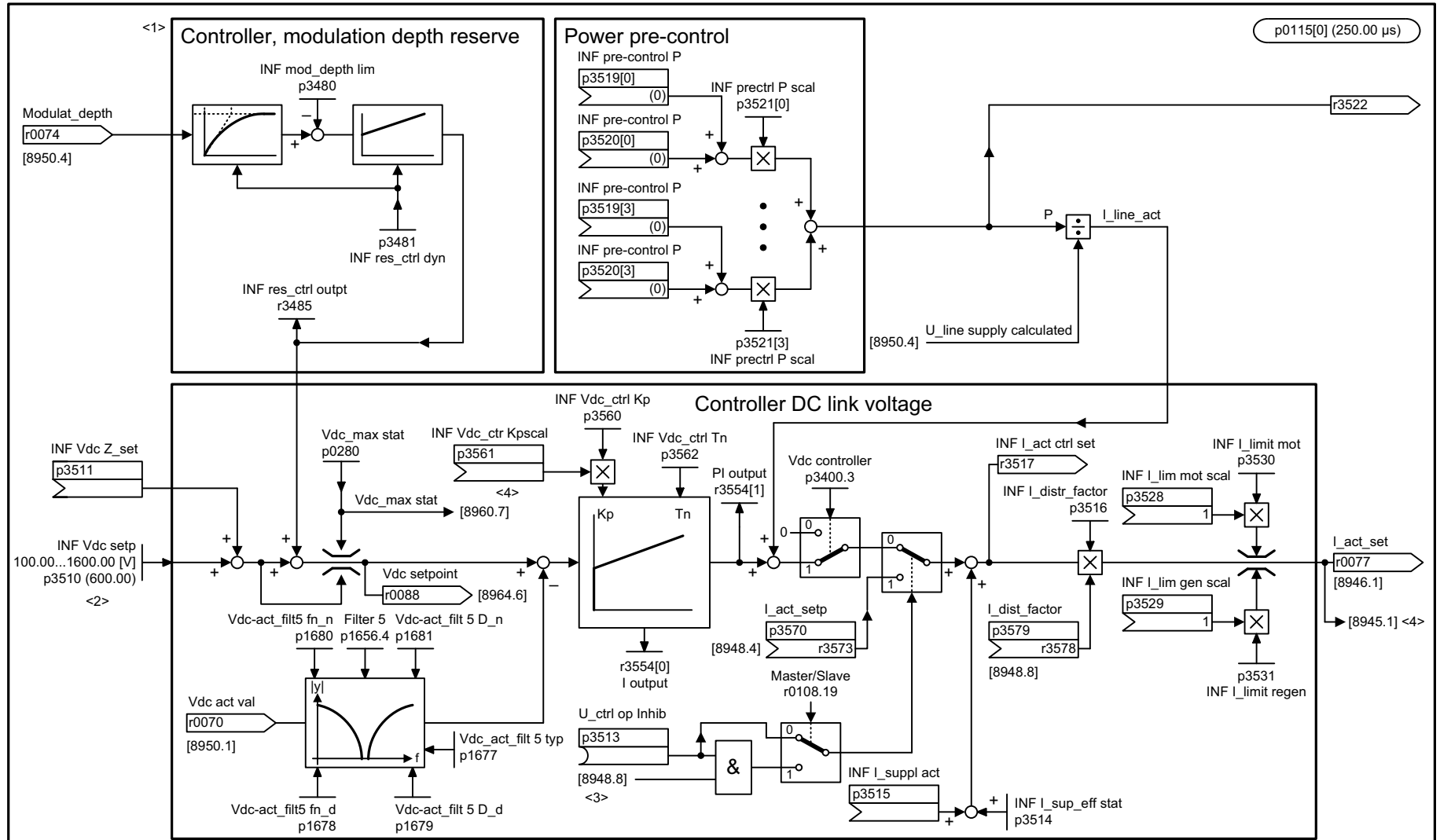
Fig. 3-339 8940 – Controller modulation depth reserve/controller DC link voltage (p3400.0 = 0)
