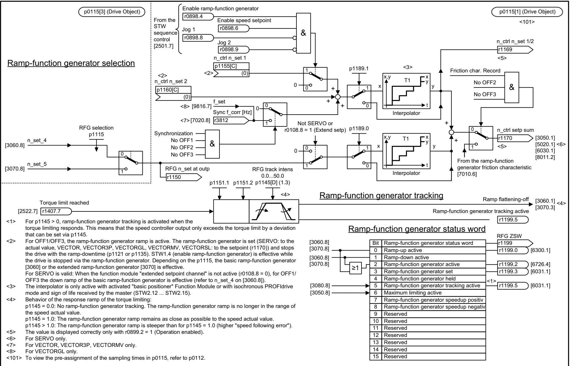
Fig. 3-159 3080 – Ramp-function generator selection, status word, tracking
