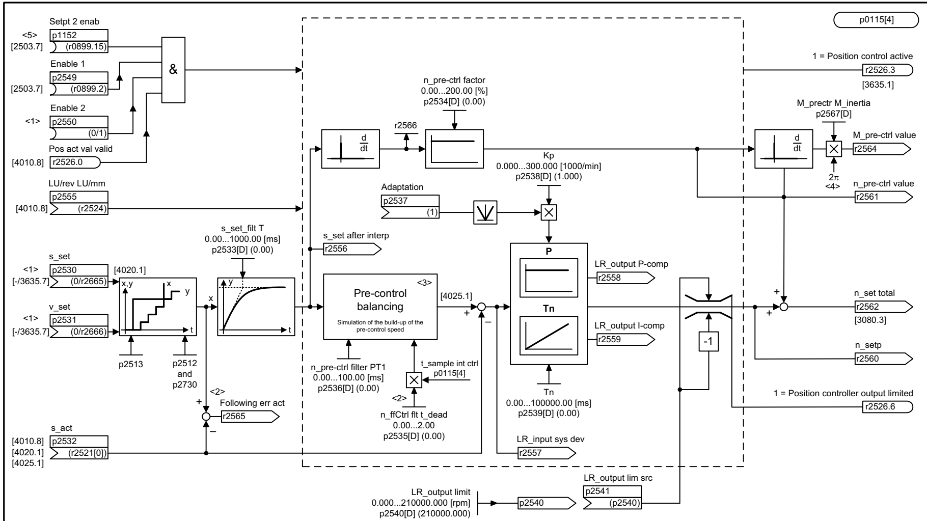
Fig. 3-179 4015 – Position controller (r0108.3 = 1)
