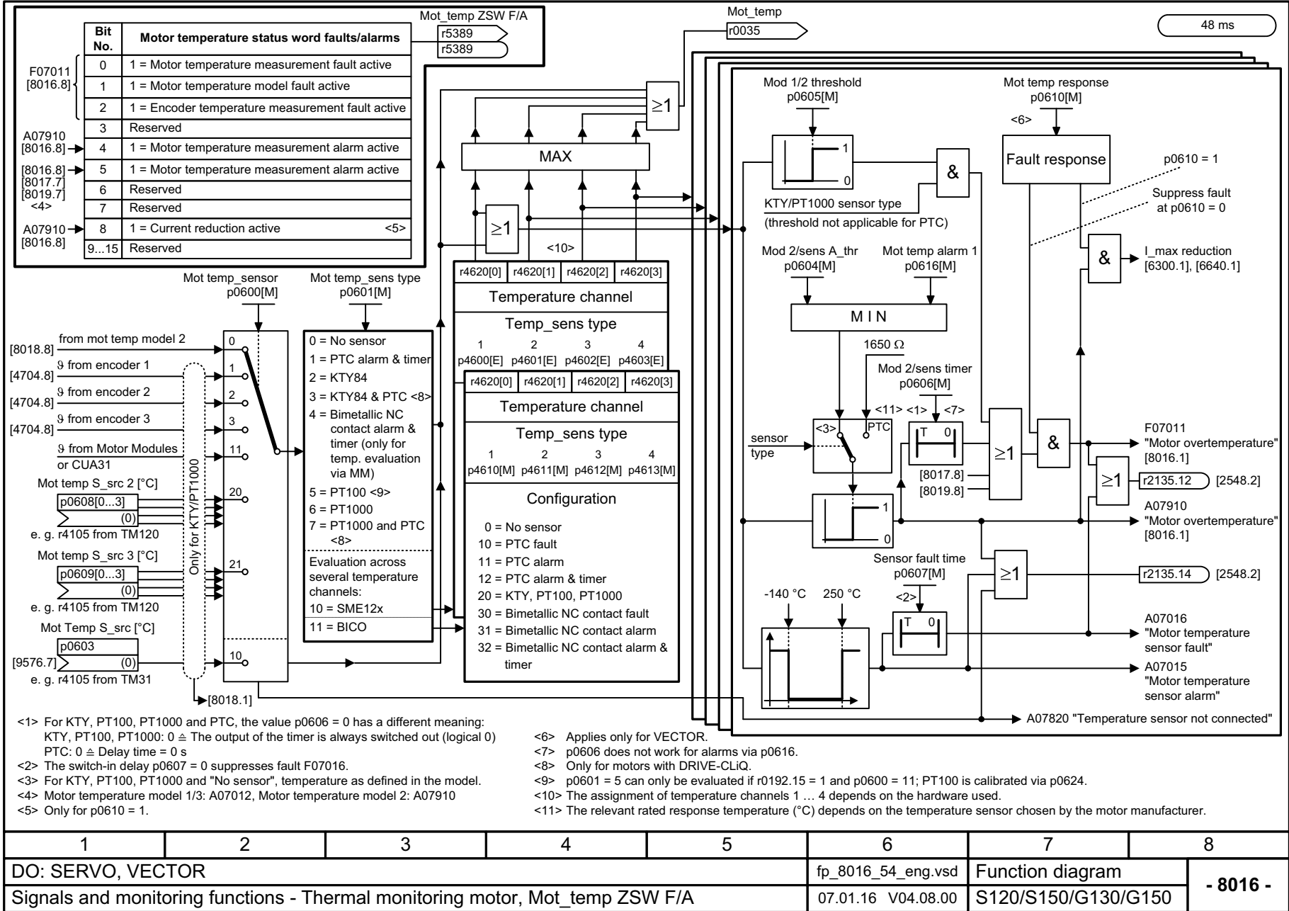
Fig. 3-297 8016 – Thermal motor monitoring, motor temperature ZSW F/A
