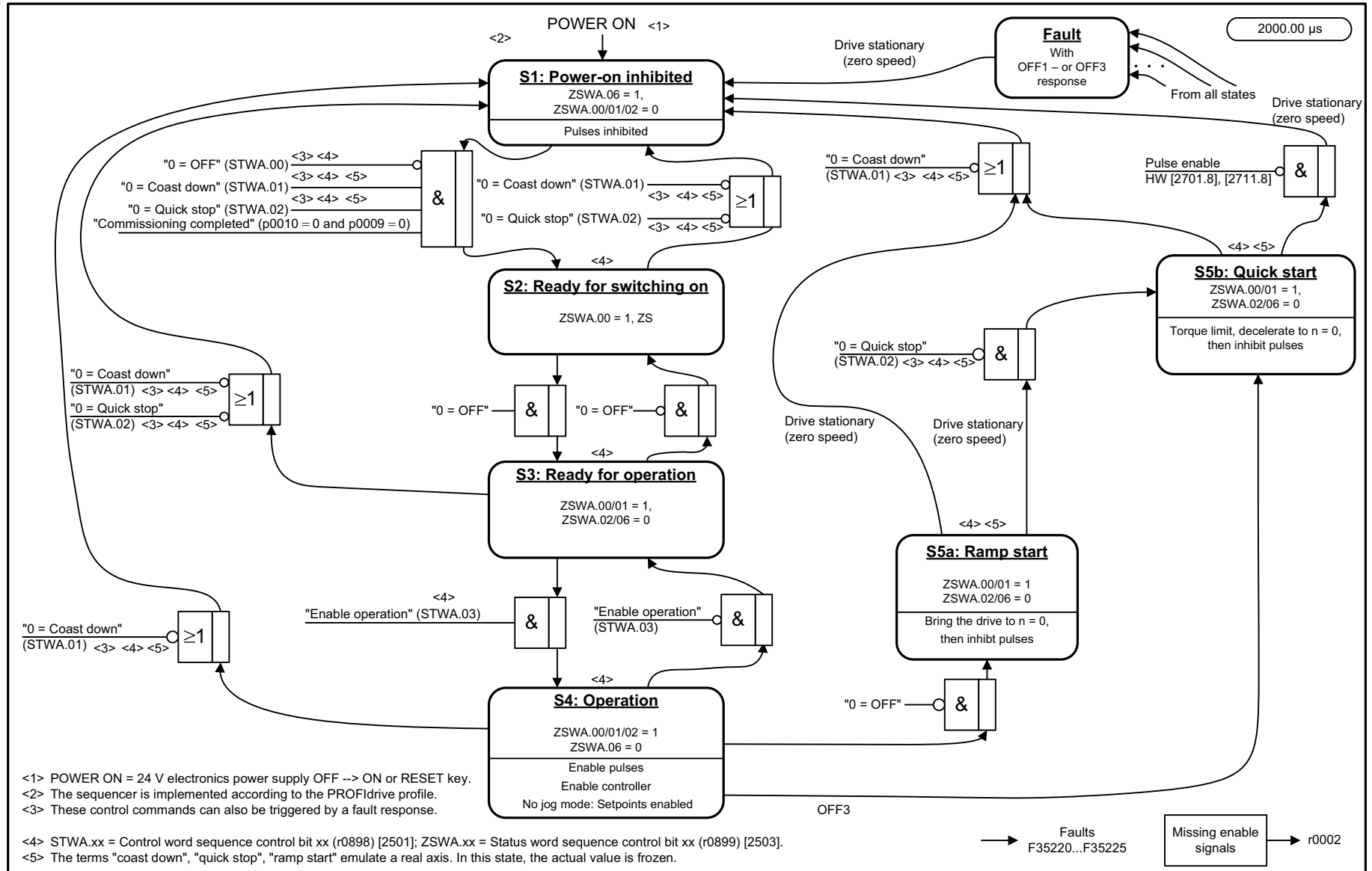
Fig. 3-391 9682 – Sequencer (p4400 = 0)
