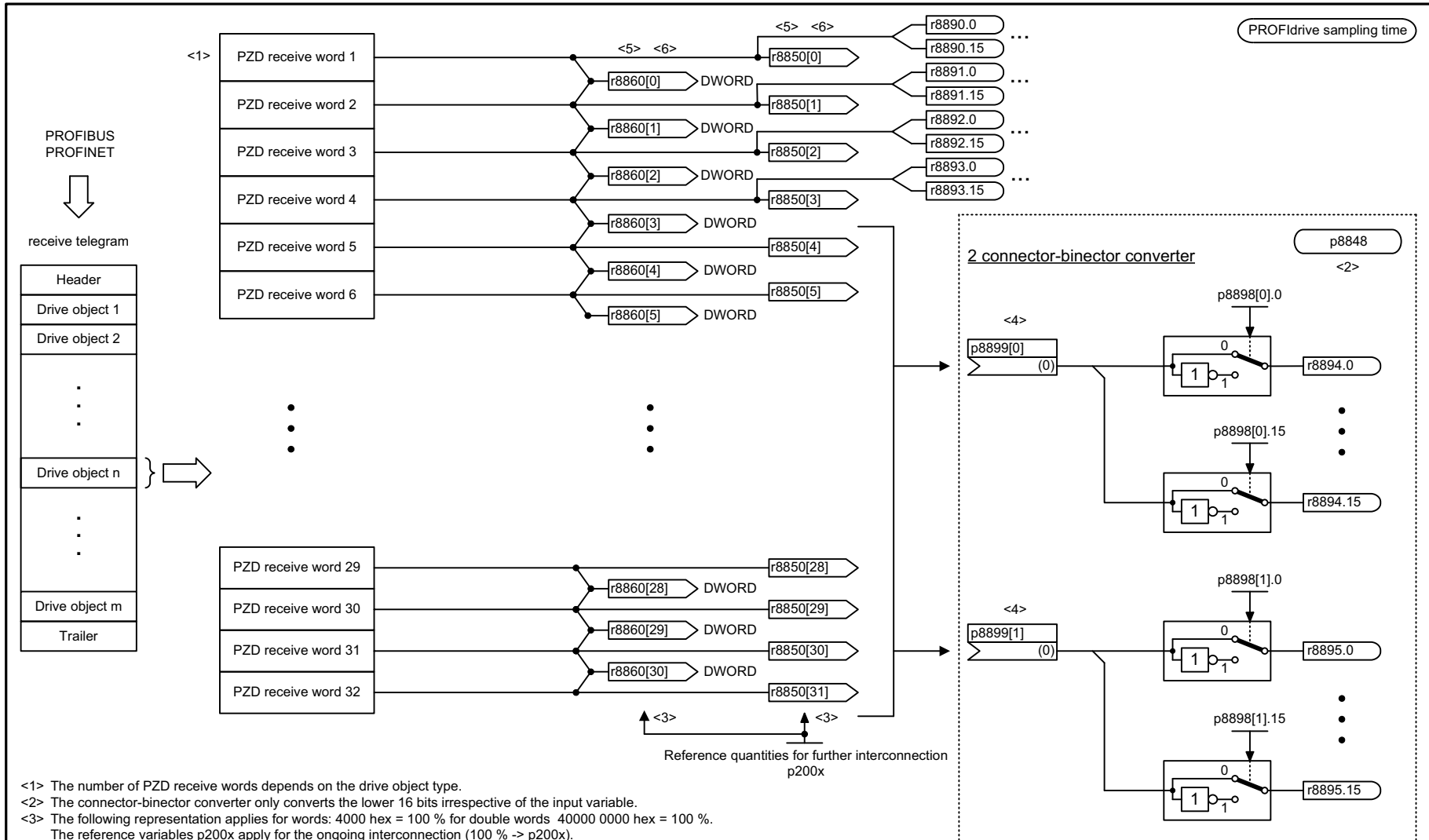
Fig. 3-82 2485 – IF2 receive telegram, free interconnection
