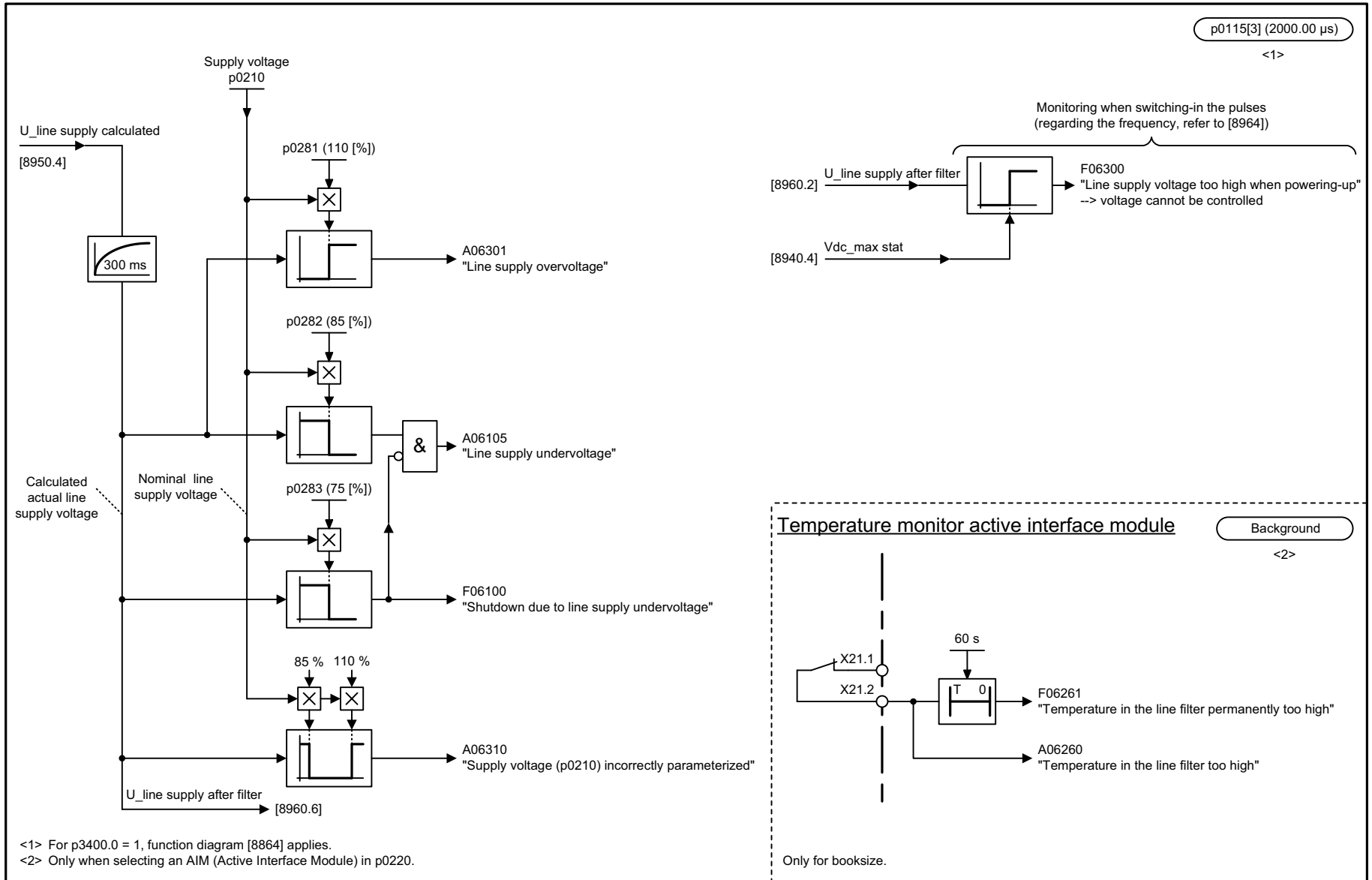
Fig. 3-345 8960 – Signals and monitoring functions, line supply voltage monitoring (p3400.0 = 0)
