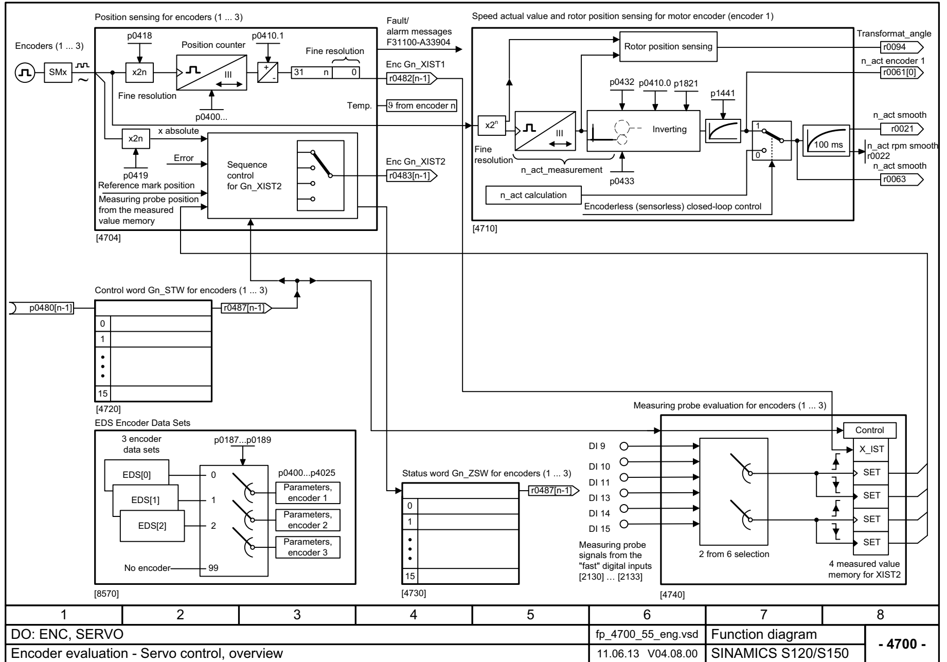
Fig. 3-182 4700 – Servo control, overview
