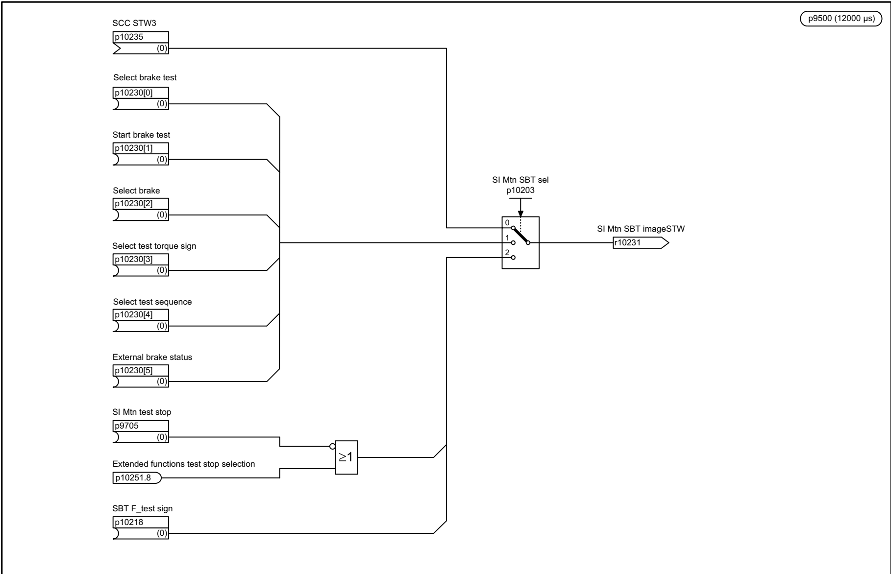
Fig. 3-127 2837 – Selection of active control word
