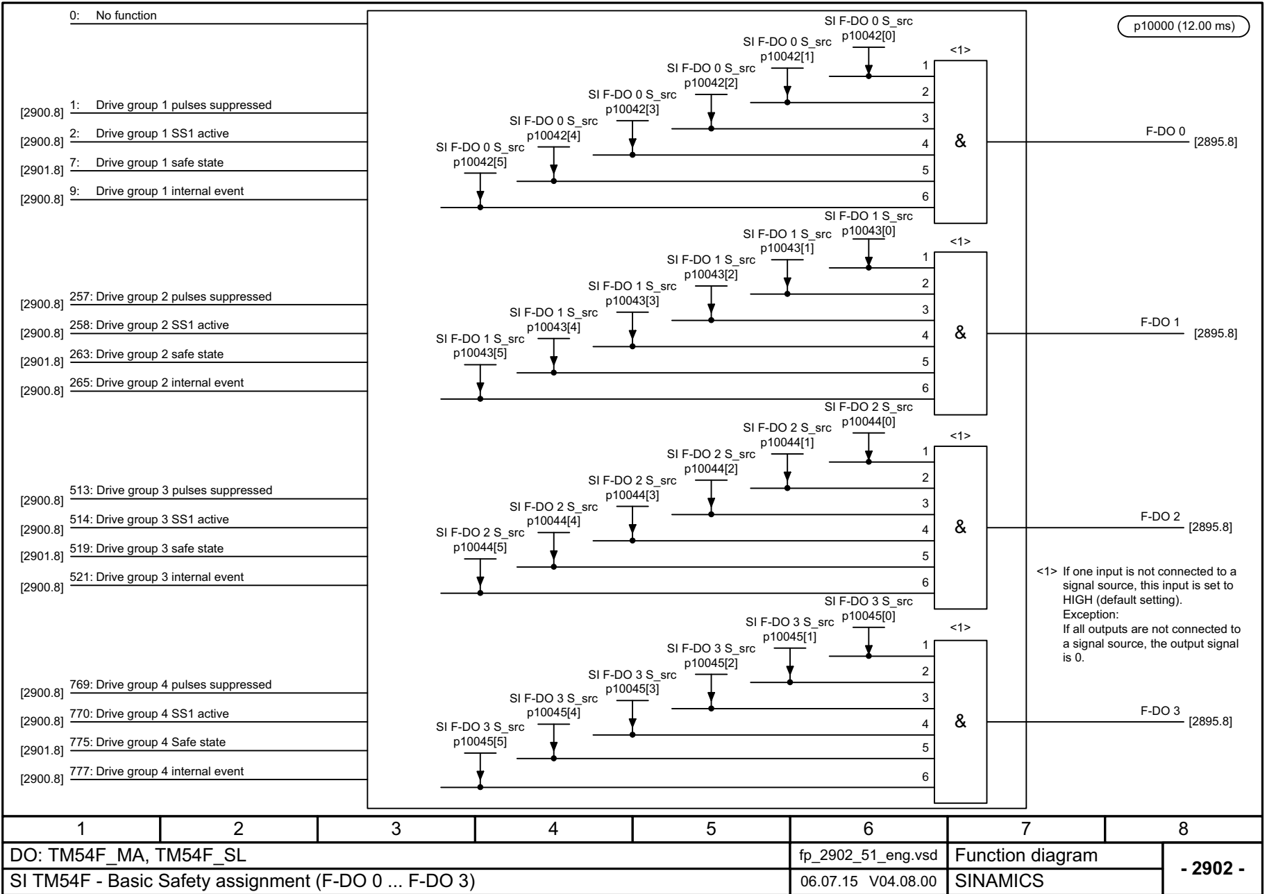
Fig. 3-145 2902 – Basic Functions assignment (F-DO 0 ... F-DO 3)
