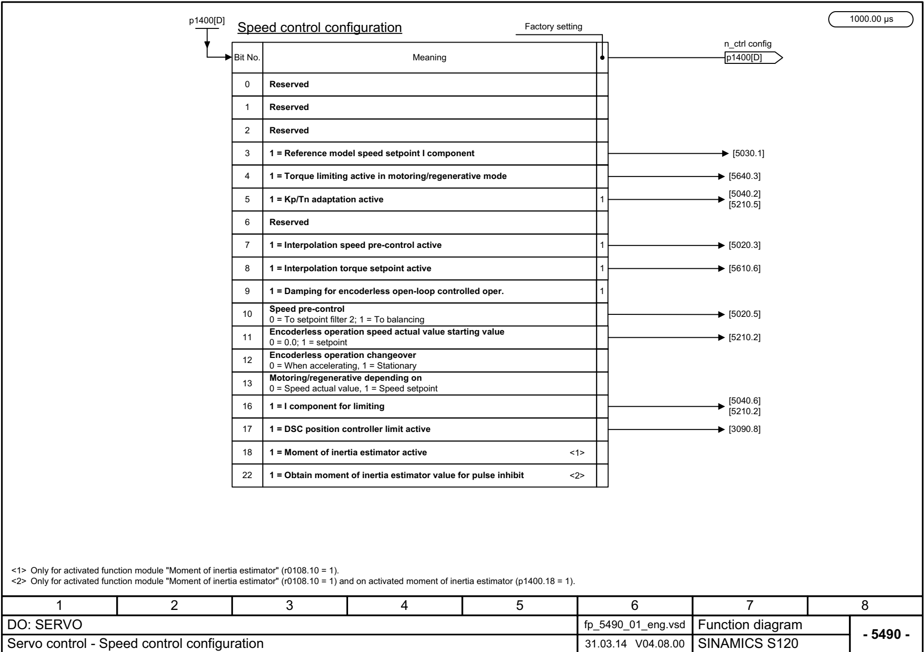
Fig. 3-214 5490 – Speed control configuration
