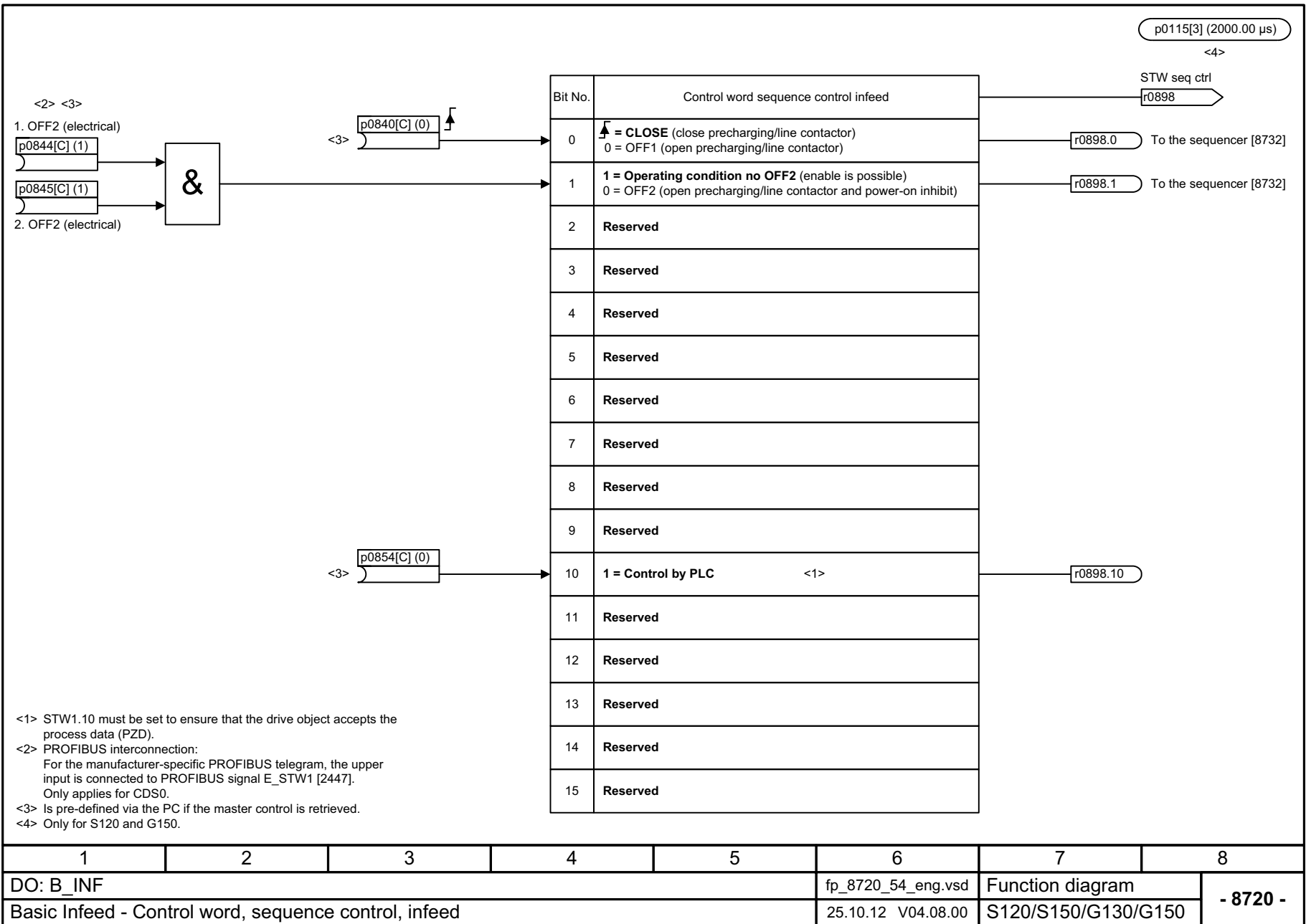
Fig. 3-318 8720 – Control word, sequence control infeed
