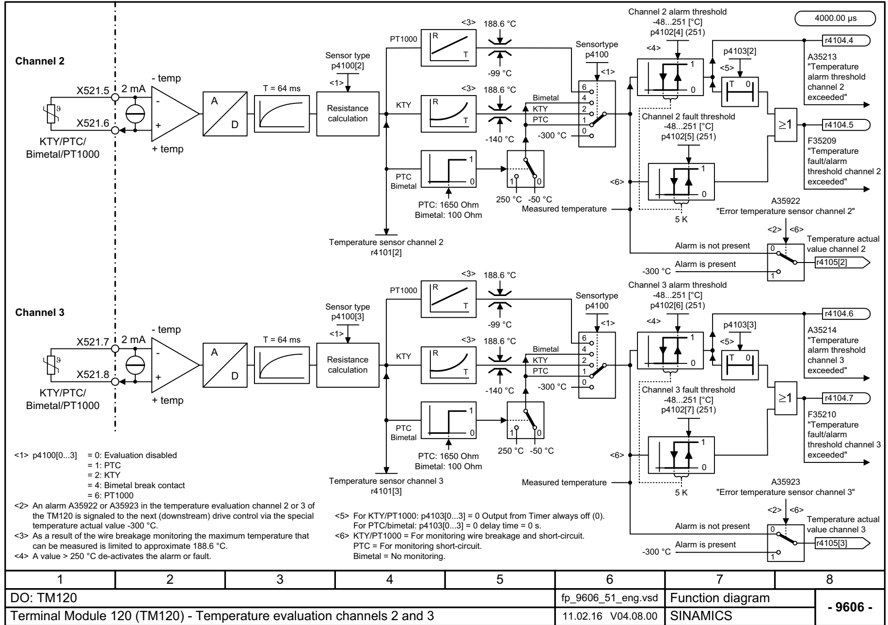
Fig. 3-375 9606 – Temperature evaluation channels 2 and 3 (KTY/PTC/bimetal)
