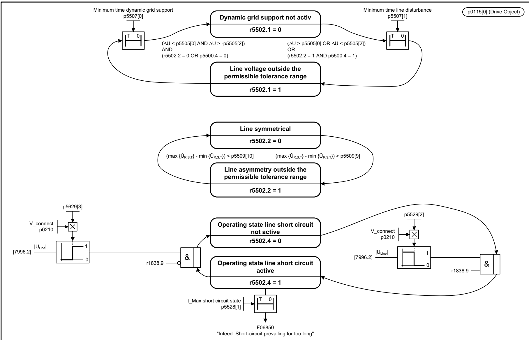
Fig. 3-290 7998 – Sequence control
