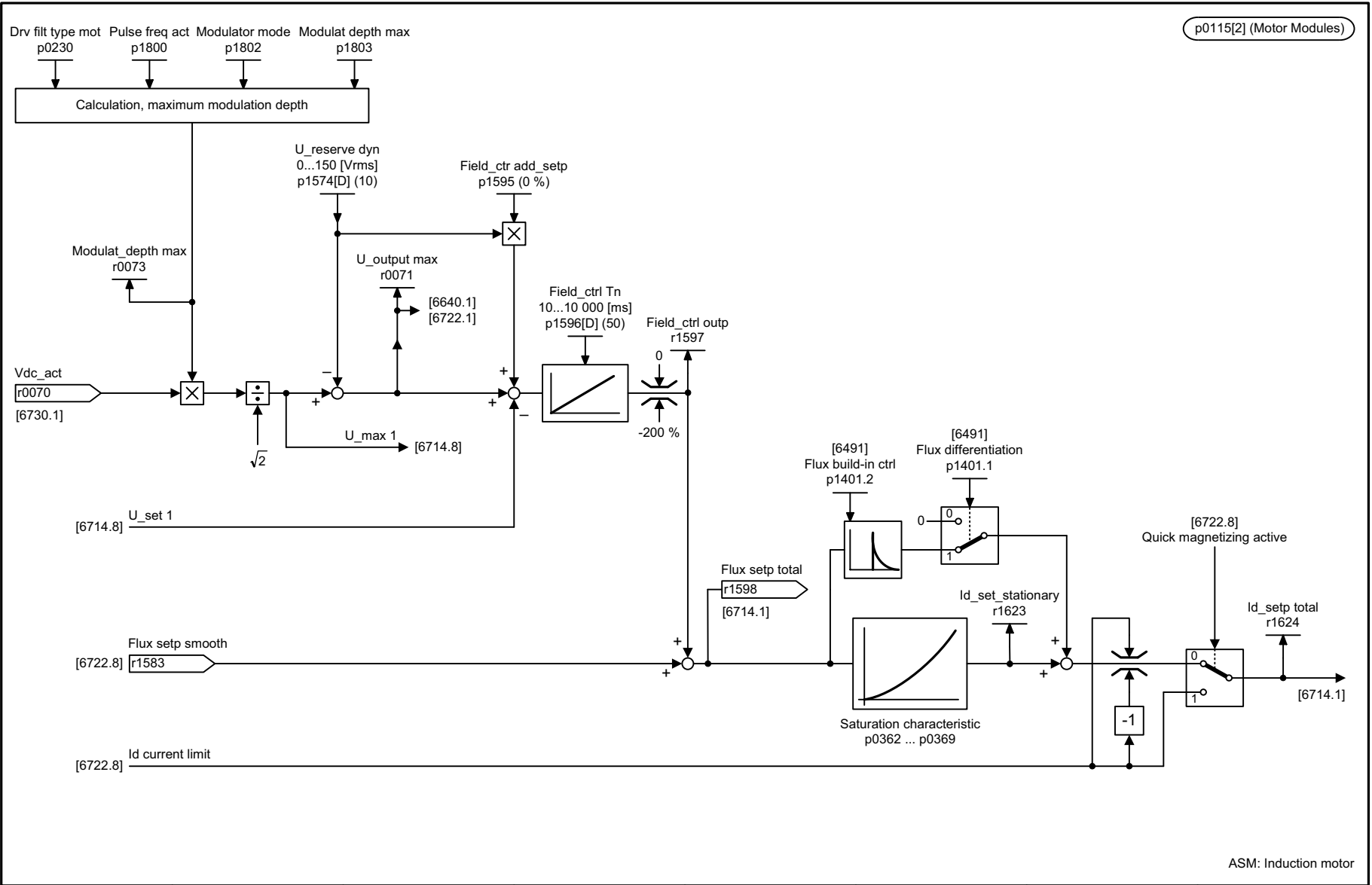
Fig. 3-249 6723 - Field weakening controller, flux controller (ASM, p0300 = 1)
