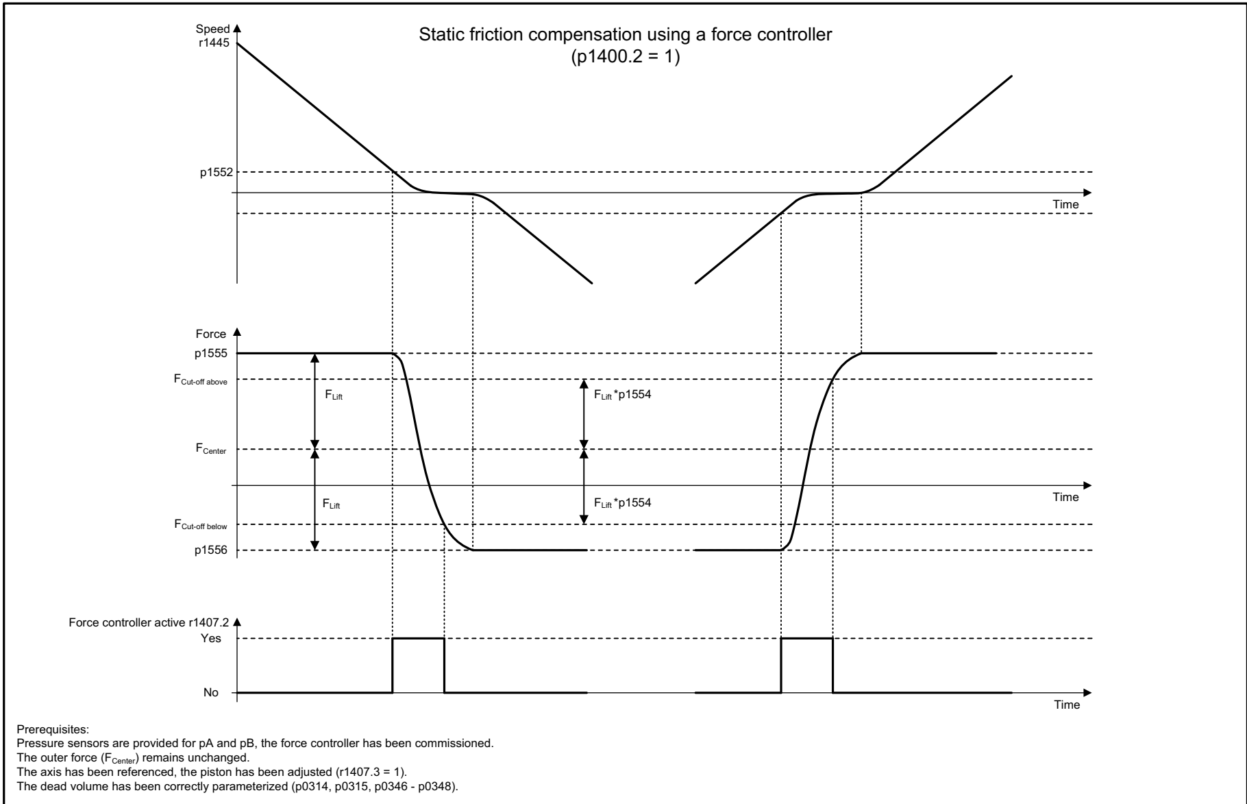
Fig. 3-197 4977 – Static friction compensation using a force controller (p1400.2 = 1)
