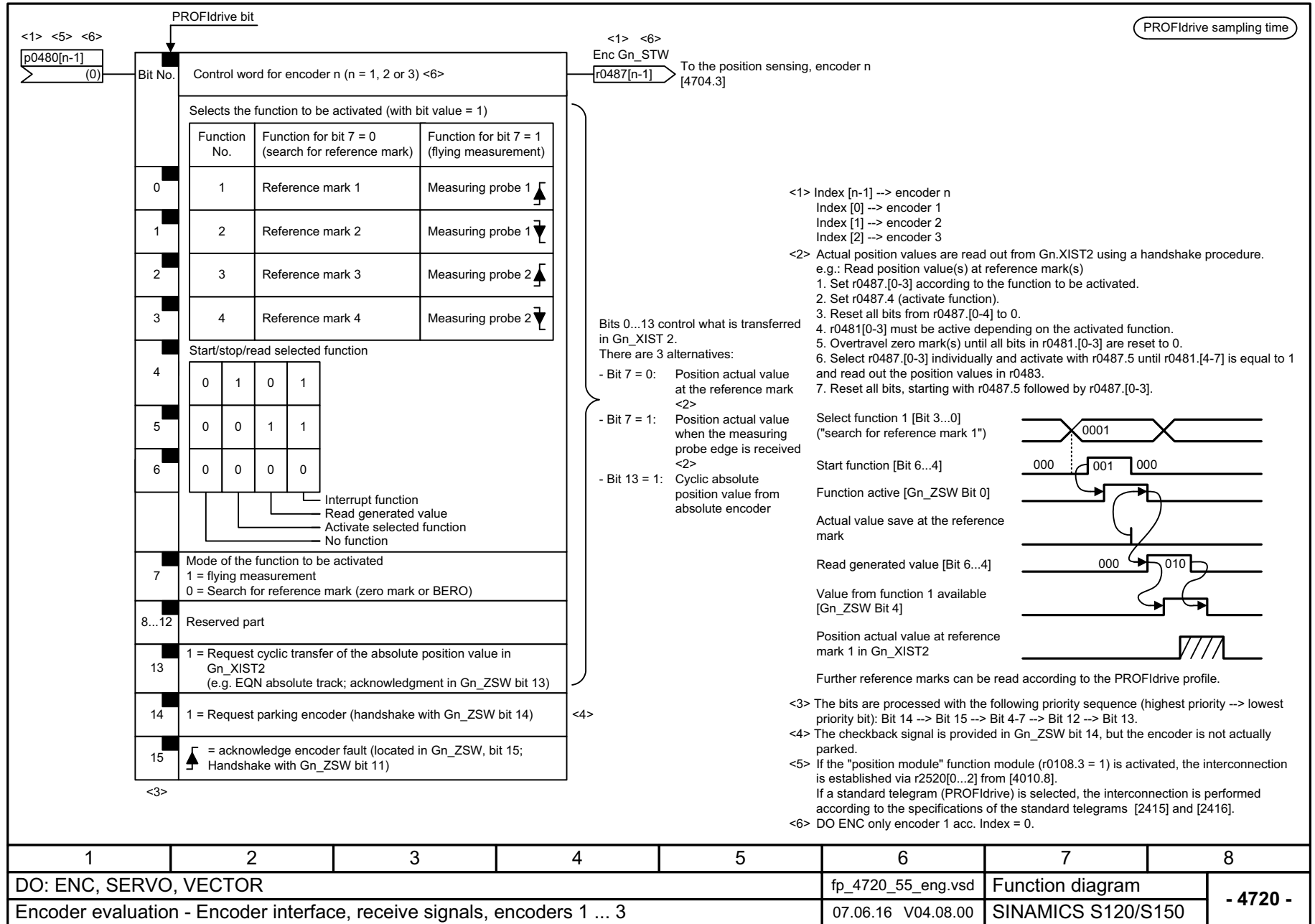
Fig. 3-188 4720 – Encoder interface, receive signals, encoders 1 ... 3
