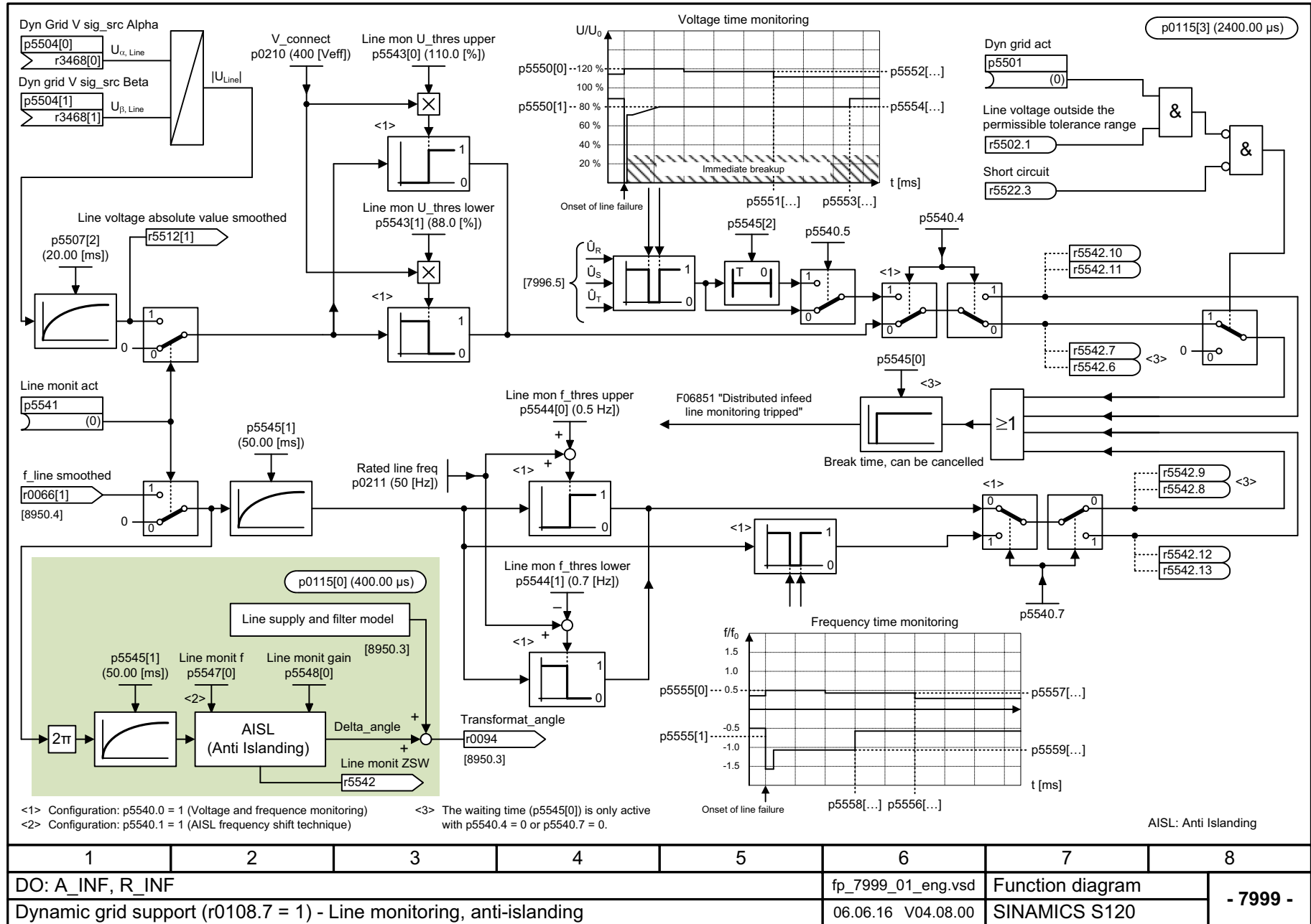
Fig. 3-291 7999 – Grid monitoring anti-islanding
