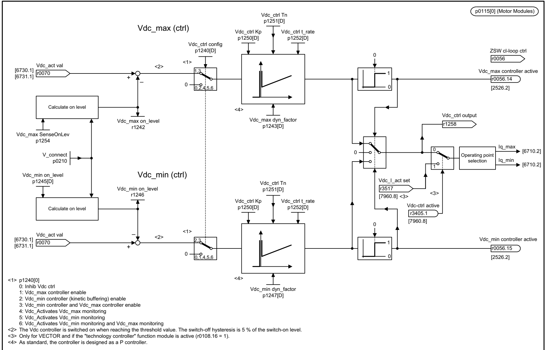
Fig. 3-234 6220 – Vdc_max controller and Vdc_min controller
