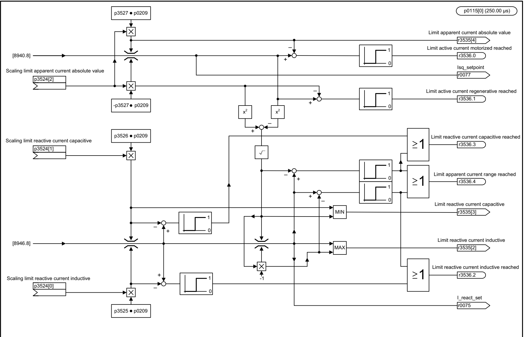
Fig. 3-340 8945 – Reactive current/apparent current limits (r0108.3 = 1)
