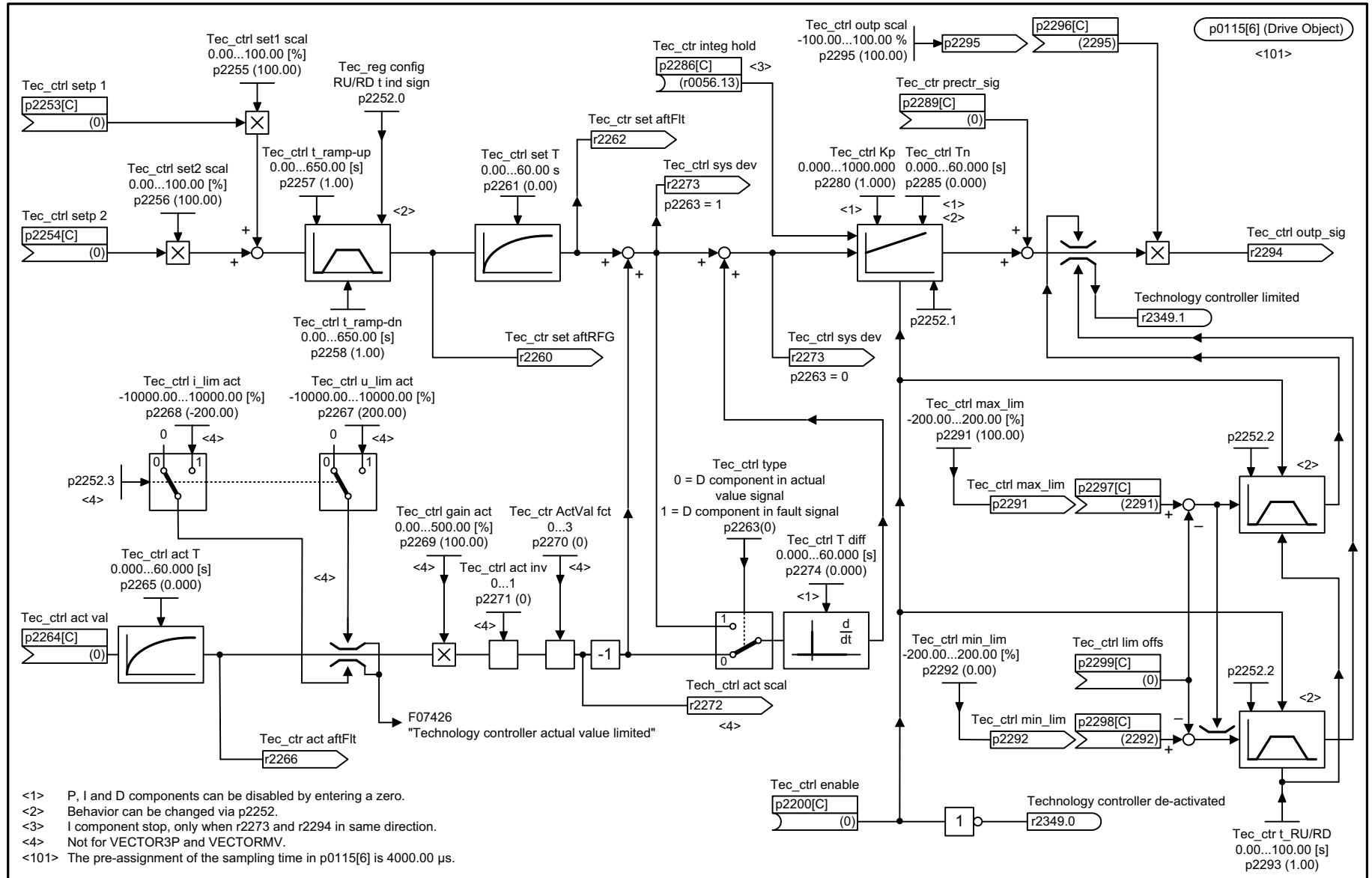
Fig. 3-274 7958 - Closed-loop control (r0108.16 = 1)
