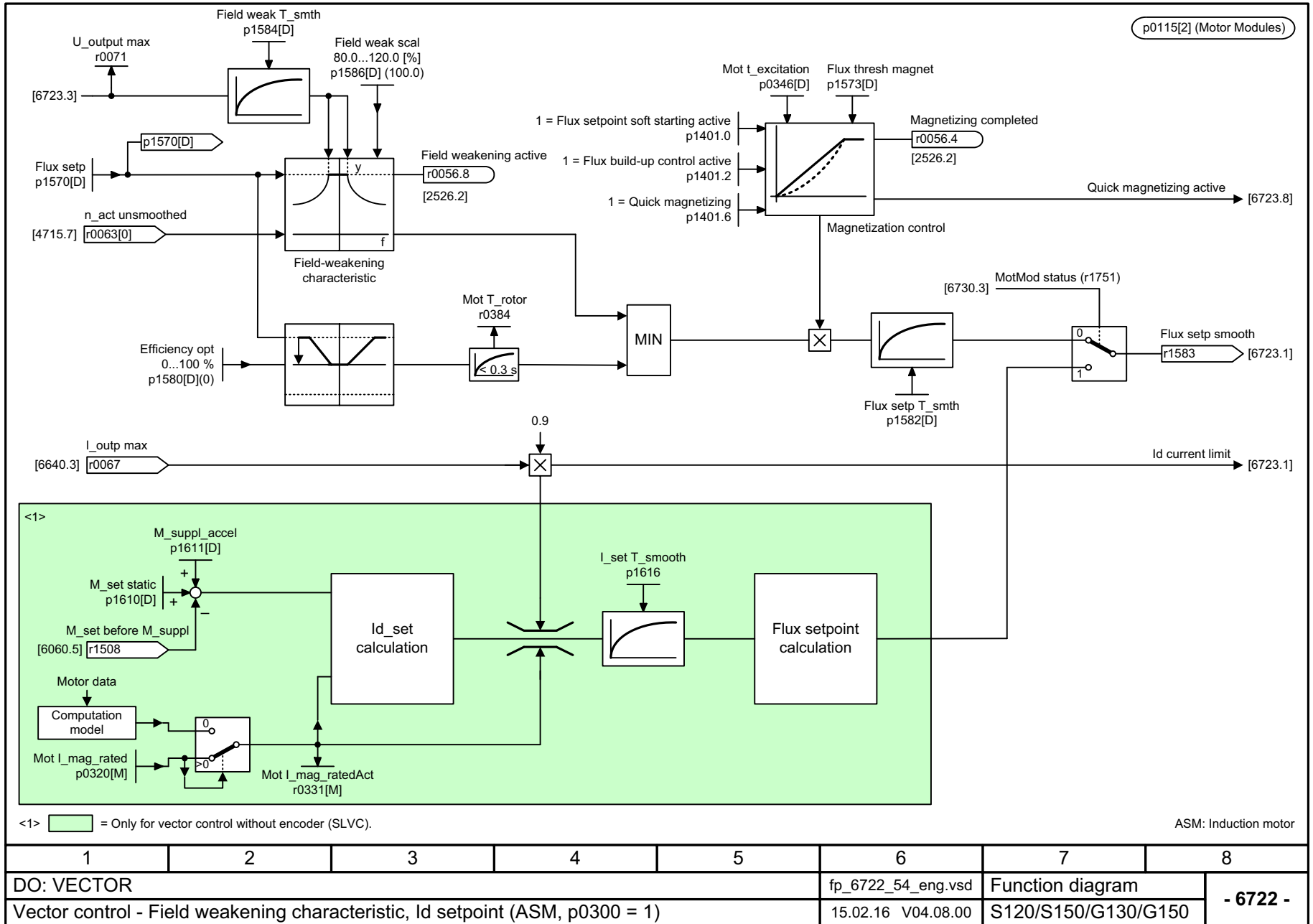
Fig. 3-248 6722 - Field weakening characteristic, Id setpoint (ASM, p0300 = 1)
