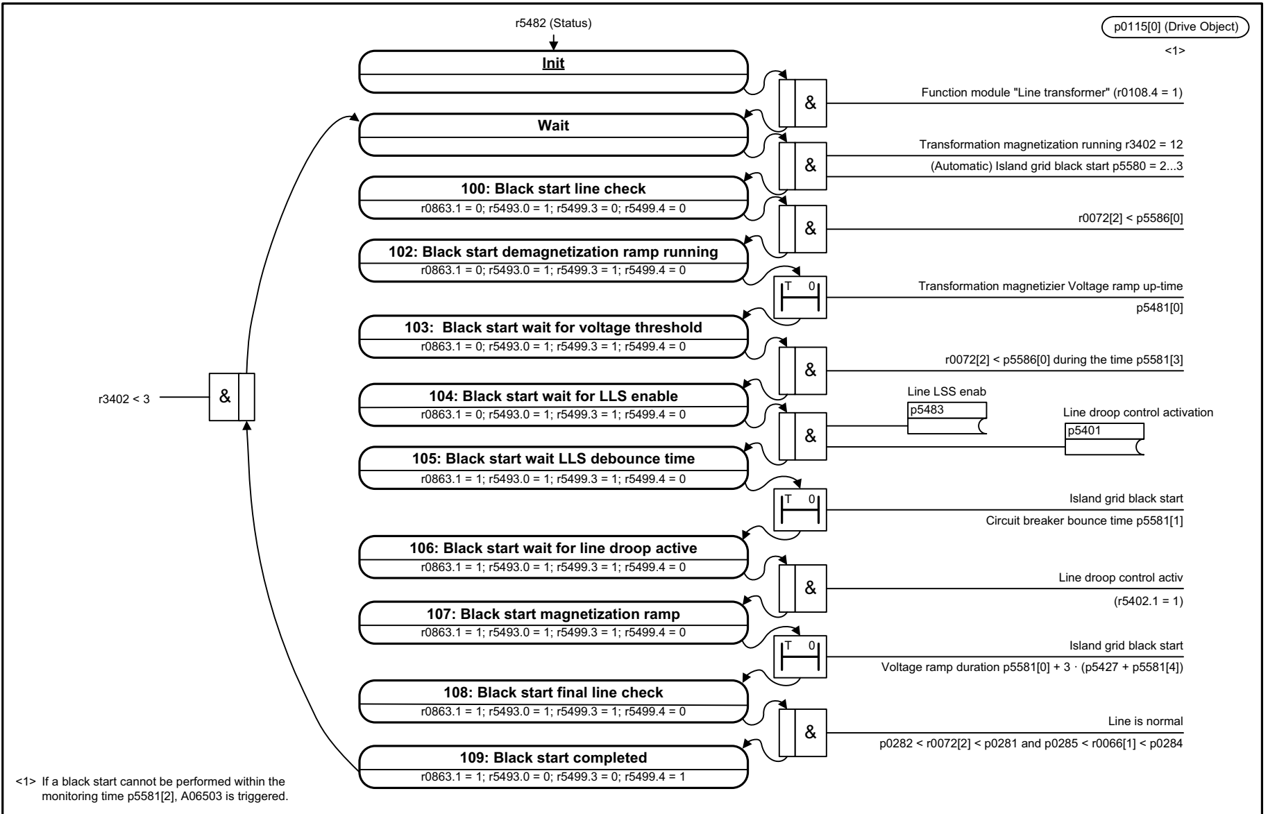
Fig. 3-281 7988 – Island grid black start sequence control
