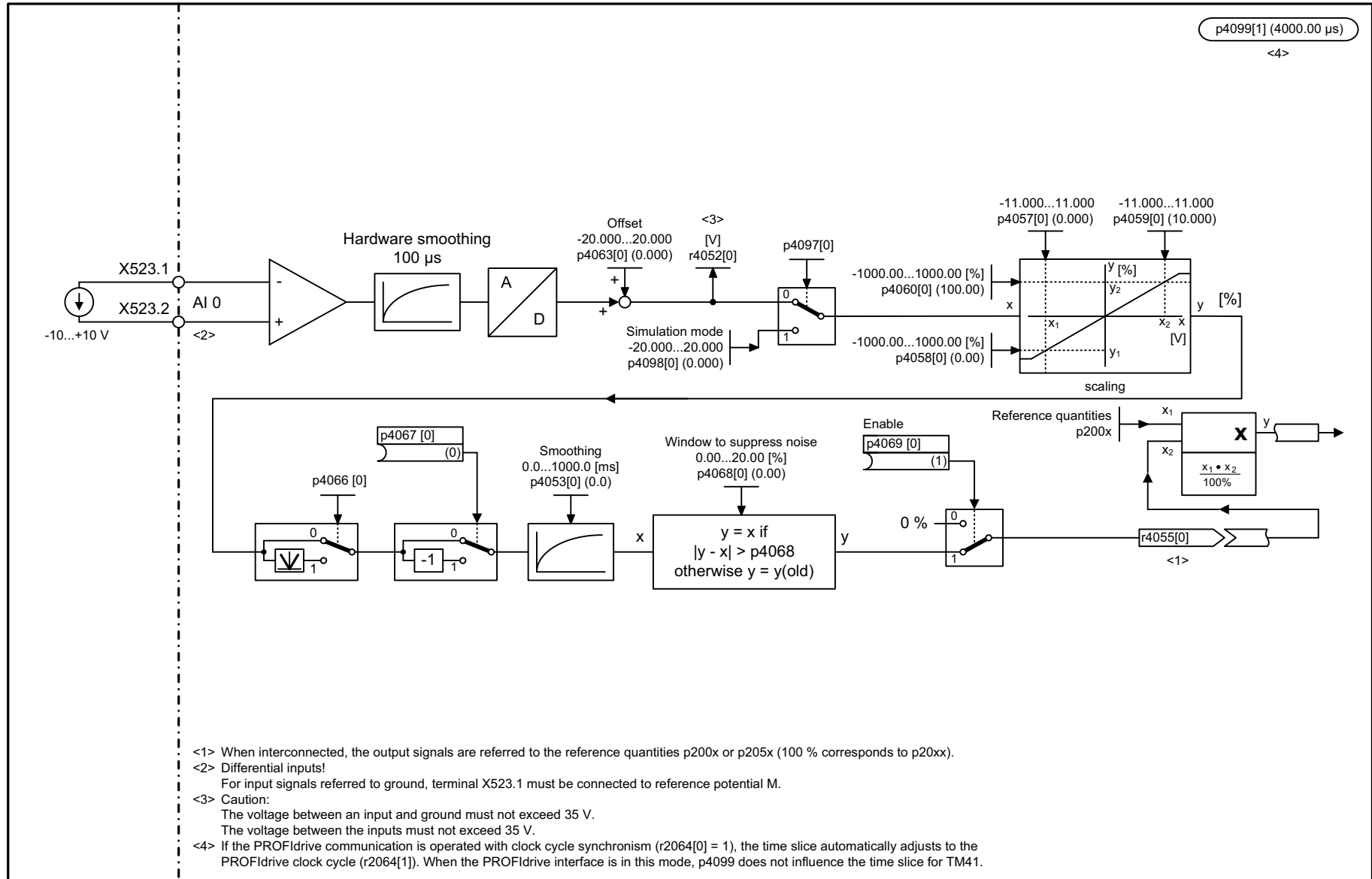
Fig. 3-383 9663 – Analog input 0 (AI 0)
