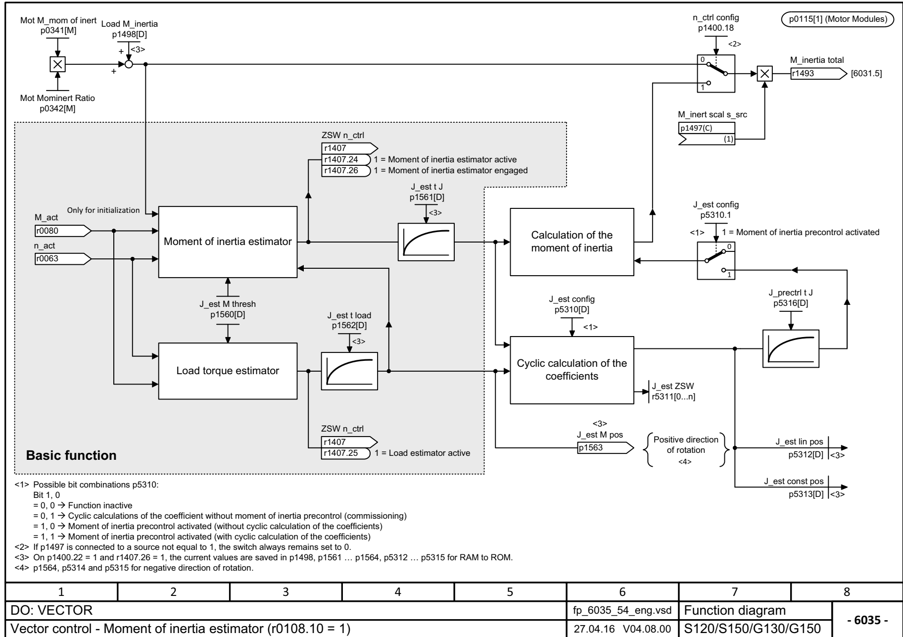
Fig. 3-230 6035 – Moment of inertia estimator (r0108.10 = 1)
