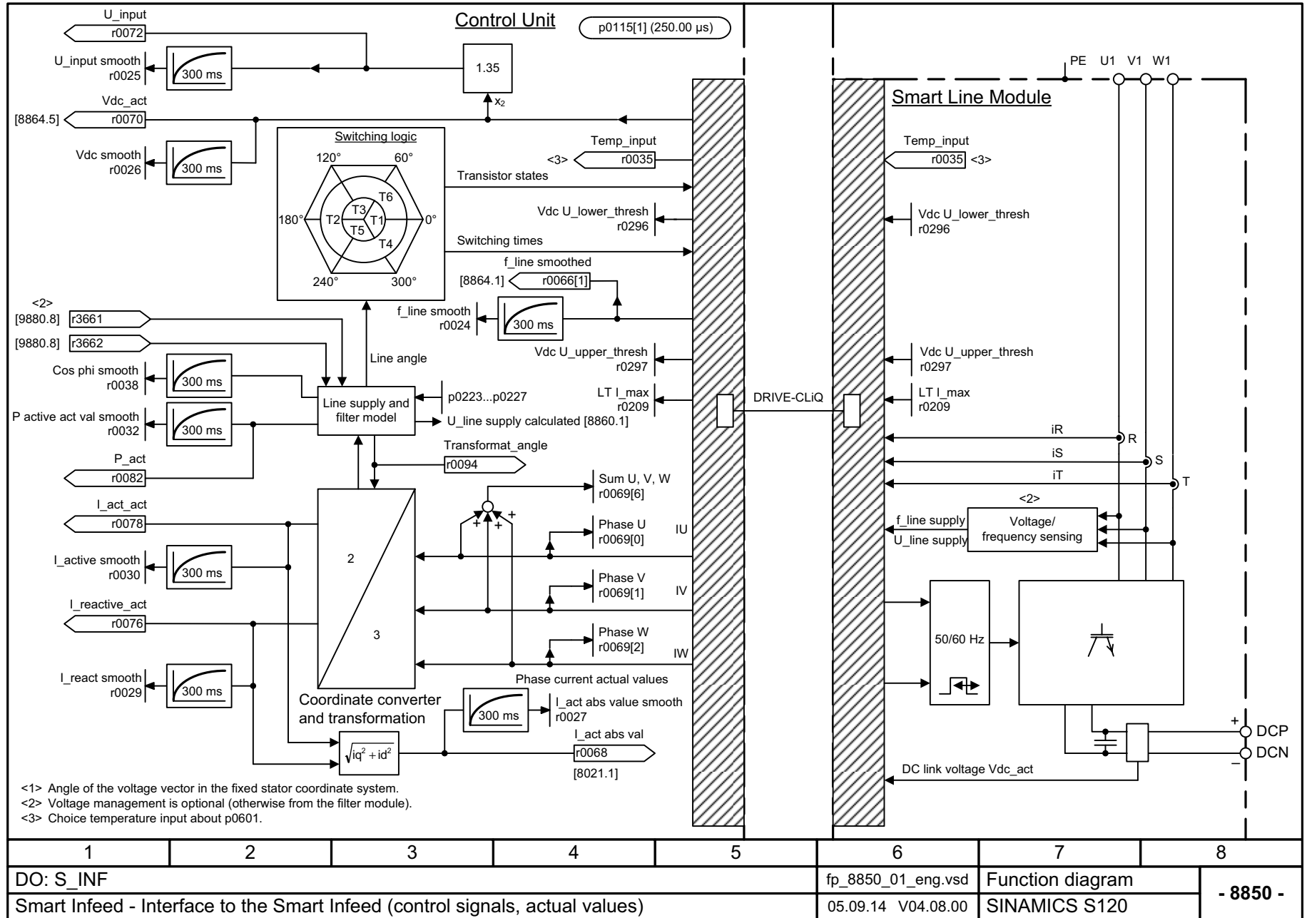
Fig. 3-330 8850 – Interface to the Smart Infeed (control signals, actual values)
