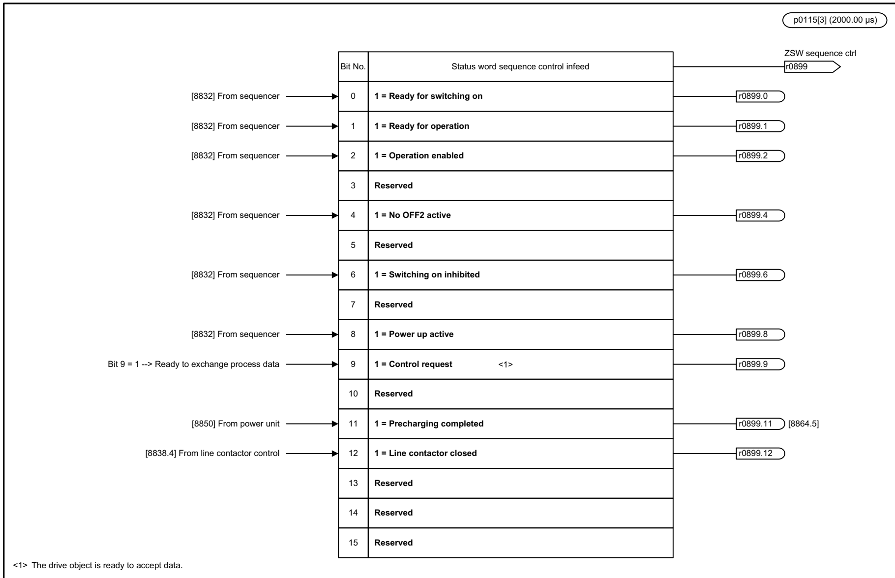
Fig. 3-326 8826 – Status word, sequence control infeed
