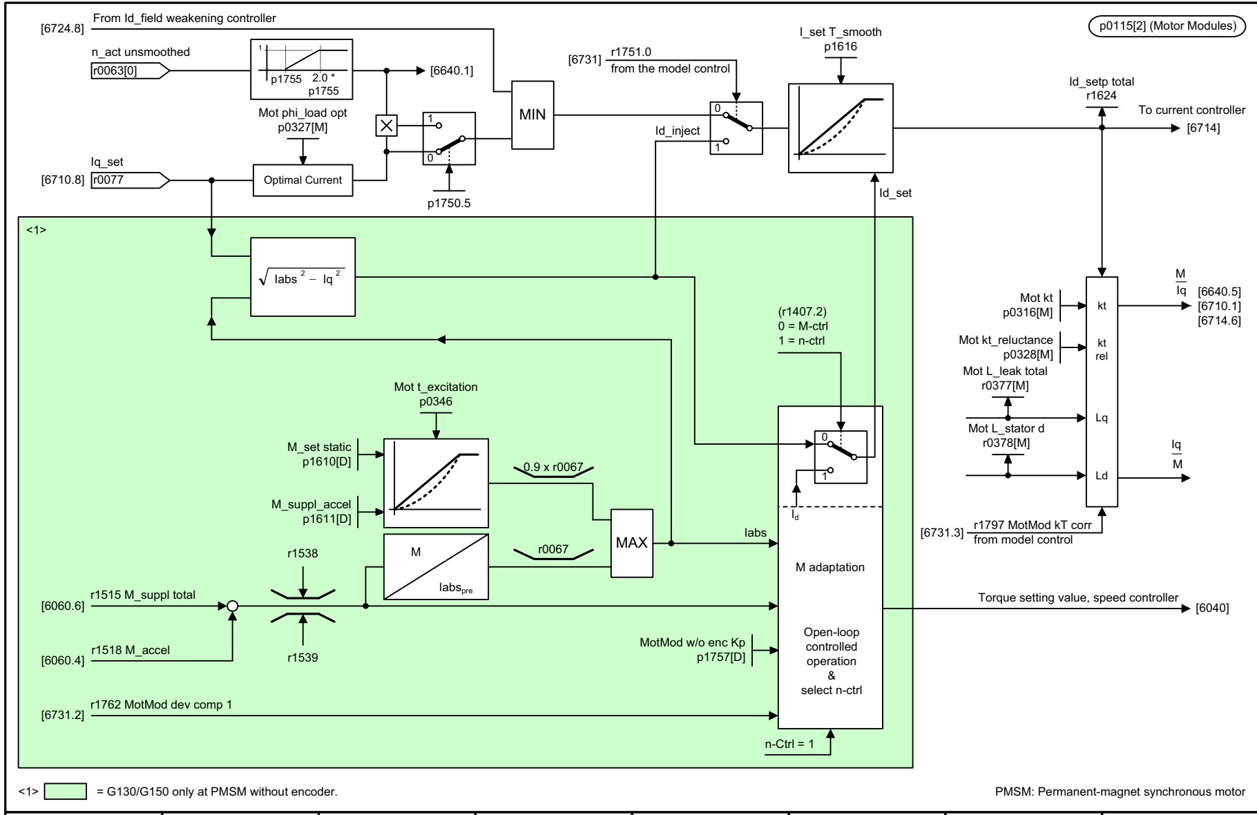
Fig. 3-247 6721 - Id setpoint (PEM, p0300 = 2)
