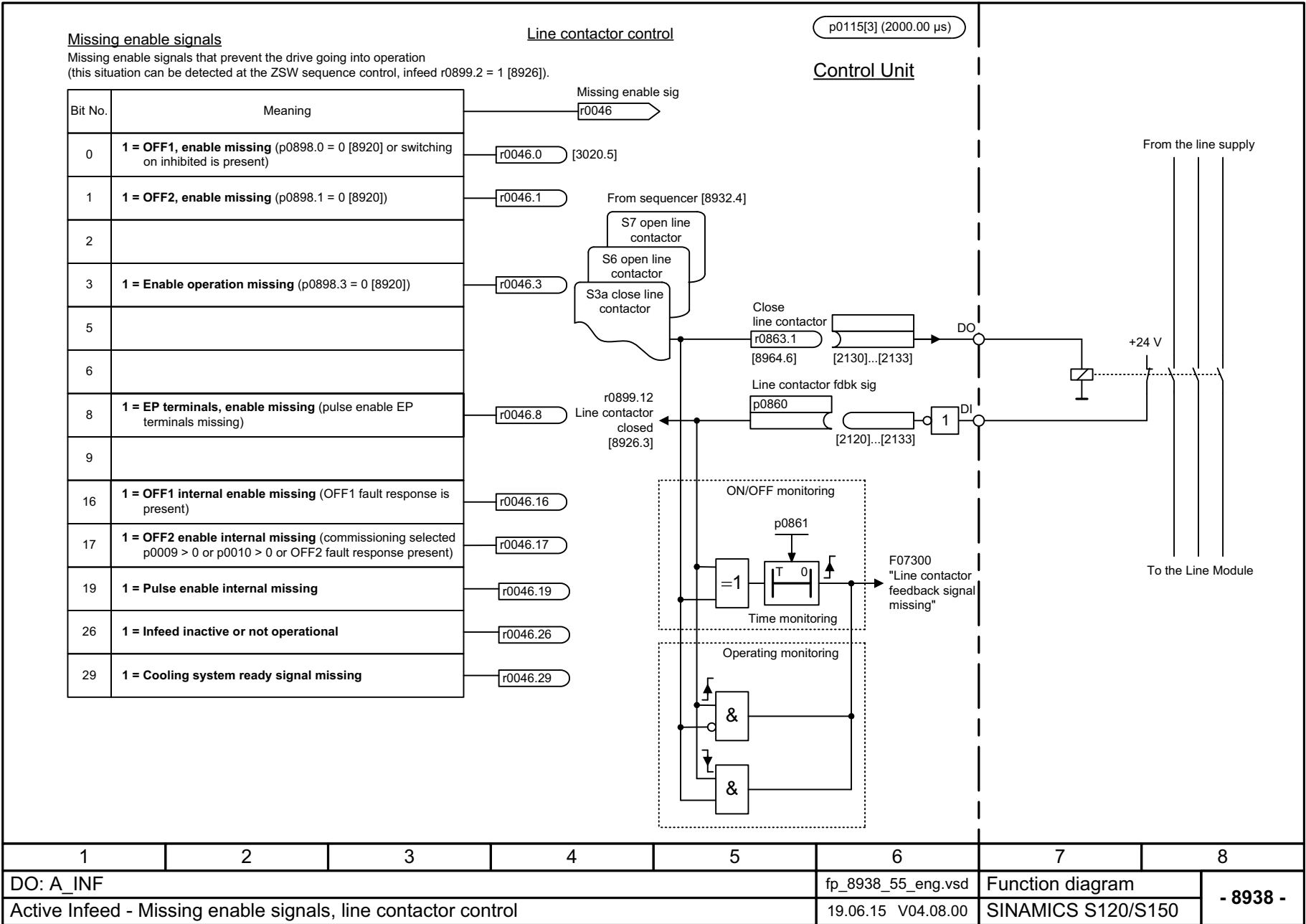
Fig. 3-338 8938 – Missing enable signals, line contactor control
