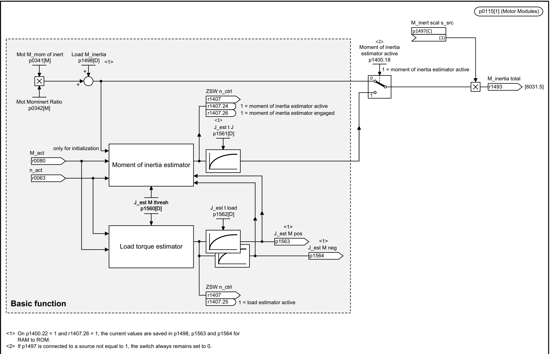
Fig. 3-205 5035 – Moment of inertia estimator (r0108.10 = 1)
