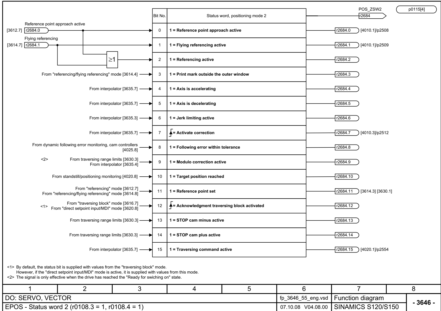
Fig. 3-176 3646 – Status word 2 (r0108.3 = 1, r0108.4 = 1)
