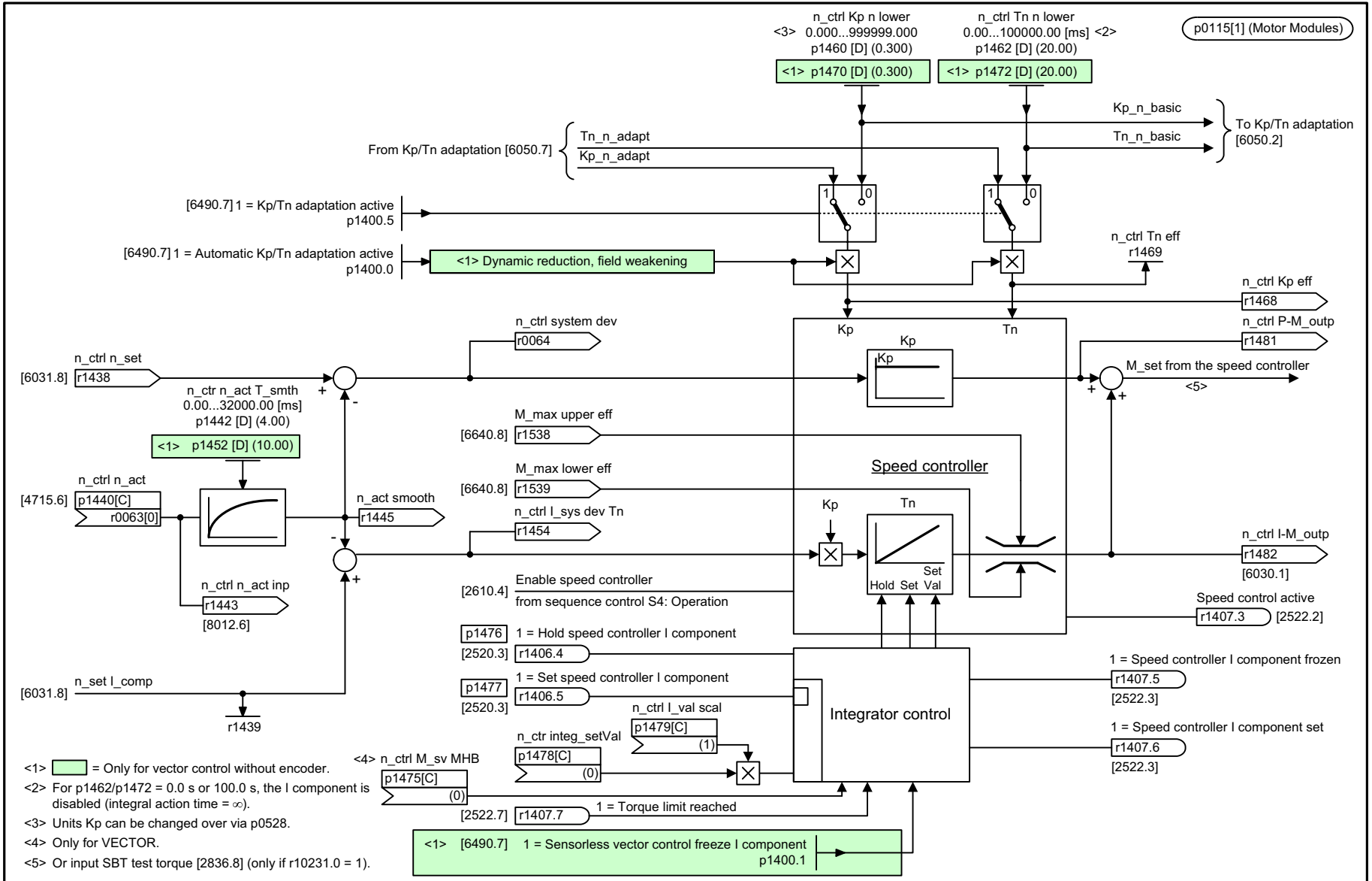
Fig. 3-231 6040 – Speed controller with/without encoder
