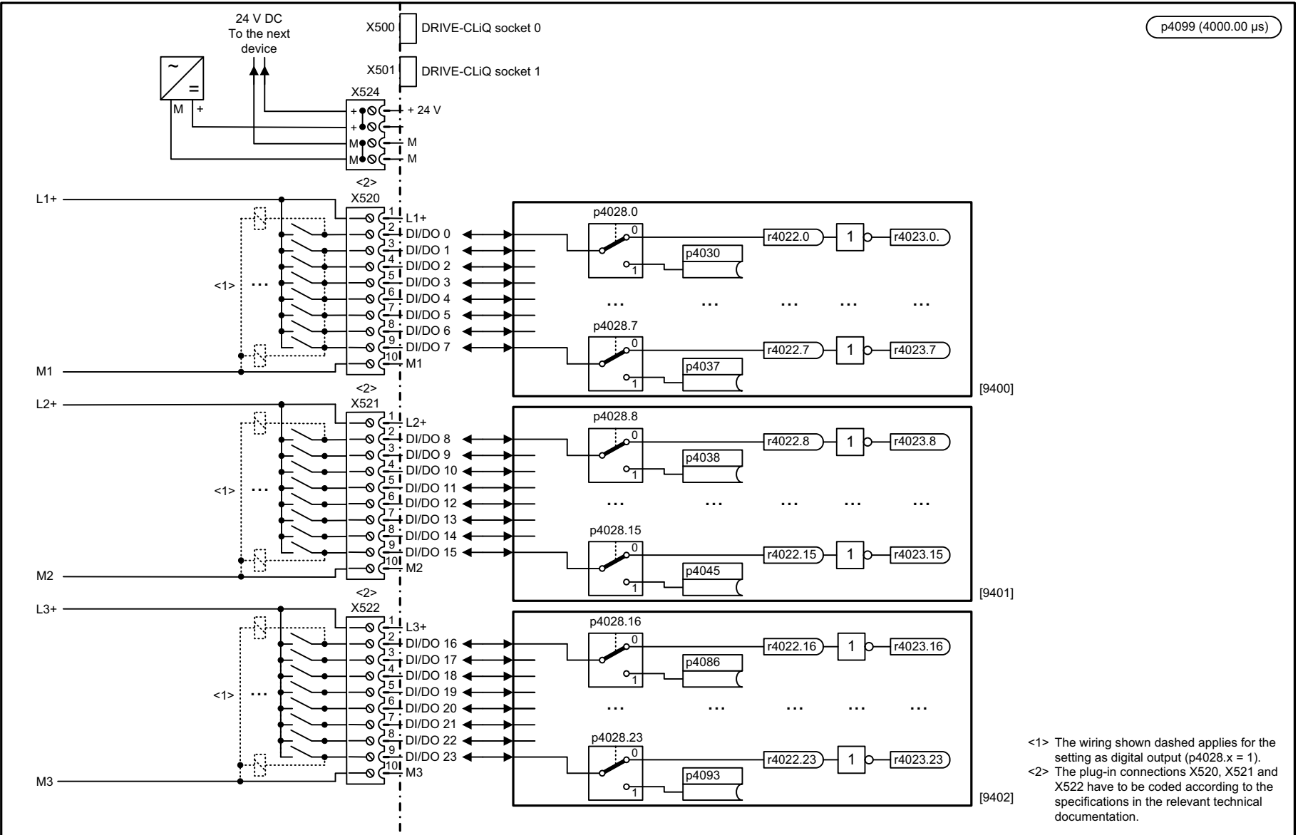
Fig. 3-359 9399 – Overview TM15DI_DO (SINAMICS)
