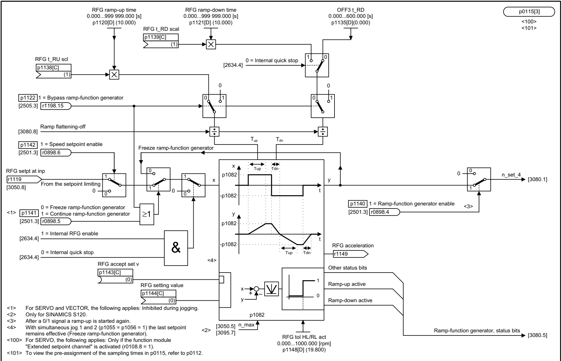
Fig. 3-157 3060 – Basic ramp-function generator
