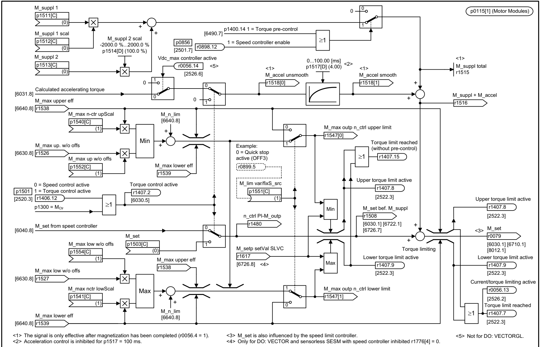
Fig. 3-233 6060 – Torque setpoint
