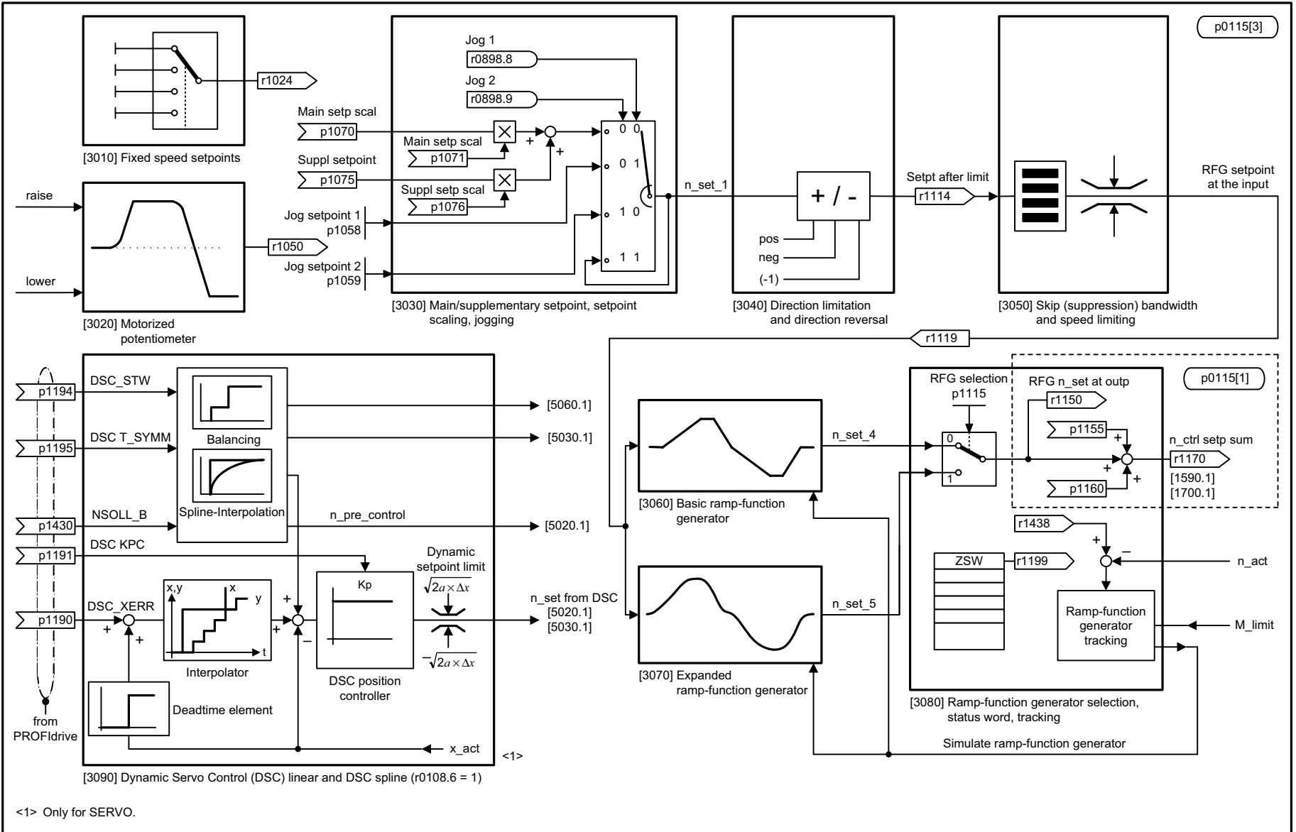
Fig. 3-151 3001 – Overview
