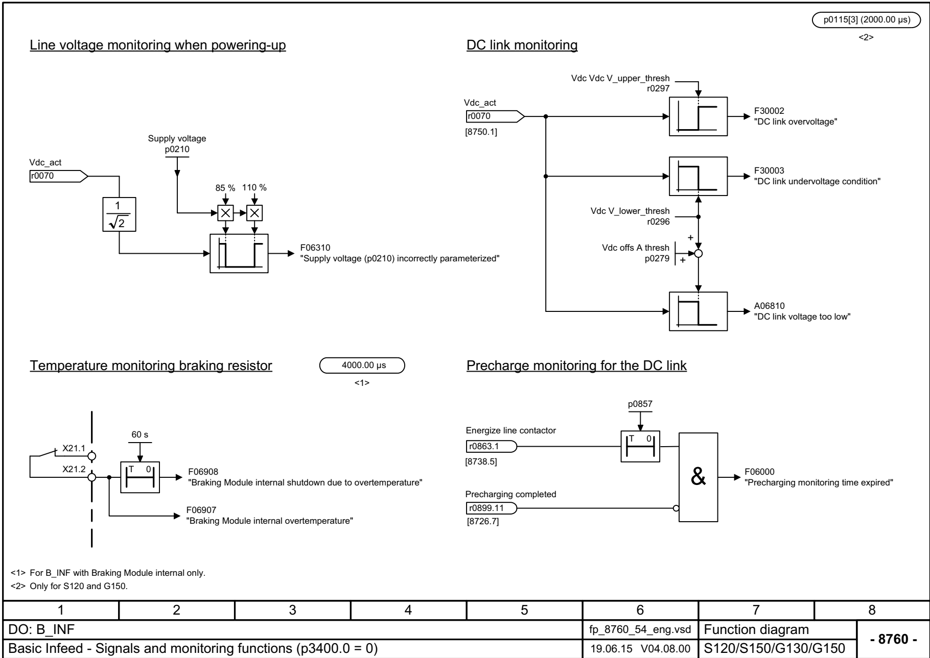
Fig. 3-323 8760 – Signals and monitoring functions (p3400.0 = 0)
