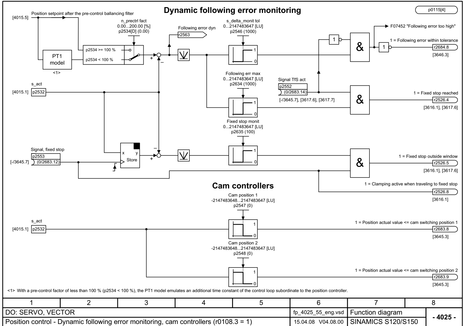
Fig. 3-181 4025 – Dynamic following error monitoring, cam controllers (r0108.3 = 1)
