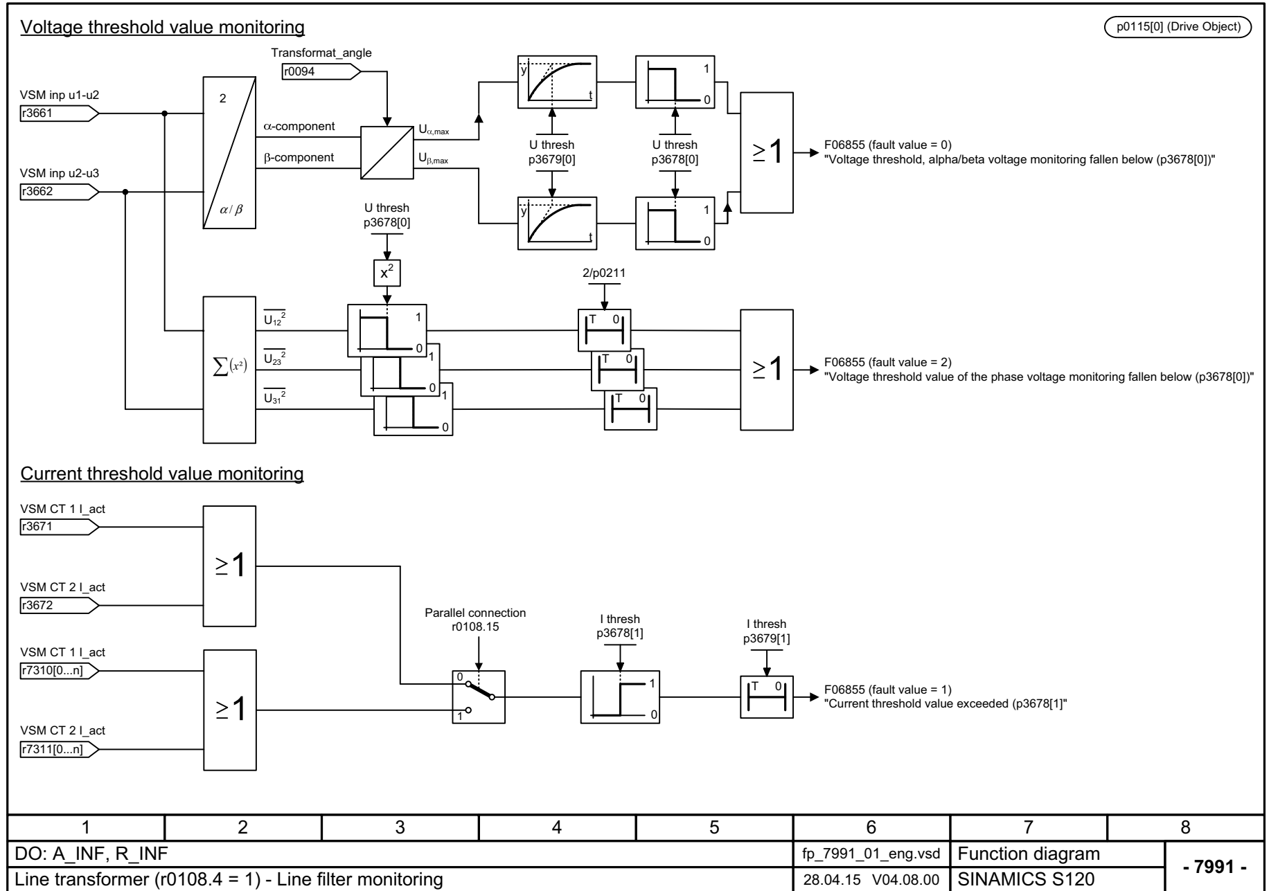
Fig. 3-284 7991 – Line filter monitoring
