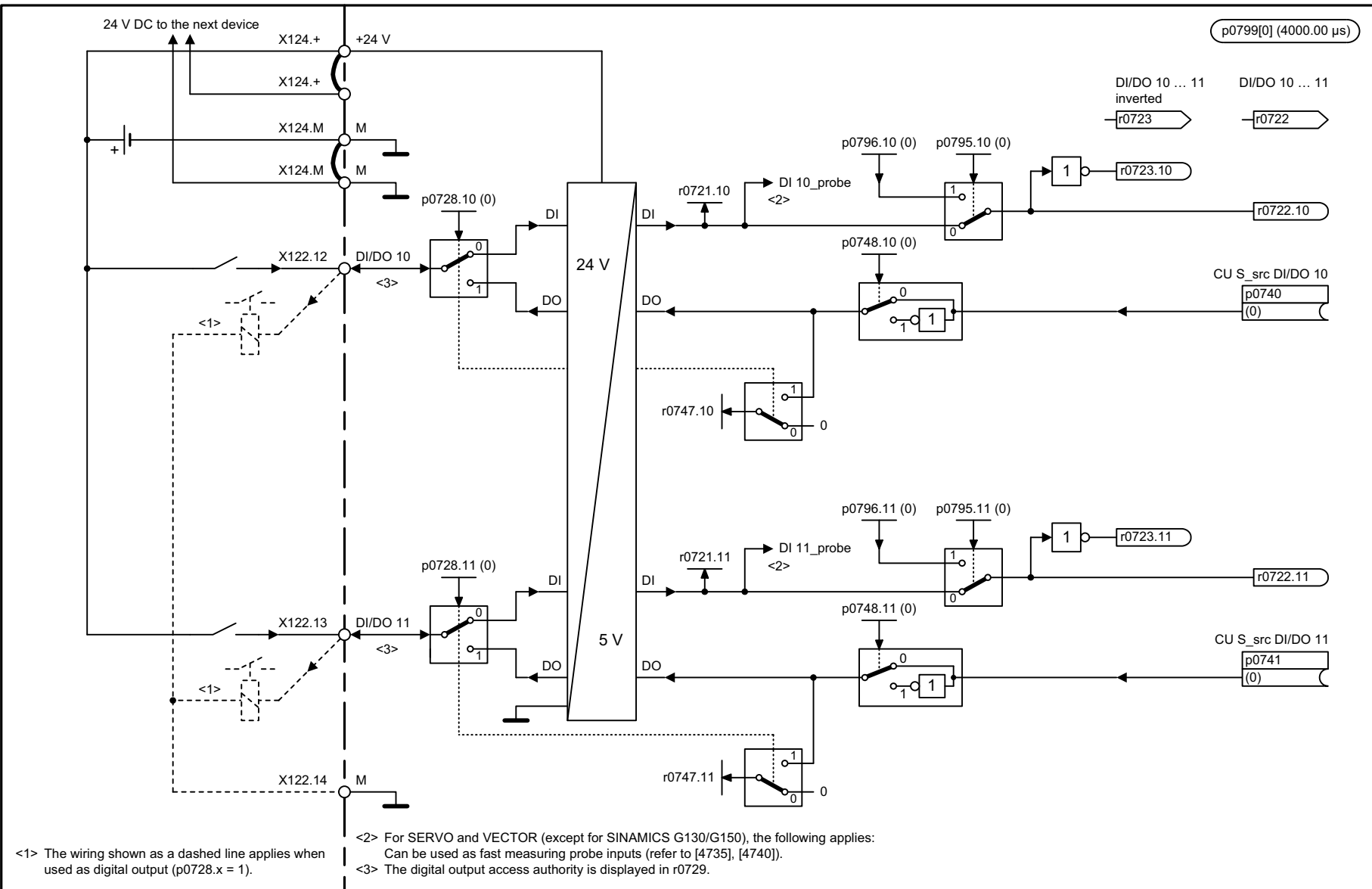
Fig. 3-18 2131 – Digital inputs/outputs, bidirectional (DI/DO 10 ... DI/DO 11)
