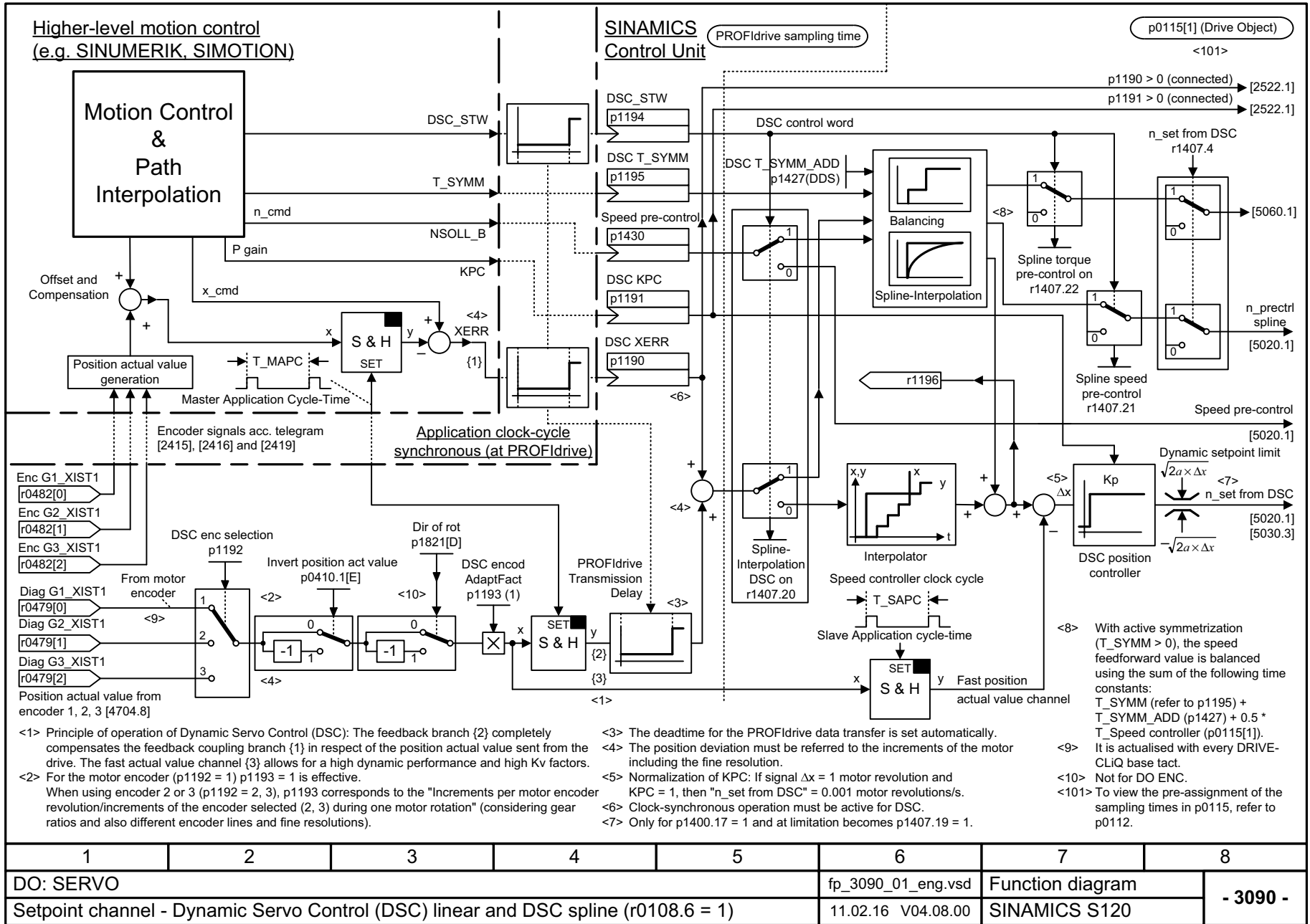
Fig. 3-161 3090 – Dynamic Servo Control (DSC) linear and DSC spline (r0108.6 = 1)
