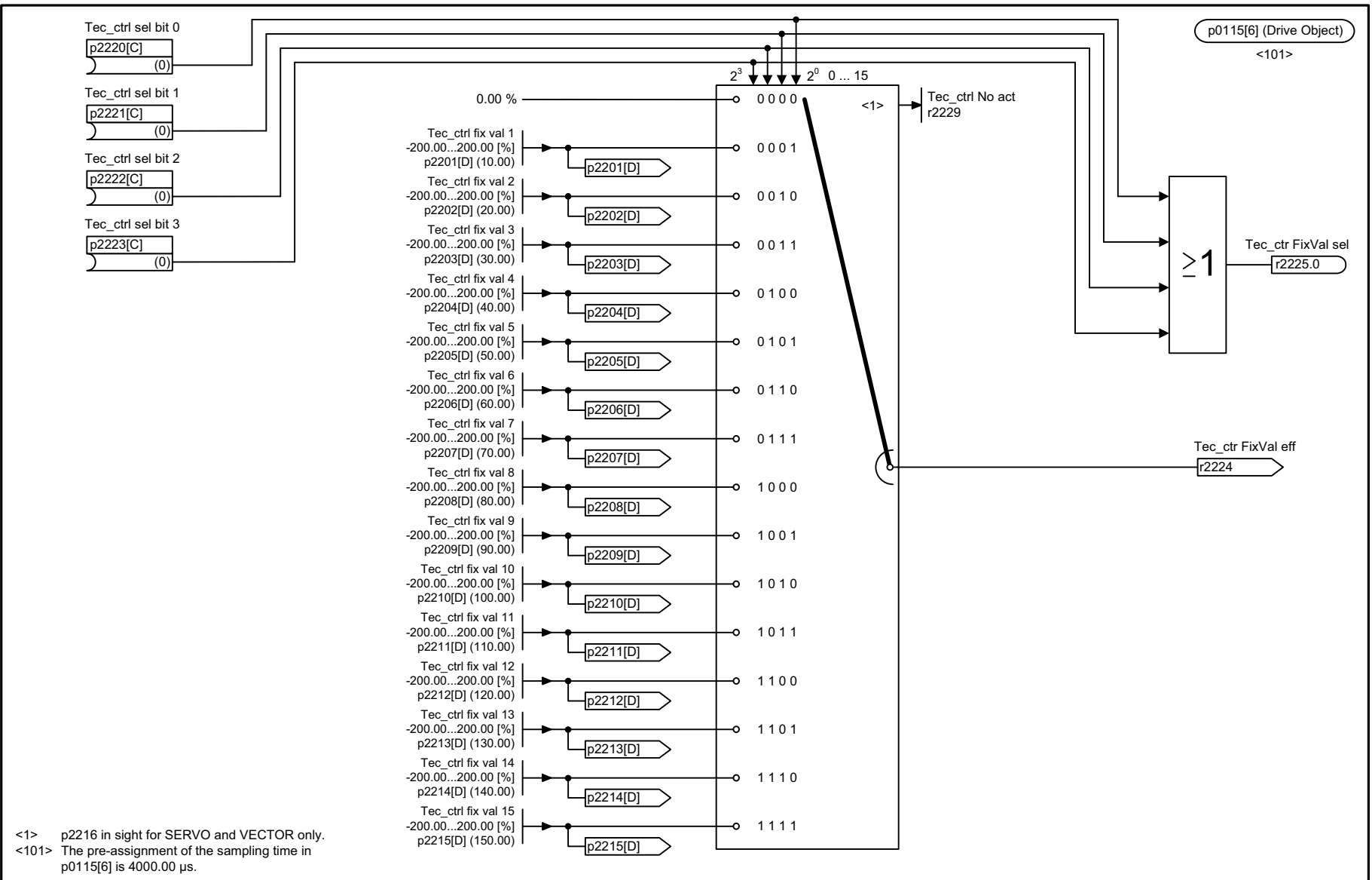
Fig. 3-271 7950 – Fixed value selection binary (r0108.16 = 1 and p2216 = 2)
