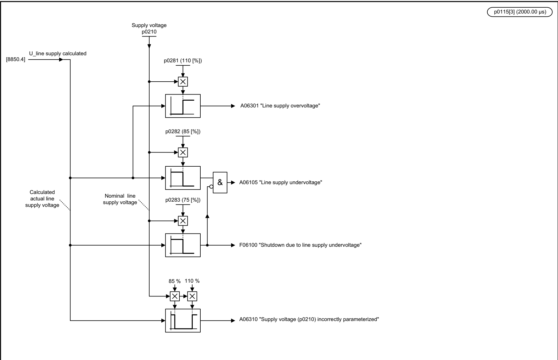
Fig. 3-331 8860 – Signals and monitoring functions, line supply voltage monitoring
