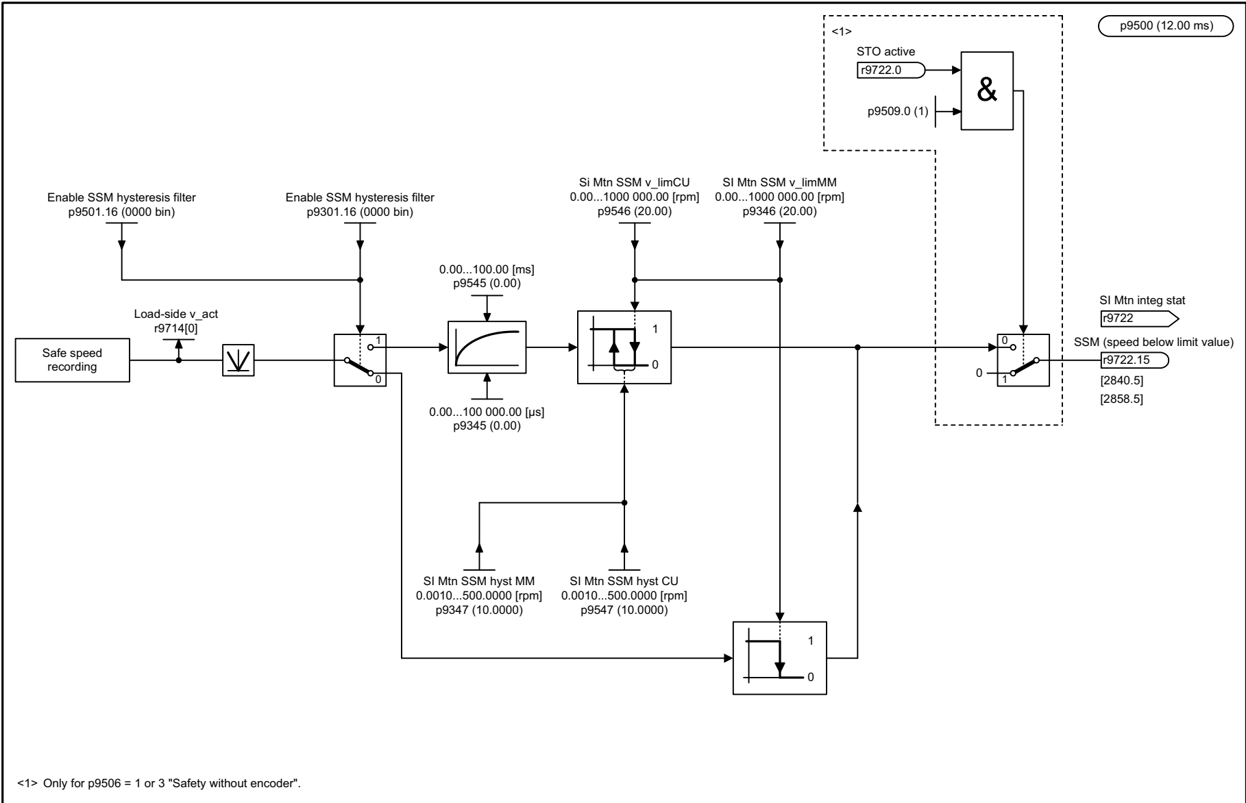
Fig. 3-123 2823 – SSM (Safe Speed Monitor)
