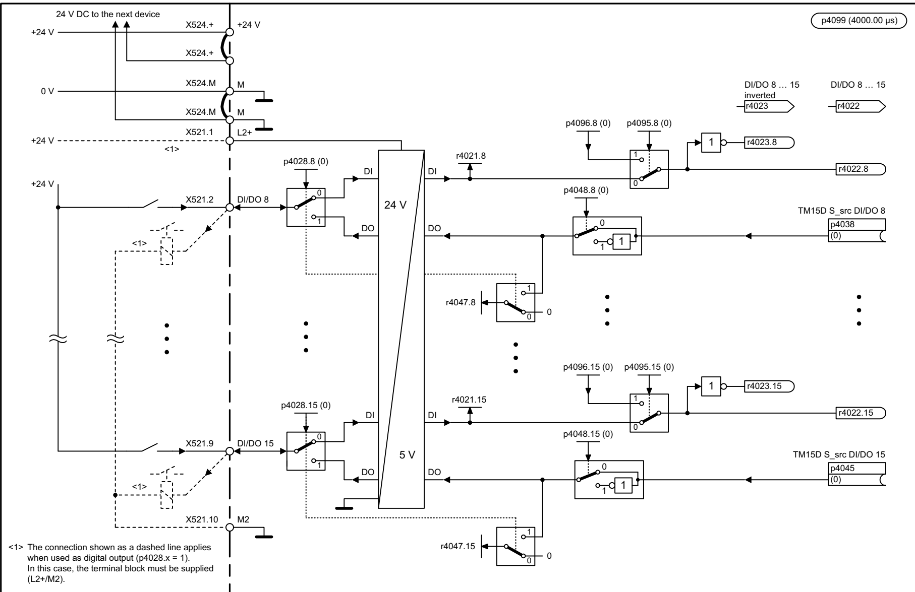
Fig. 3-361 9401 – Digital inputs/outputs, bidirectional (DI/DO 8 ... DI/DO 15)
