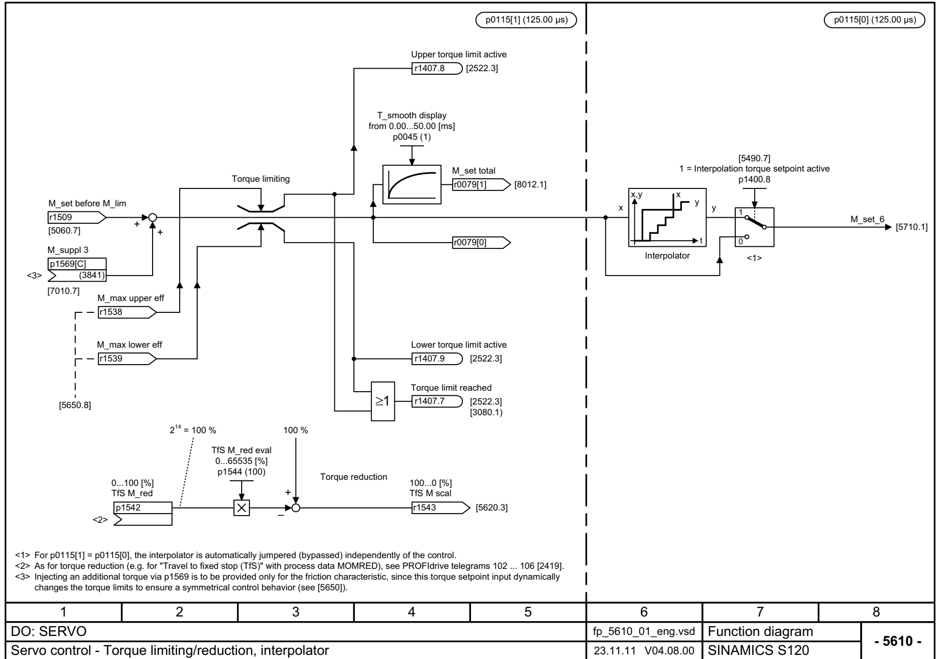
Fig. 3-216 5610 – Torque limiting/reduction, interpolator
