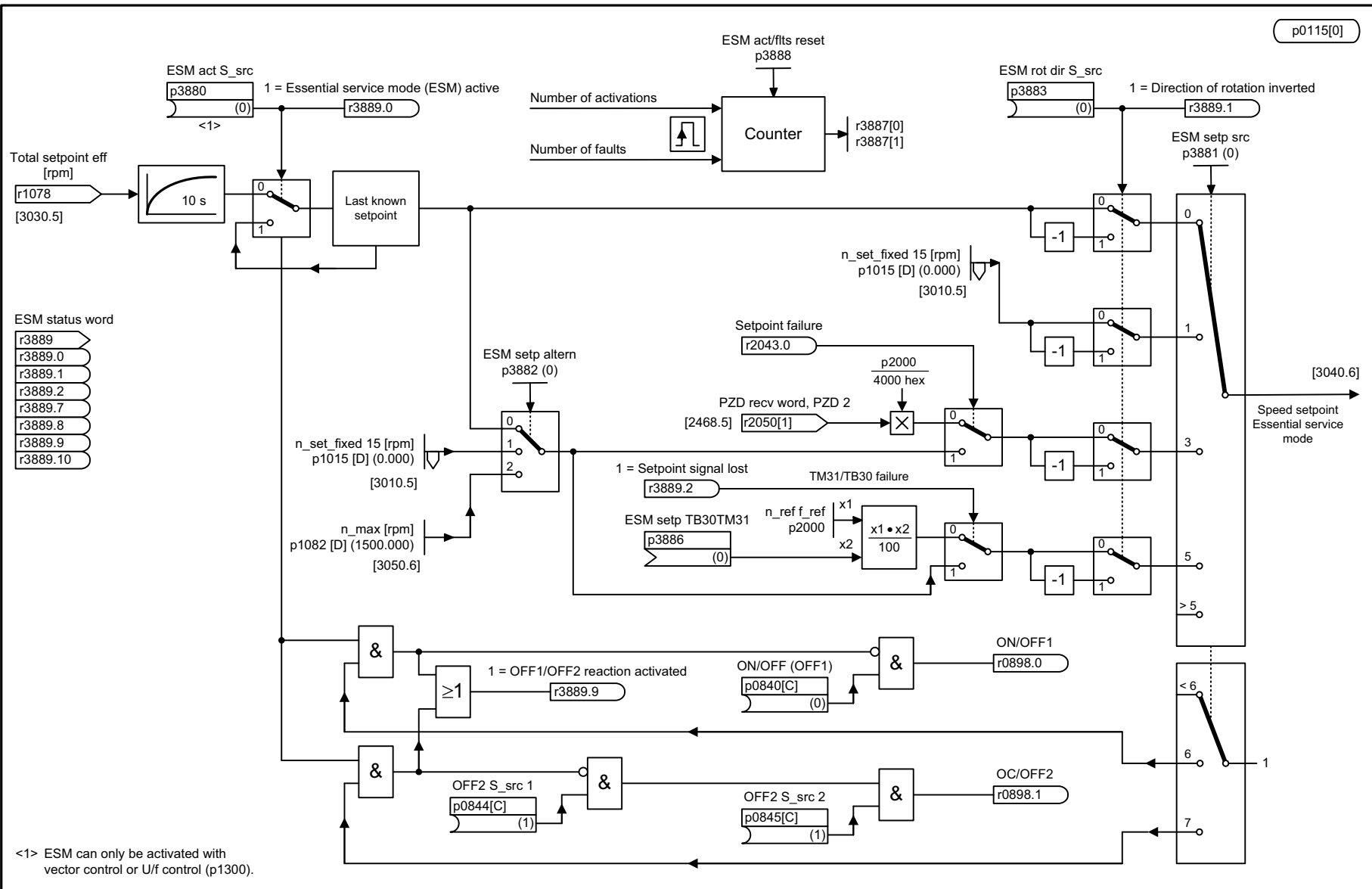
Fig. 3-270 7033 – Essential service mode (ESM)
