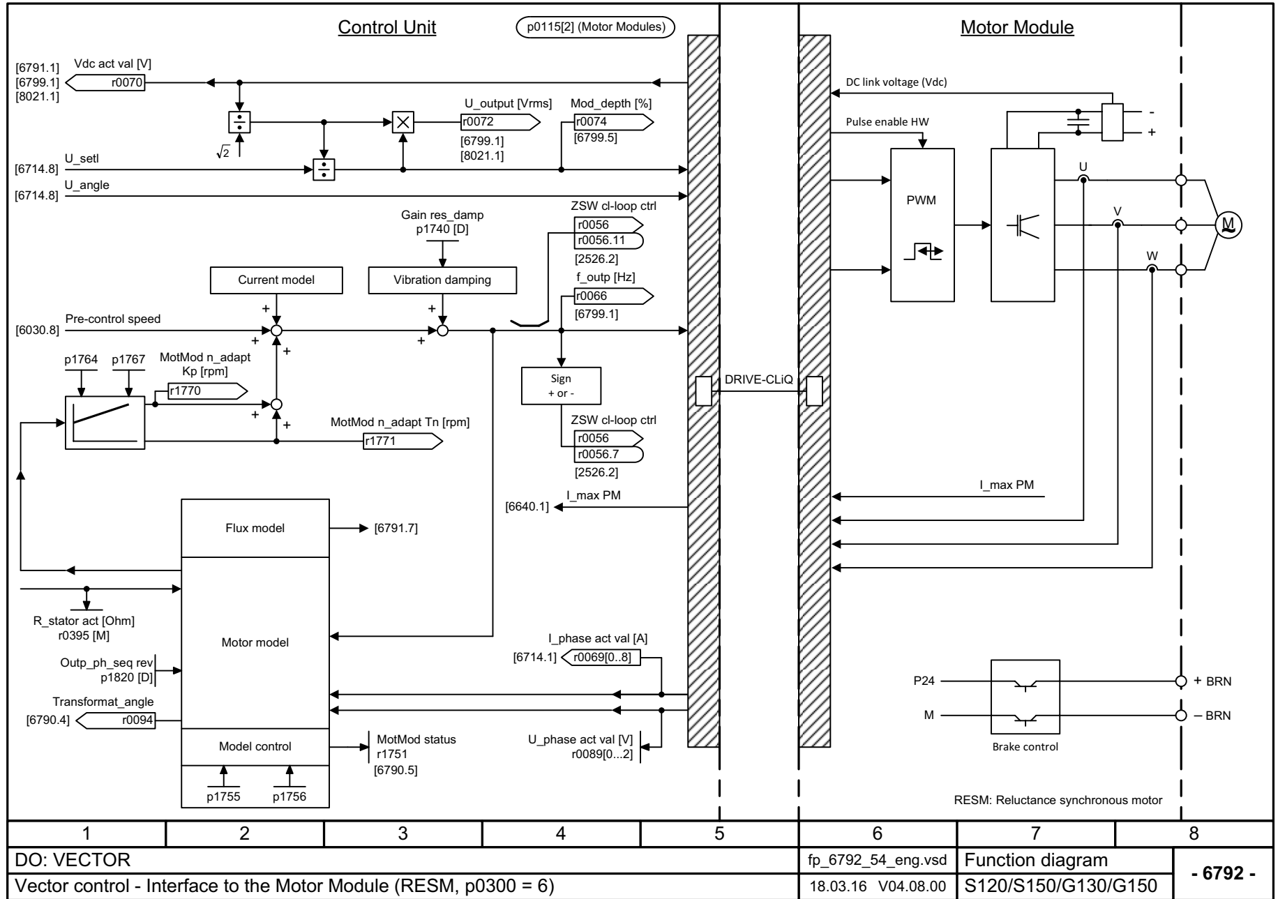
Fig. 3-260 6792 – Interface to the Motor Module (RESM, p0300 = 6)
