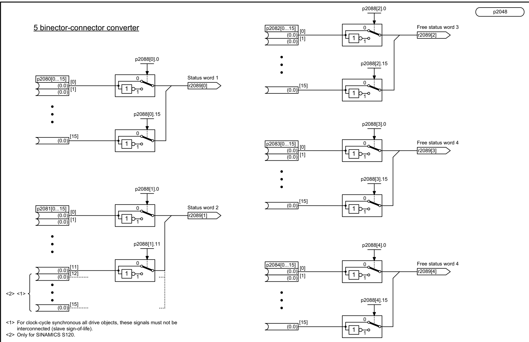
Fig. 3-75 2472 - IF1 status words, free interconnection
