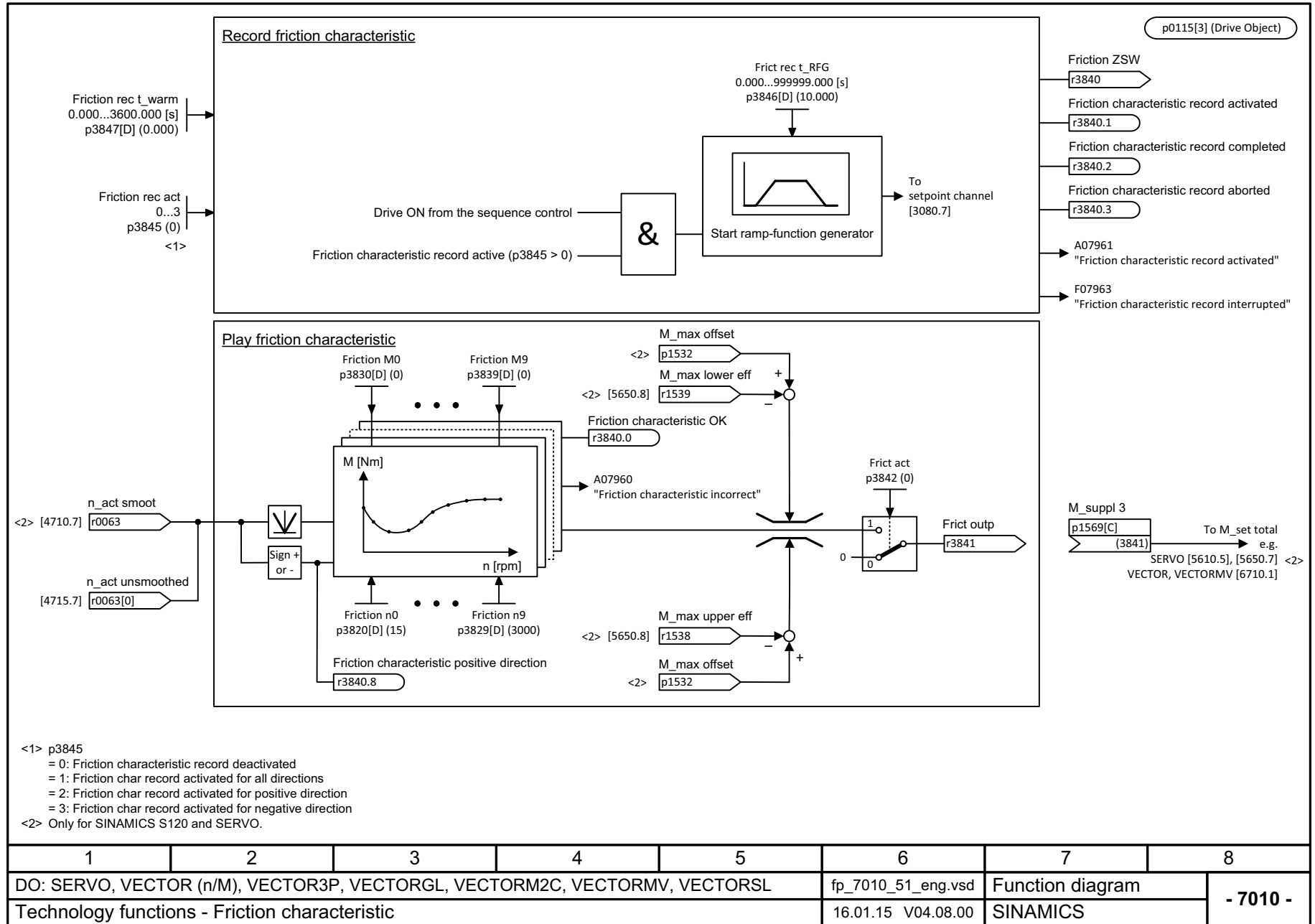
Fig. 3-263 7010 – Friction characteristic
