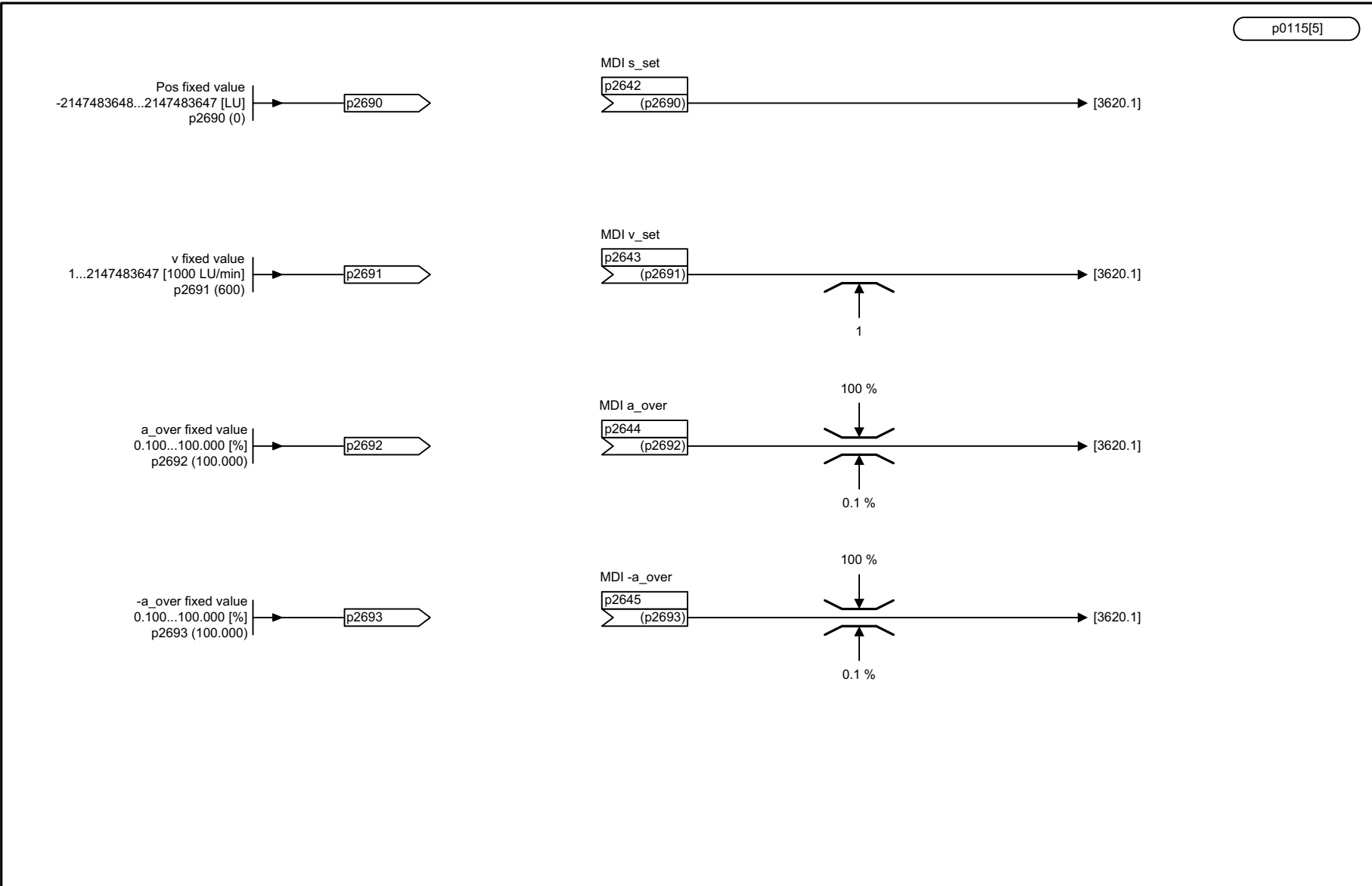
Fig. 3-169 3618 – Direct setpoint input/MDI mode, dynamic values (r0108.4 = 1)
