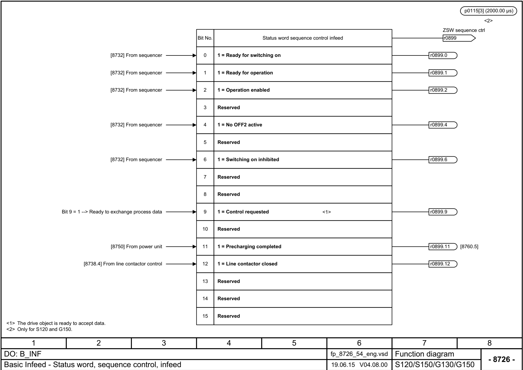
Fig. 3-319 8726 – Status word, sequence control infeed
