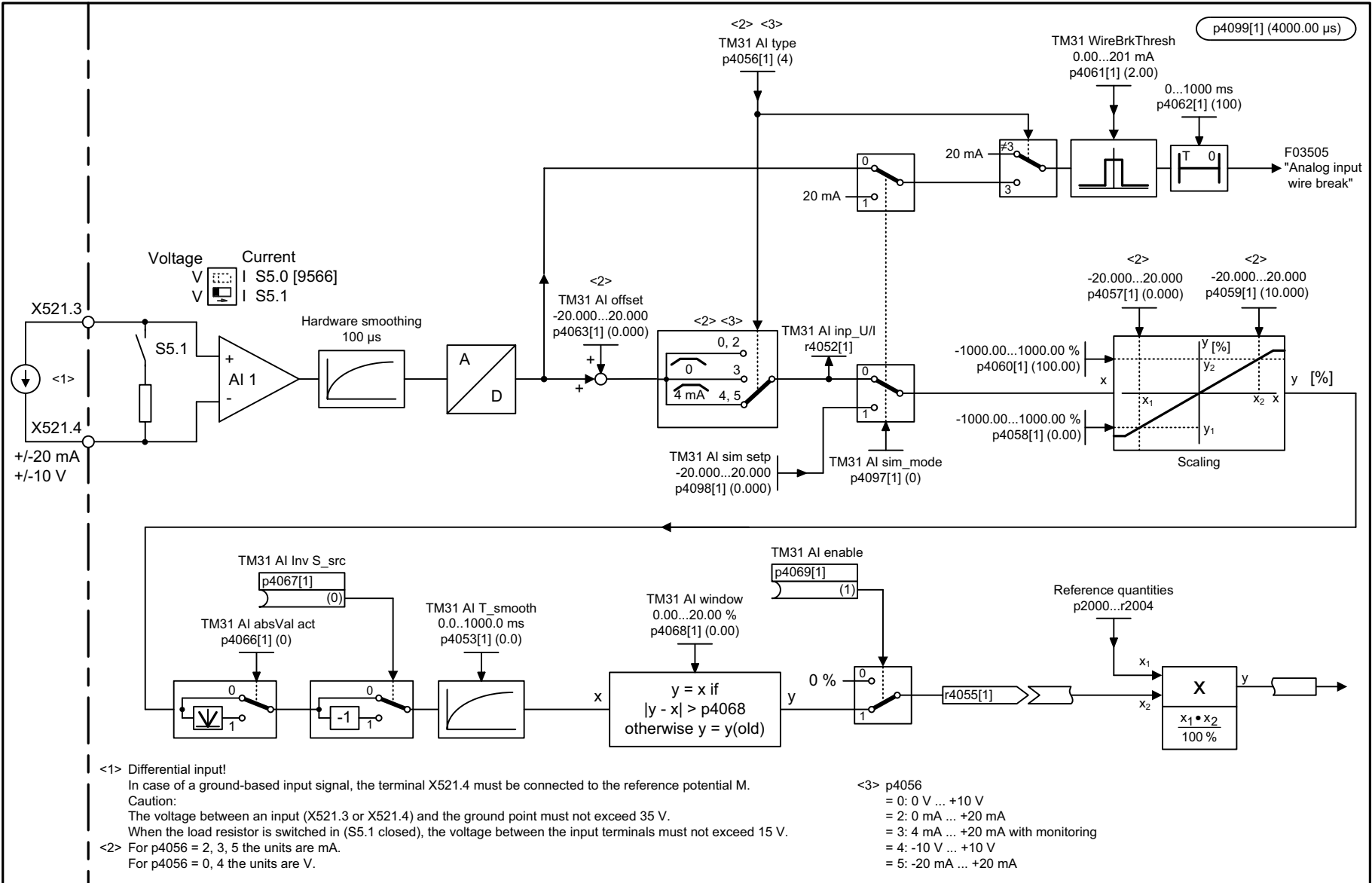
Fig. 3-371 9568 – Analog input 1 (AI 1)
