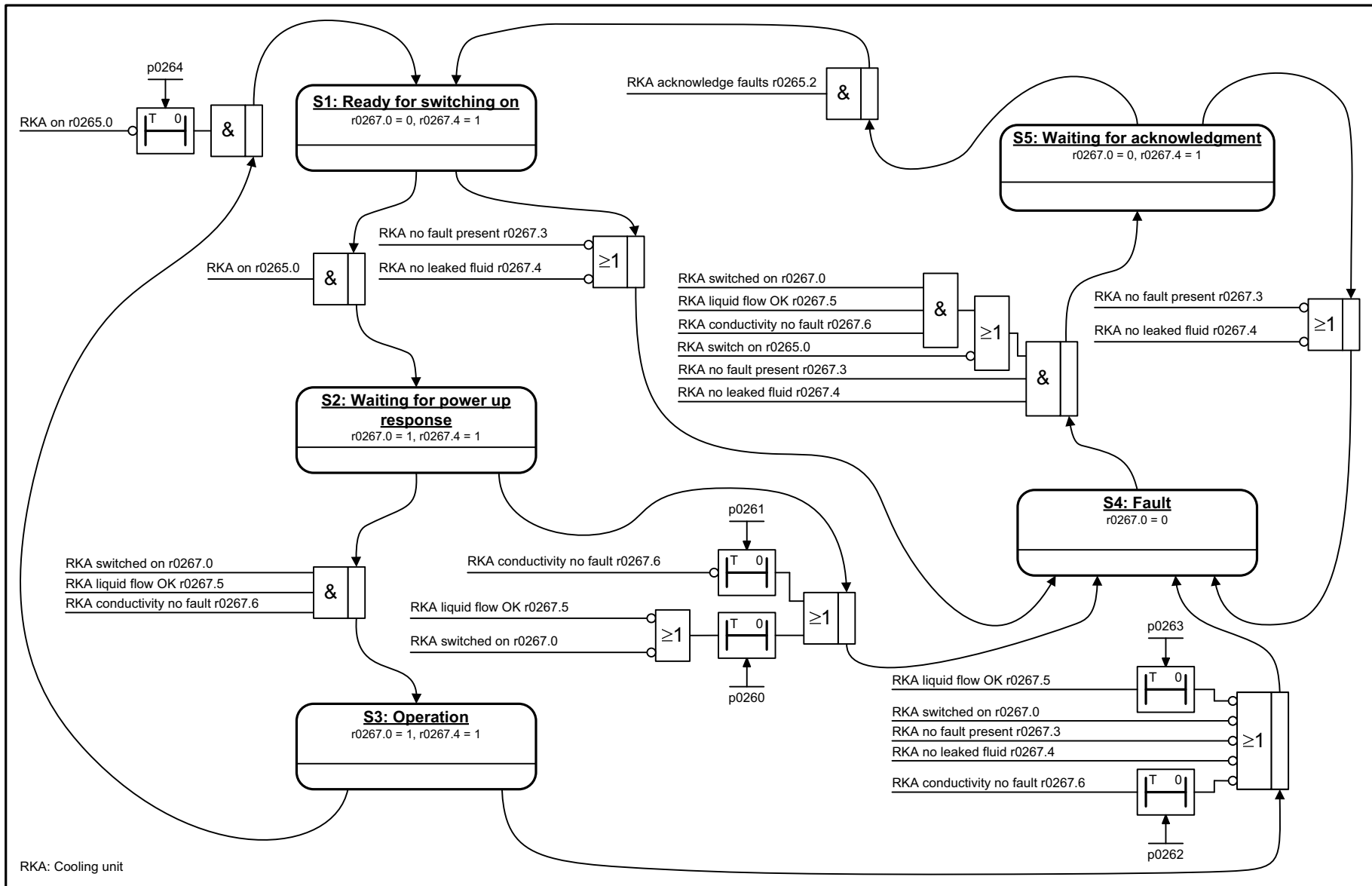
Fig. 3-394 9795 – Cooling unit, sequence control (r0108.28 = 1)
