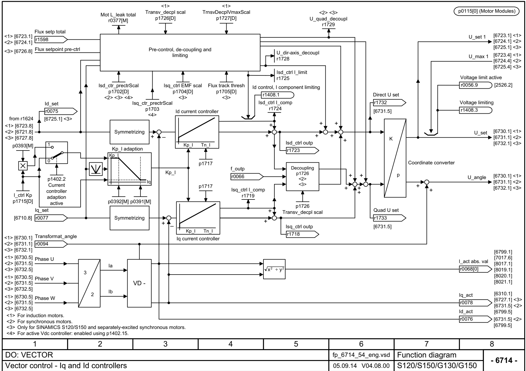
Fig. 3-246 6714 – Iq and Id controllers
