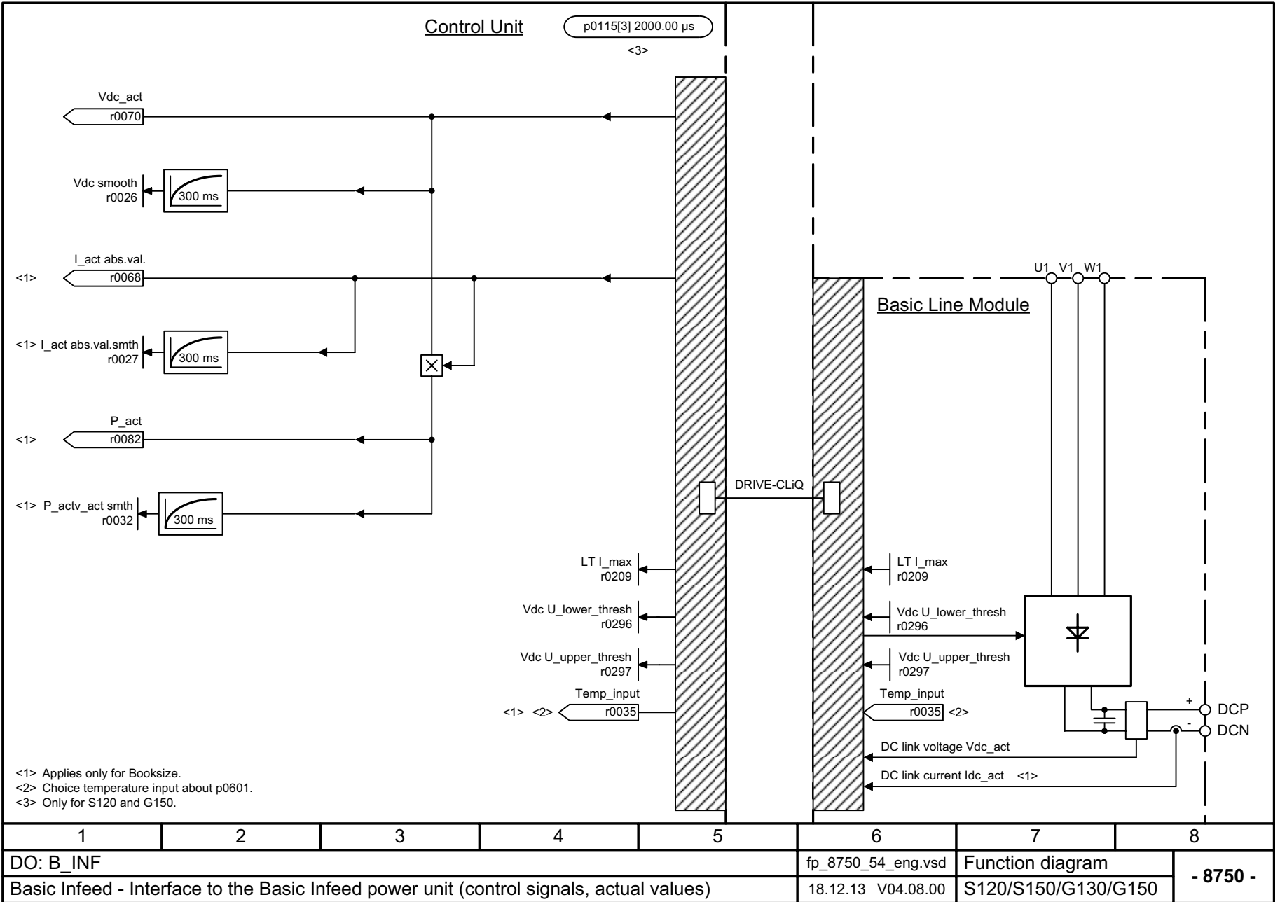
Fig. 3-322 8750 – Interface to the Basic Infeed power unit (control signals, actual values)
