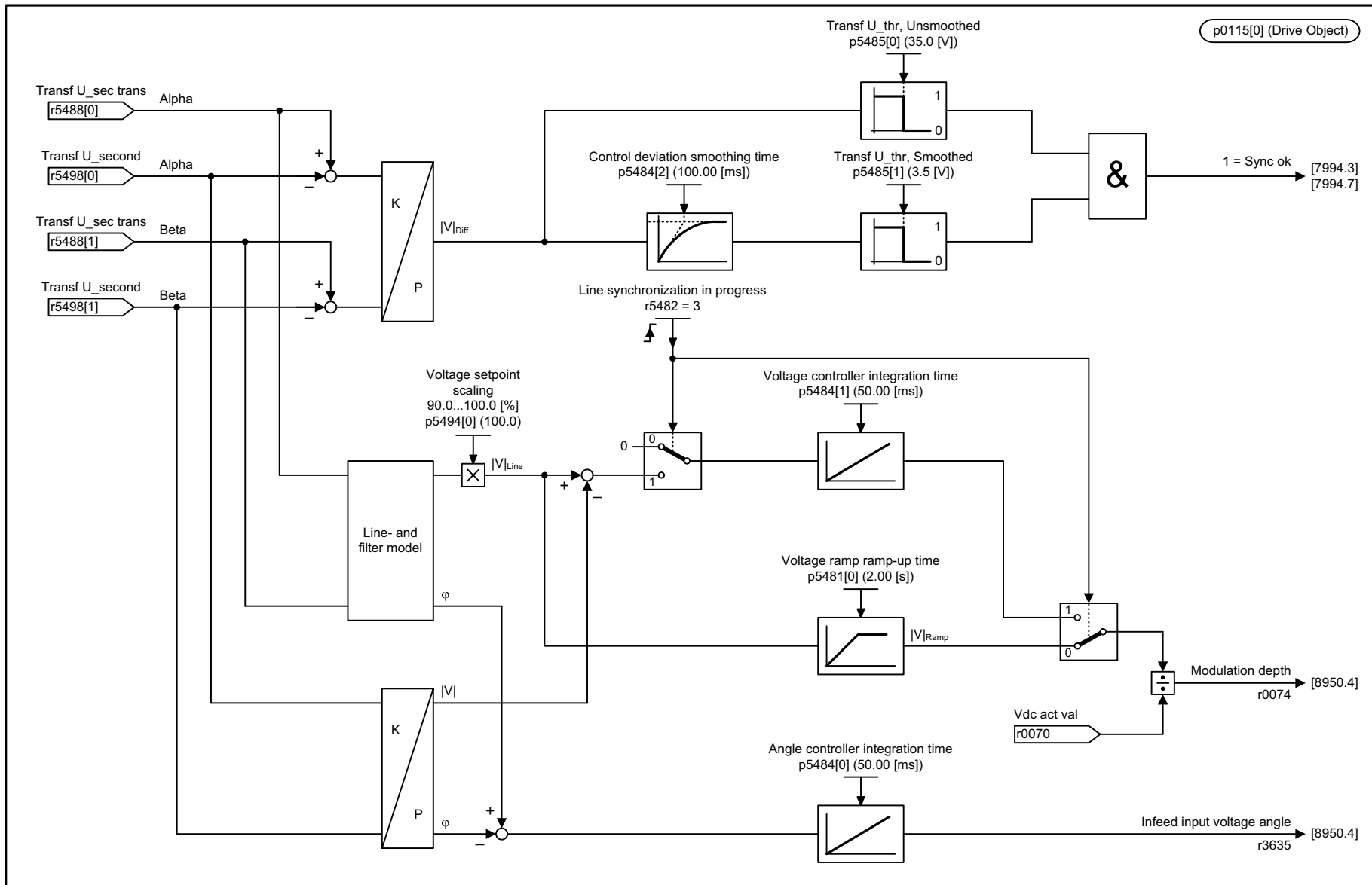
Fig. 3-286 7993 – Transformer magnetization, voltage threshold
