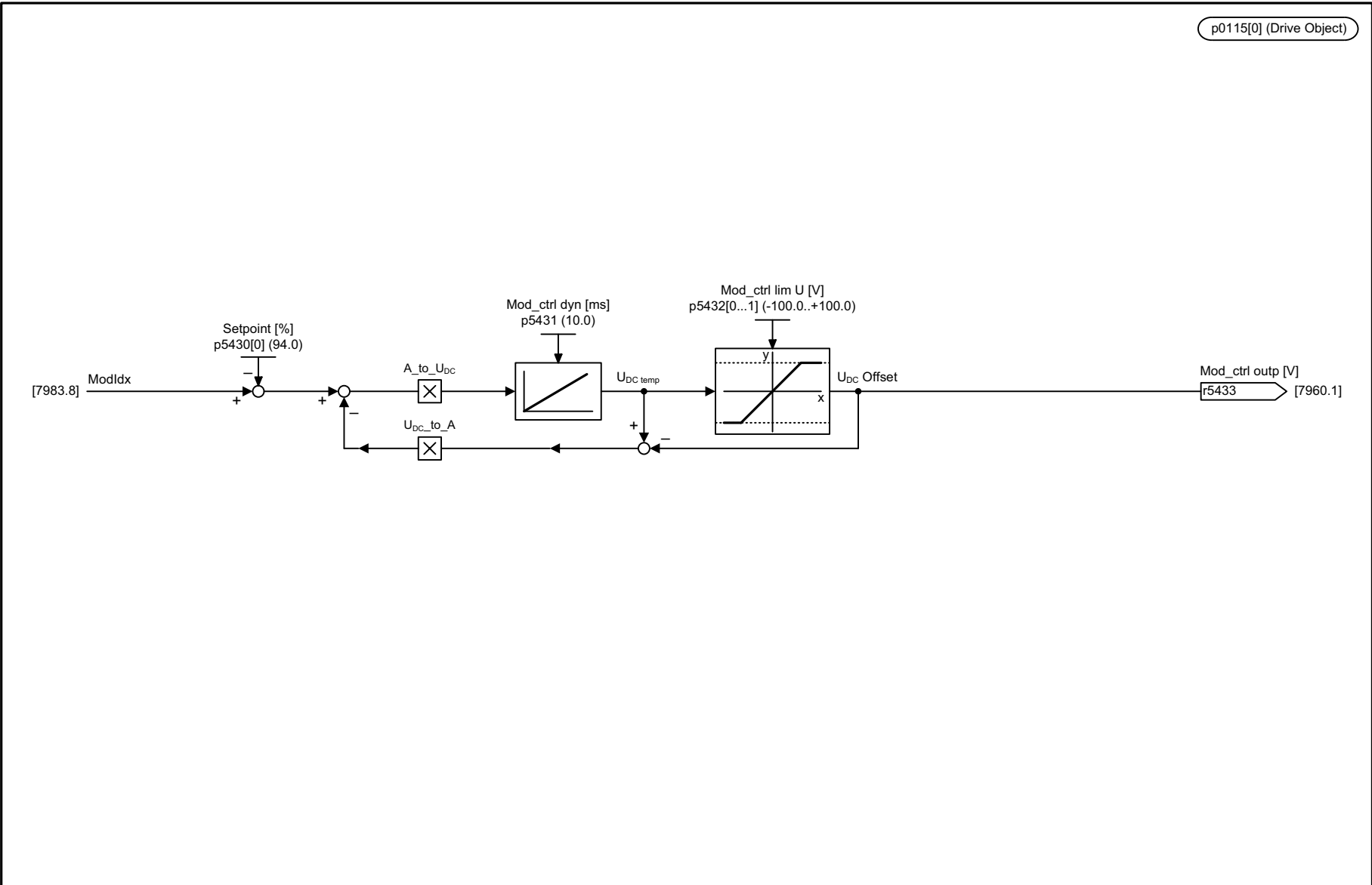
Fig. 3-278 7984 – Modulation depth control
