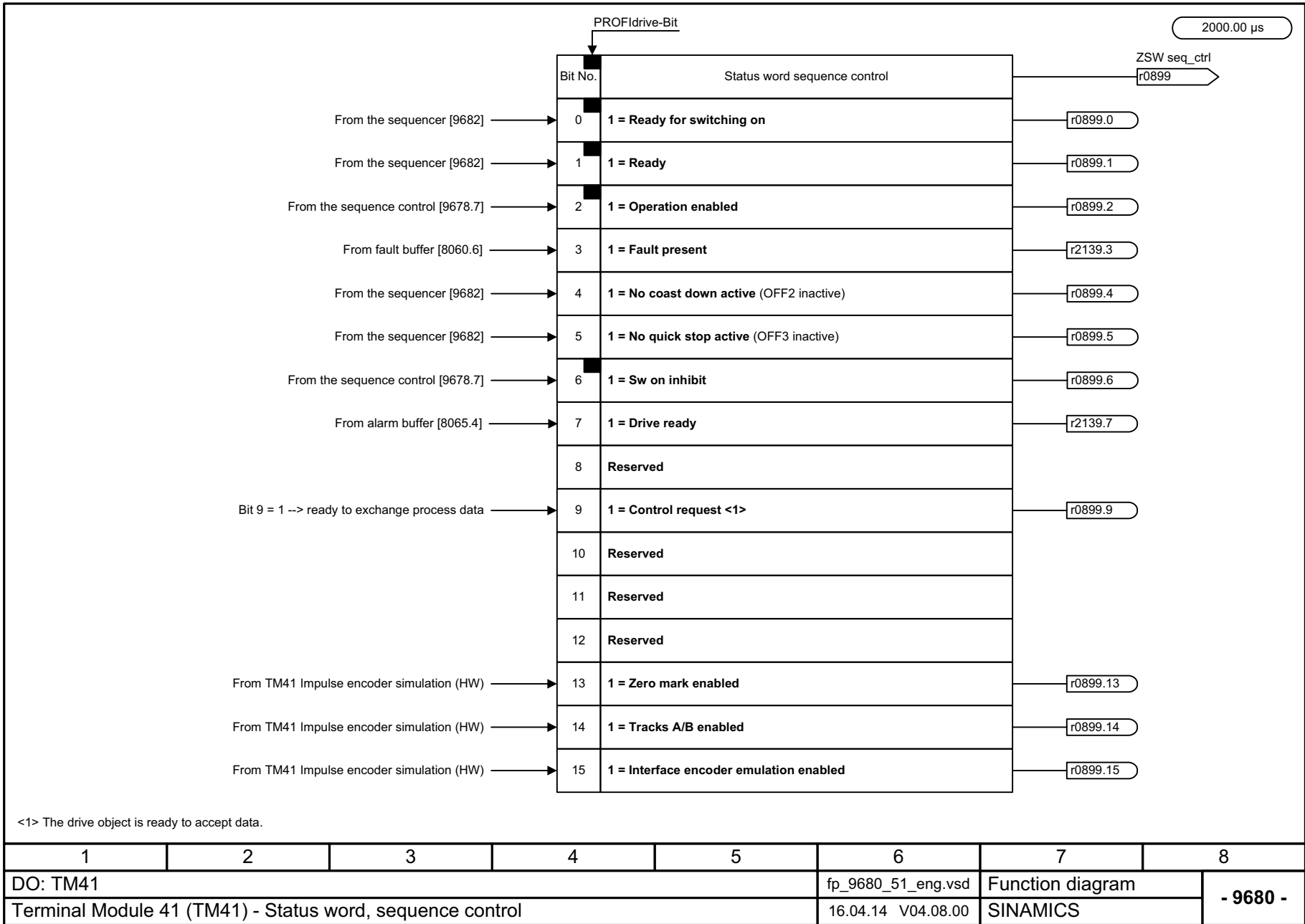
Fig. 3-389 9680 – Status word, sequence control
