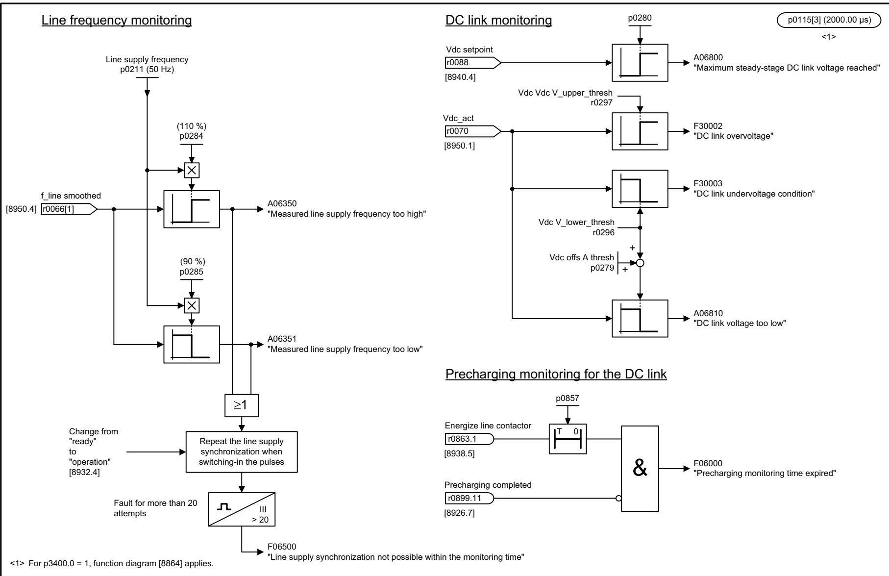
Fig. 3-346 8964 – Signals and monitoring functions, line frequency/Vdc monet. (p3400.0 = 0)
