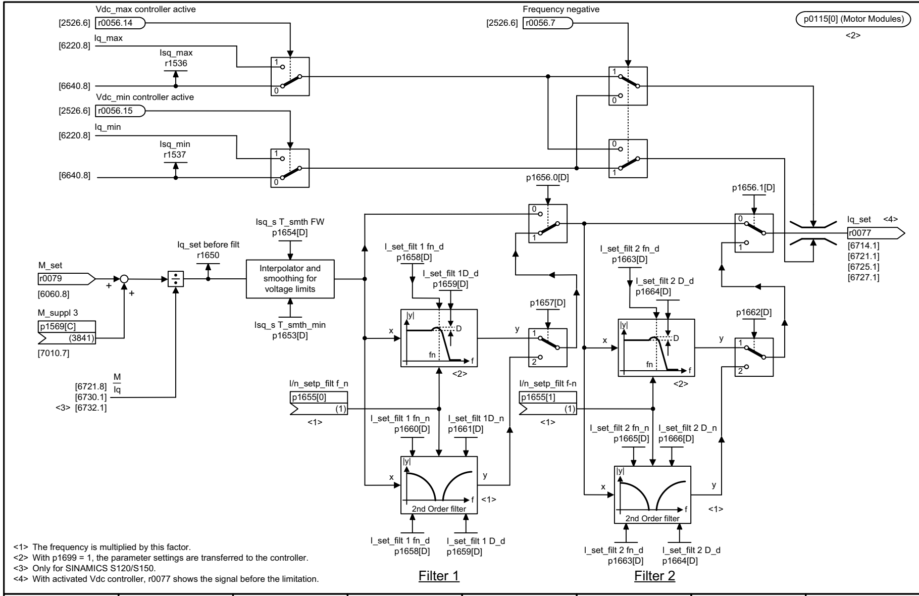
Fig. 3-245 6710 – Current setpoint filter
