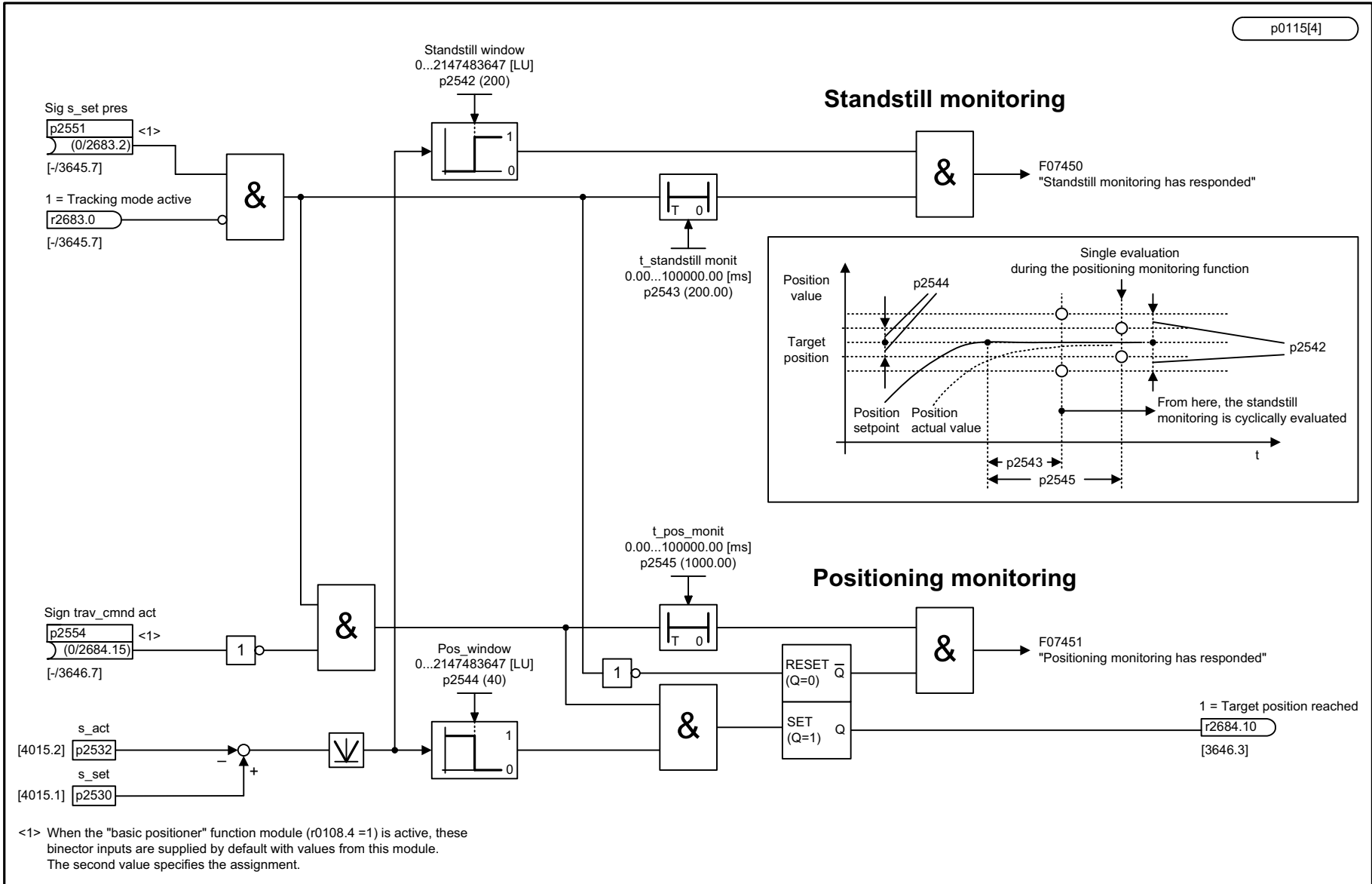
Fig. 3-180 4020 – Standstill monitoring / positioning monitoring (r0108.3 = 1)
