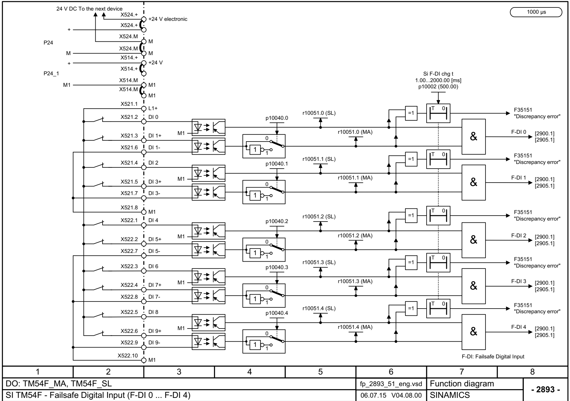
Fig. 3-140 2893 – Fail-safe digital inputs (F-DI 0 ... F-DI 4)
