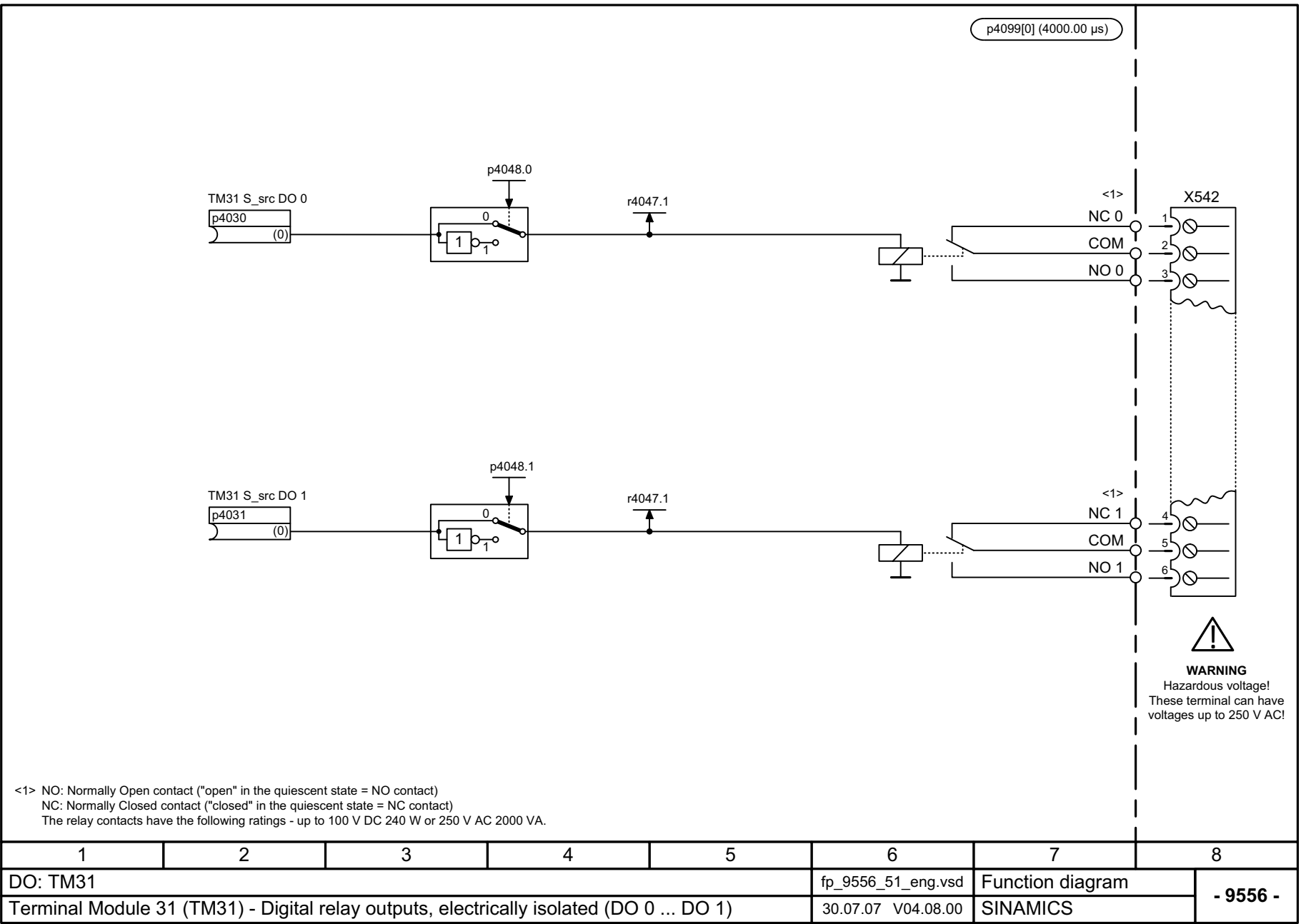
Fig. 3-367 9556 – Digital relay outputs, electrically isolated (DO 0 ... DO 1)
