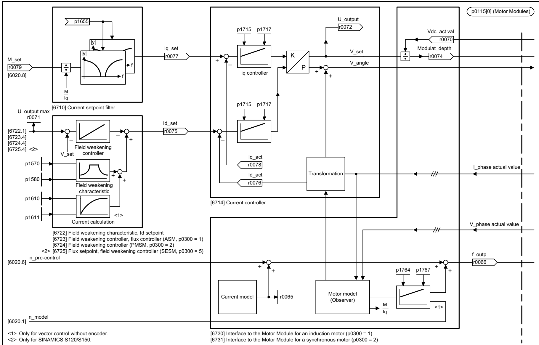
Fig. 3-244 6700 – Current control, overview
