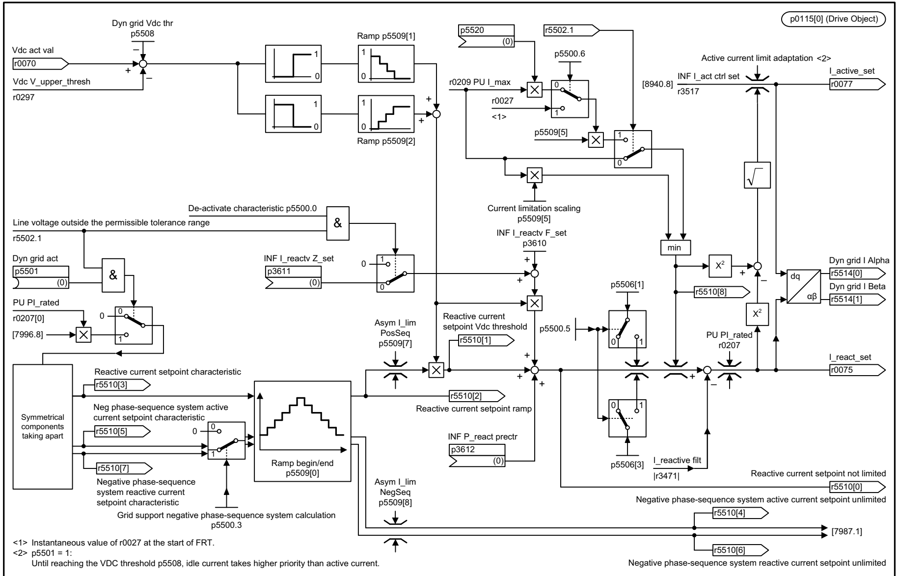
Fig. 3-289 7997 - Current limits (p5501 = 1)
