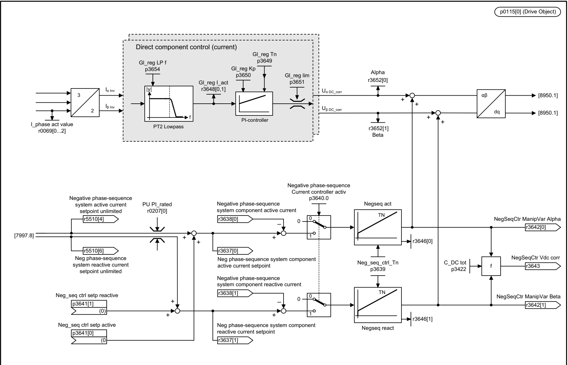
Fig. 3-280 7987 – Direct component control, negative sequence system controller
