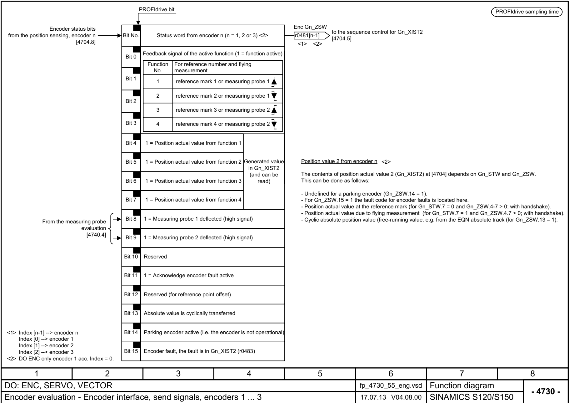
Fig. 3-189 4730 – Encoder interface, send signals, encoders 1 ... 3
