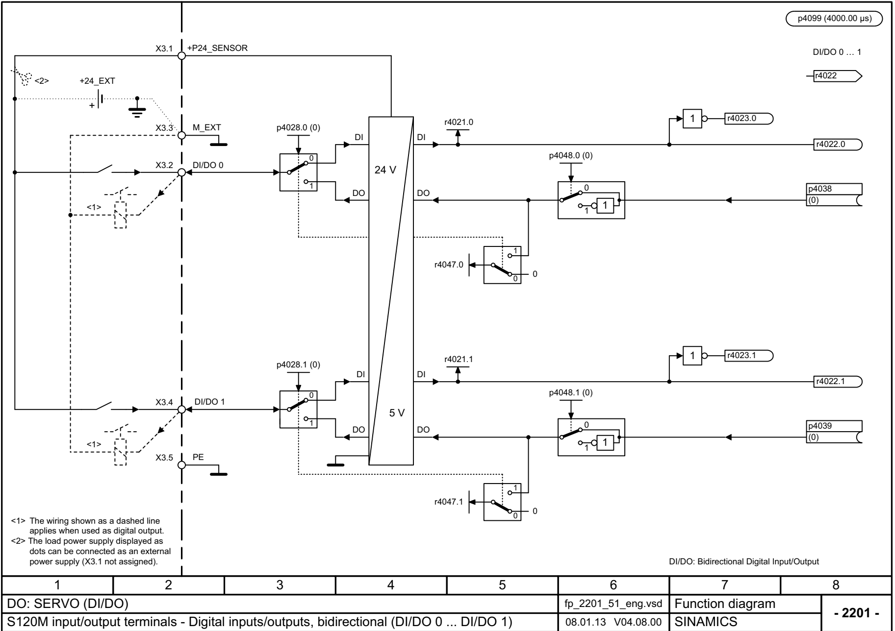
Fig. 3-31 2201 – Digital inputs/outputs, bidirectional (DI/DO 0 ... DI/DO 1)
