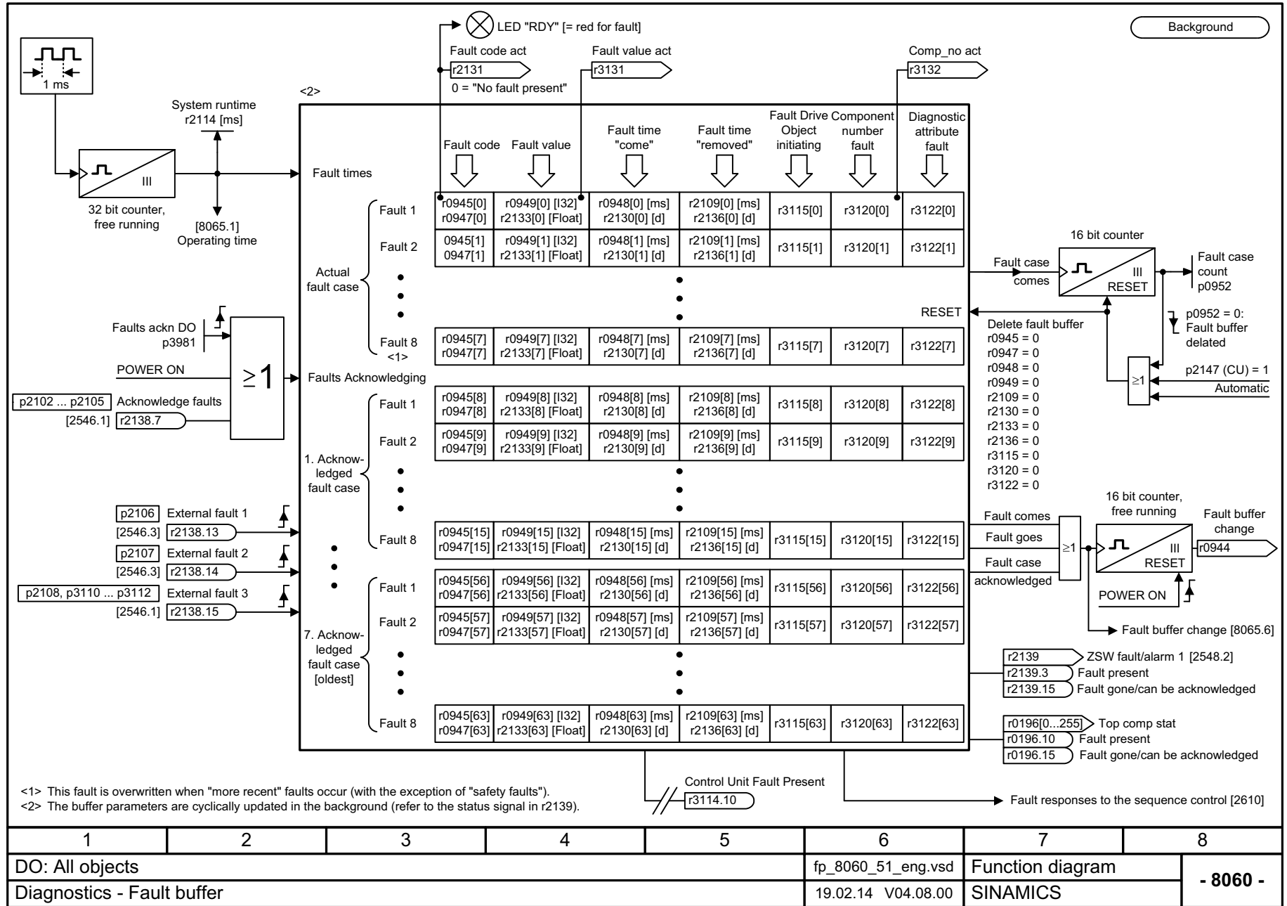
Fig. 3-305 8060 – Fault buffer
