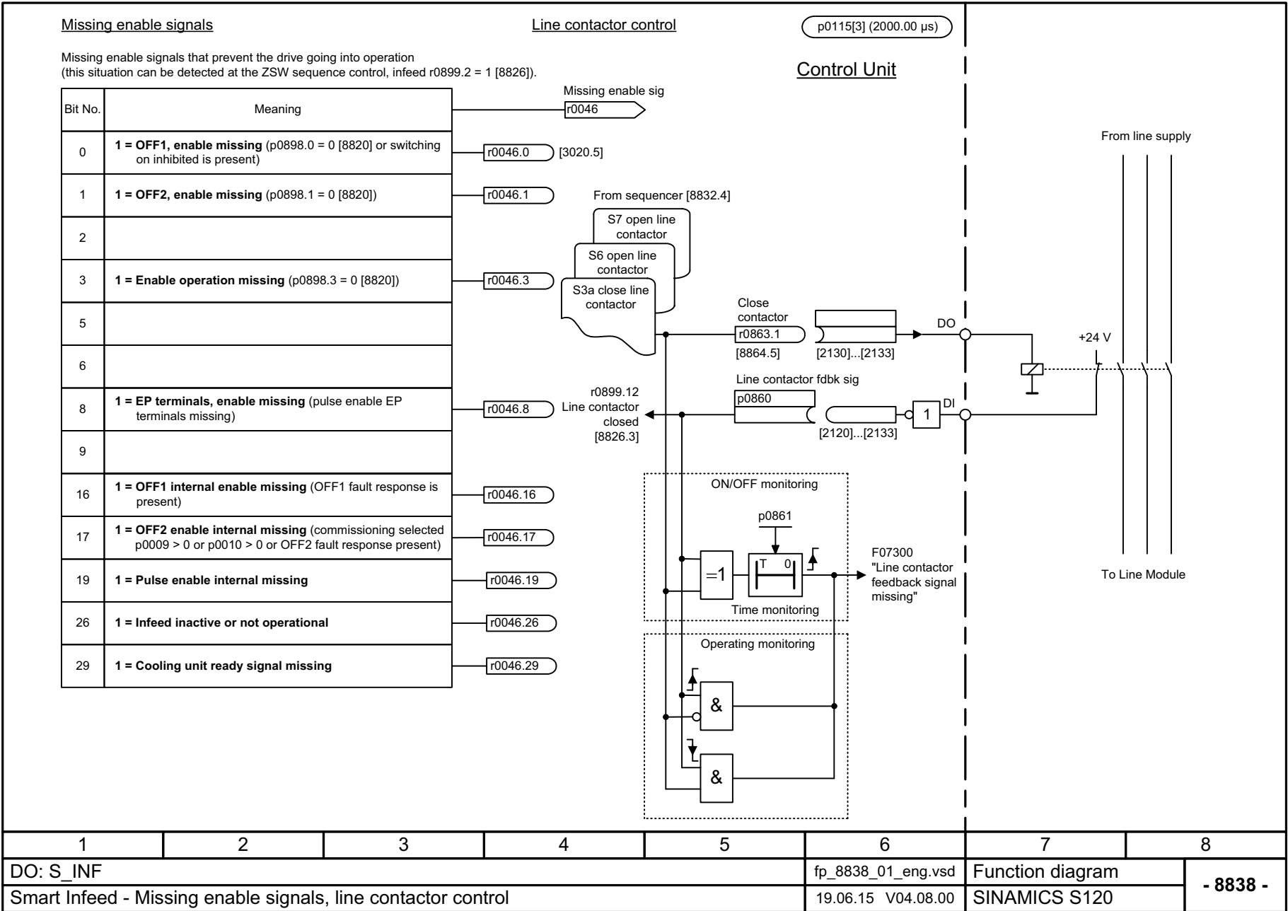
Fig. 3-329 8838 – Missing enable signals, line contactor control
