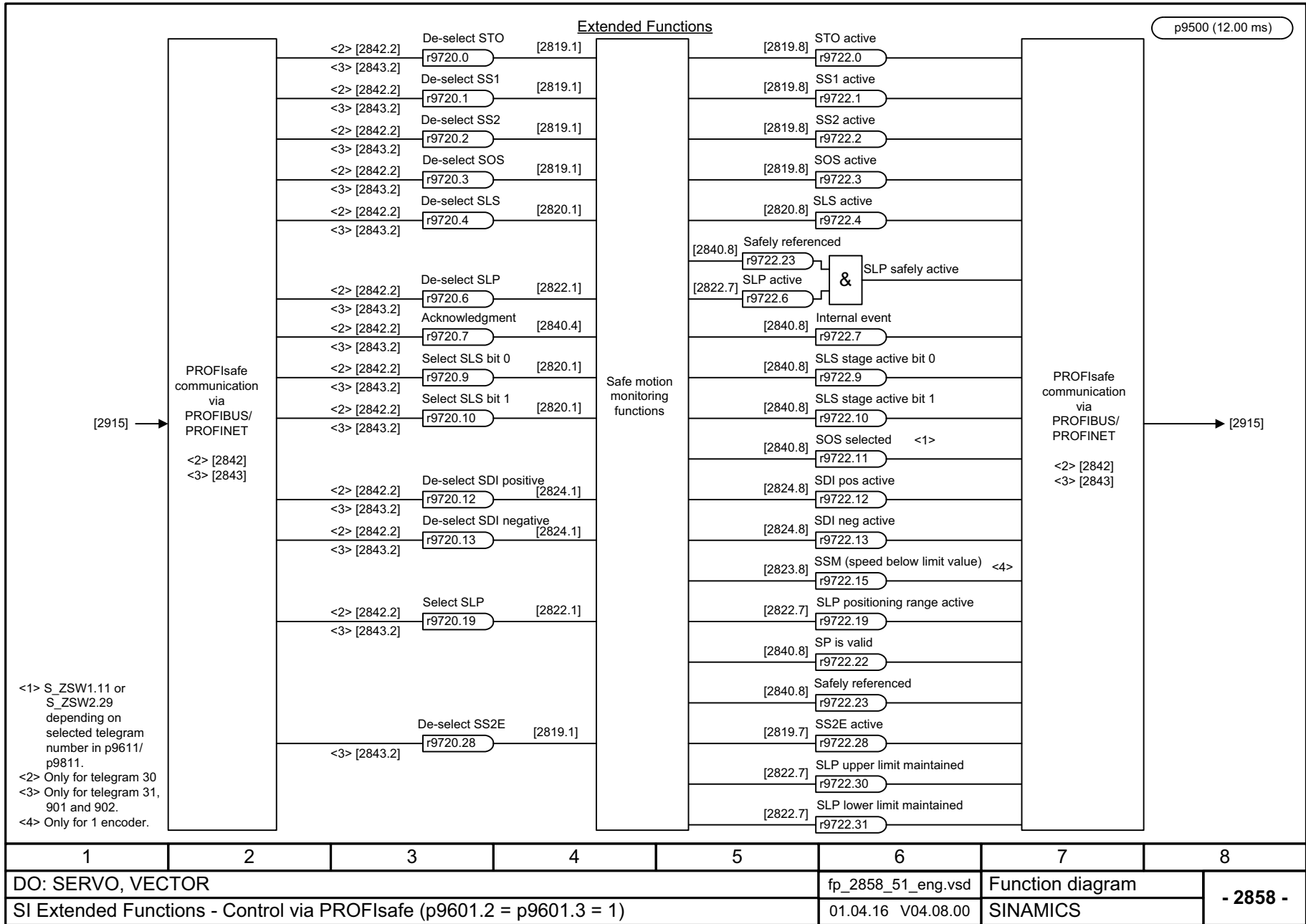
Fig. 3-131 2858 – Control via PROFIsafe (p9601.2 = p9601.3 = 1)
