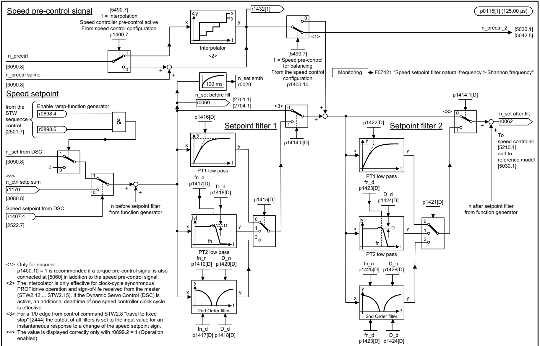
Fig. 3-203 5020 – Speed setpoint filter and speed precontrol
