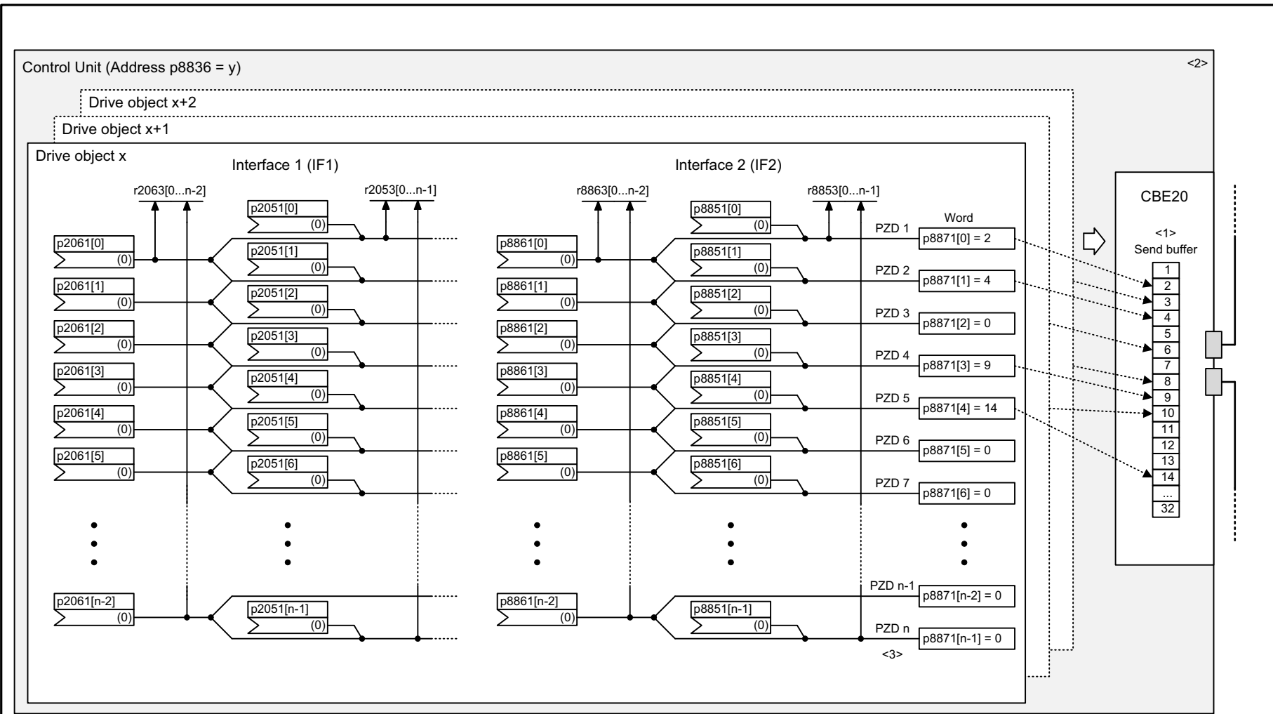
Fig. 3-30 2200 – SINAMICS Link send data (r0108.31 = 1, p8835 = 3)
