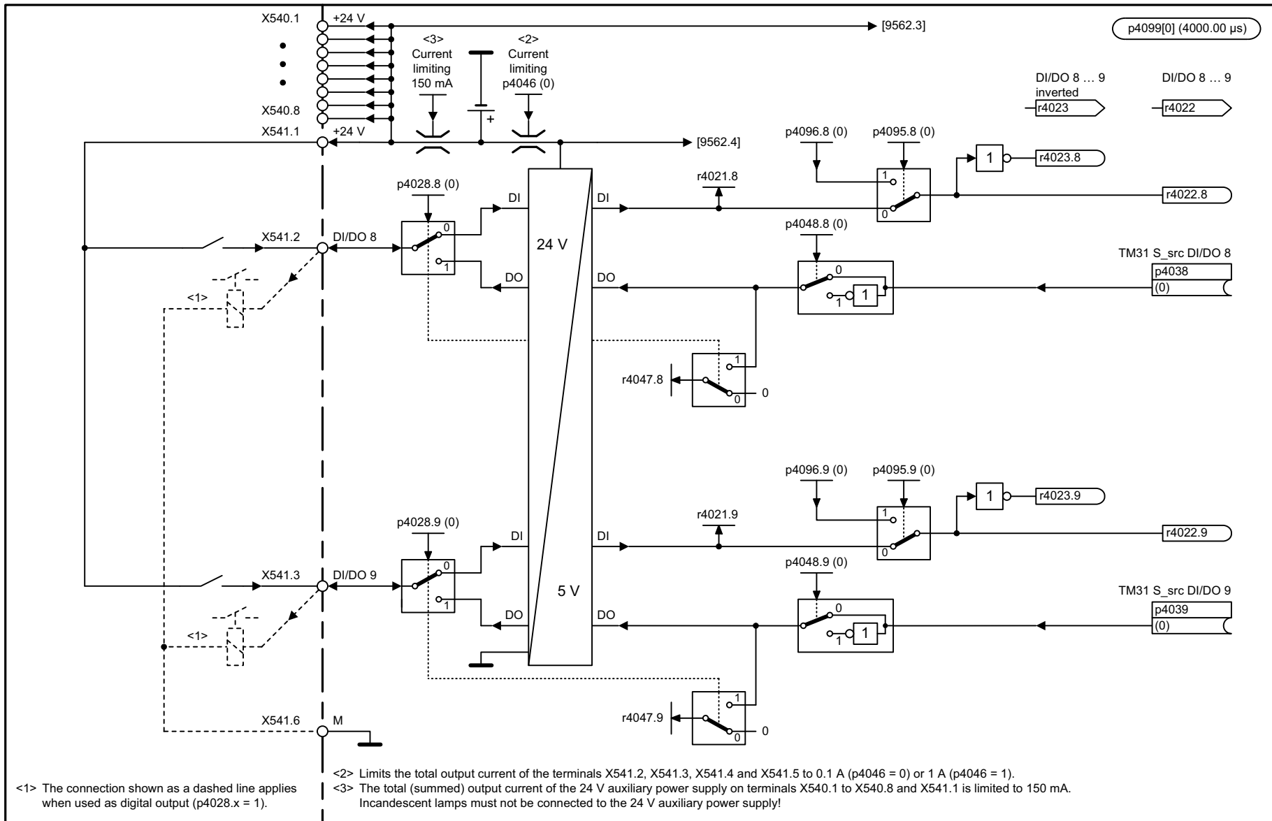
Fig. 3-368 9560 – Digital inputs/outputs, bidirectional (DI/DO 8 ... DI/DO 9)
