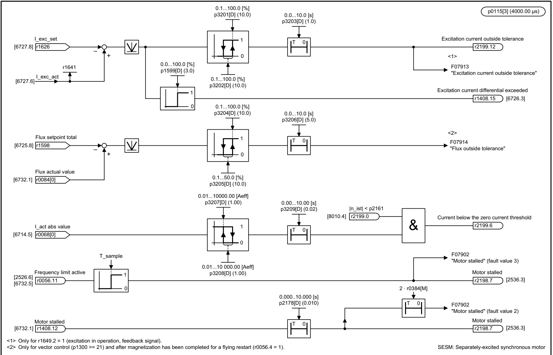
Fig. 3-301 8020 – Separately excited synchronous motor (SESM; p0300 = 5)
