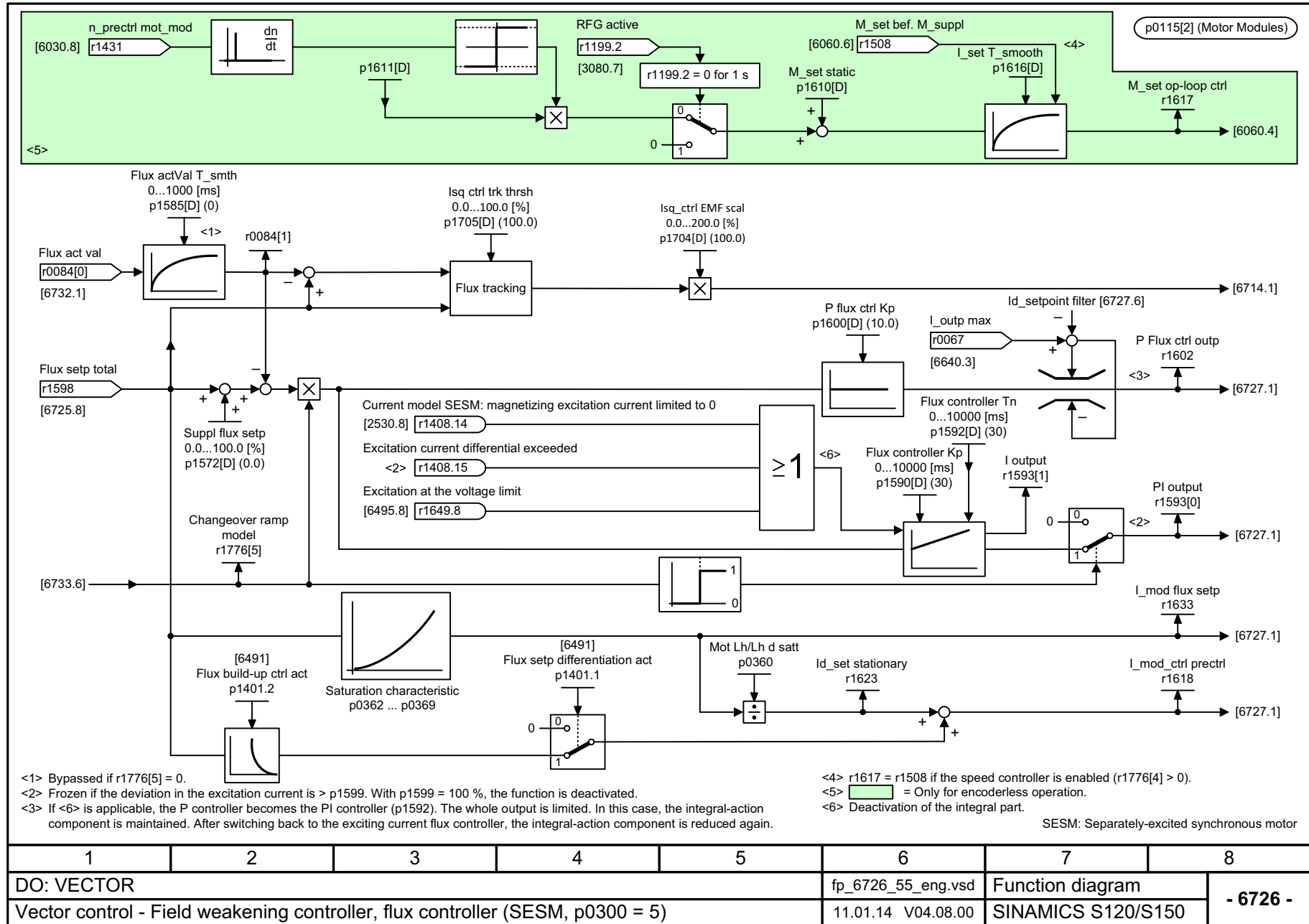
Fig. 3-252 6726 – Field weakening controller, flux controller (FEM, p0300 = 5)
