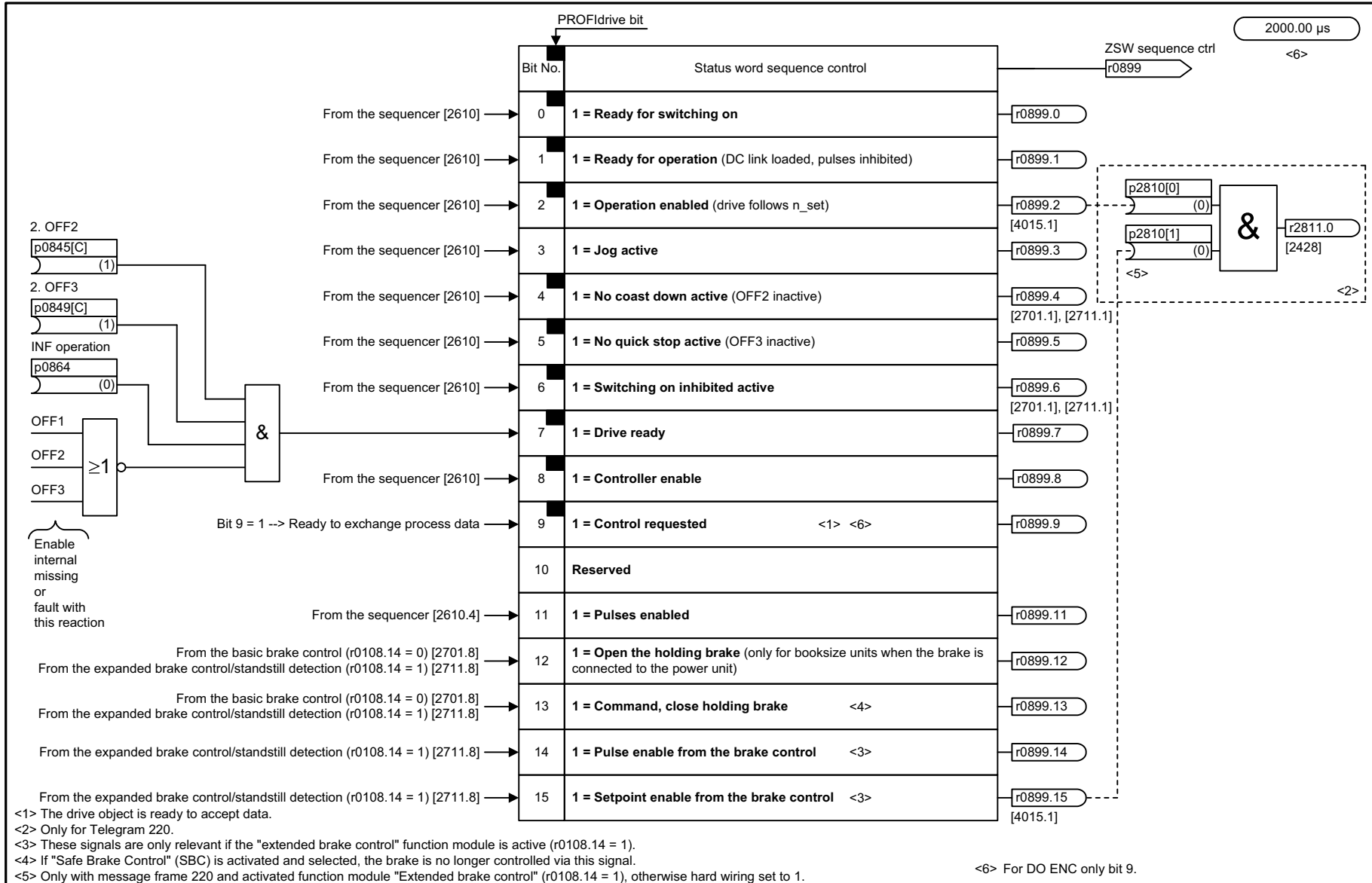
Fig. 3-94 2503 – Status word, sequence control
