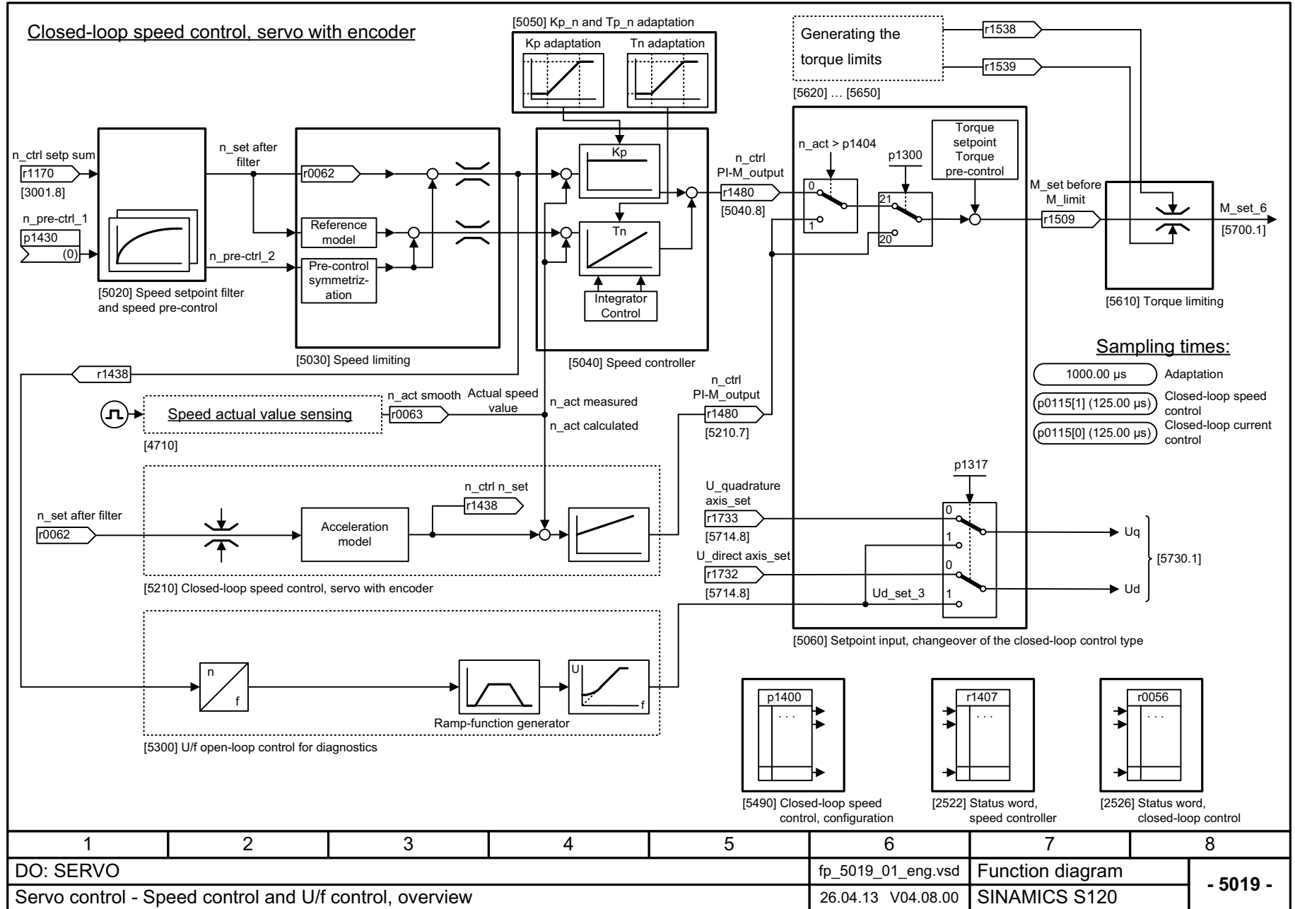
Fig. 3-202 5019 – Speed control and U/f control, overview
