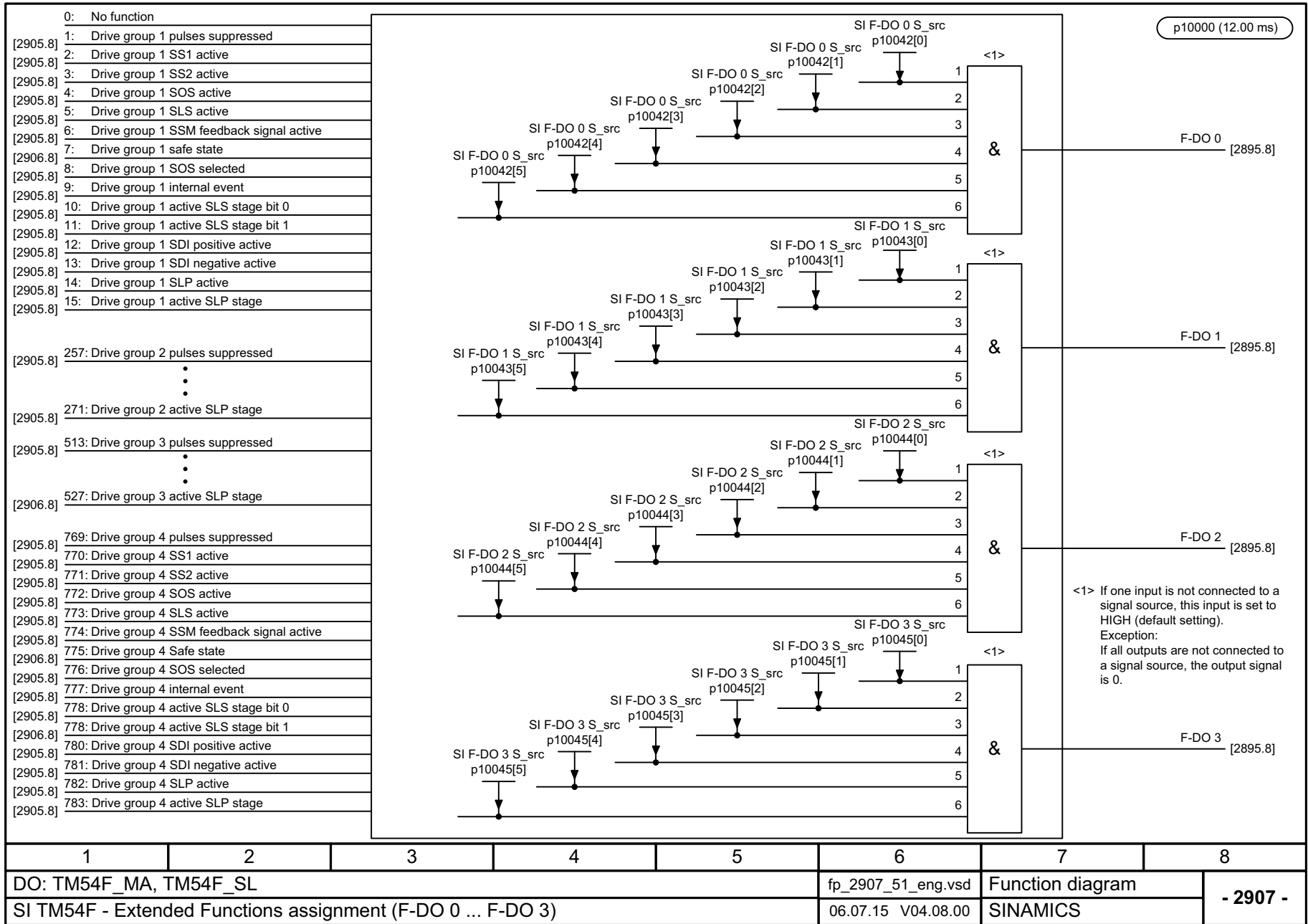
Fig. 3-148 2907 – Extended Functions assignment (F-DO 0 ... F-DO 3)
