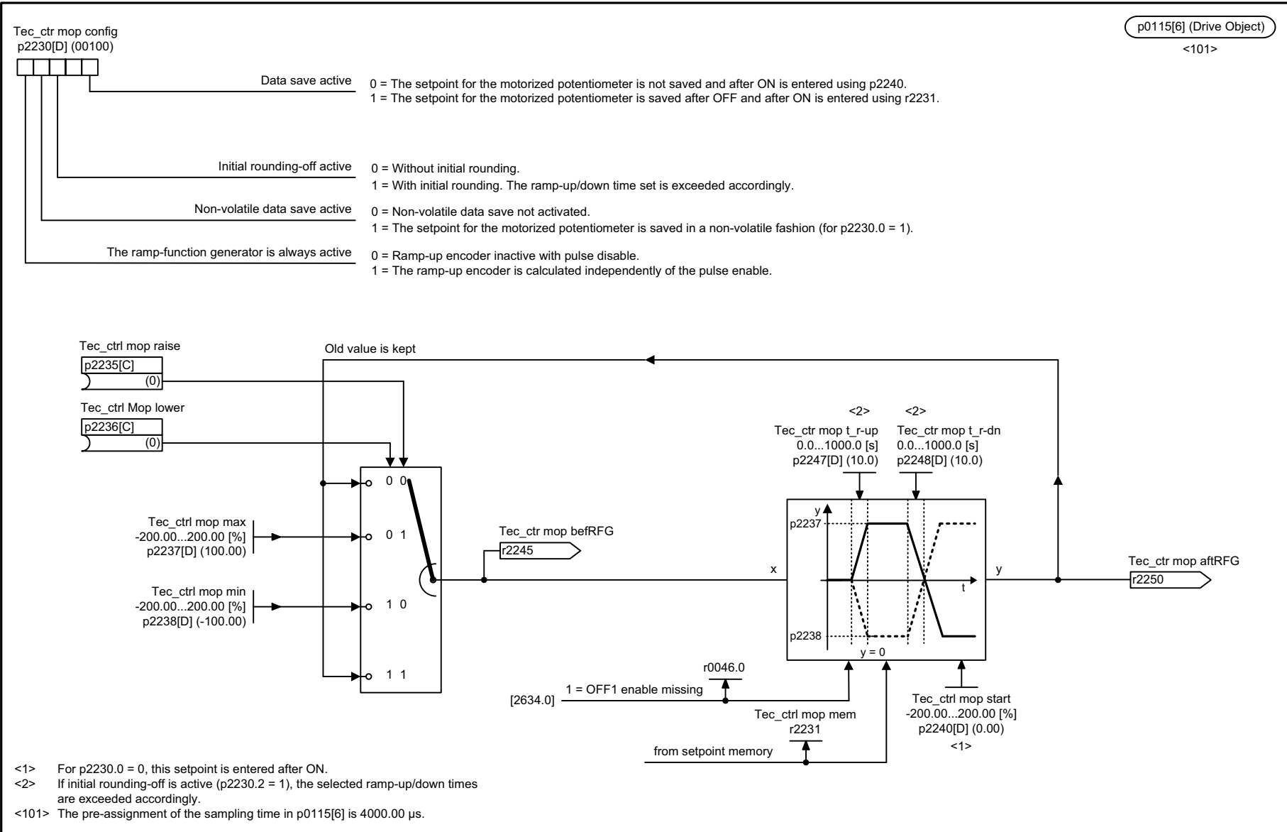
Fig. 3-273 7954 – Motorized potentiometer (r0108.16 = 1)
