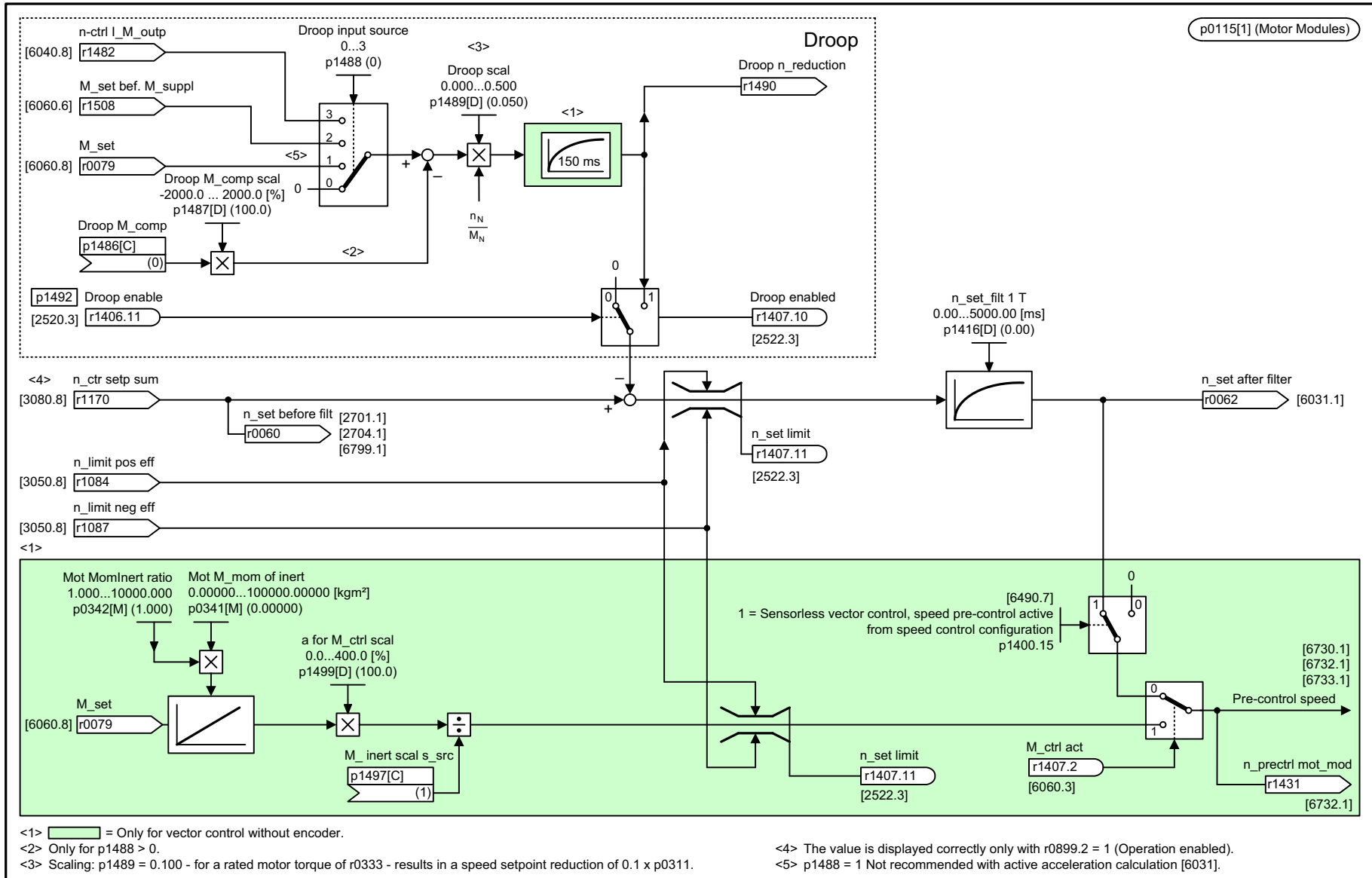
Fig. 3-228 6030 – Speed setpoint, droop
