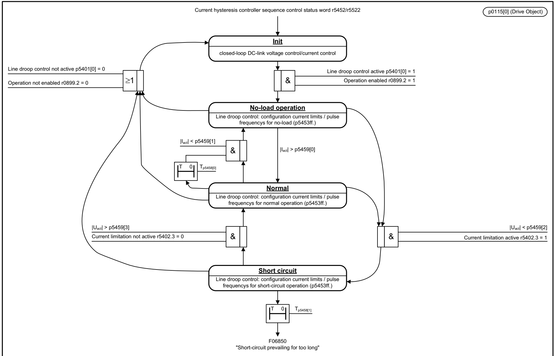
Fig. 3-279 7986 – Sequence control, overcurrent
