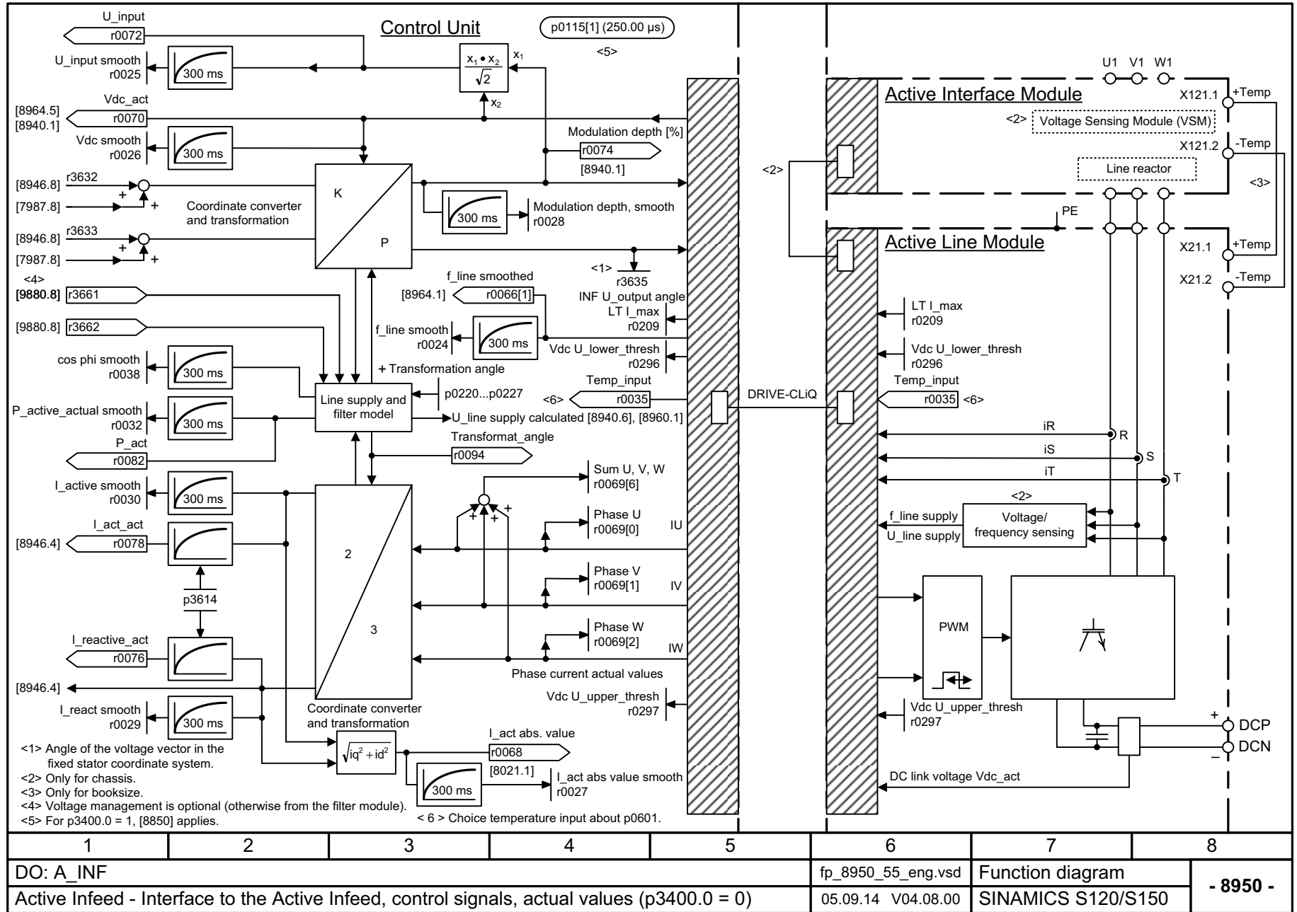
Fig. 3-343 8950 – Interface to the Active Infeed, control signals, actual values (p3400.0 = 0)
