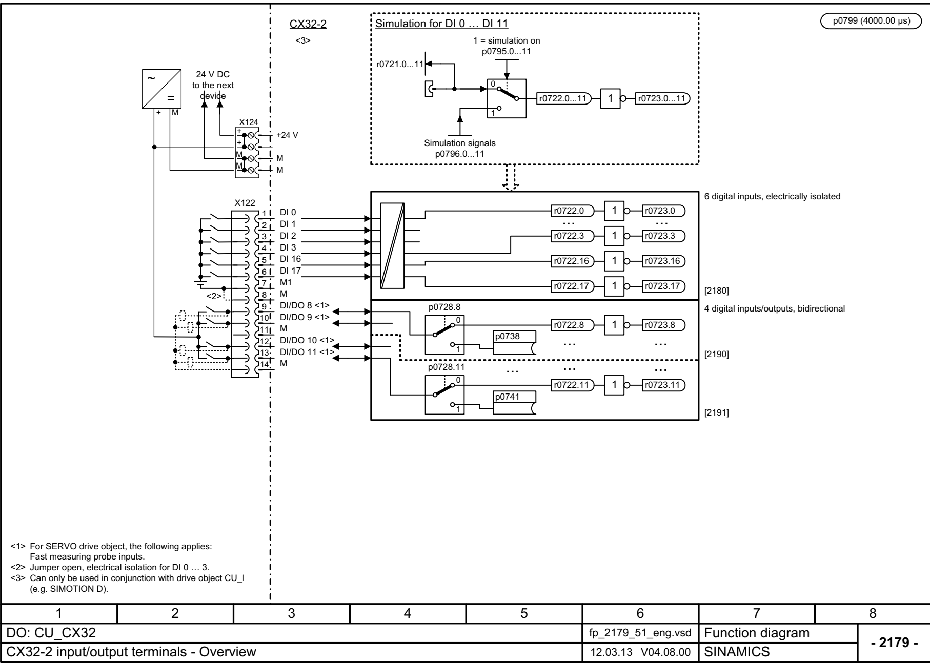
Fig. 3-21 2179 – Overview
