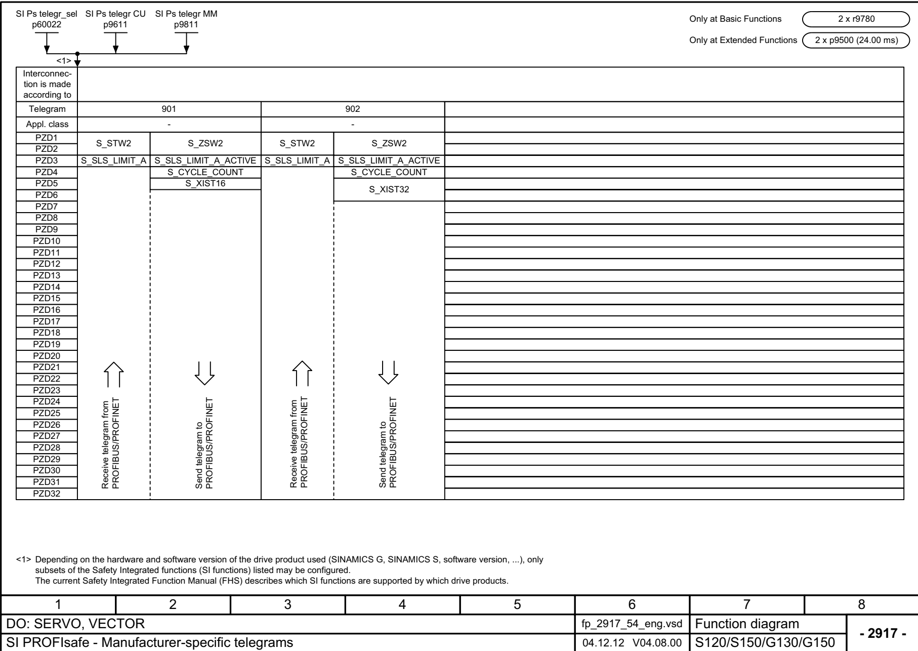
Fig. 3-150 2917 – Manufacturer-specific telegrams
