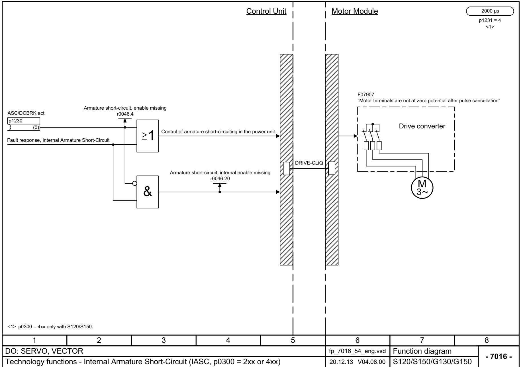
Fig. 3-267 7016 – Internal armature short-circuit (IASC, p0300 = 2xx or 4xx)
