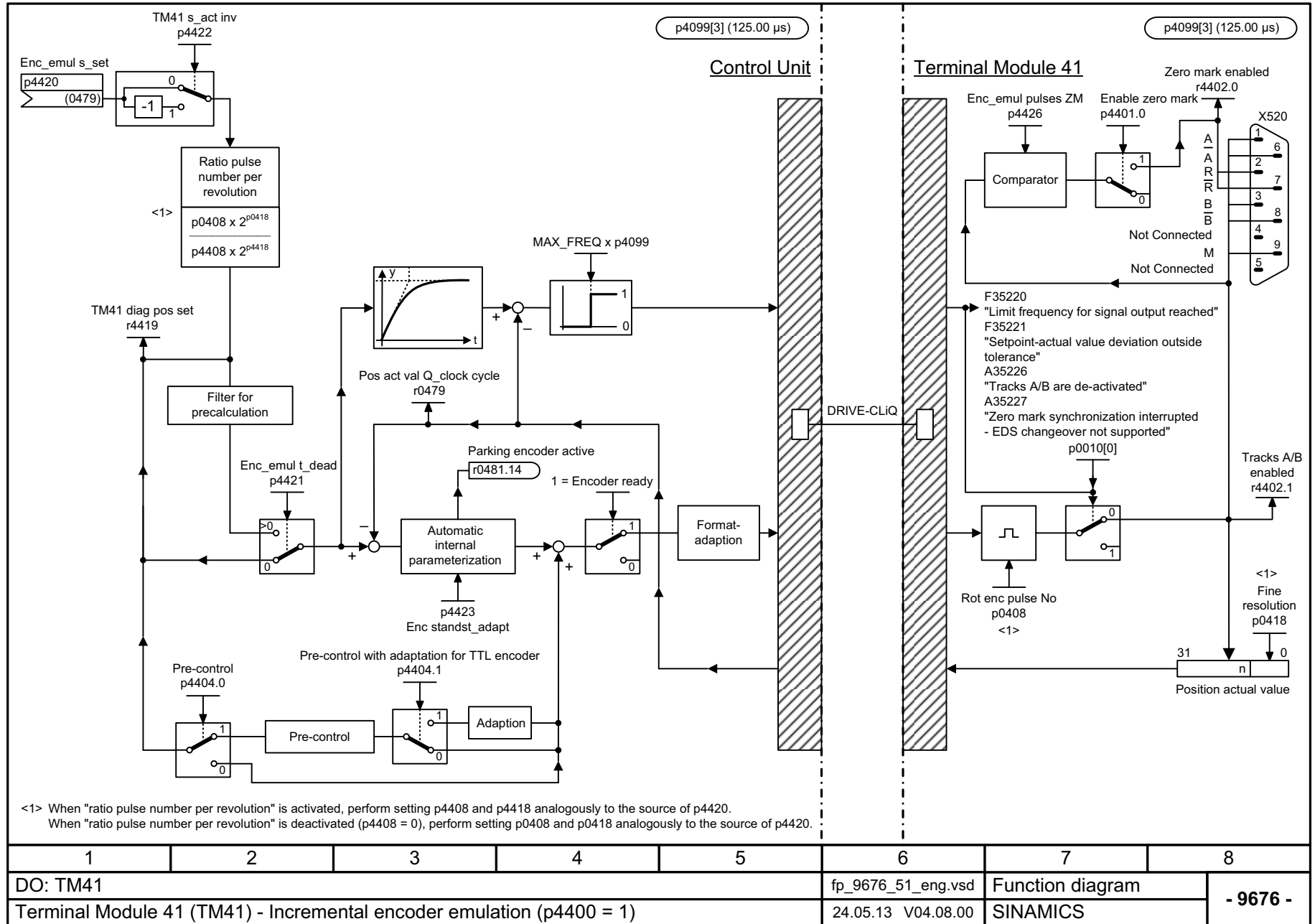
Fig. 3-385 9676 – Incremental encoder emulation (p4400 = 1)
