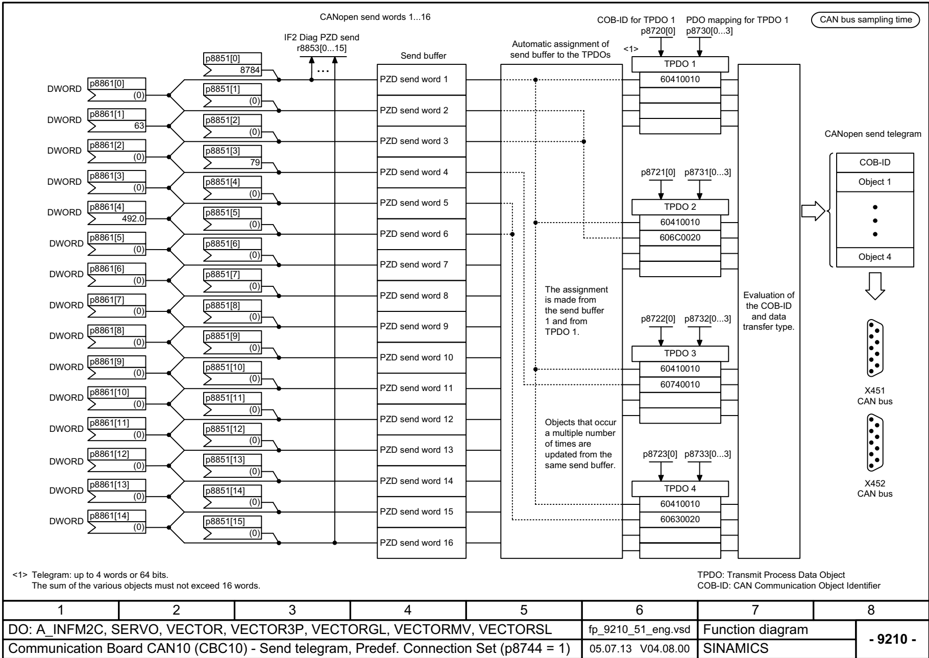
Fig. 3-355 9210 – Send telegram, Predefined Connection Set (p8744 = 1)
