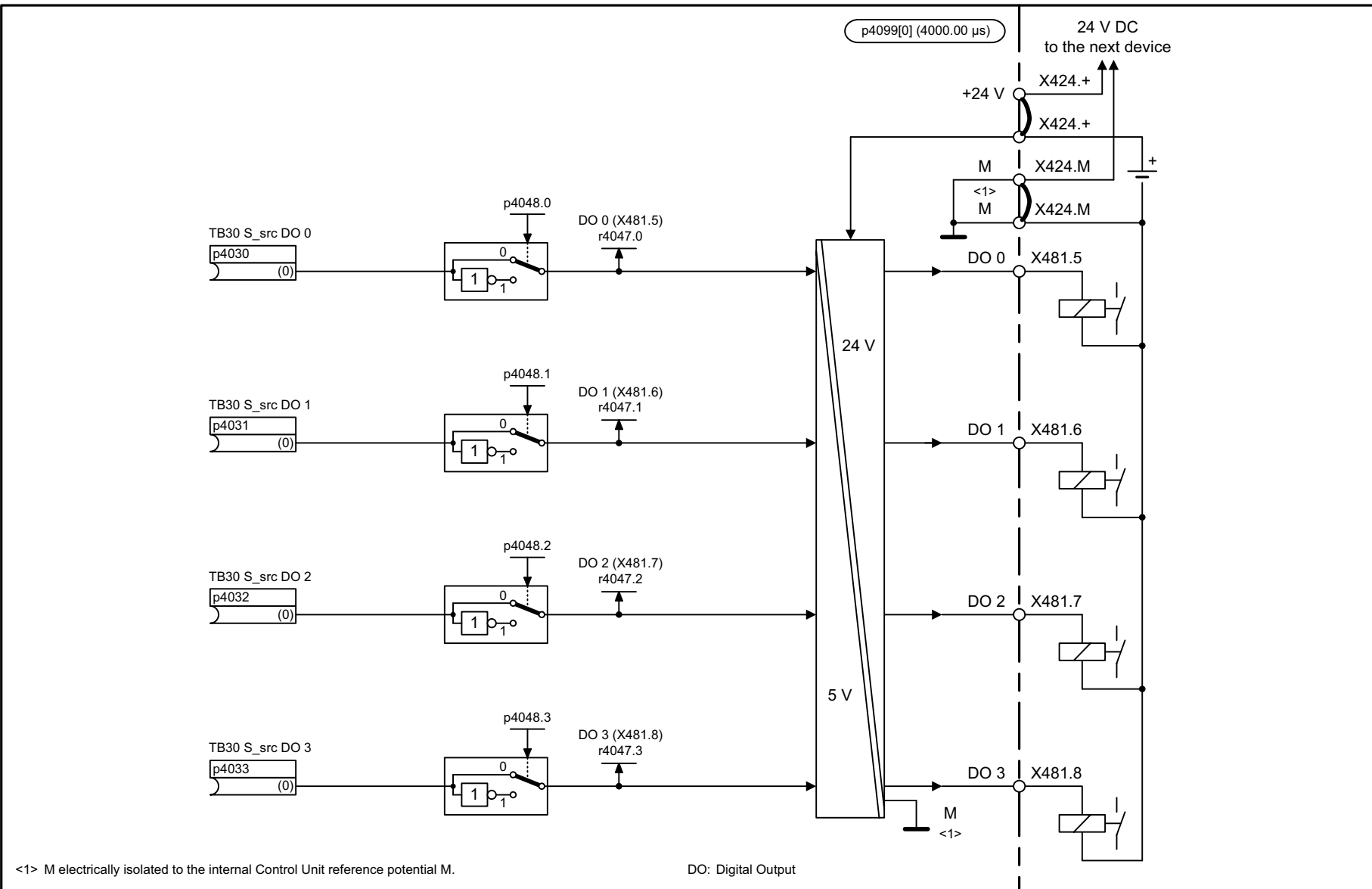
Fig. 3-349 9102 – Digital outputs, electrically isolated (DO 0 ... DO 3)
