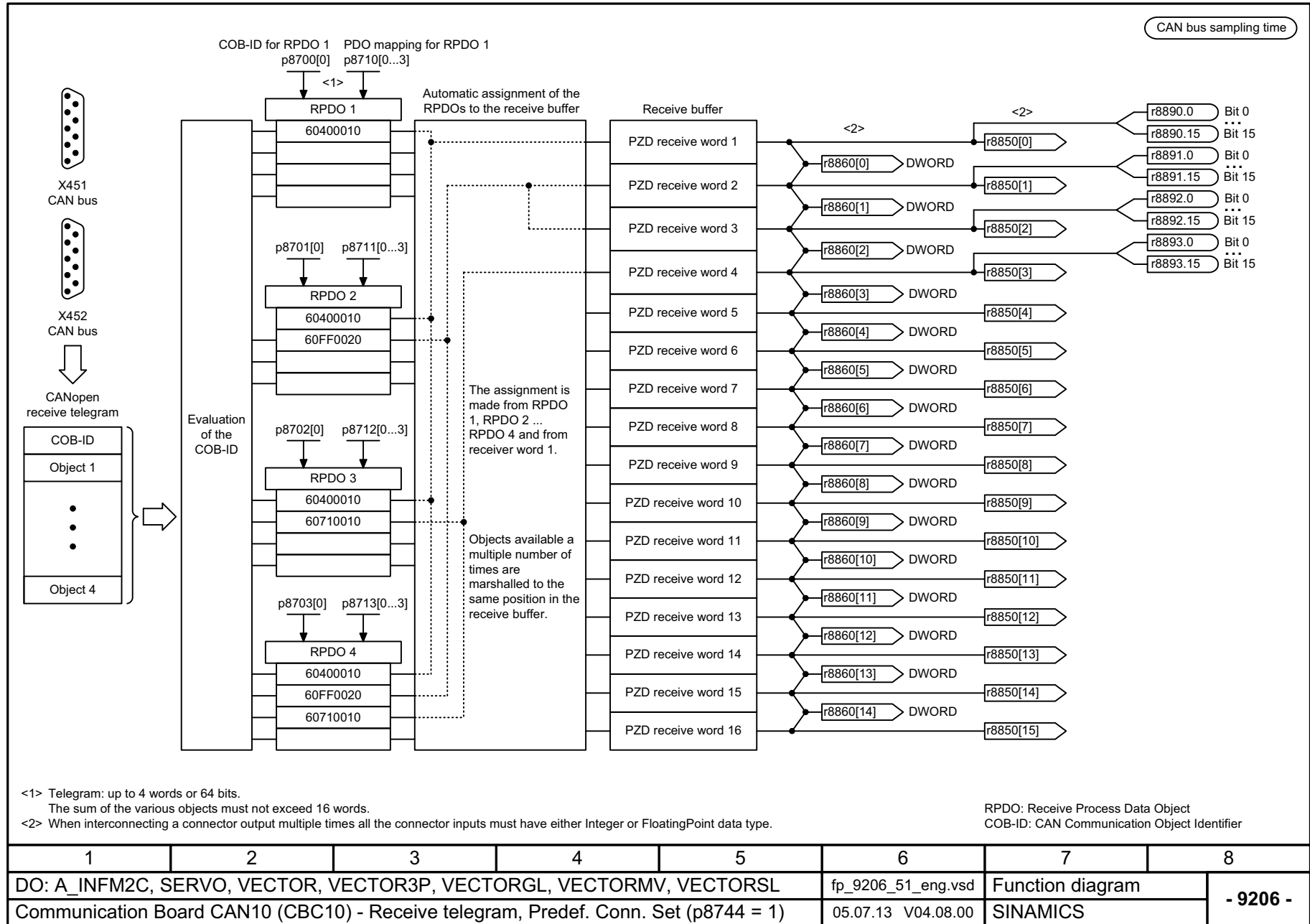
Fig. 3-353 9206 – Receive telegram, Predefined Connection Set (p8744 = 1)
