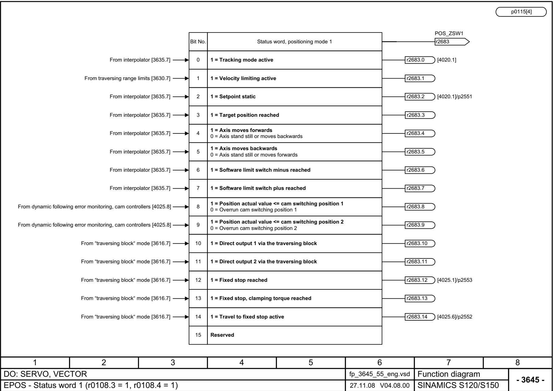
Fig. 3-175 3645 – Status word 1 (r0108.3 = 1, r0108.4 = 1)
