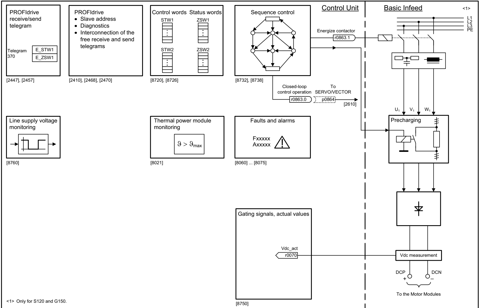
Fig. 3-317 8710 – Overview
