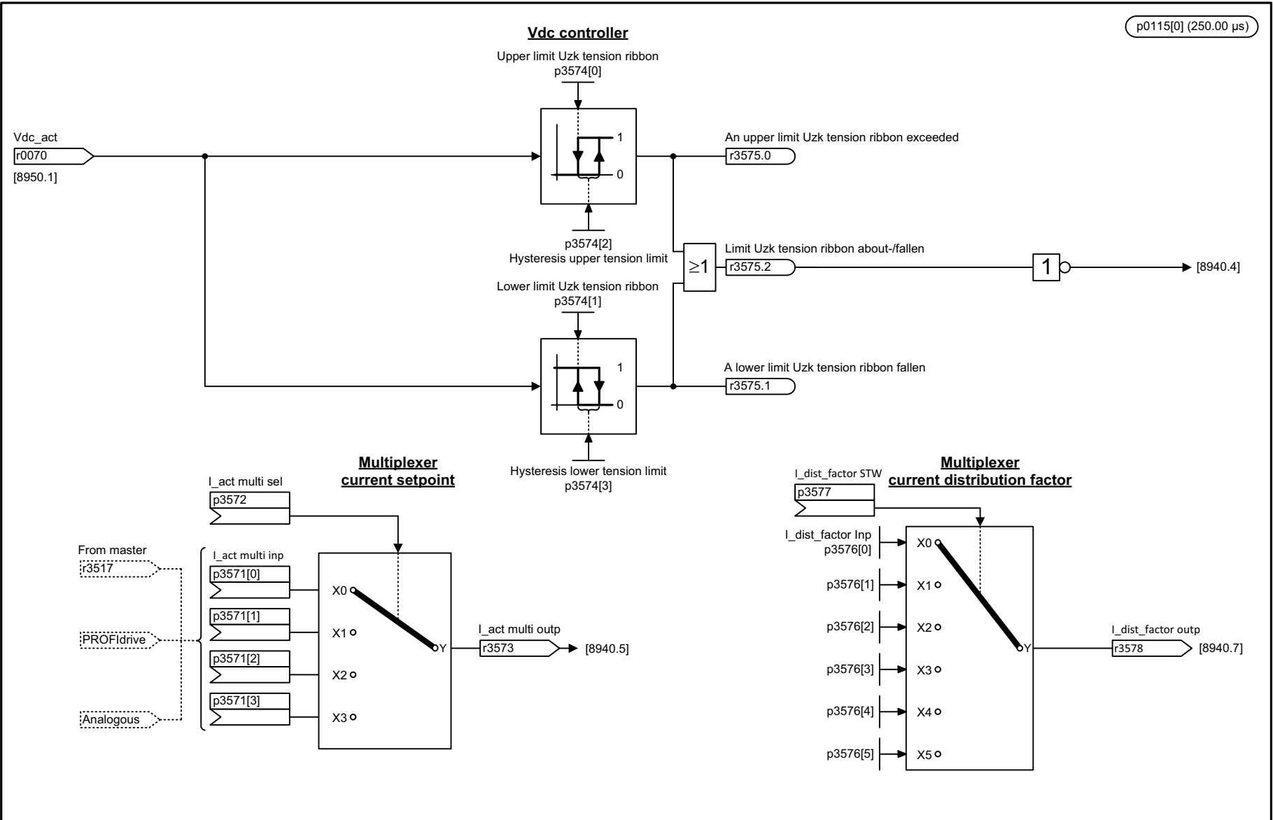
Fig. 3-342 8948 – Master/slave (r0108.19 = 1)
