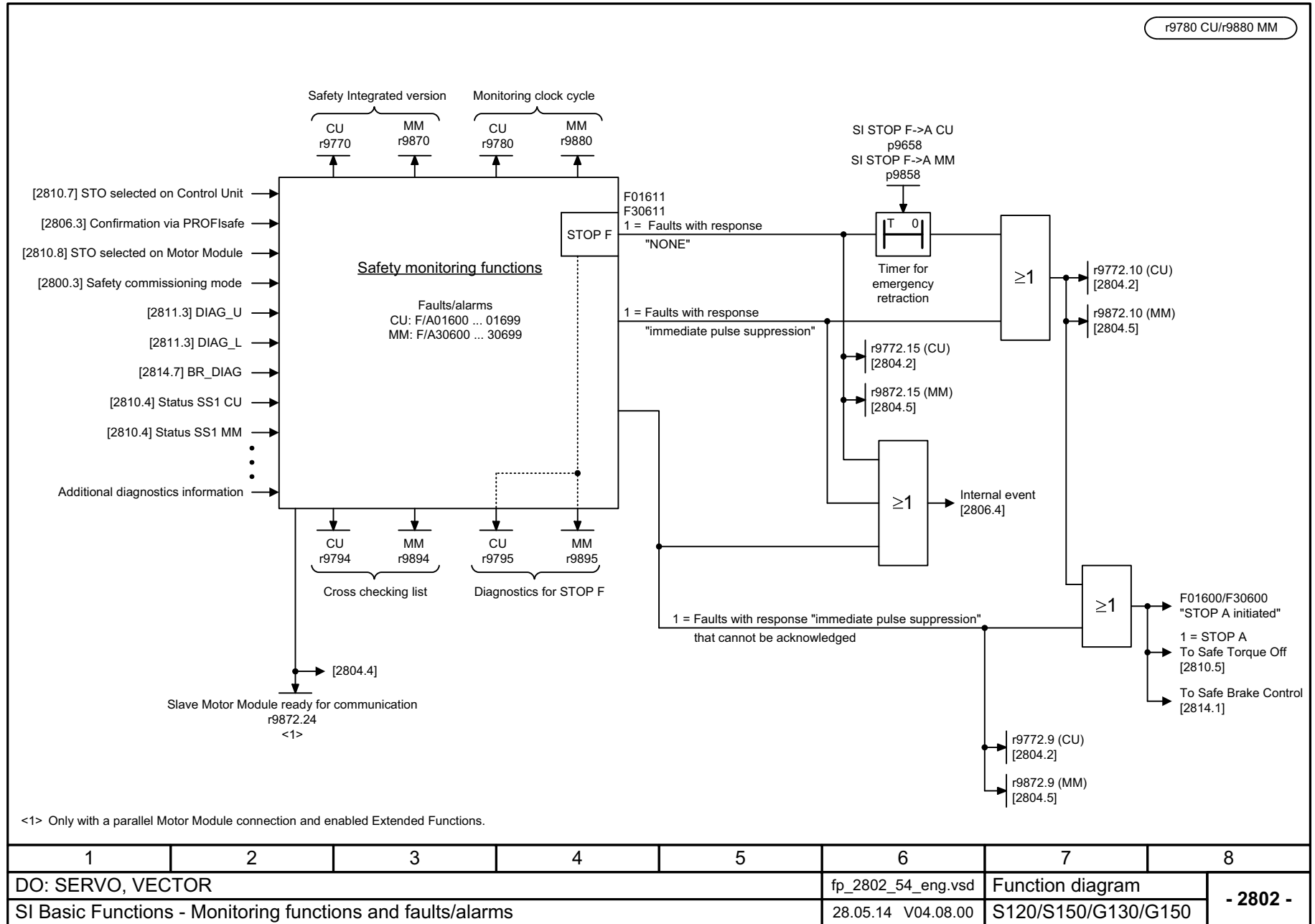
Fig. 3-112 2802 – Monitoring functions and faults/alarms
