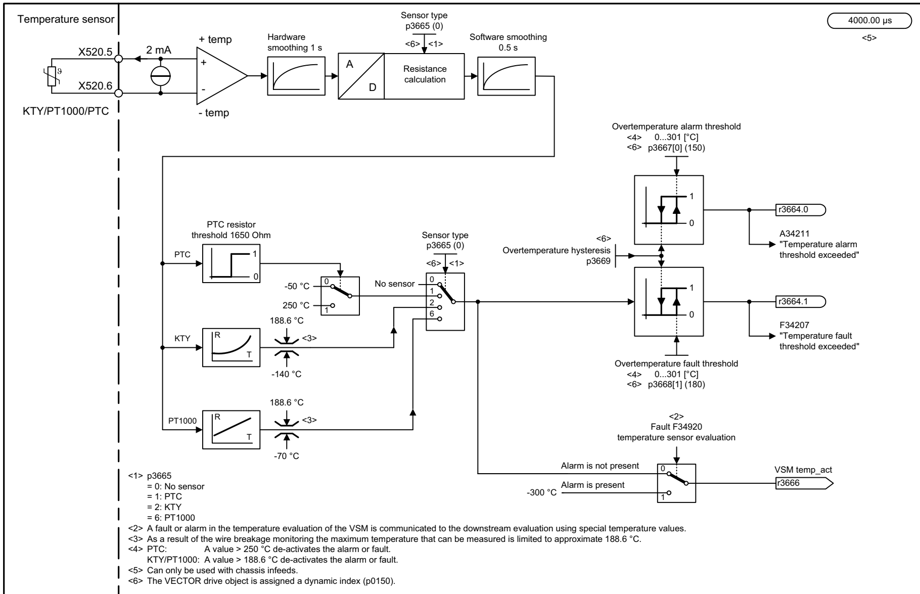
Fig. 3-397 9886 – Temperature evaluation
