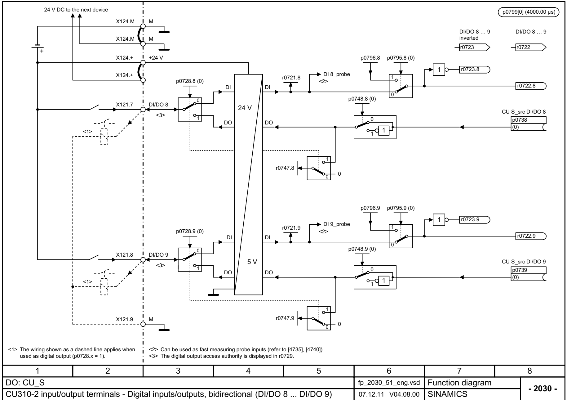
Fig. 3-8 2030 – Digital inputs/outputs, bidirectional (DI/DO 8 ... DI/DO 9)
