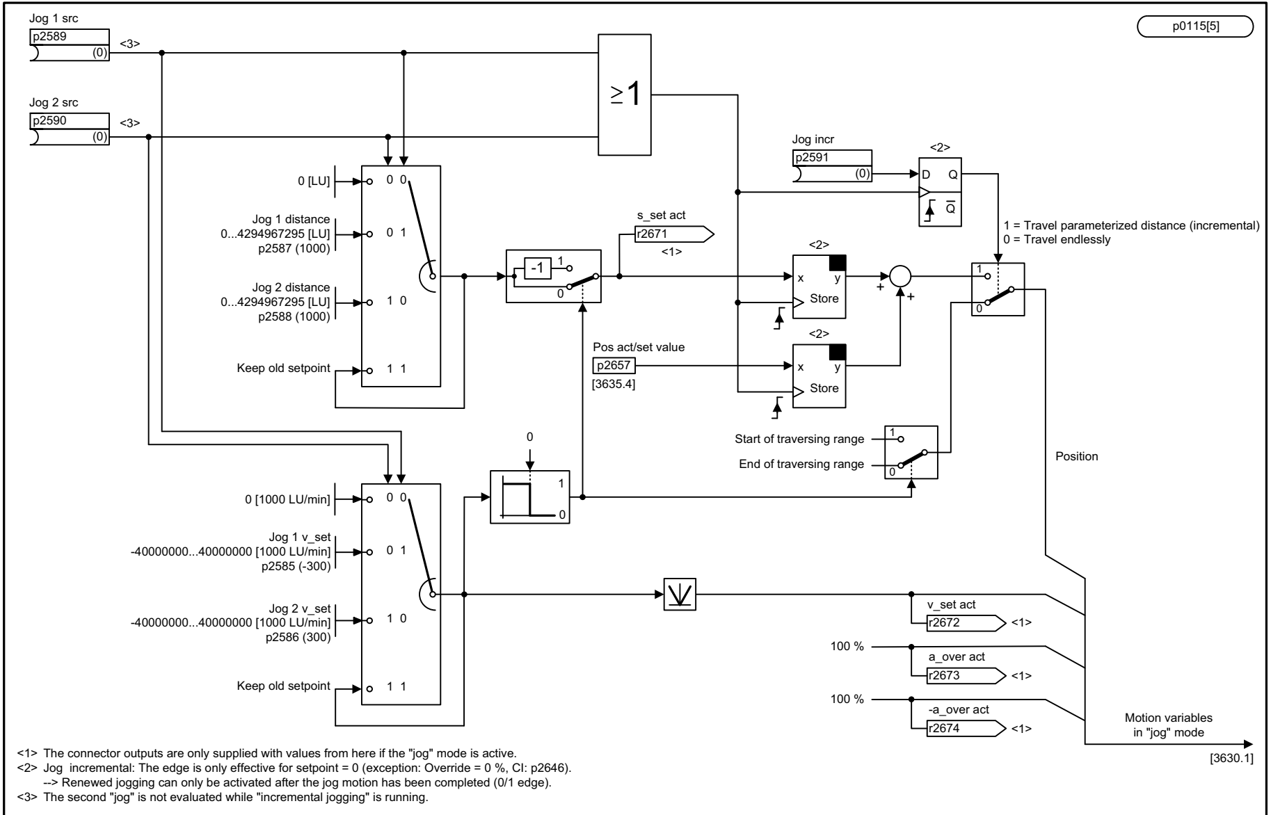
Fig. 3-163 36110 - Jog mode (r0108.4 = 1)
