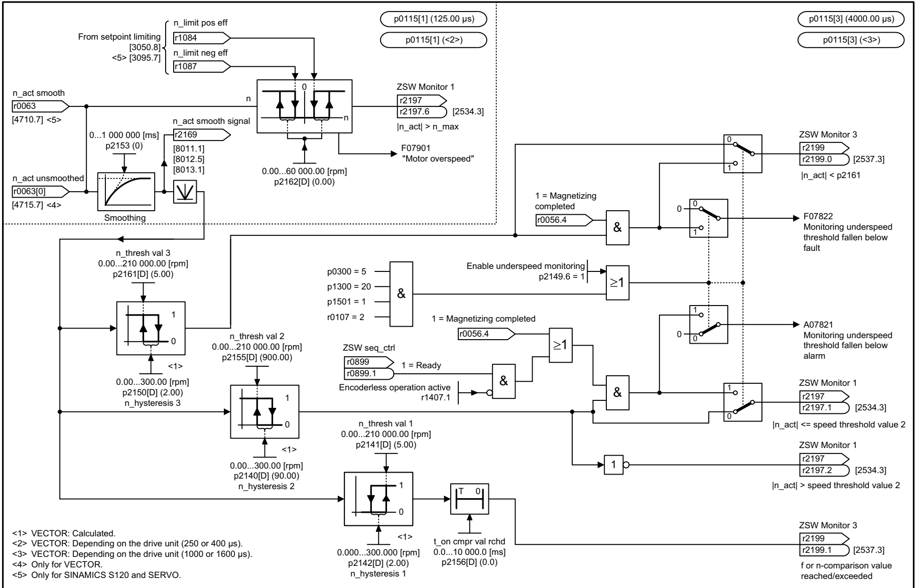
Fig. 3-293 8010 – Speed signals 1
