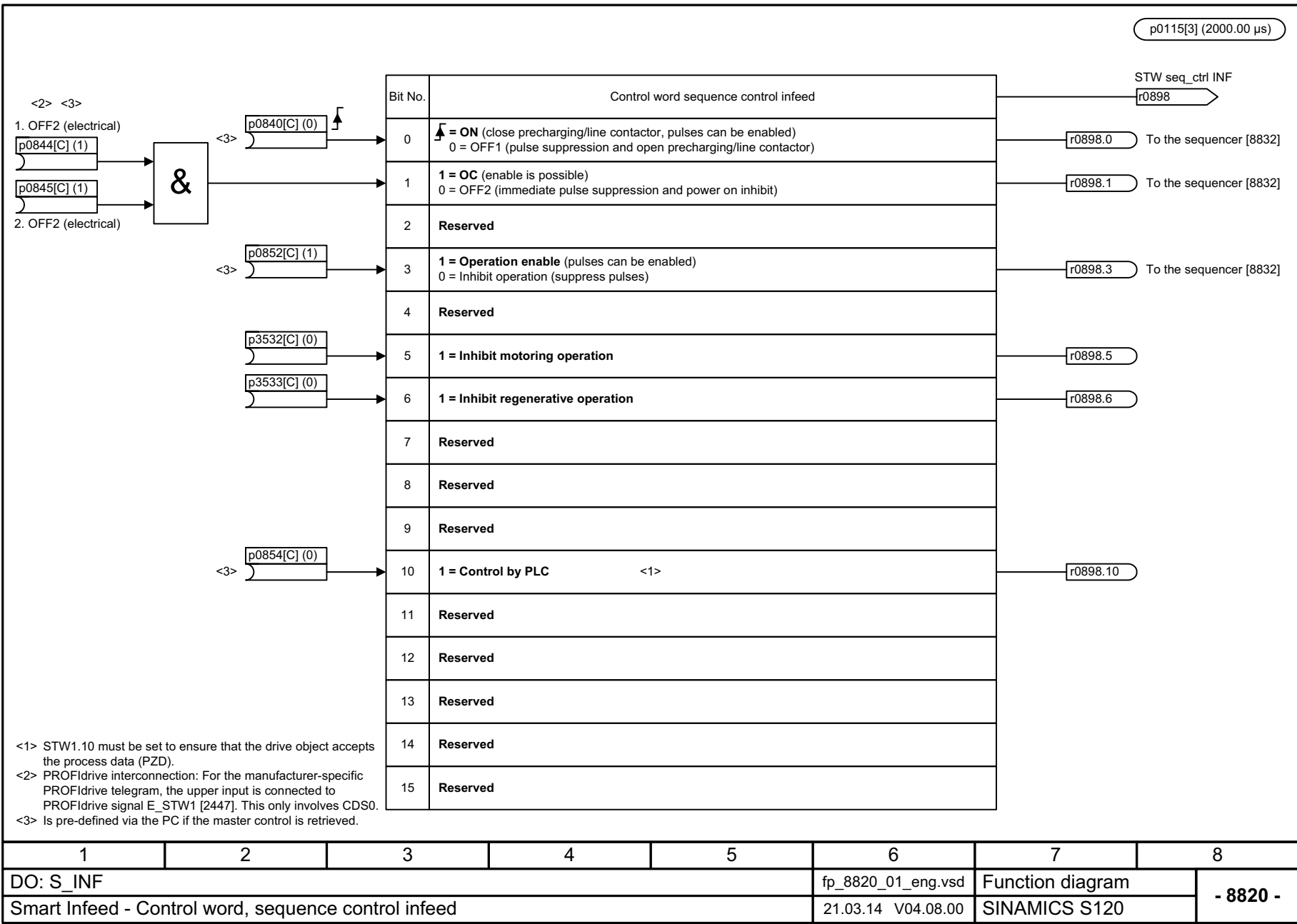
Fig. 3-325 8820 – Control word, sequence control infeed
