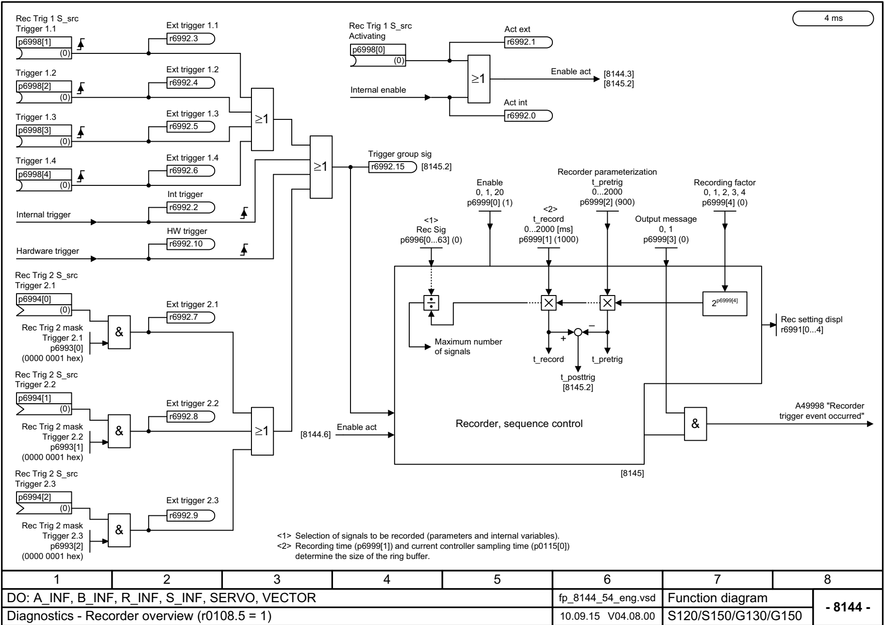
Fig. 3-310 8144 - Recorder overview (r0108.5 = 1)
