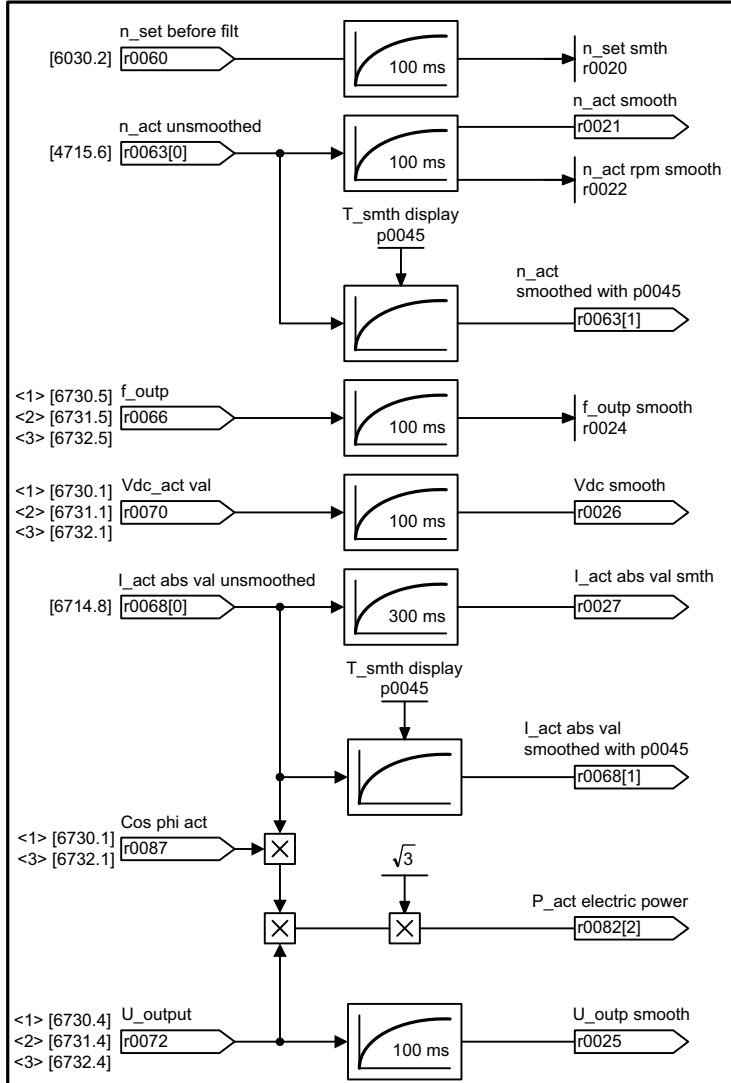
Fig. 3-261 6799 – Display signals
