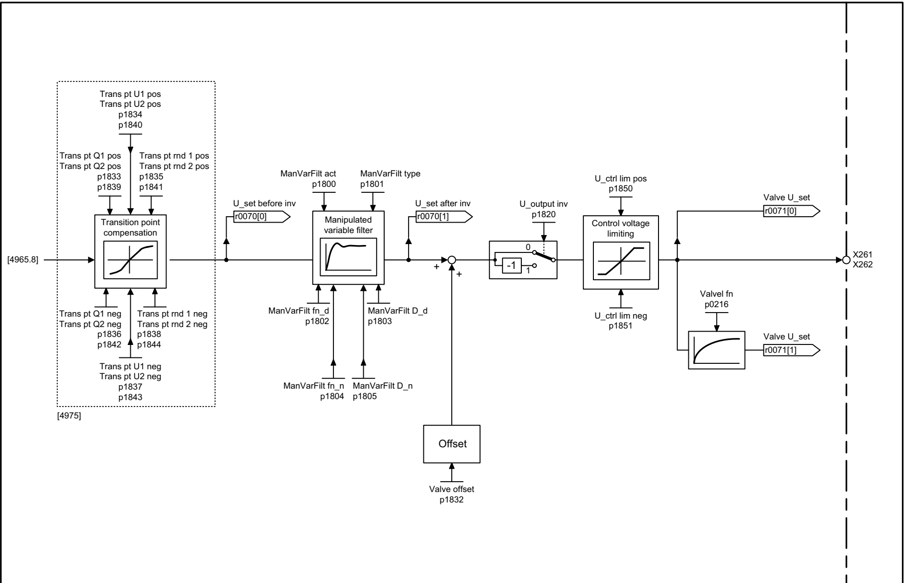
Fig. 3-194 4966 – Transition point compensation
