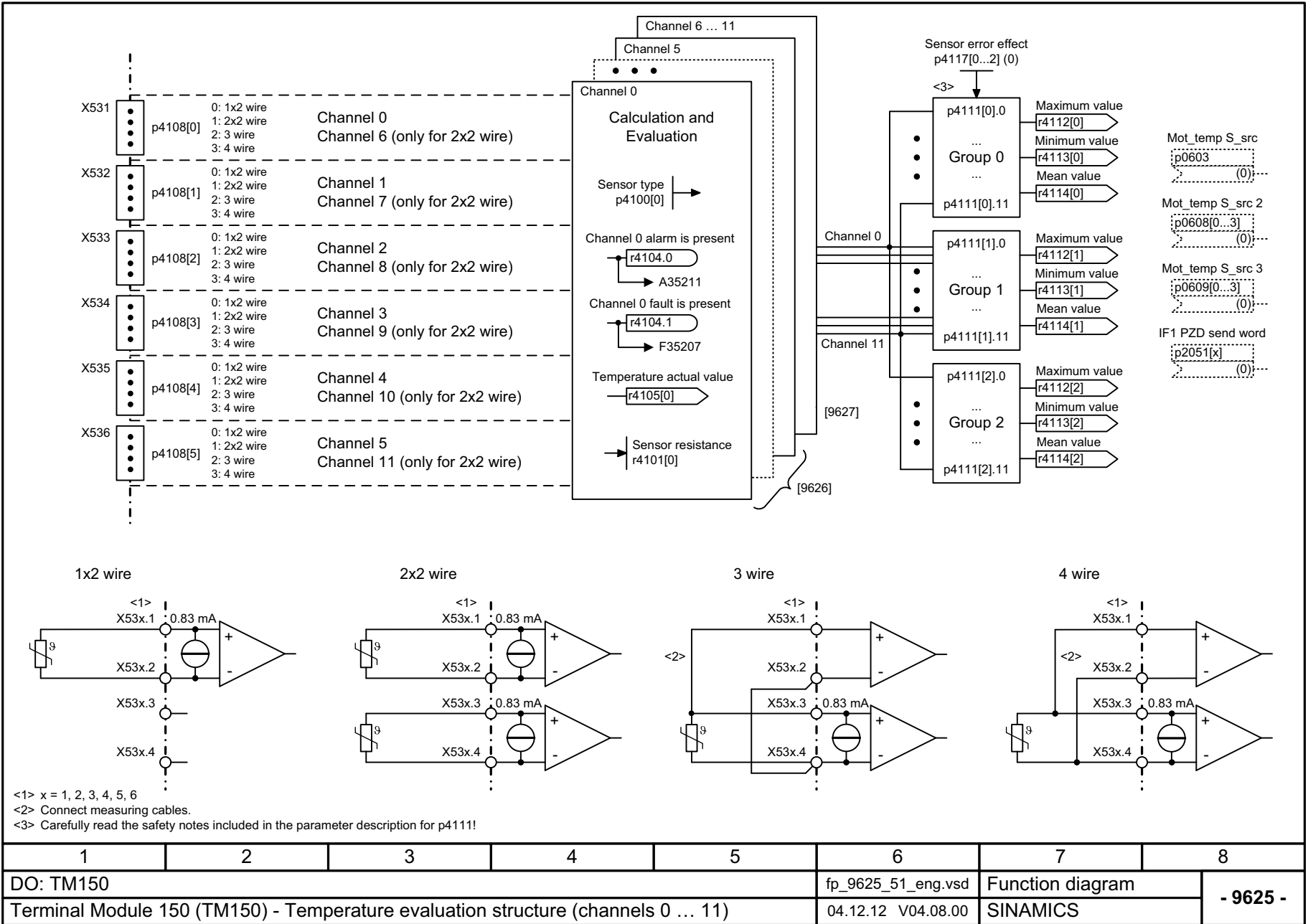
Fig. 3-376 9625 – Temperature evaluation structure (channels 0 ... 11)
