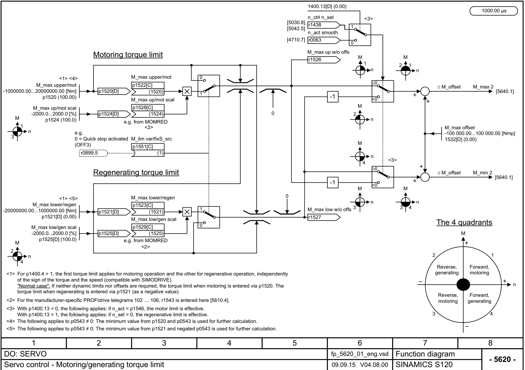
Fig. 3-217 5620 – Motoring/generating torque limit
