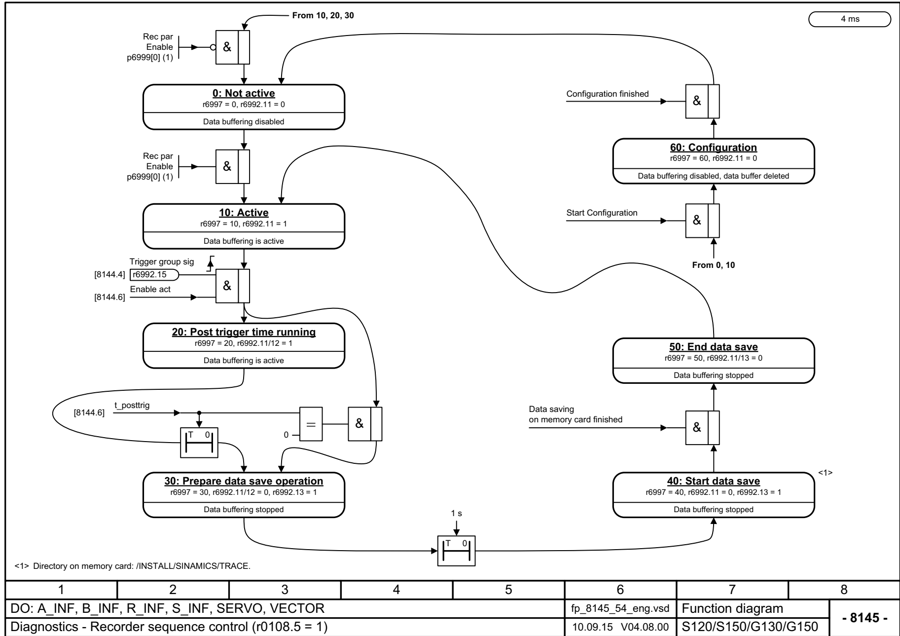
Fig. 3-311 8145 – Recorder sequence control (r0108.5 = 1)
