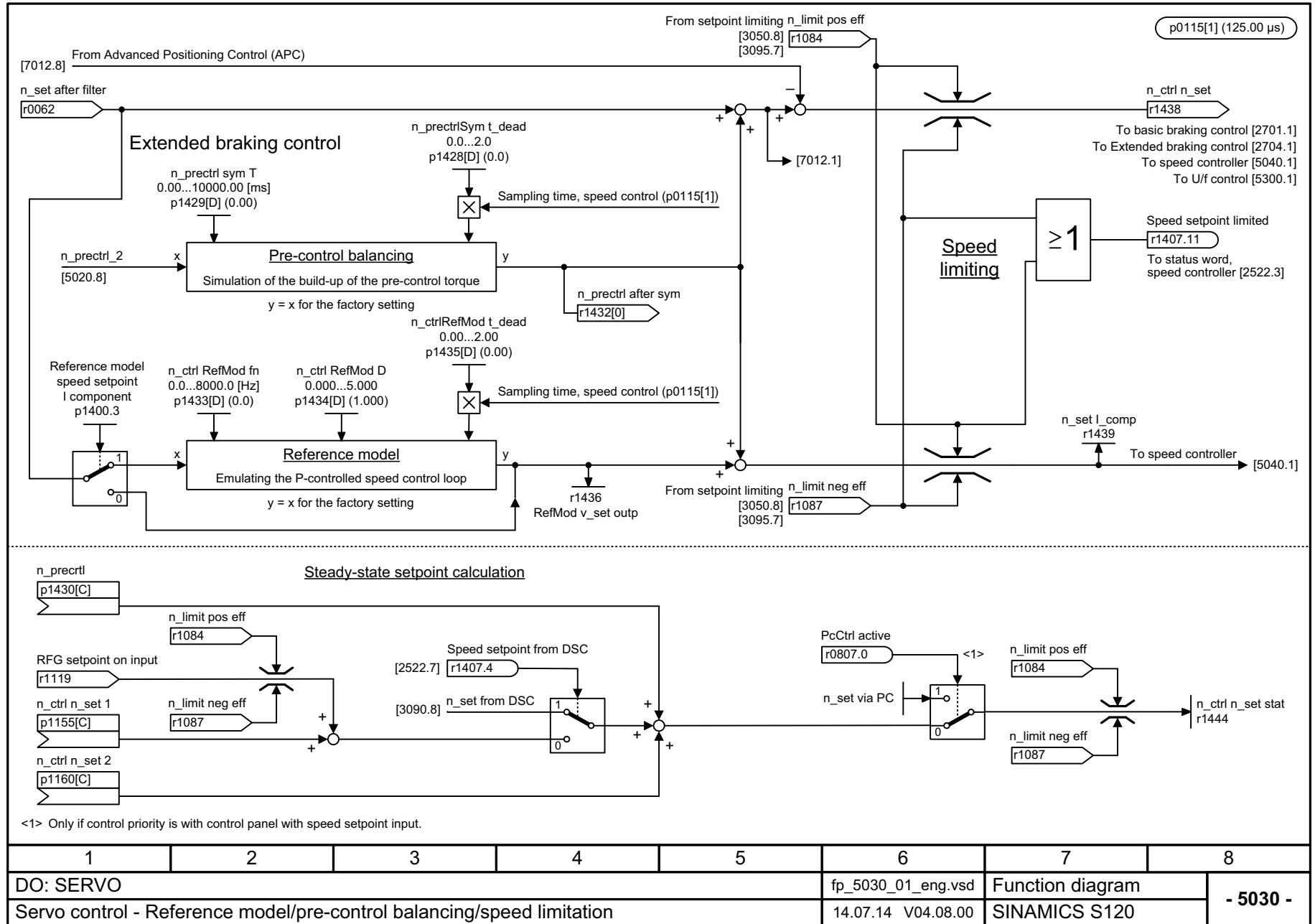
Fig. 3-204 5030 – Reference model/pre-control balancing/speed limitation
