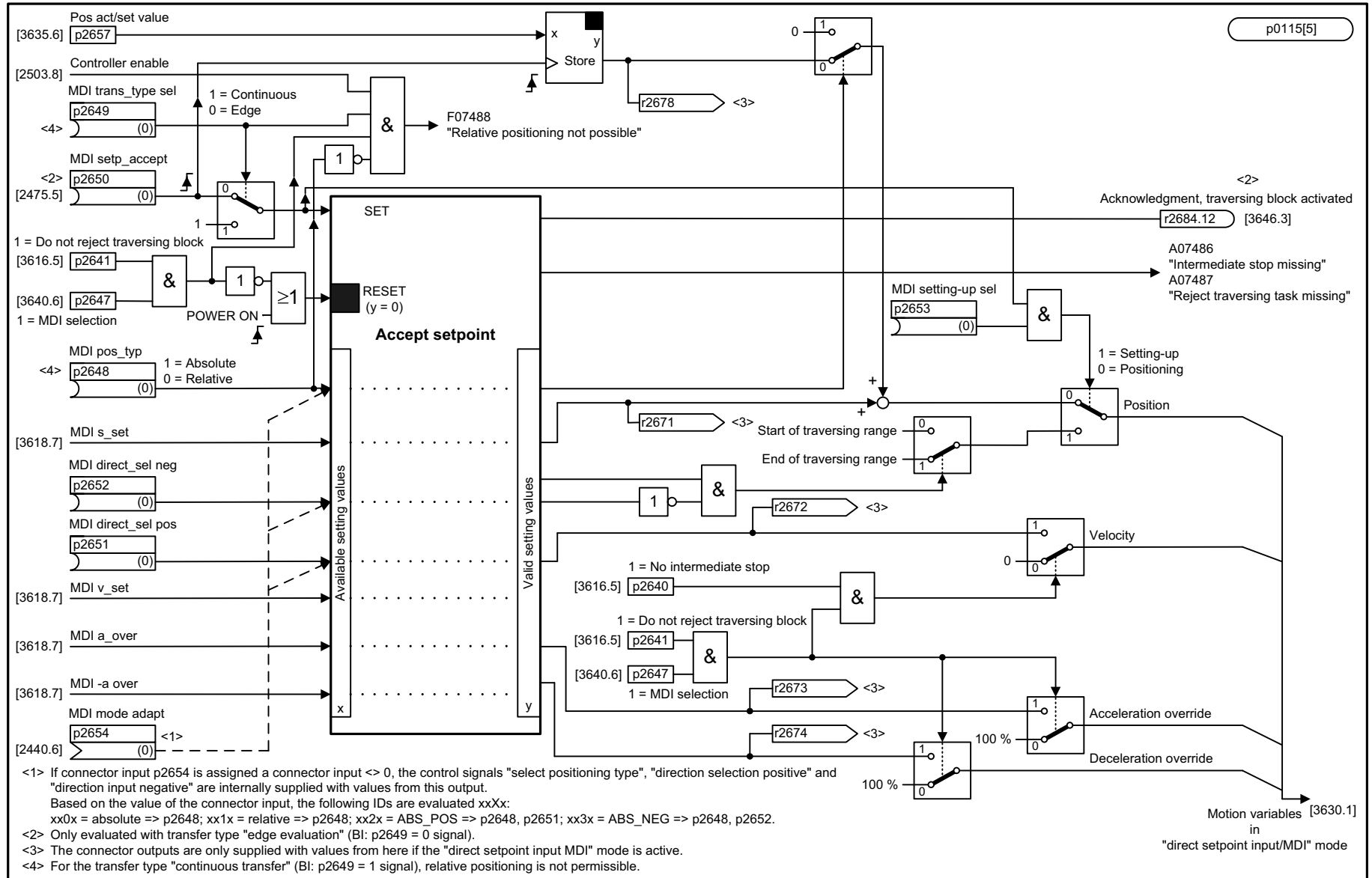
Fig. 3-170 3620 – Direct setpoint input/MDI mode (r0108.4 = 1)
