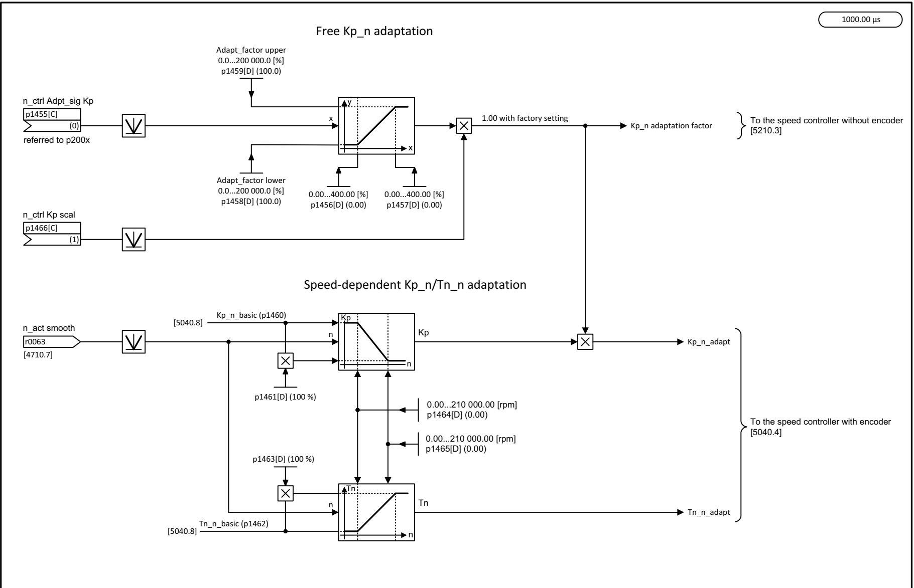
Fig. 3-209 5050 – Speed controller adaptation (Kp_n/Tn_n adaptation)
