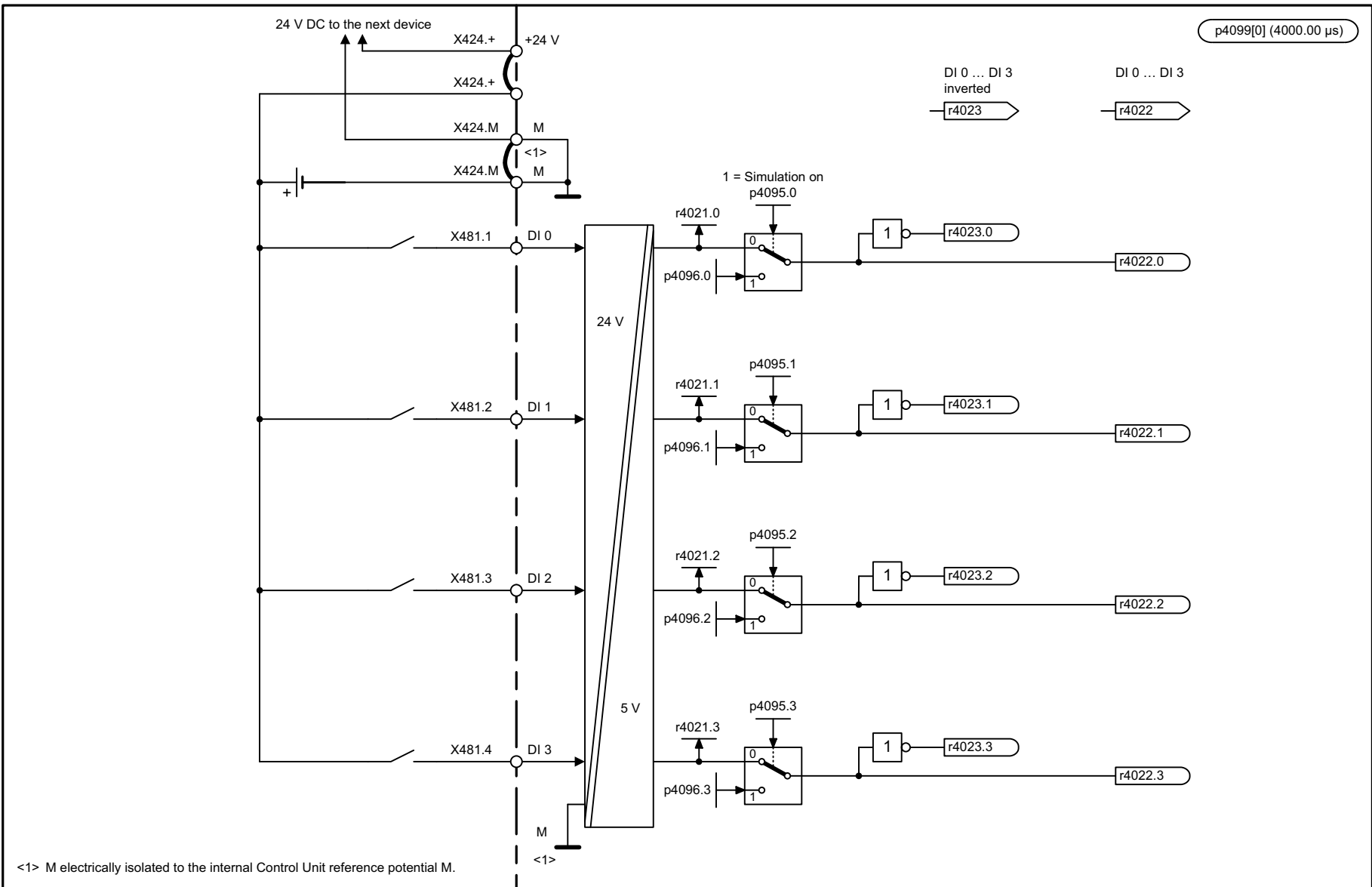
Fig. 3-348 9100 – Digital inputs, electrically isolated (DI 0 ... DI 3)
