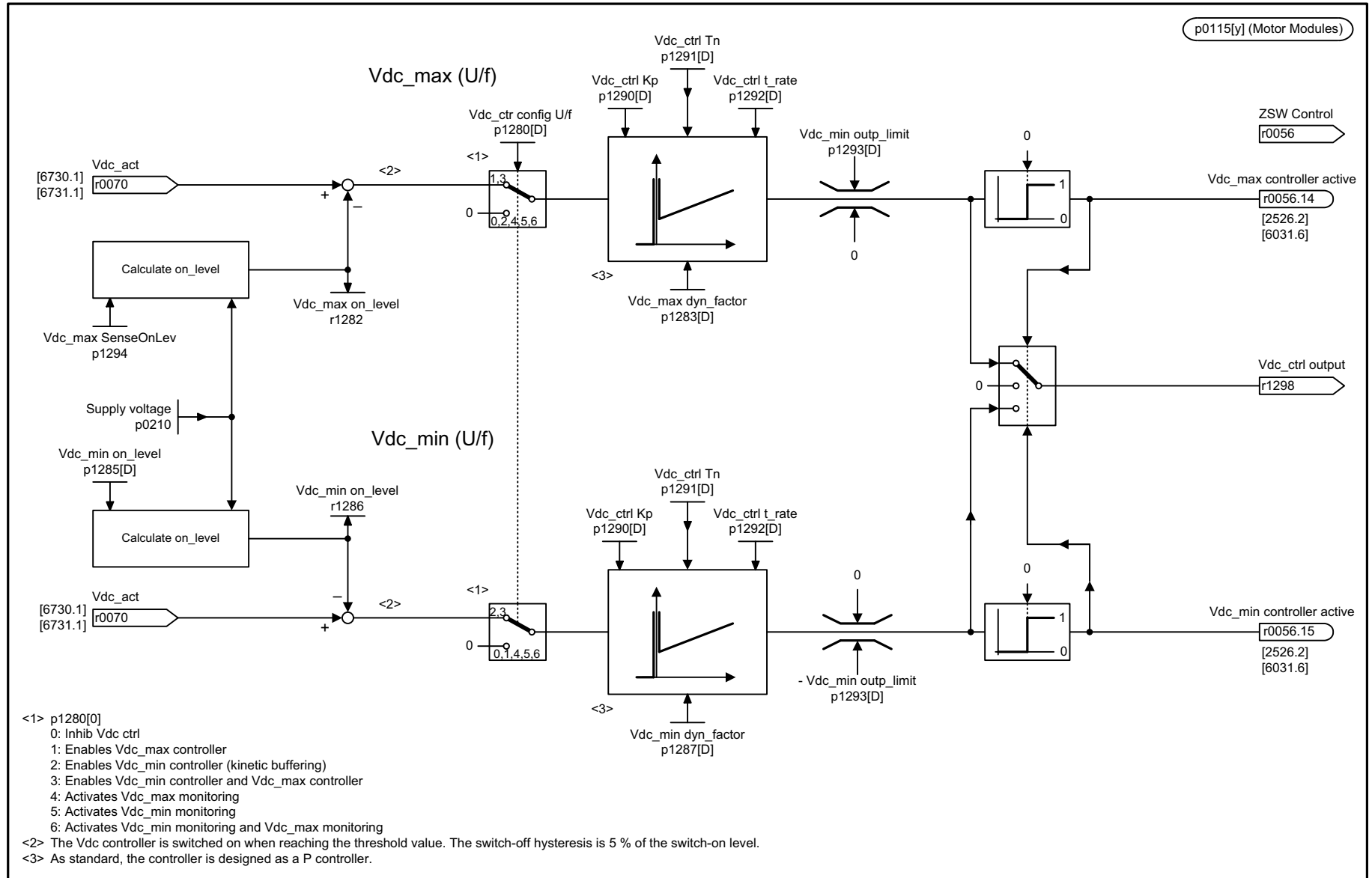
Fig. 3-238 6320 – Vdc_max controller and Vdc_min controller (U/f)
