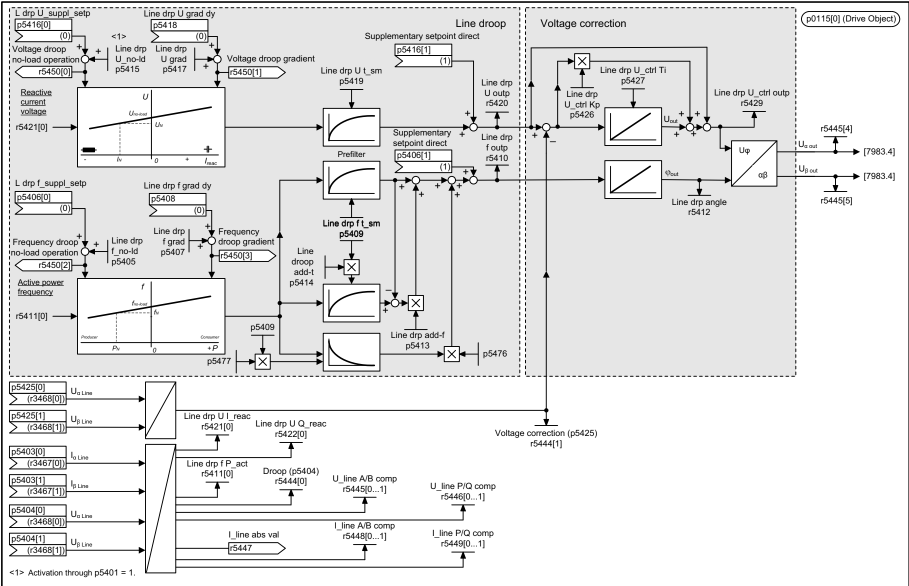
Fig. 3-276 7982 – Line droop, voltage correction control
