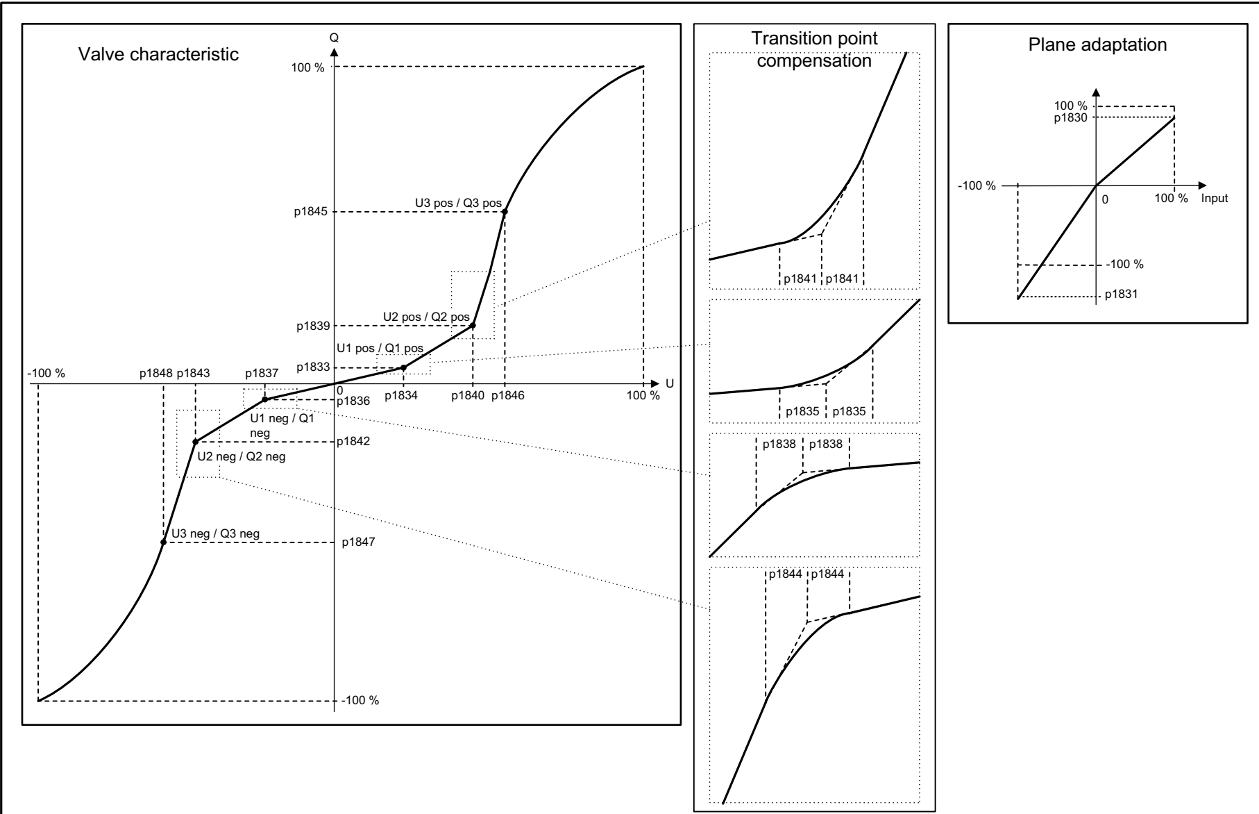
Fig. 3-196 4975 – Valve characteristic, plane adaptation
