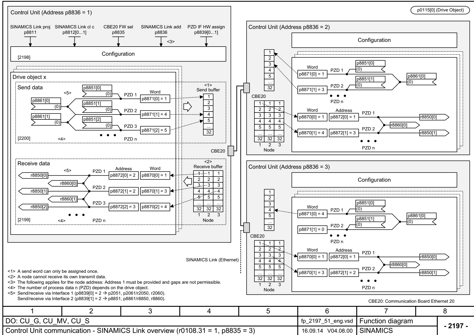
Fig. 3-27 2197 – SINAMICS Link overview (r0108.31 = 1, p8835 = 3)
