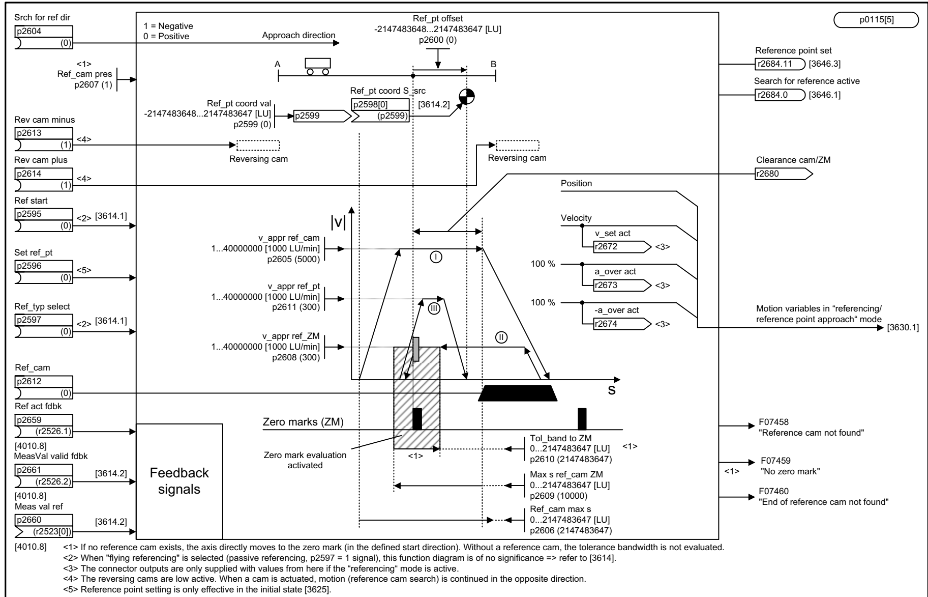
Fig. 3-164 3612 – Referencing/reference point approach mode (r0108.4 = 1) (p2597 = 0 signal)
