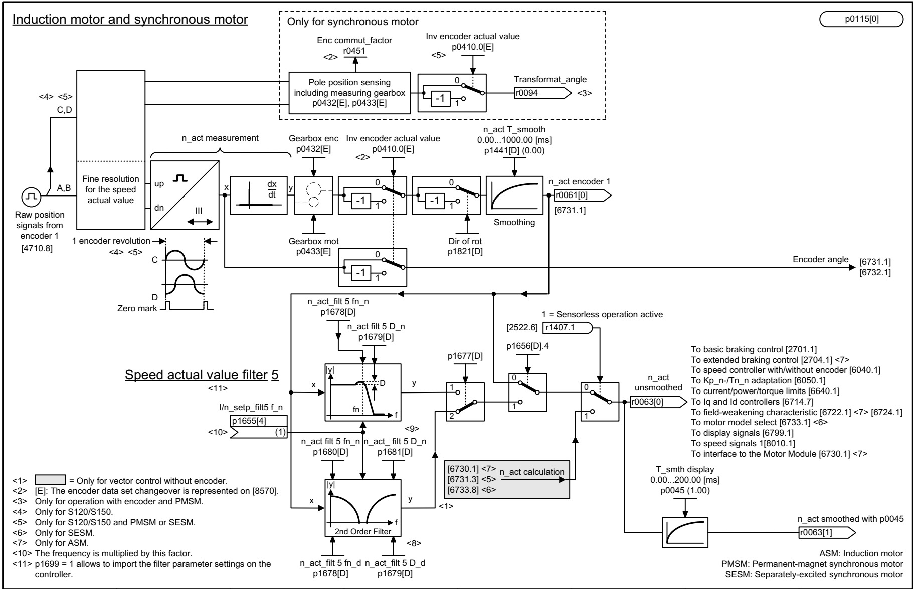
Fig. 3-187 4715 – Speed actual value and pole position sensing, encoder 1, n_act_filter 5
