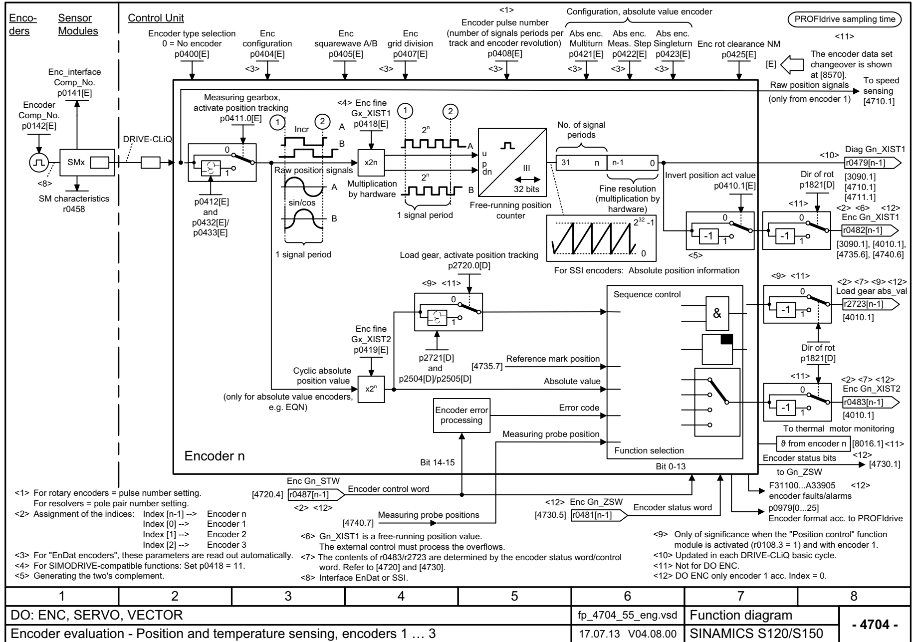
Fig. 3-184 4/704 – Position and temperature sensing, encoders 1 ... 3
