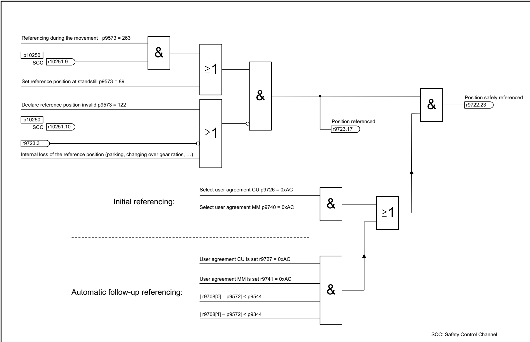
Fig. 3-121 2821 – Safe referencing
