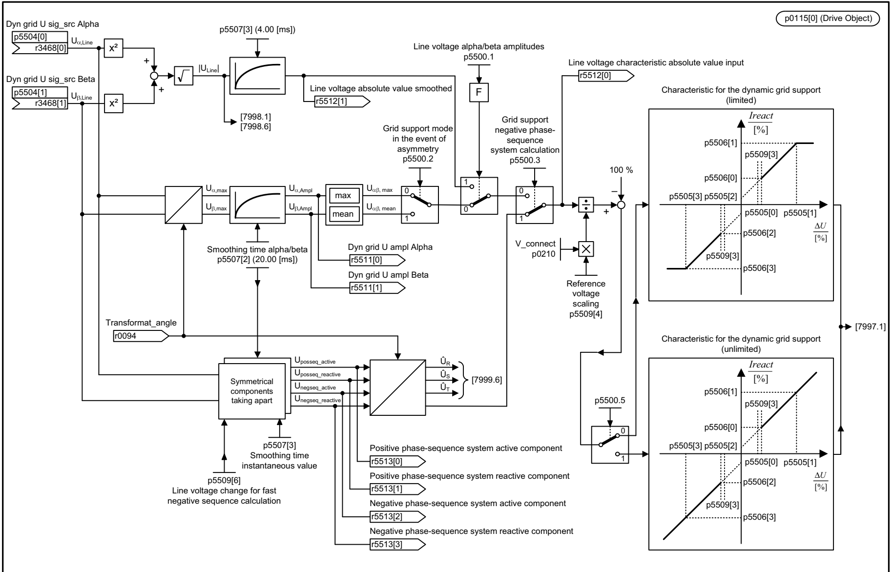
Fig. 3-288 7996 – Characteristic
