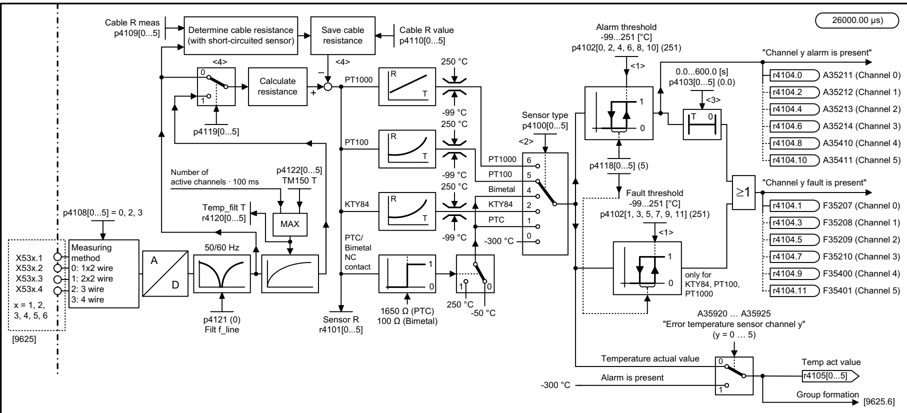
Fig. 3-377 9626 – Temperature evaluation 1x2, 3, 4 wire (channels 0 ... 5)
