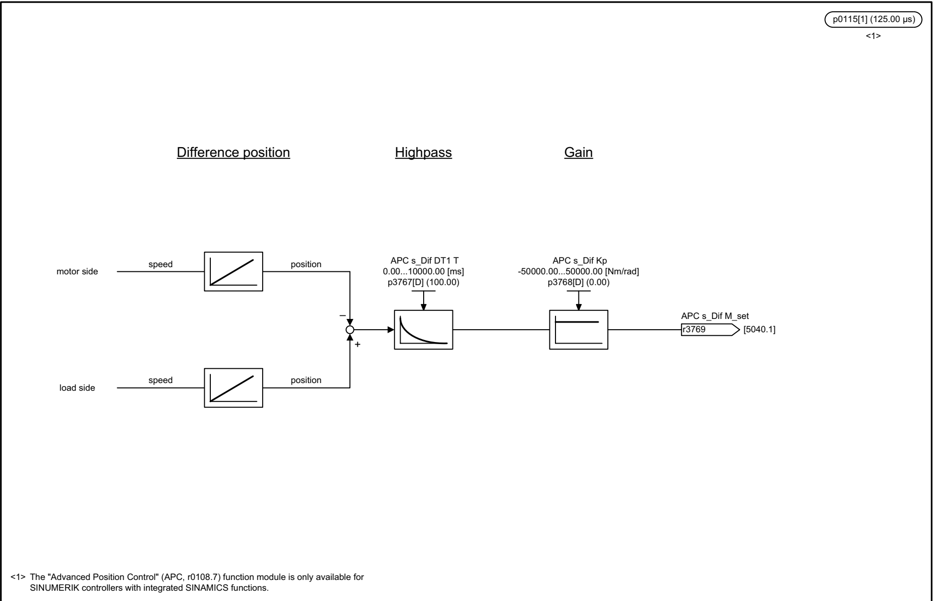
Fig. 3-265 7013 – APC differential position gain (APC, r0108.7 = 1)
