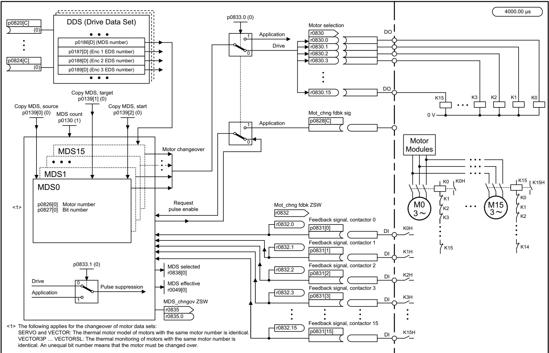
Fig. 3-315 8575 – Motor Data Sets (MDS)
