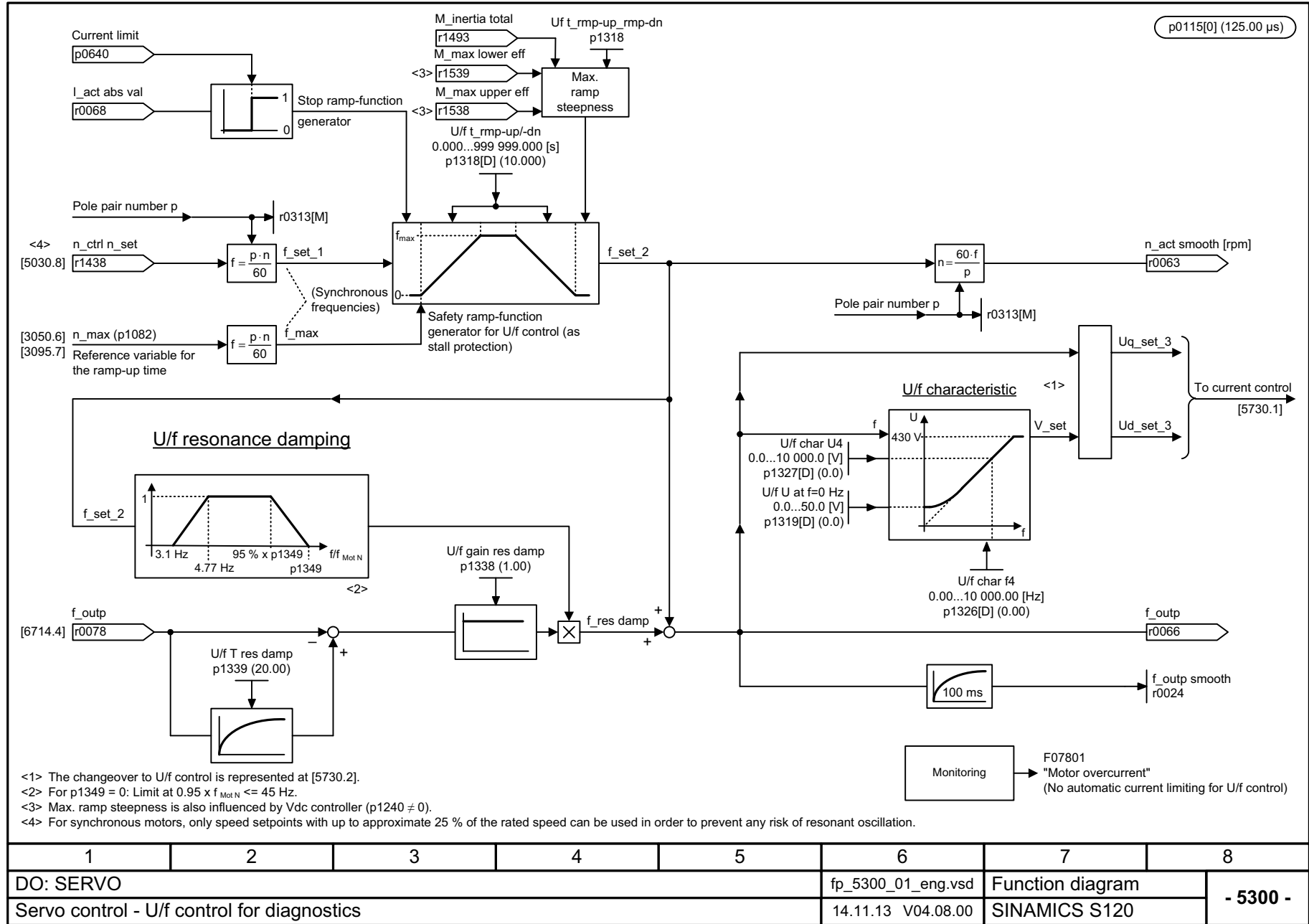
Fig. 3-212 5300 – U/f control for diagnostics
