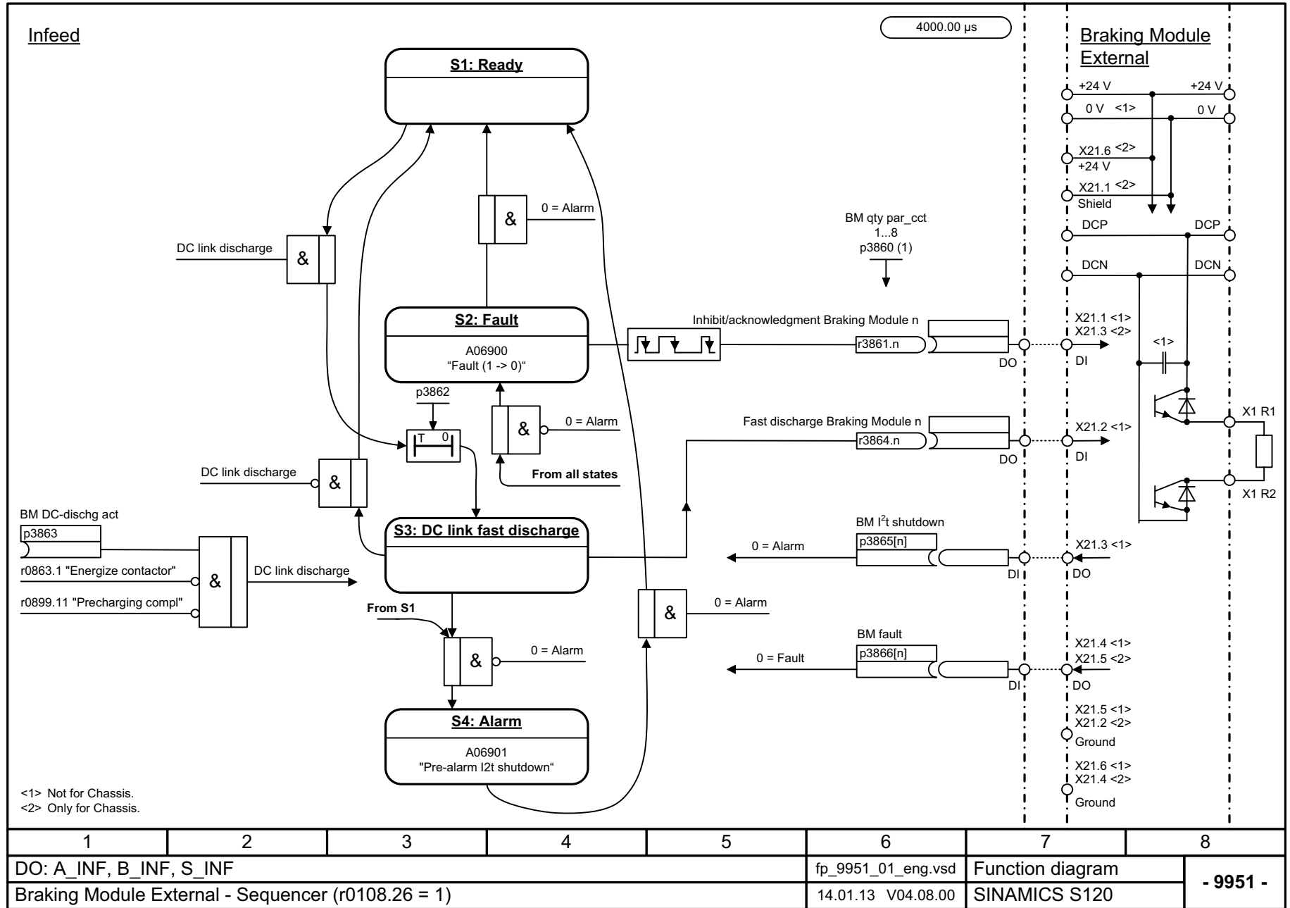
Fig. 3-399 9951 – Sequencer (r0108.26 = 1)
