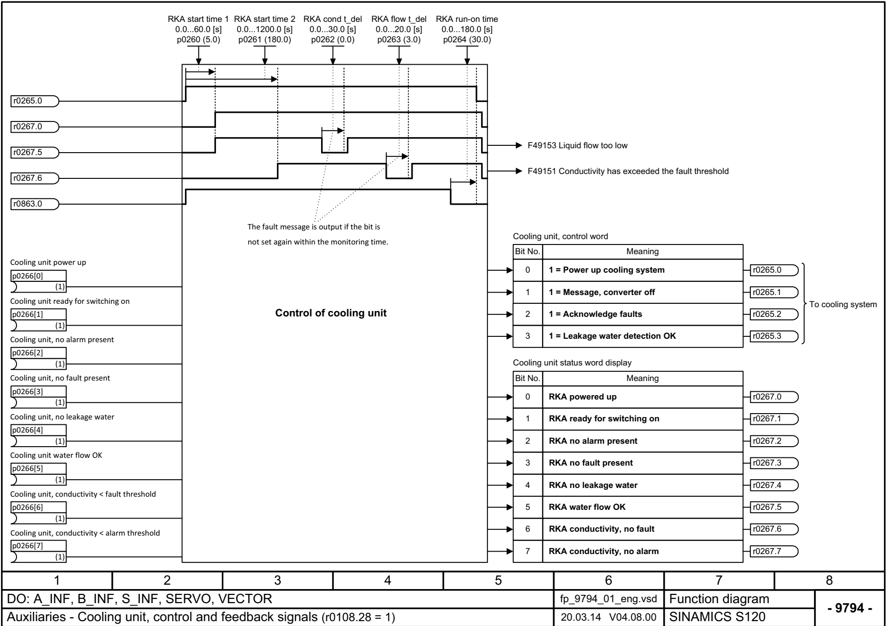
Fig. 3-393 9794 – Cooling unit, control and feedback signals (r0108.28 = 1)
