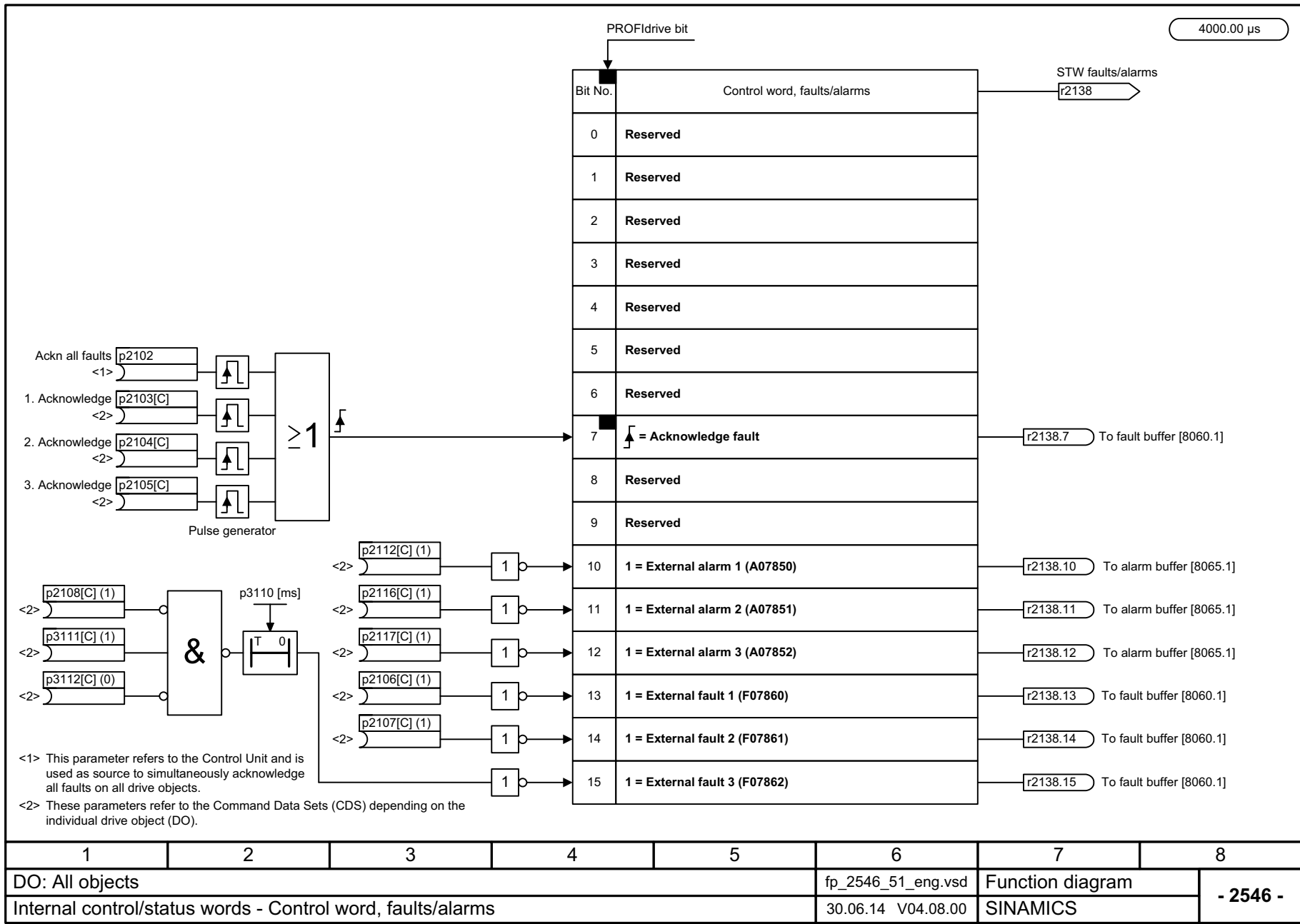
Fig. 3-103 2546 – Control word, faults/alarms
