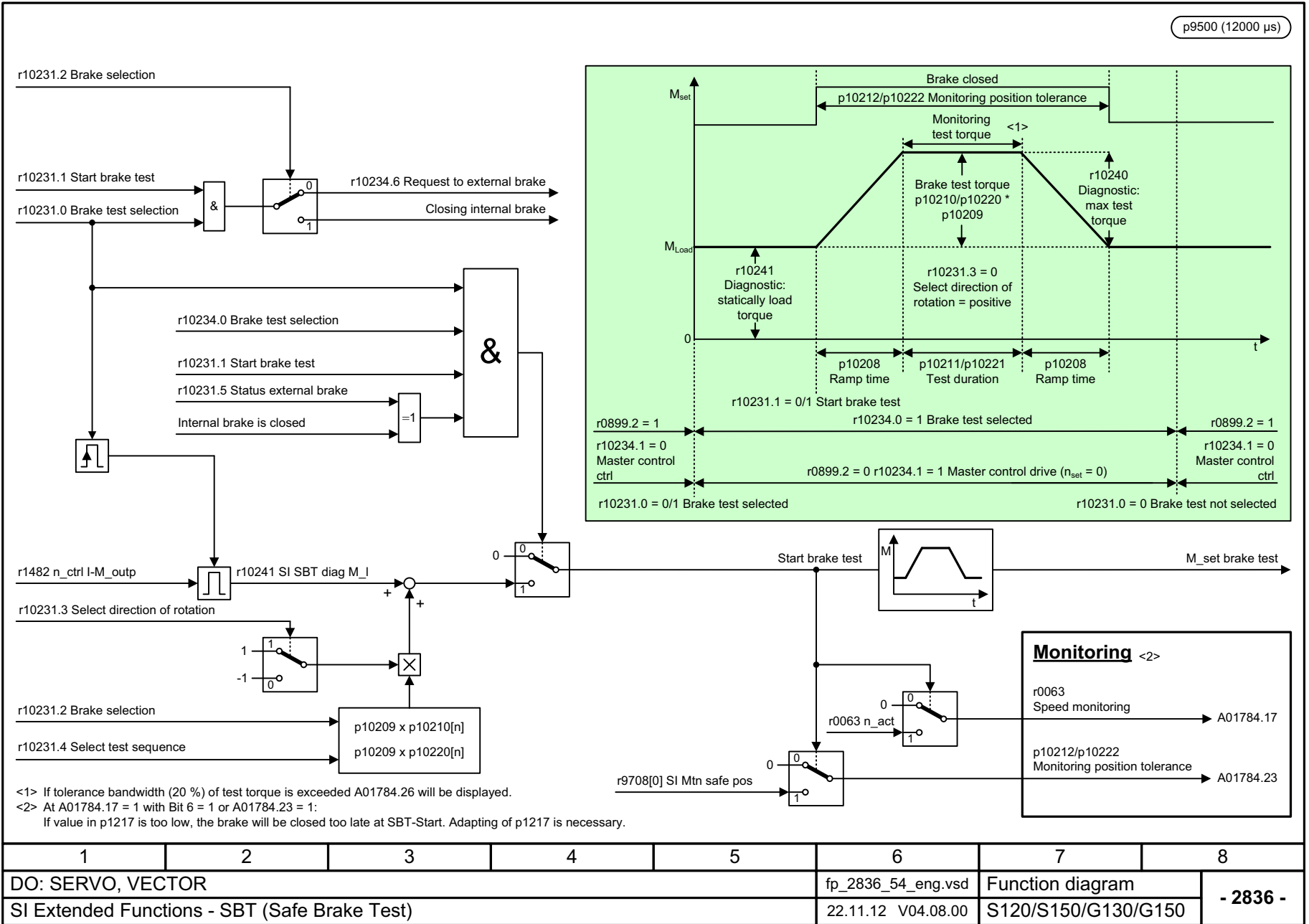
Fig. 3-126 2836 – SBT (Safe Brake Test)
