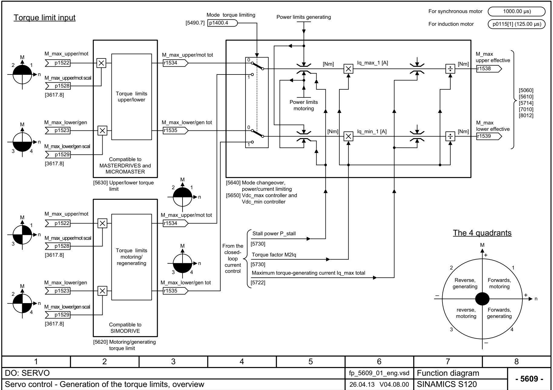
Fig. 3-215 5609 – Generation of the torque limits, overview
