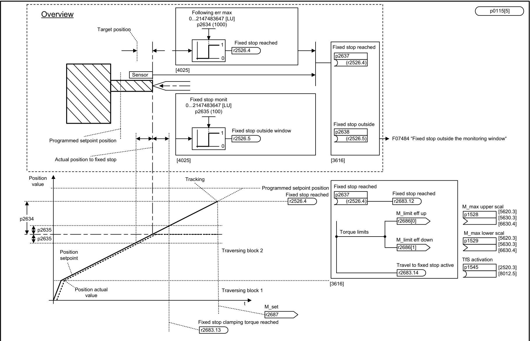
Fig. 3-168 3617 – Travel to fixed stop (r0108.4 = 1)
