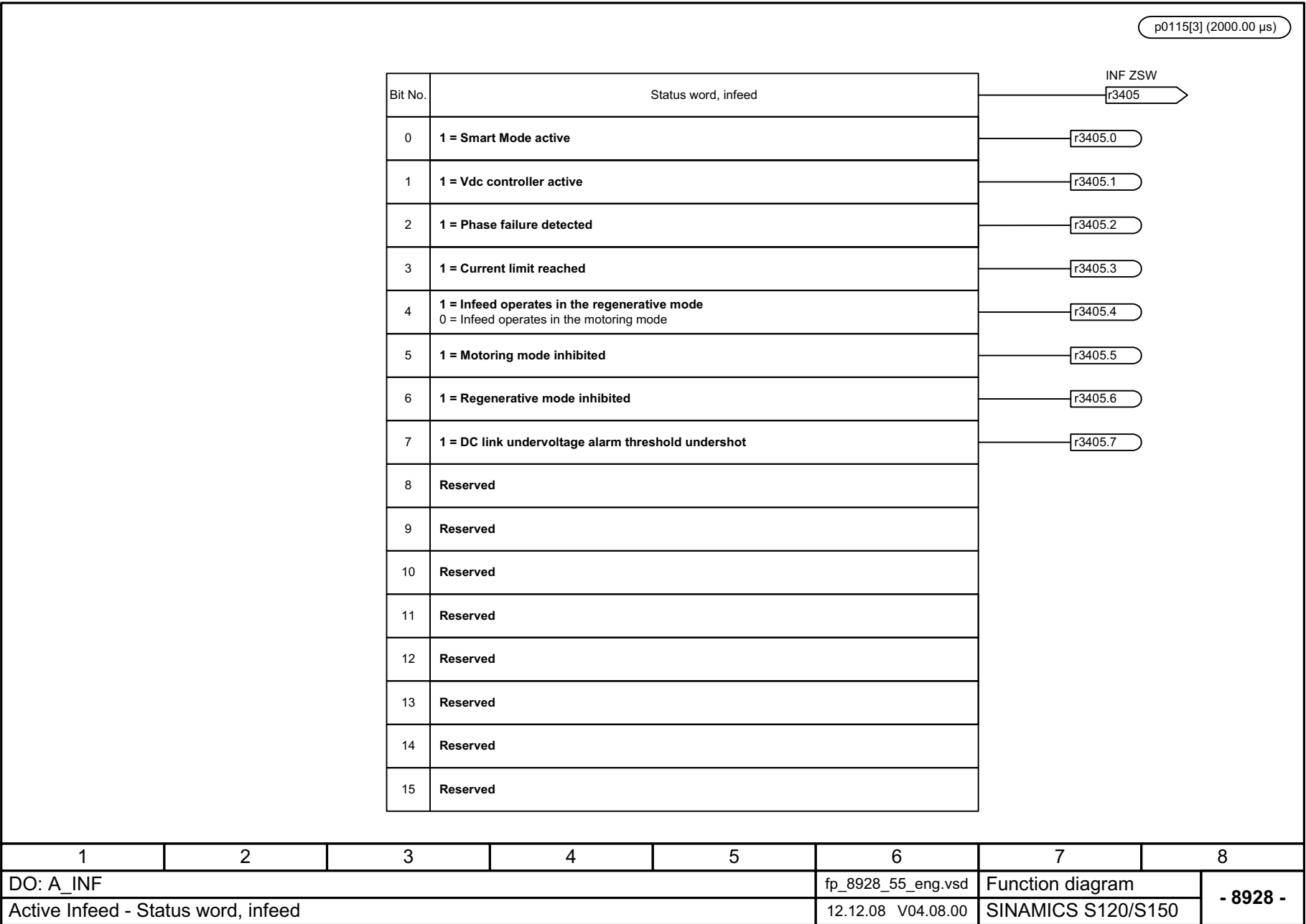
Fig. 3-336 8928 – Status word, infeed
