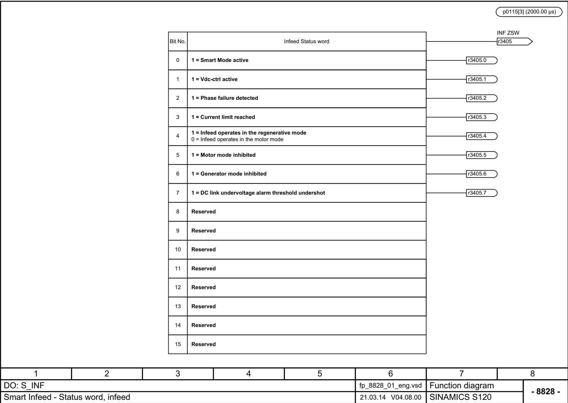
Fig. 3-327 8828 – Status word, infeed
