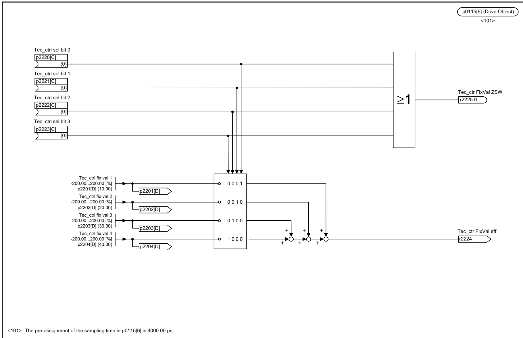
Fig. 3-272 7951 – Fixed values, direct selection (r0108.16 = 1 and p2216 = 1)
