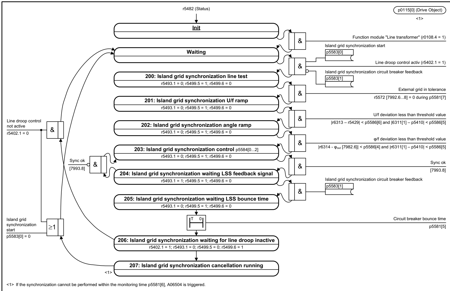
Fig. 3-282 7989 – Island grid synchronization, sequence control
