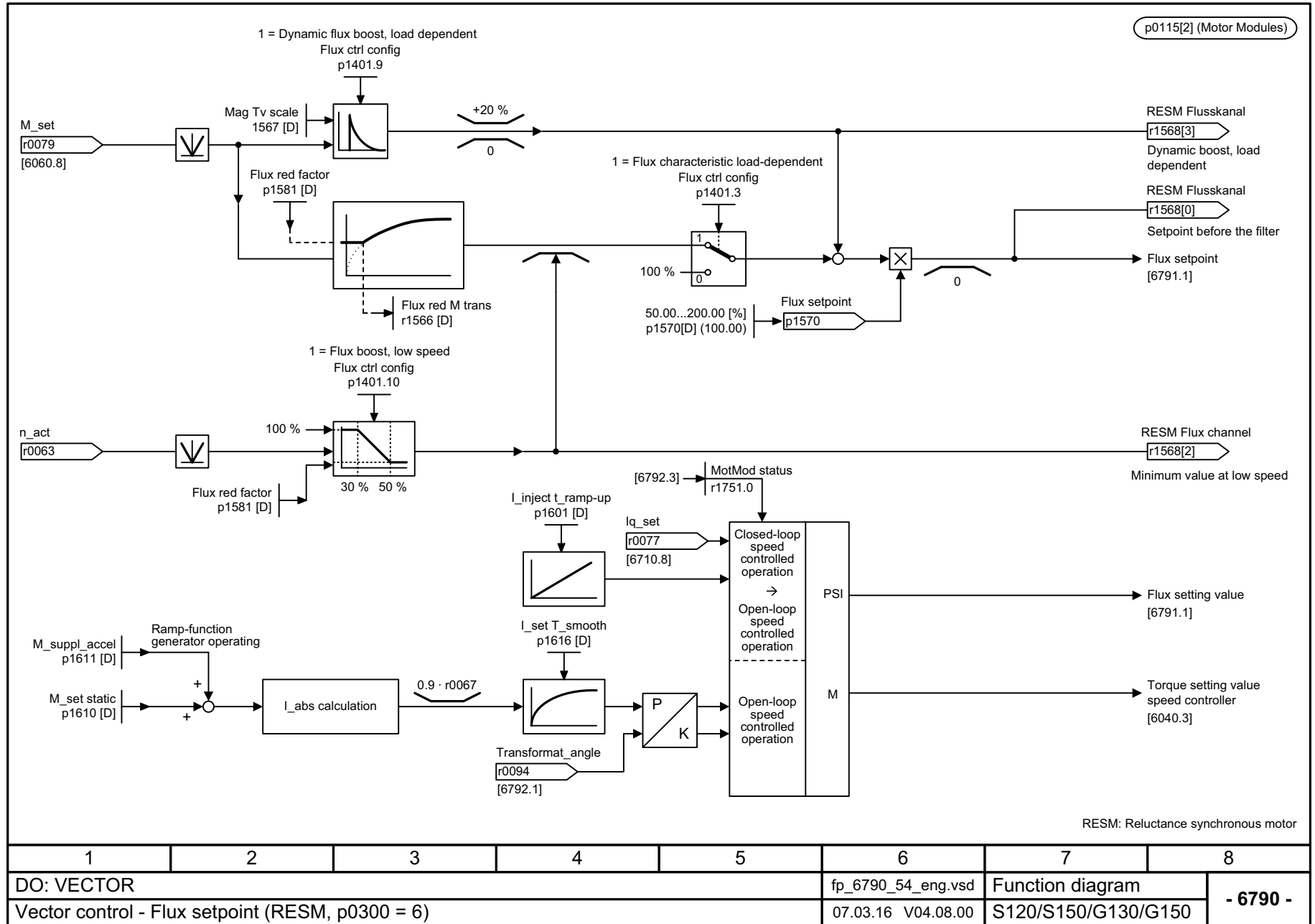
Fig. 3-258 6790 – Flux setpoint (RESM, p0300 = 6)
