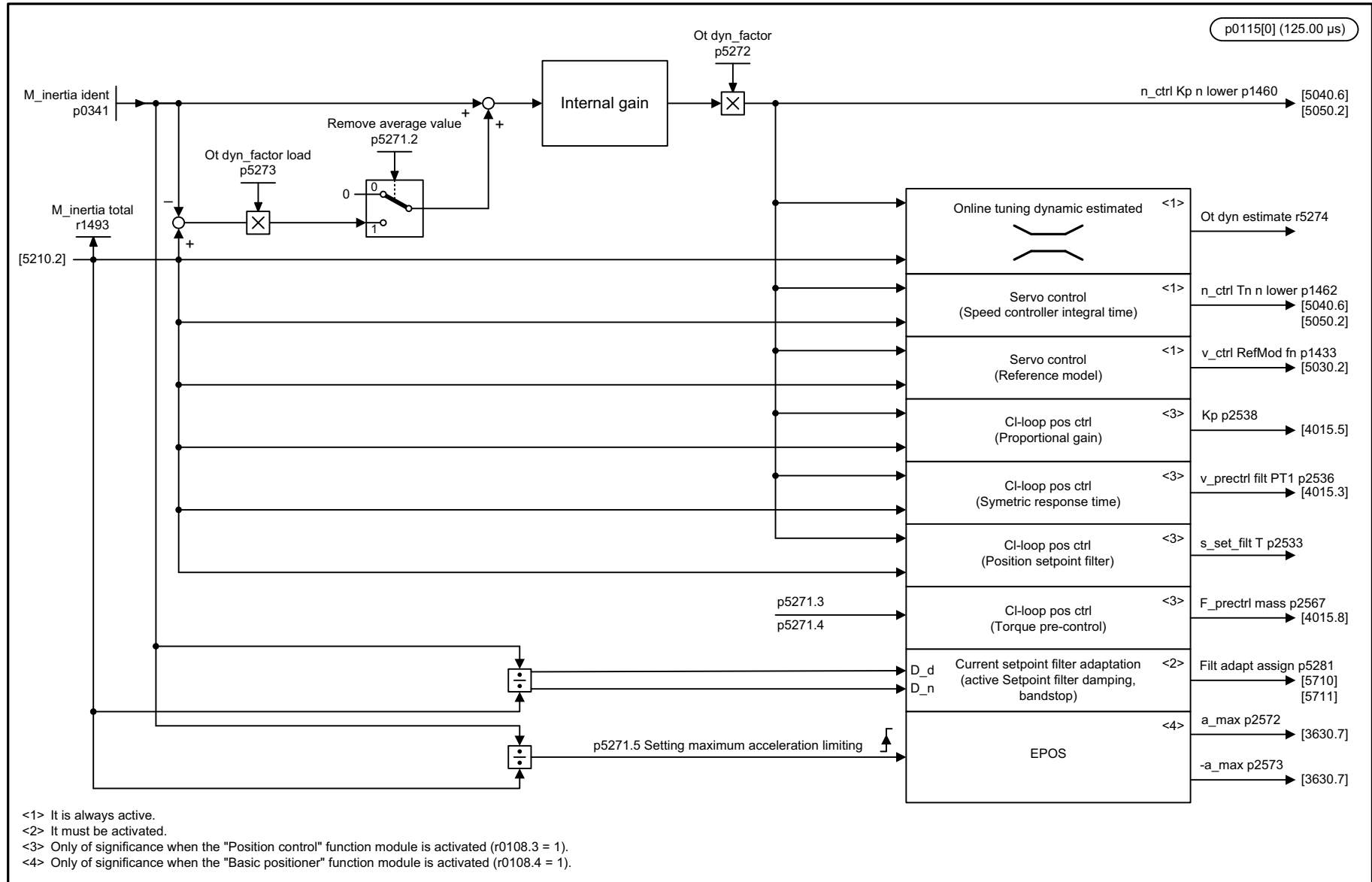
Fig. 3-208 5045 – Online tuning with activated moment of inertia estimator (r0108.10 = 1)
