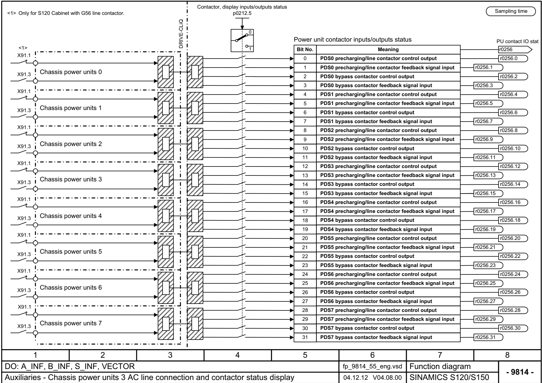
Fig. 3-395 9814 – Chassis power units, 3 AC line connection and contactor status display
