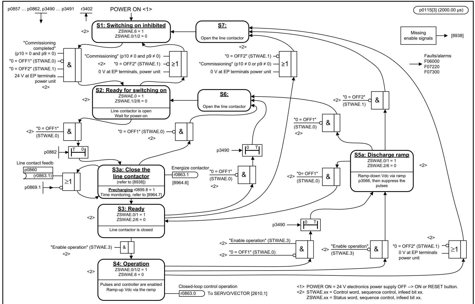
Fig. 3-337 8932 – Sequencer
