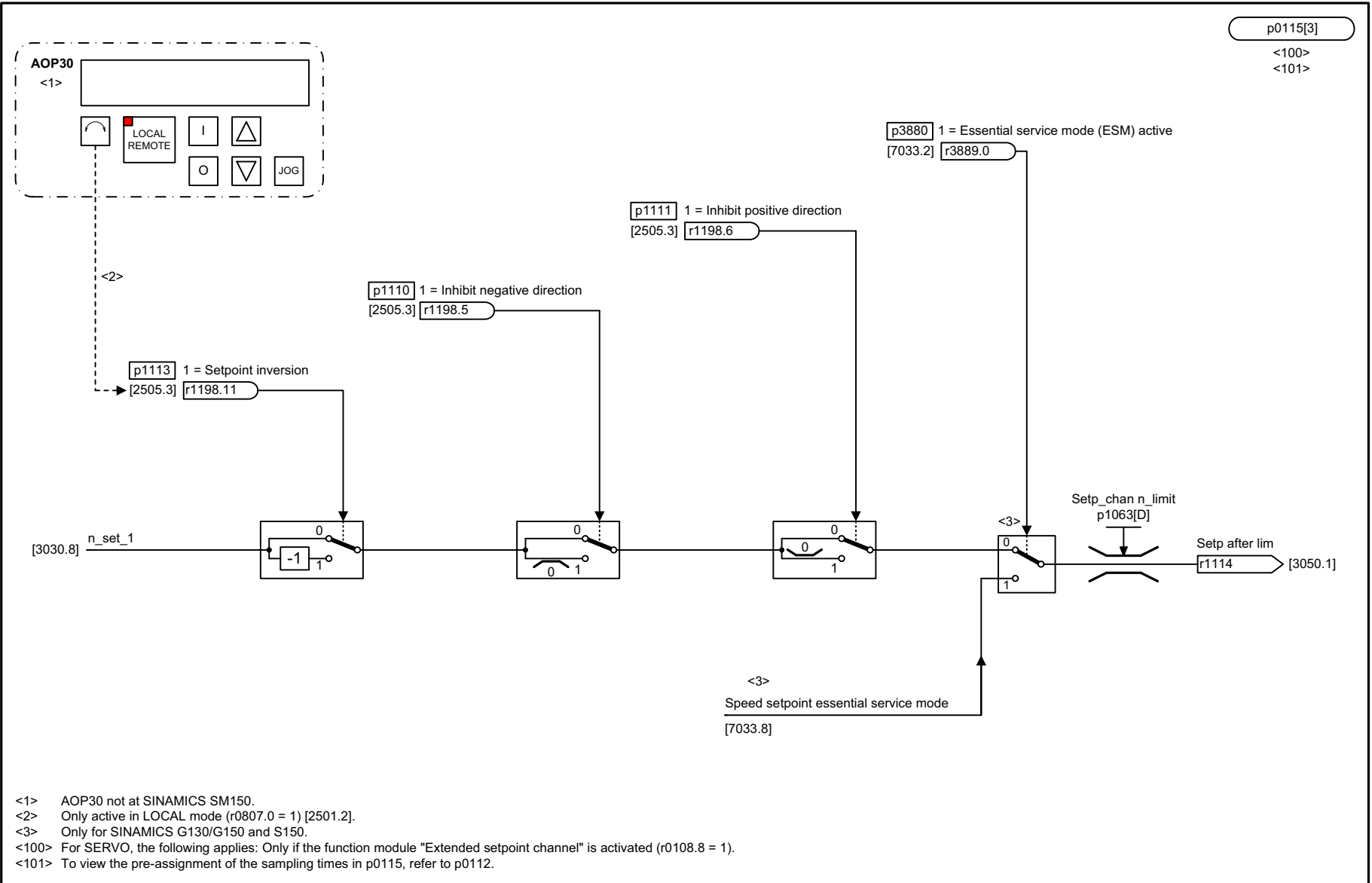
Fig. 3-155 3040 – Direction limitation and direction reversal
