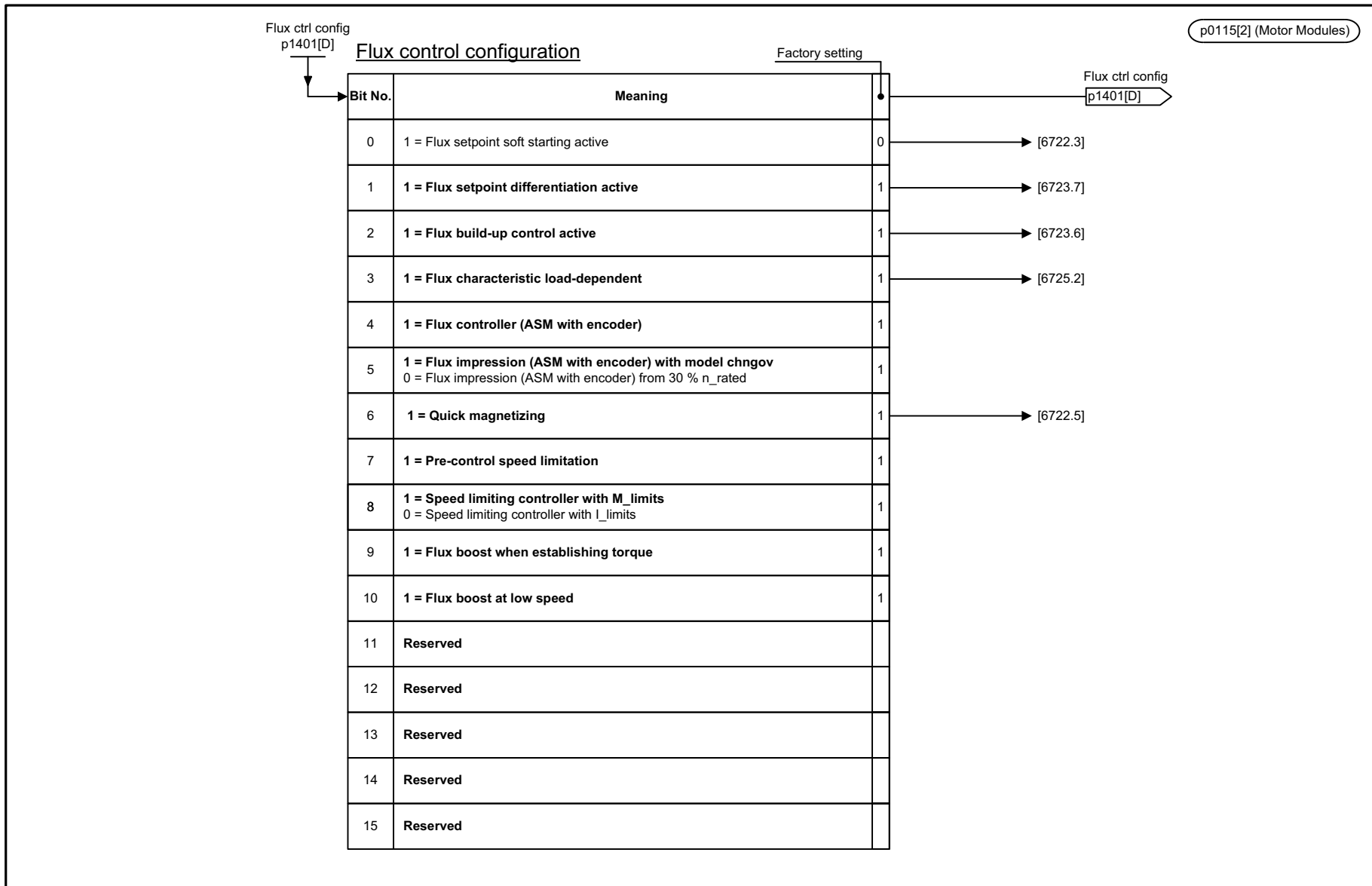
Fig. 3-240 6491 – Flux control configuration
