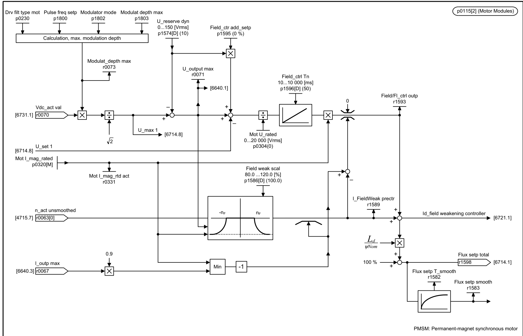
Fig. 3-250 6724 – Field weakening controller (PEM; p0300 = 2)
