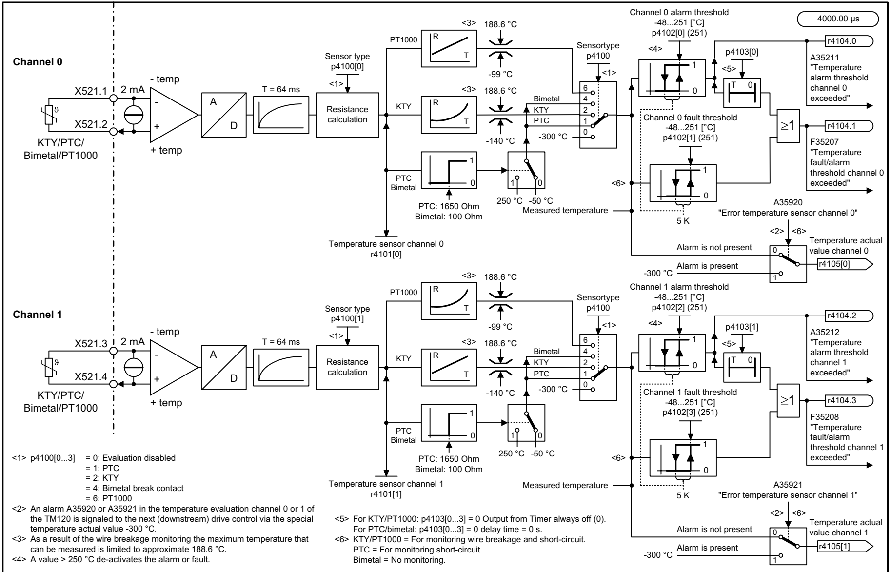
Fig. 3-374 9605 – Temperature evaluation channels 0 and 1 (KTY/PTC/bimetal)
