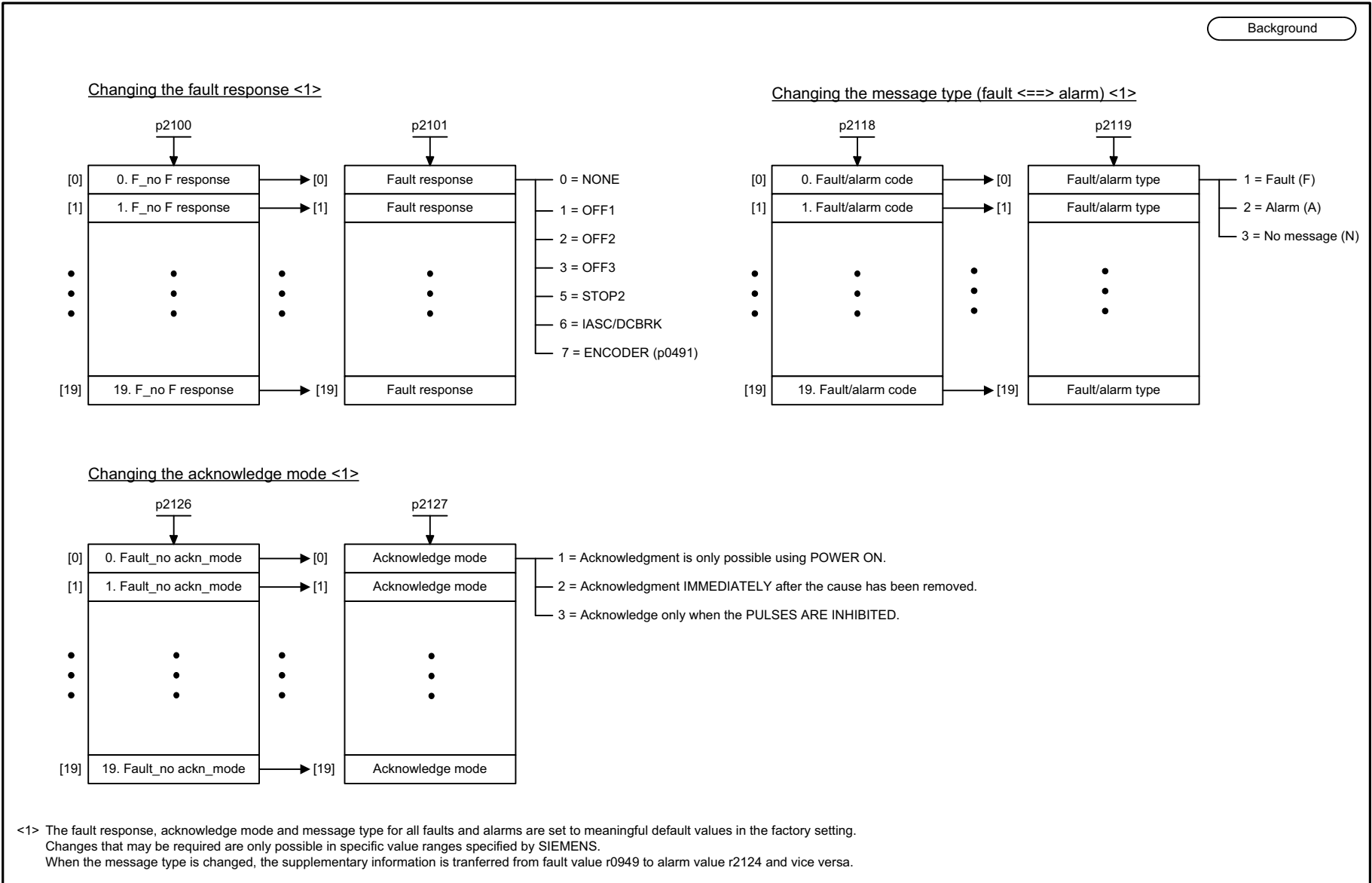
Fig. 3-308 8075 – Faults/alarms configuration
