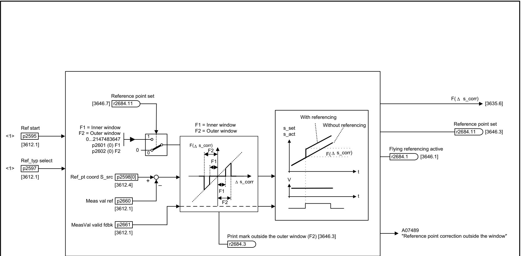
Fig. 3-165 3614 – Flying referencing mode (r0108.4 = 1) (p2597 = 1 signal)
