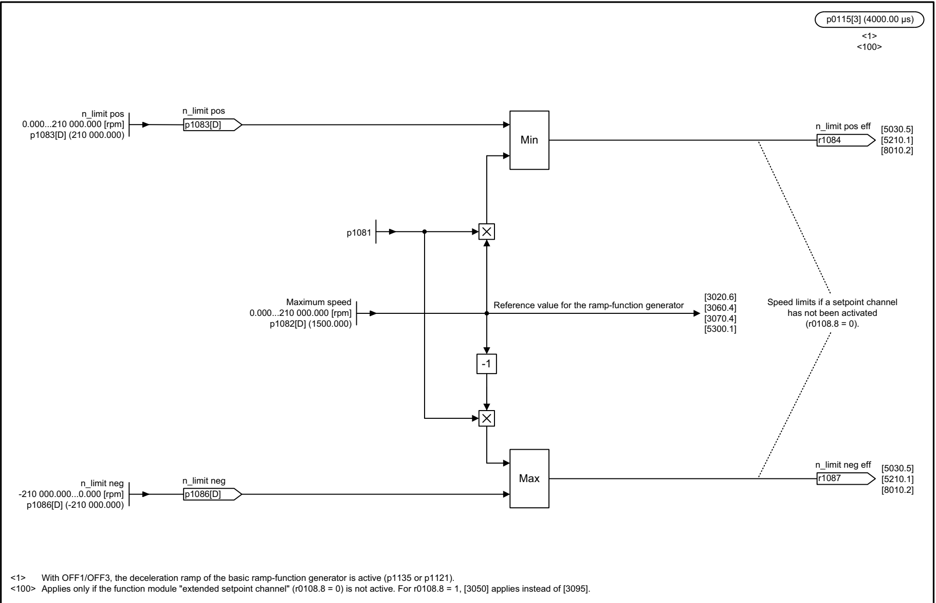
Fig. 3-162 3095 – Generation of the speed limits (r0108.8 = 0)
