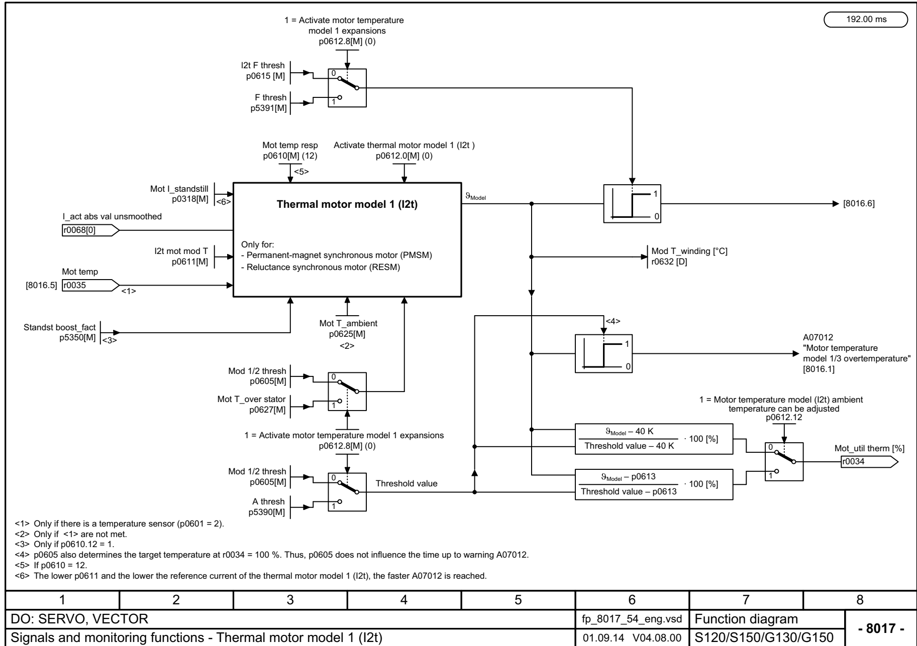
Fig. 3-298 8017 – Motor temperature model 1 (I2t)
