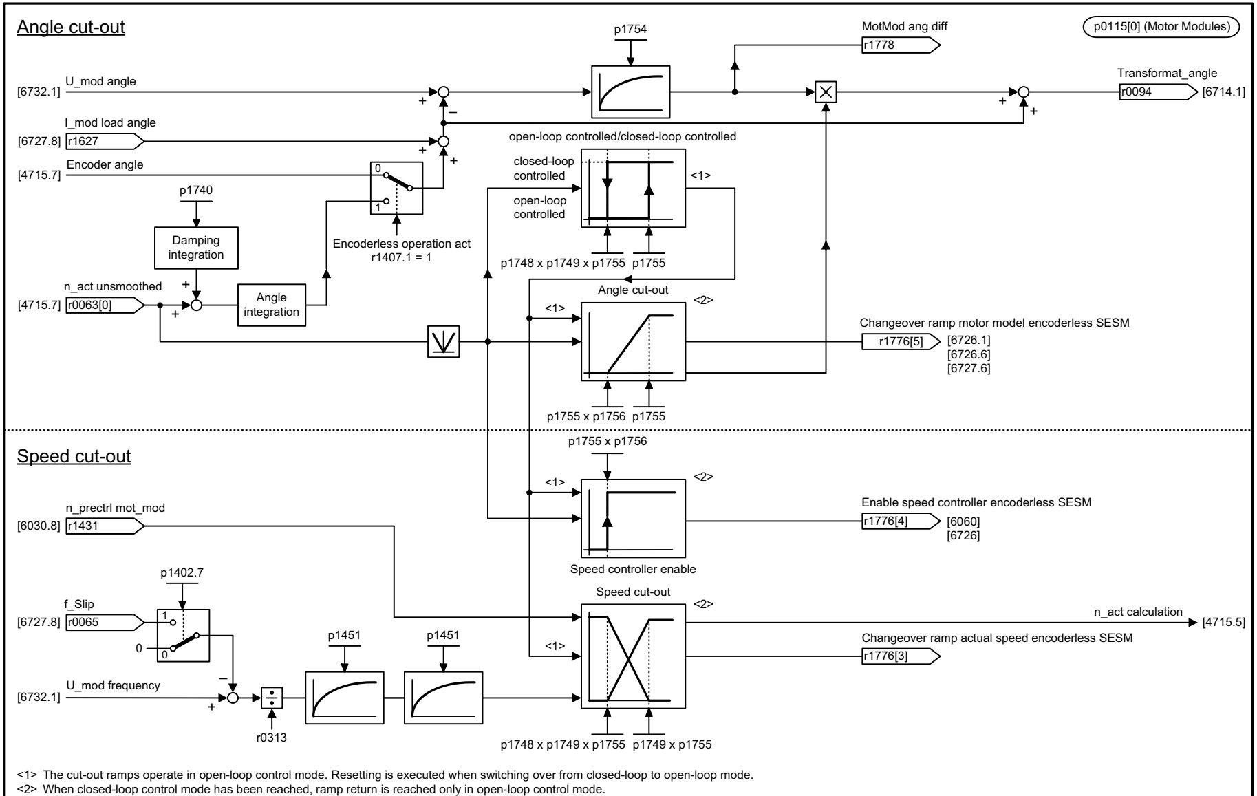
Fig. 3-257 6733 – Motor model selection (FEM and p1300 = 20, p0300 = 5)
