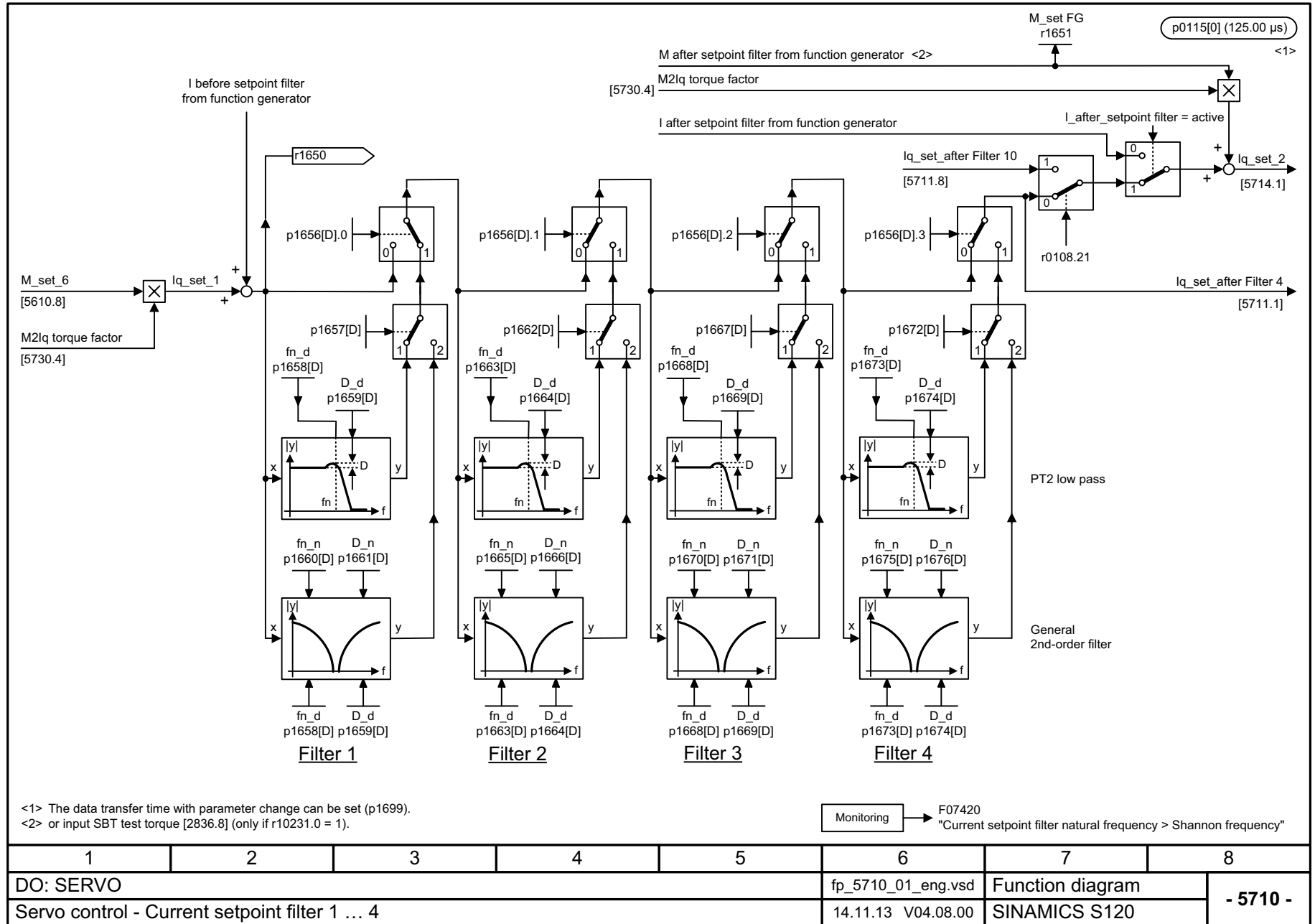
Fig. 3-222 5710 – Current setpoint filter 1 ... 4
