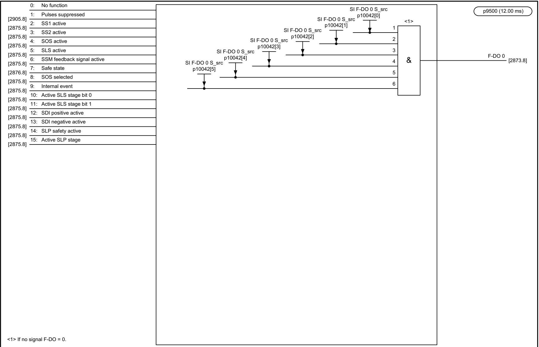
Fig. 3-136 2877 – CU310-2 assignment (F-DO 0)
