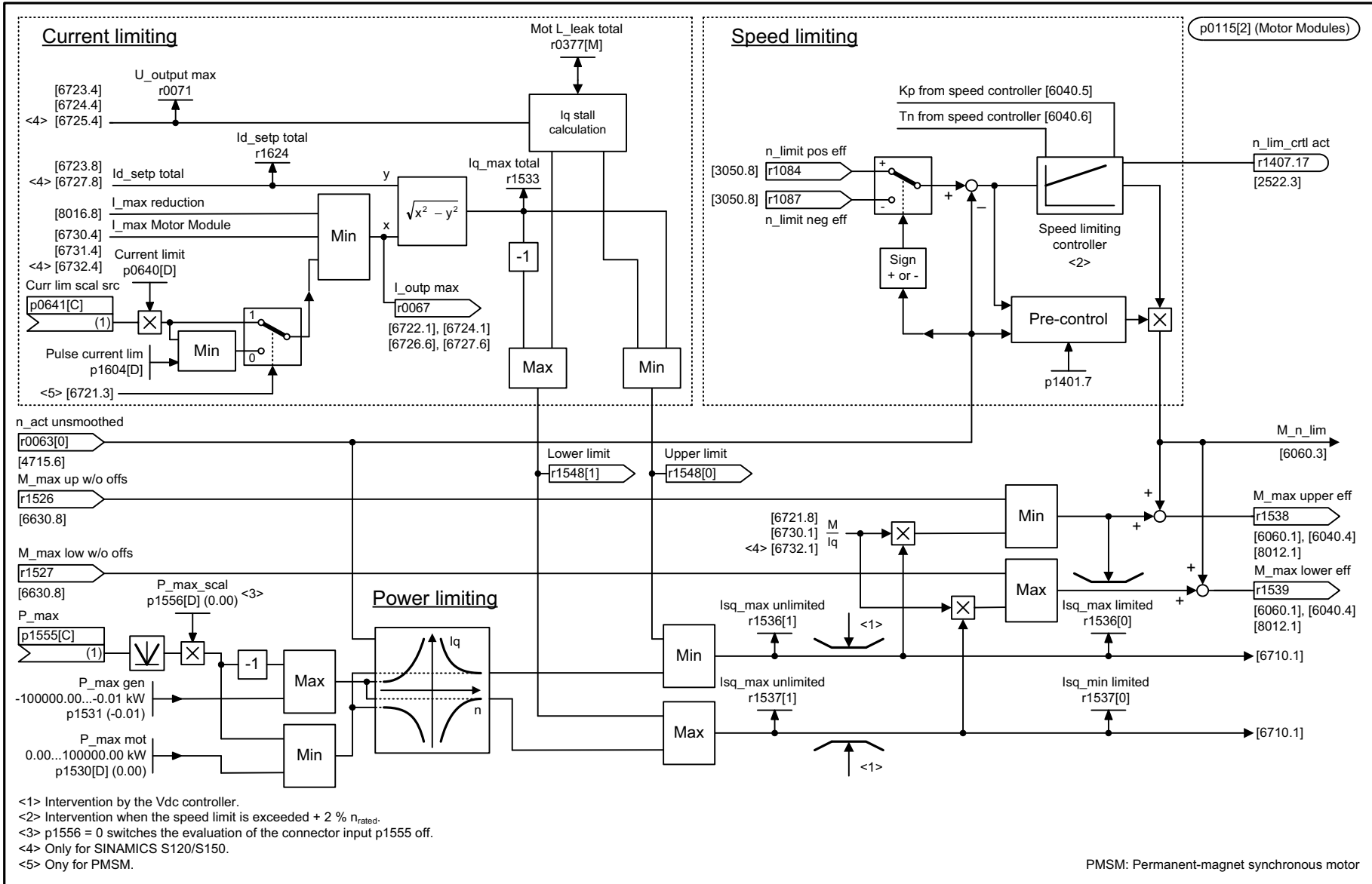
Fig. 3-243 6640 – Current/power/torque limits
