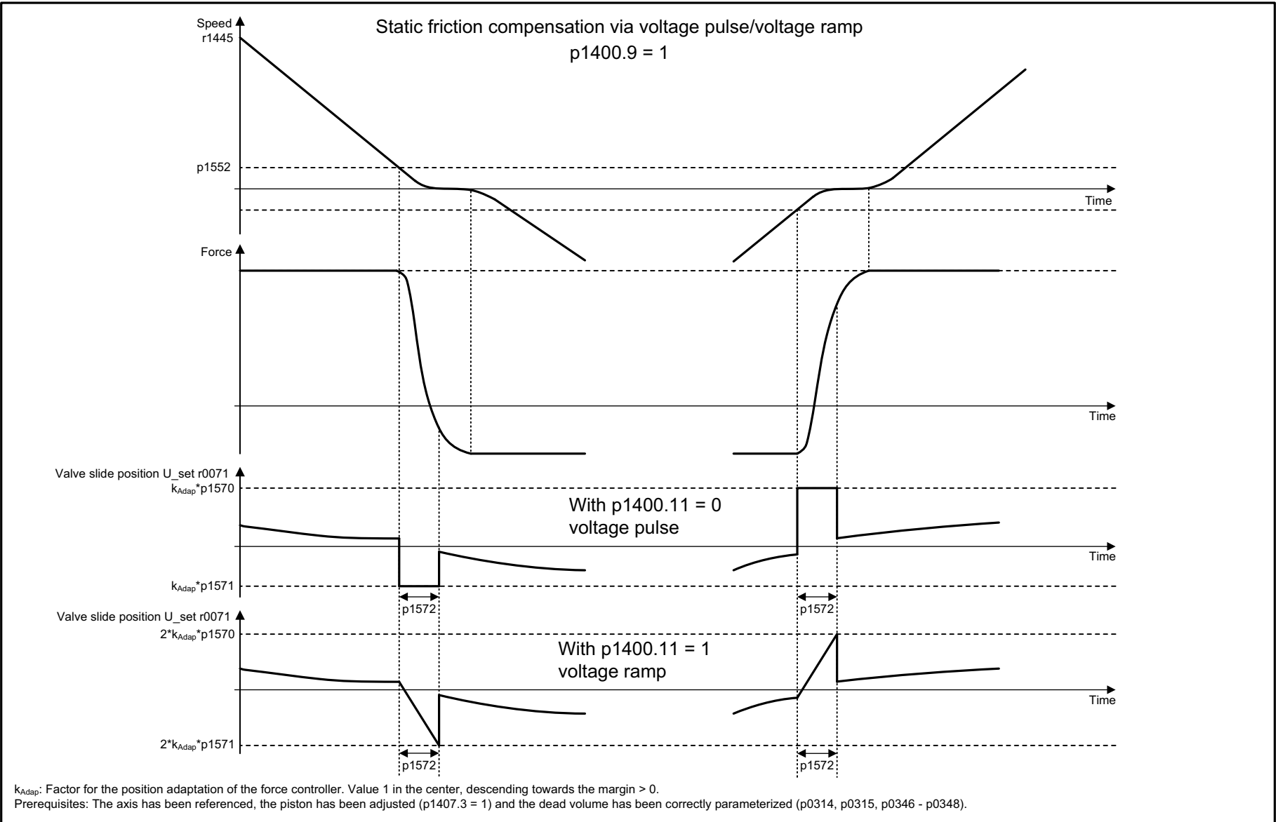
Fig. 3-198 4978 – Static friction compensation via voltage pulse / voltage ramp
