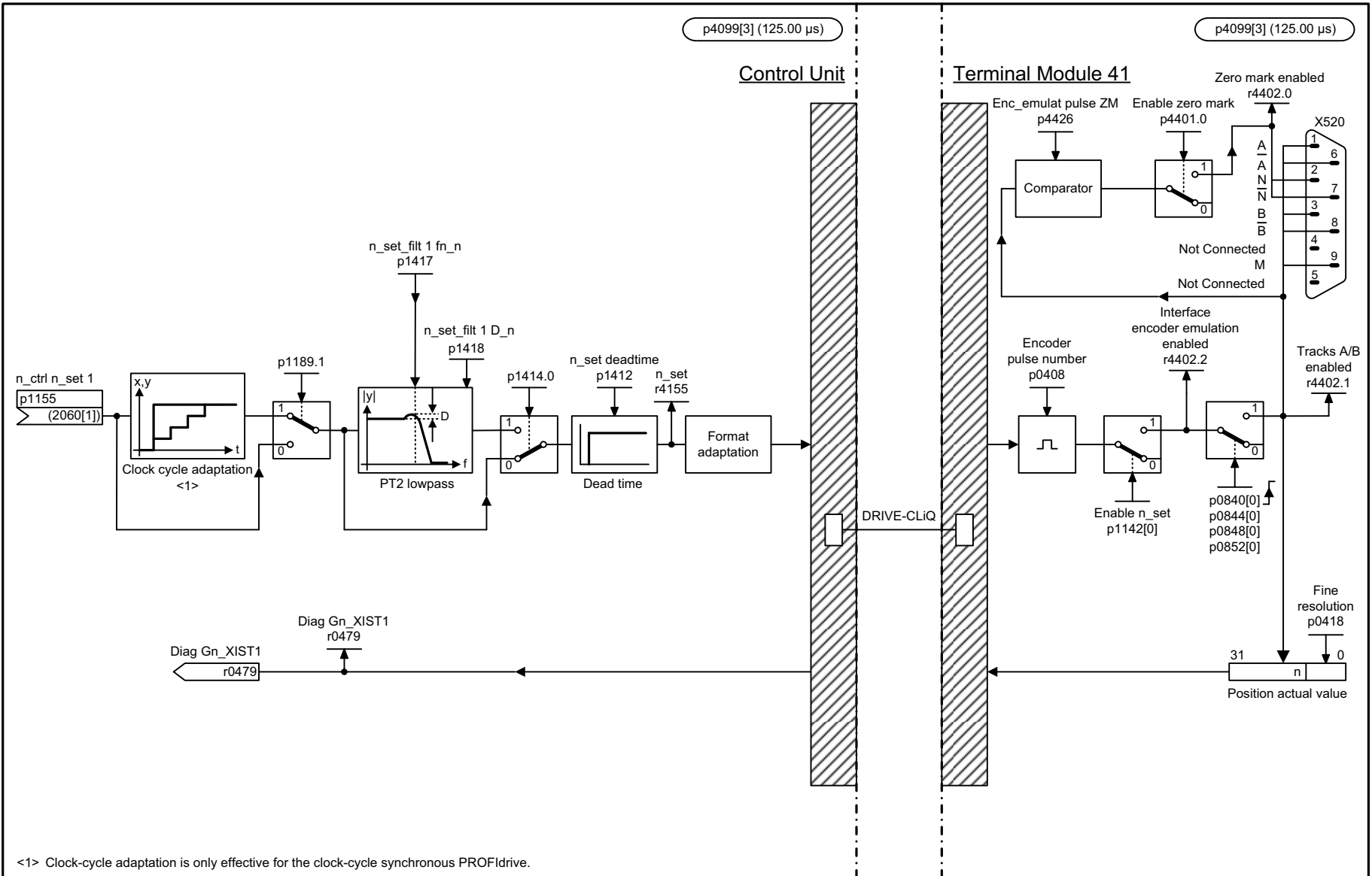
Fig. 3-384 9674 - Incremental encoder emulation (p4400 = 0)
