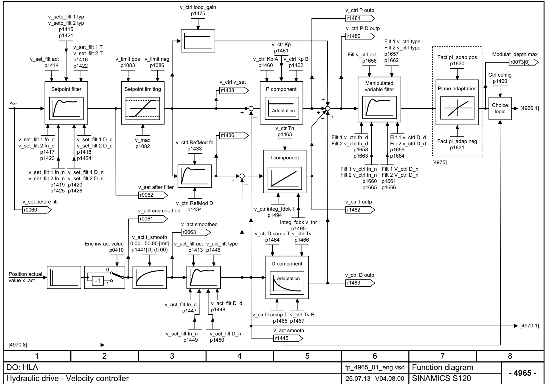
Fig. 3-193 4965 – Velocity controller
