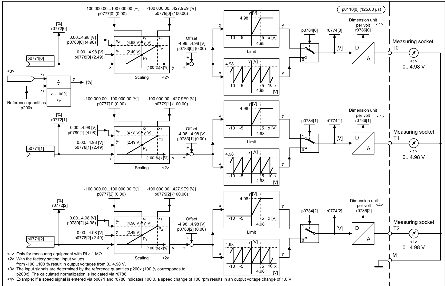
Fig. 3-309 8134 – Measuring sockets (T0, T1, T2)
