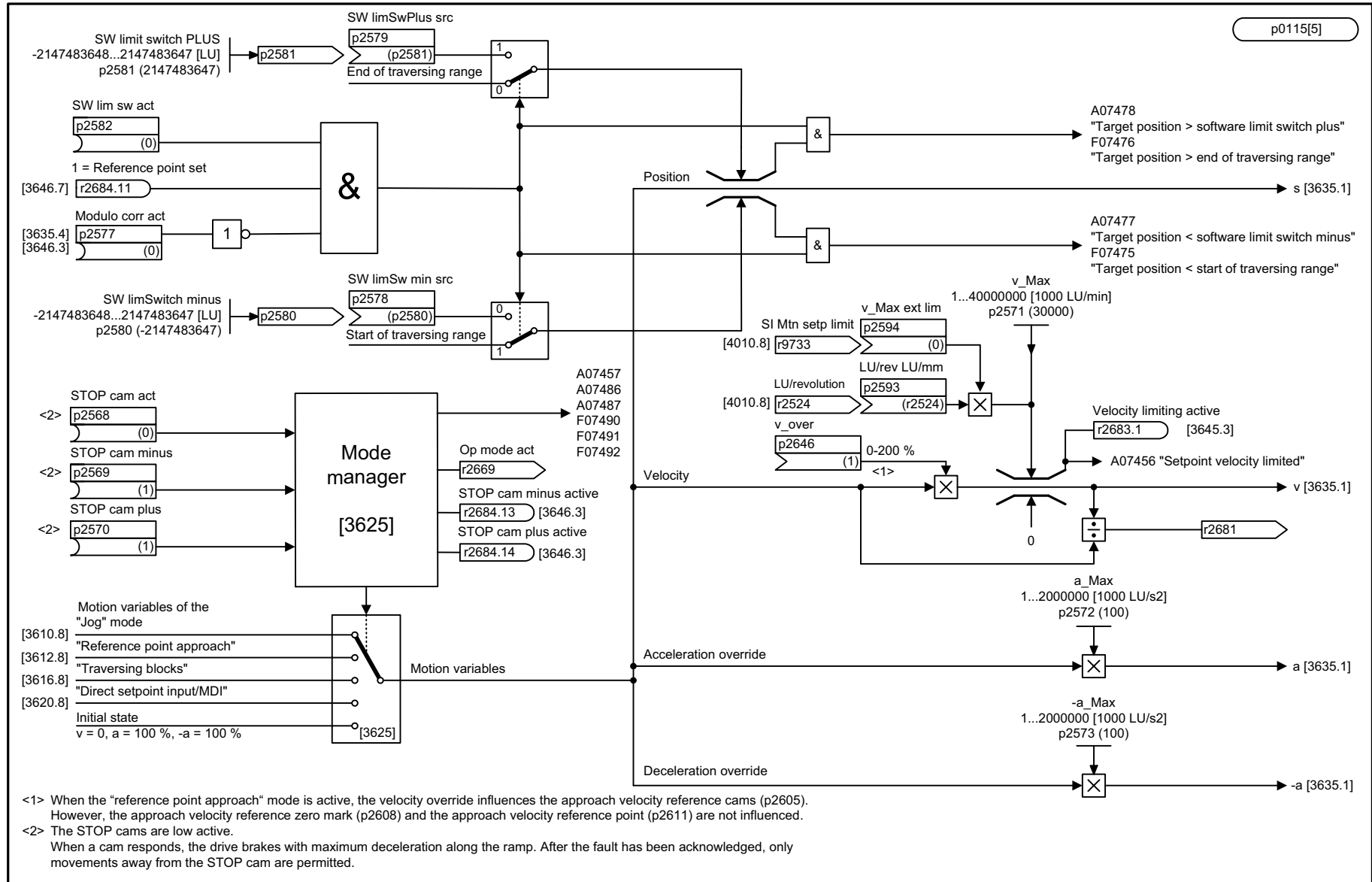
Fig. 3-172 3630 – Traversing range limits (r0108.4 = 1)
