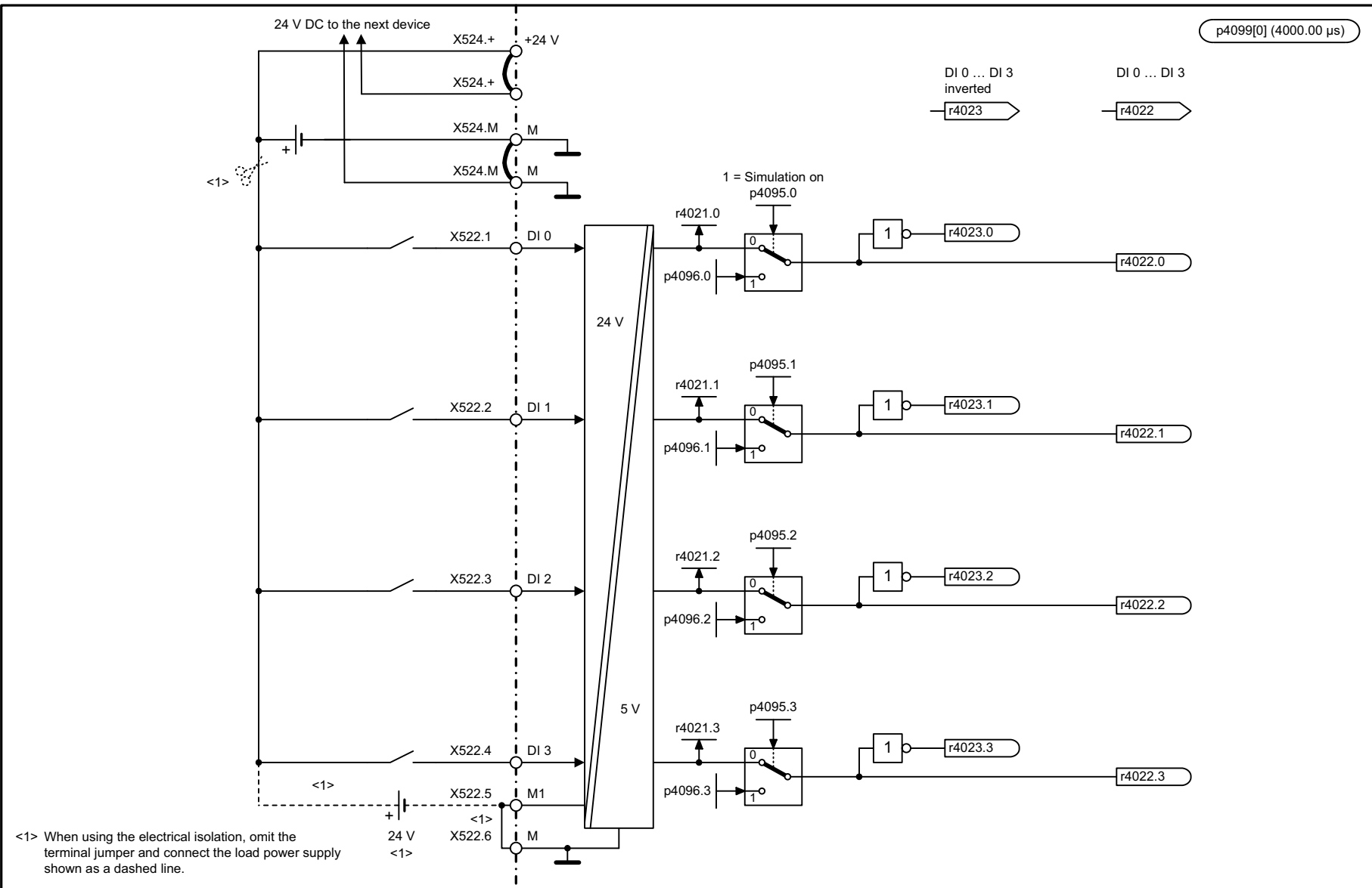
Fig. 3-380 9660 – Digital inputs, electrically isolated (DI 0 ... DI 3)
