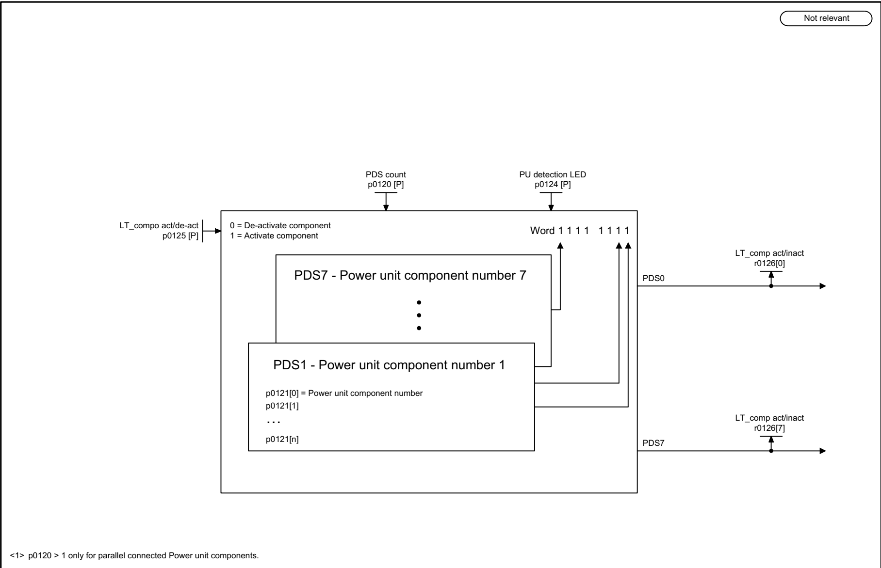
Fig. 3-316 8580 – Power unit Data Sets (PDS)
