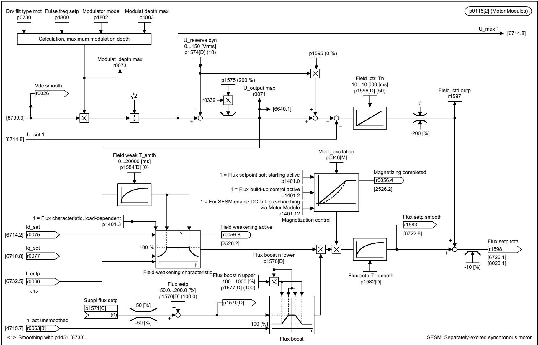
Fig. 3-251 6725 – Flux setpoint, field weakening controller (FEM, p0300 = 5)
