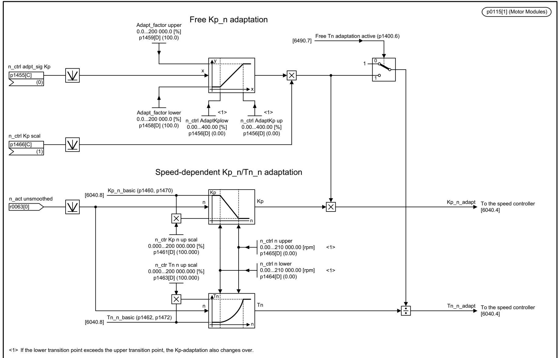
Fig. 3-232 6050 – Speed controller adaptation (Kp_n/Tn_n adaptation)
