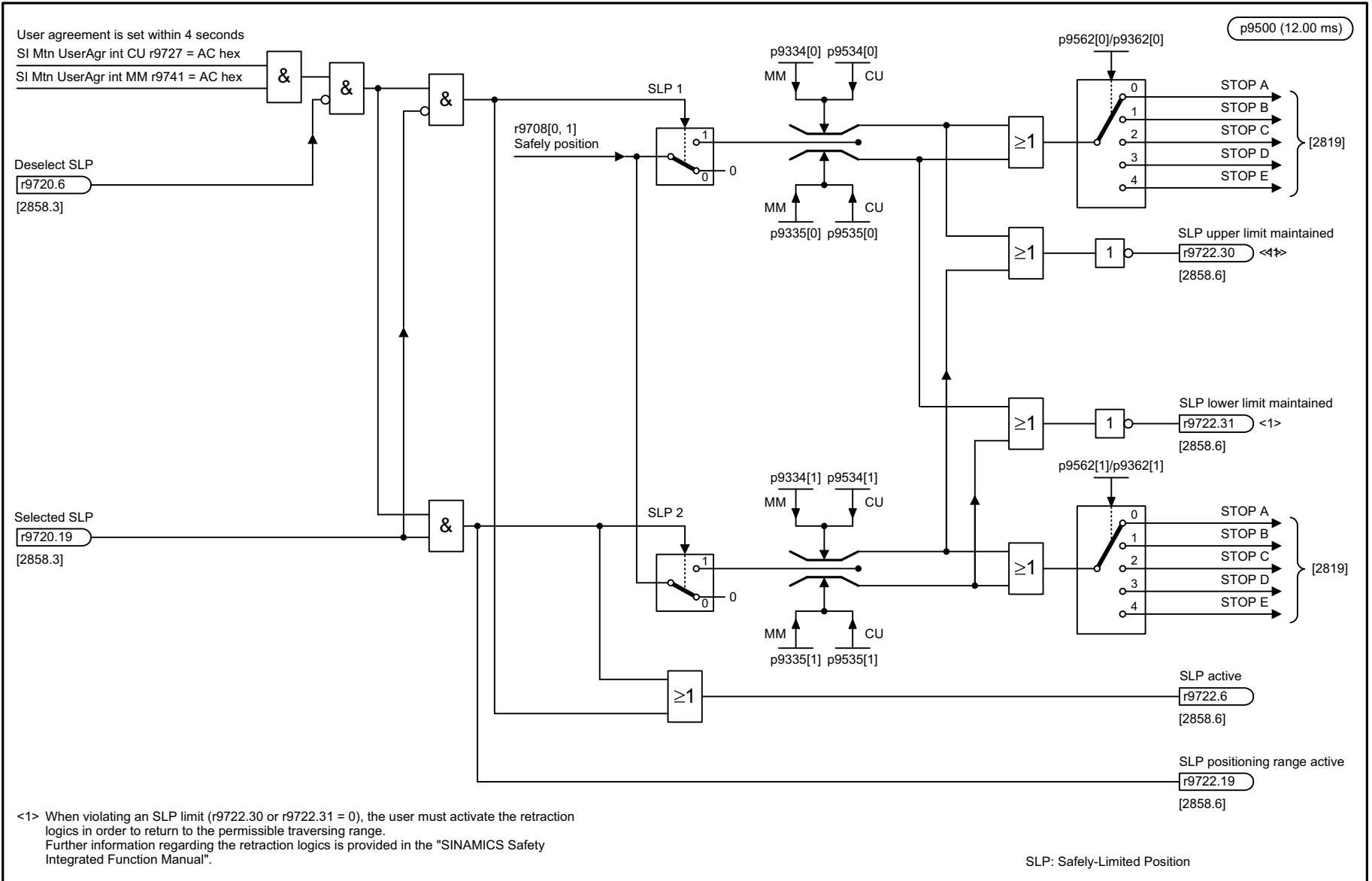
Fig. 3-122 2822 - SLP (Safely Limited Position)
