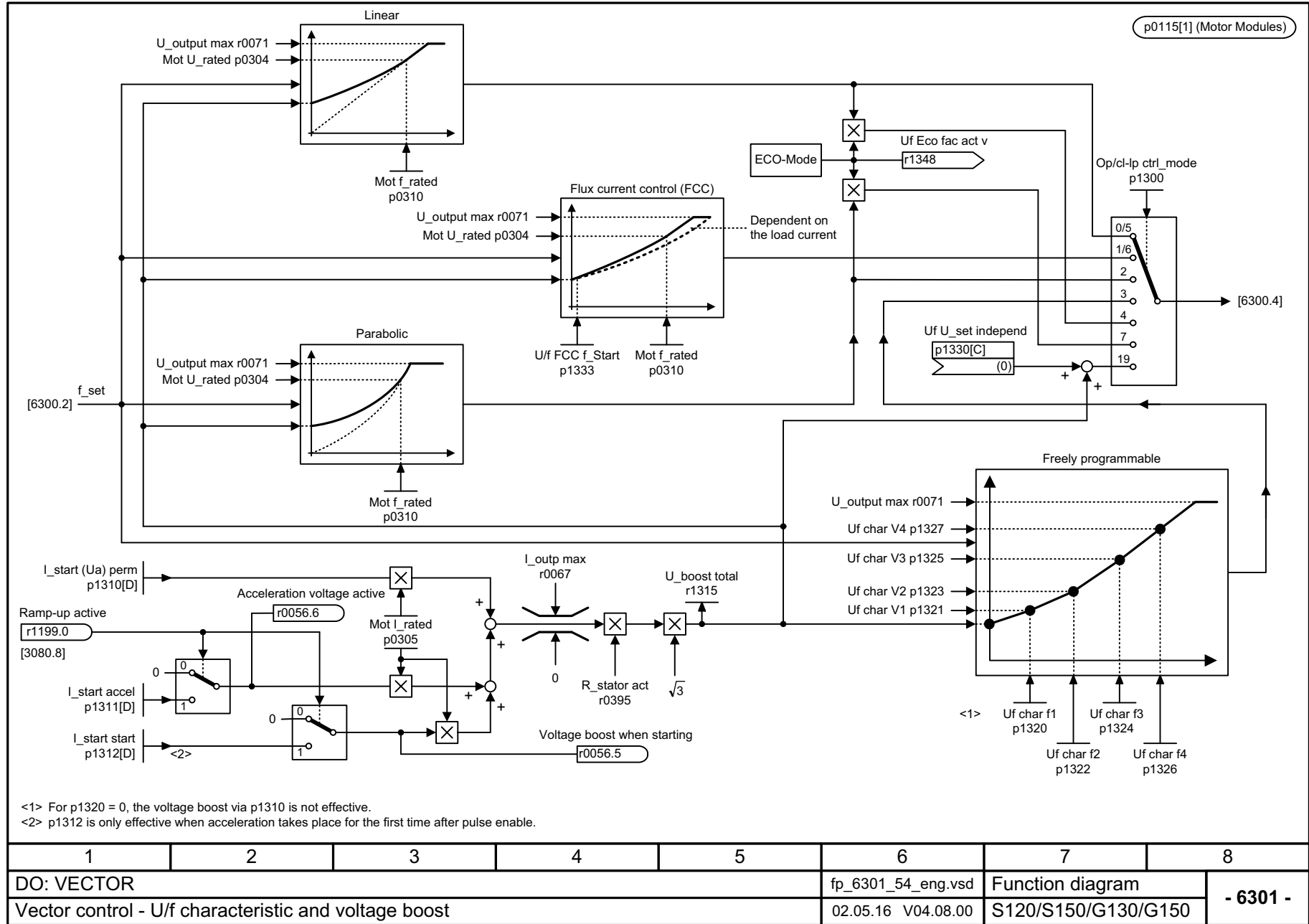
Fig. 3-236 6301 – U/f characteristic and voltage boost
