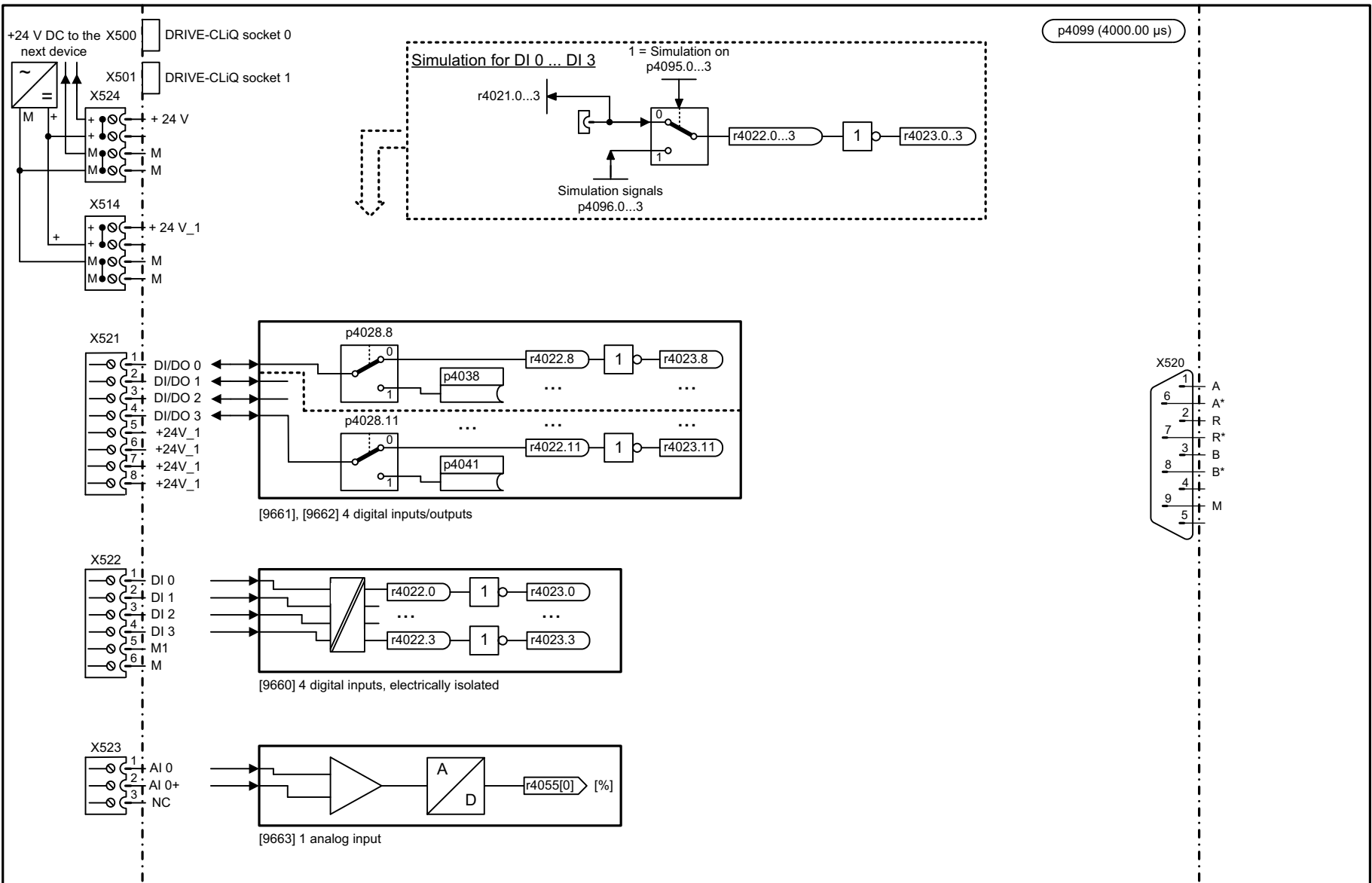
Fig. 3-379 9659 – Overview
