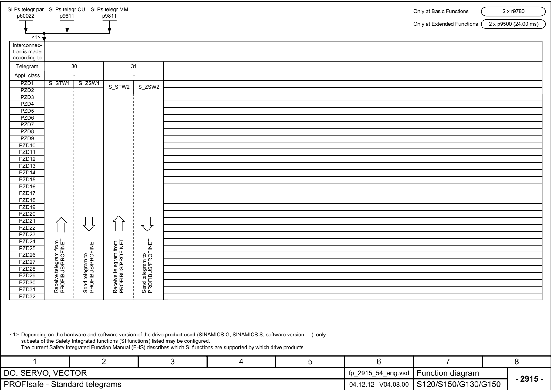
Fig. 3-149 2915 – Standard telegrams
